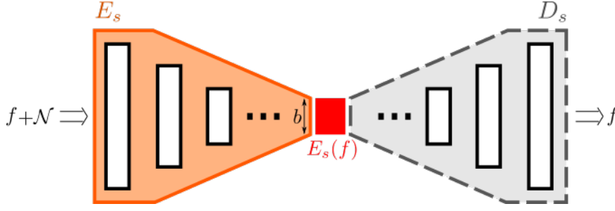
Figure 3.2: Source Autoencoder Architecture. This architecture finds a latent space representation ( E_s(f) ) of source task s . Every fully connected layer is followed by a batch normalization layer and a LRELU layer. These three layers are represented as a single white block for visual clarity. Block size is usually half of its predecessor to approximate wanted output size of encoder b . Added noise \mathcal{N} and batch normalization layers help for more robust latent representation of f , E_s(f) .
