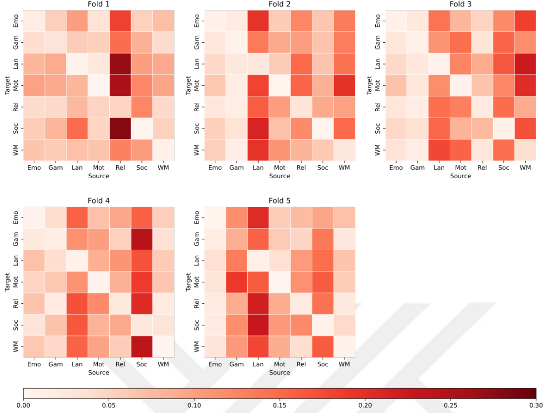
Figure 4.3: Generated Transferability Graphs per Fold. For visual clarity, the distance formula e^{-20x} is used for every cell x . Lower values mean better expected transferability. Note that apart from using the same cognitive task as both source and target having the best expected transferability, there is no common structure between folds. Although general overlap between resulting transferability graphs are sparse, it can be seen that relative expected transferring performance from the same source have similar characteristics throughout the folds.
