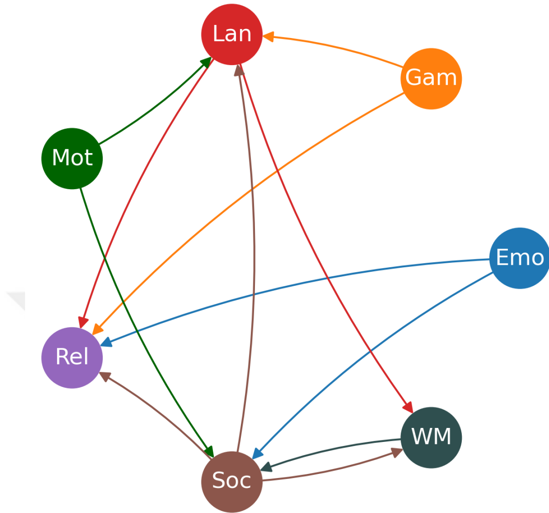
Figure 4.13: Resulting Global Transferability Graph with at least 2 Transferability Graph Suggestions. Majority of connections suggested by the average confusion graph also suggested by the transferability graphs except working memory as the source cognitive task which has only one transference in the global transference graph as the source cognitive task. All Connections which social cognition is the source cognitive task suggested by the average confusion graph on the other hand also suggested by the transferability graphs. For all other cognitive tasks as source cognitive task, 2 connection out of 3 suggested by the average confusion graph are selected as the connection in the global transferability graph.
