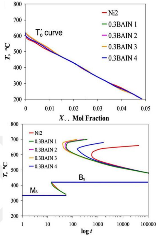
Figure 2.14. a) T_0' curve and b) TTT diagram of the designed steels [52].
