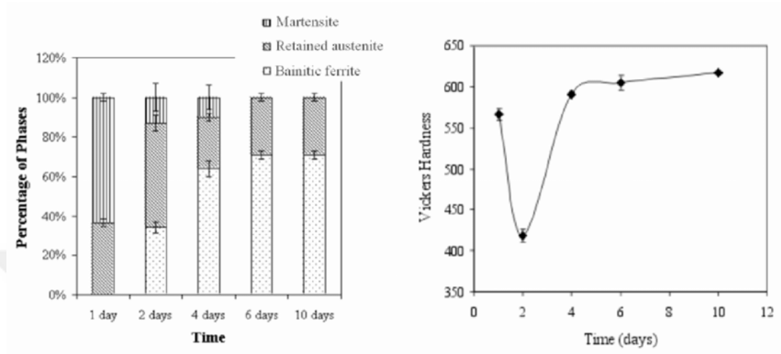
Figure 2.7. The changes of phases and hardness values in bainitic steel isothermal treated 200 °C for 1 to 10 days.
