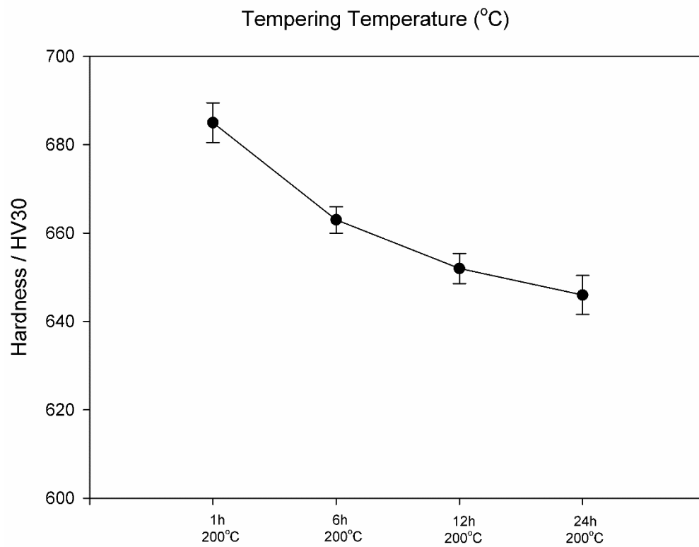
Figure 4.26. Hardness vs. tempering temperature of C-Mn-Si alloy.
