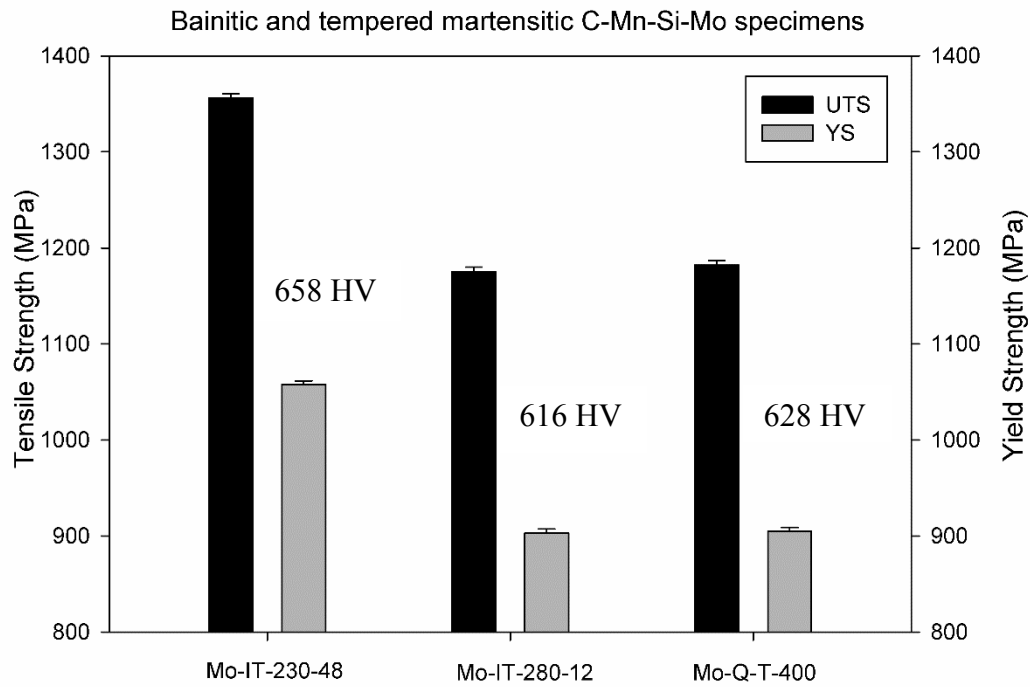
Figure 4.29. Comparison of tensile strength and yield strength values of bainitic and tempered martensitic C-Mn-Si-Mo specimens.
