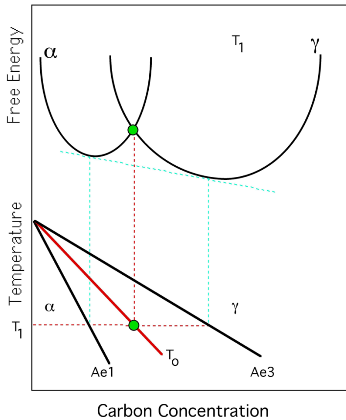
Figure 2.8. Definition of the T_0 curve [18].
