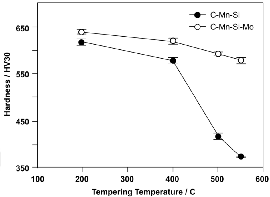
Figure 4.25. Hardness values of bainitic C-Mn-Si and bainitic C-Mn-Si-Mo alloy.
