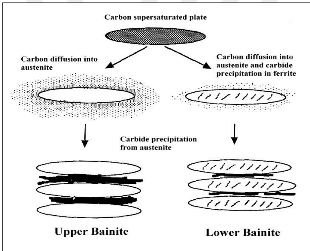
Figure 2.3. A schematic view of carbon diffusion during the bainite transformation [15].
