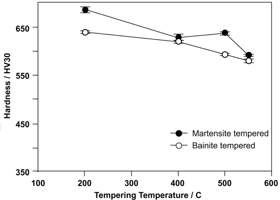
Figure 4.24. The hardness results of martensitic and bainitic C-Mn-Si-Mo specimens.
