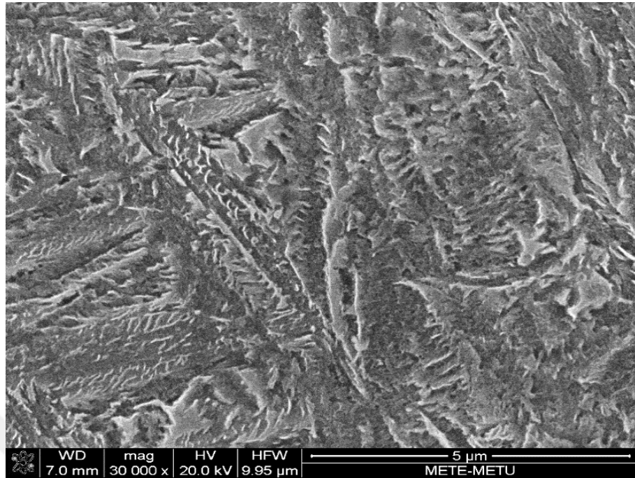
Figure 4.21. SEM micrograph of Mo-IT-280-1.
