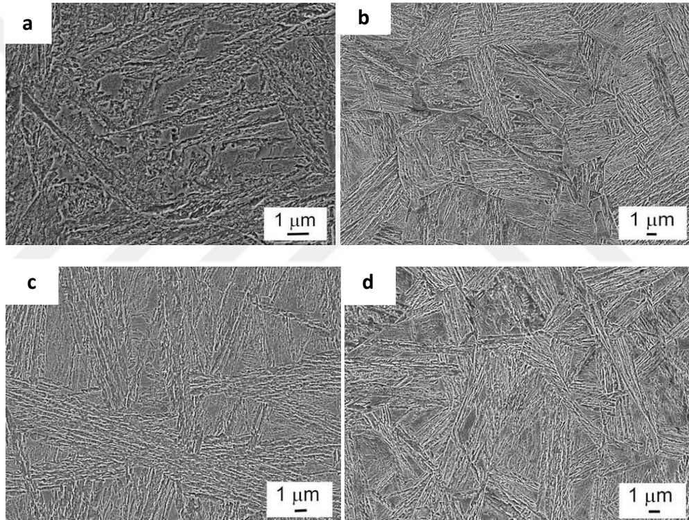
Figure 2.13. SEM micrographs from 0.3BAIN1 to 0.3BAIN4 air cooled (a) 600°C, (b:d) 500°C, respectively.
