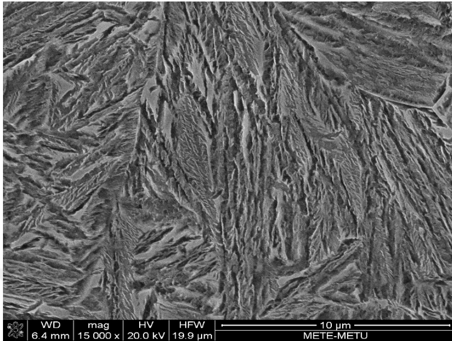
Figure 4.11. SEM micrograph of IT-300-1.
