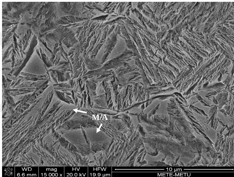
Figure 4.10. SEM micrograph of IT-300-1/4.
