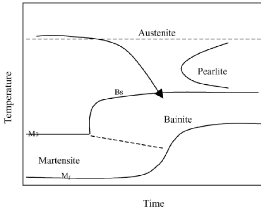
Figure 2.5. A schematic view of CCT diagram.
