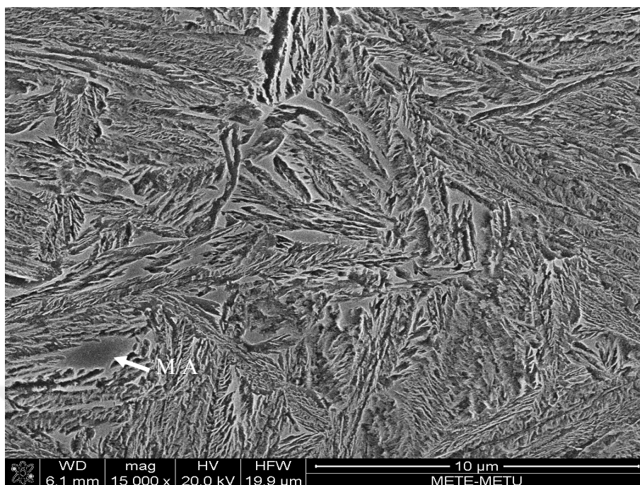
Figure 4.8. SEM micrograph of IT-250-1.
