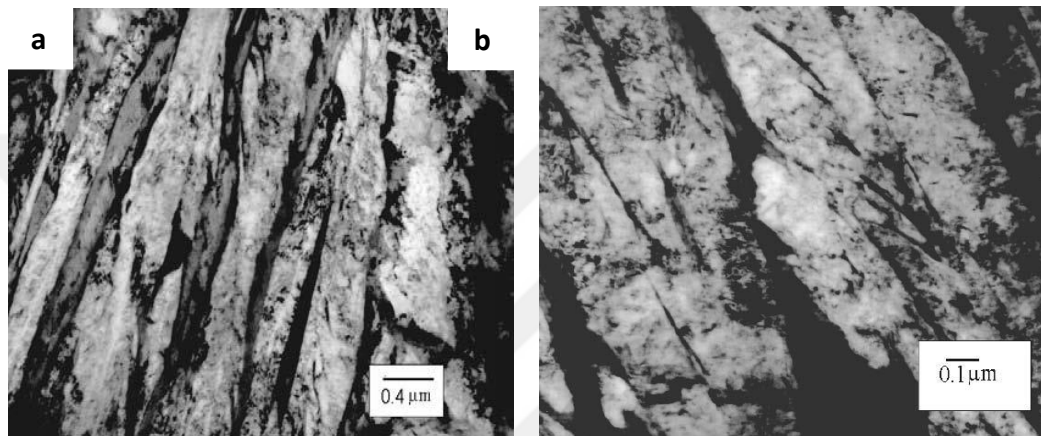
Figure 2.12. Transmission electron micrographs of bainitic ferrite and retained austenite films (a) Ni1 alloy; (b) Ni2 alloy [8].
