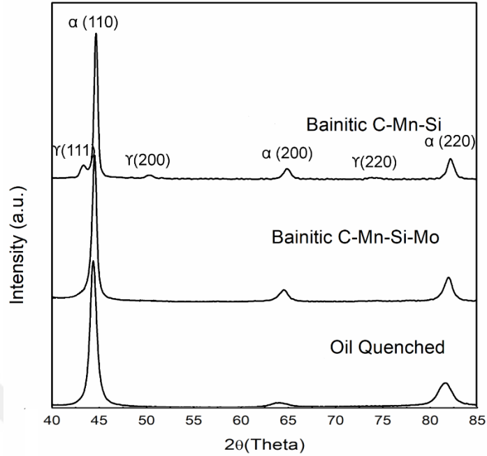
Figure 4.33. Comparison of XRD patterns of Q, Mo-IT-230-48, and IT-250-12 specimens. In IT-250-12 specimens, austenite peaks \gamma (111), \gamma (200), \gamma (220) are observed.
