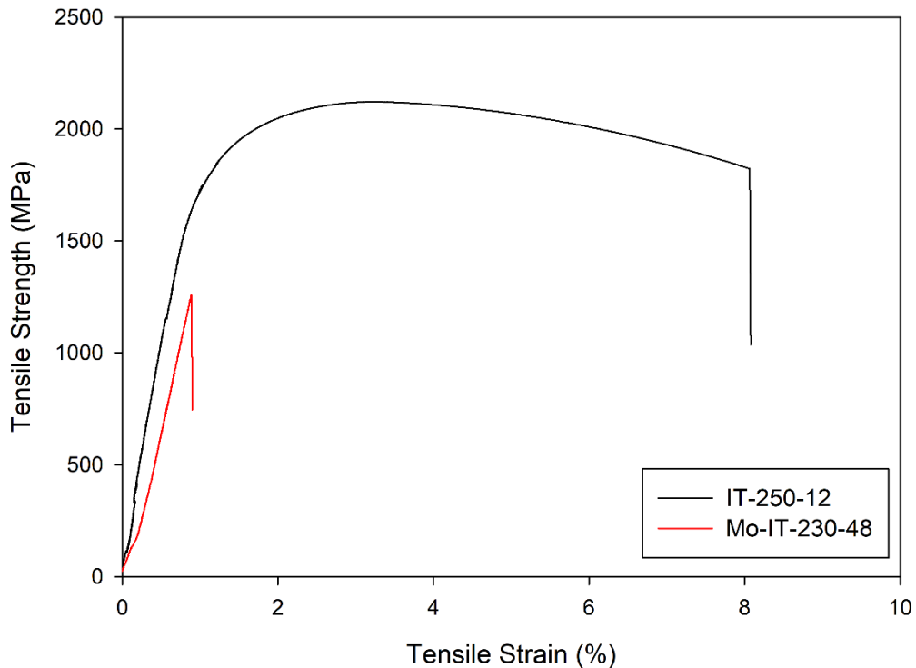
Figure 4.28. Stress strain curves of IT-250-12 and Mo-IT-230-48 specimens.
