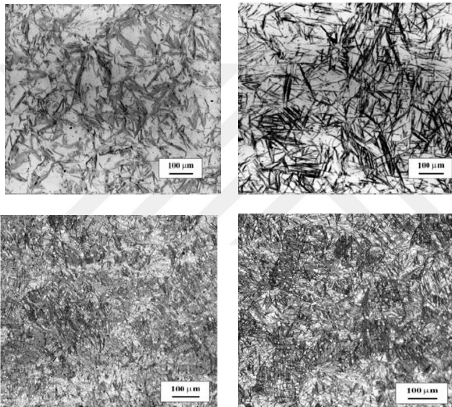
Figure 2.6. Optic micrographs of the bainitic steel at 200°C (a) for 1 day, (b) for 2 days, (c) for 4 days and (d) for 6 days [40].
