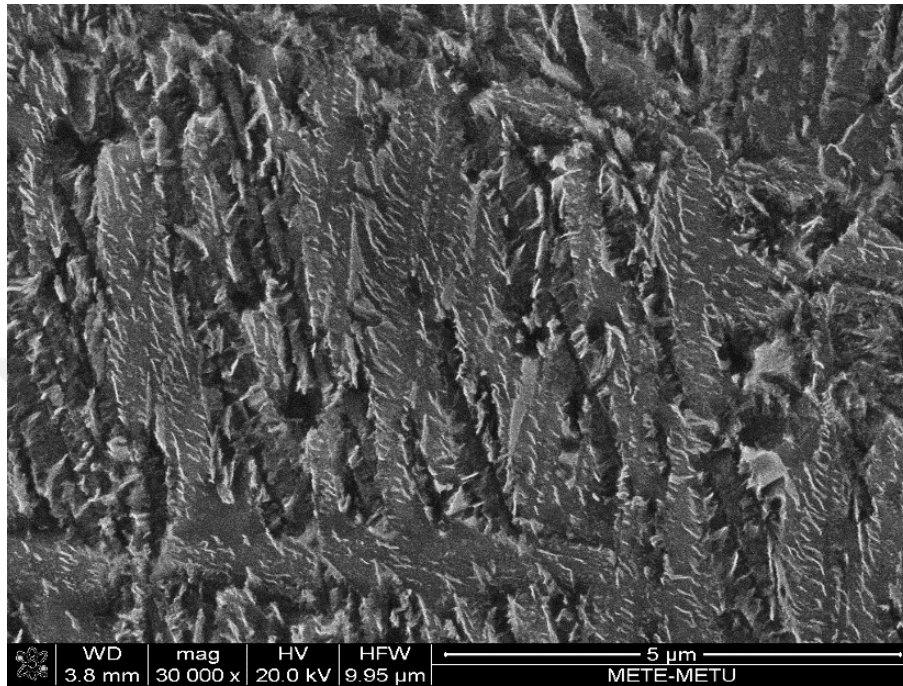
Figure 4.35. SEM micrograph of Mo-IT-280-12. Very thin, elongated carbide precipitation within and between the sheaves can be seen (white precipitates).
