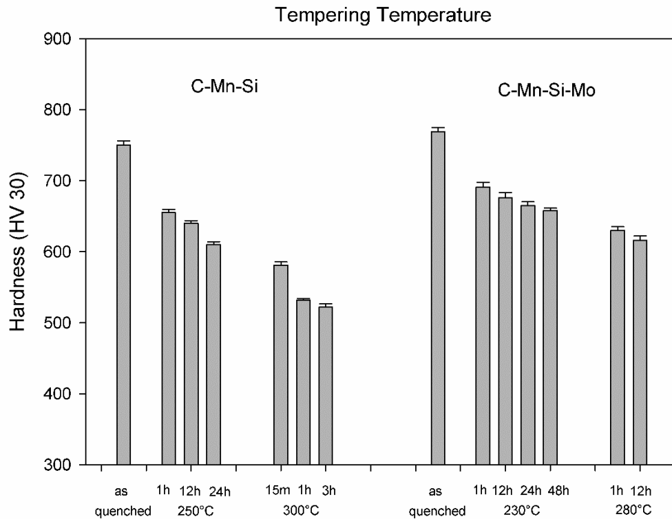
Figure 4.30. Hardness values of the isothermal treated C-Mn-Si and C-Mn-Si-Mo alloys.
