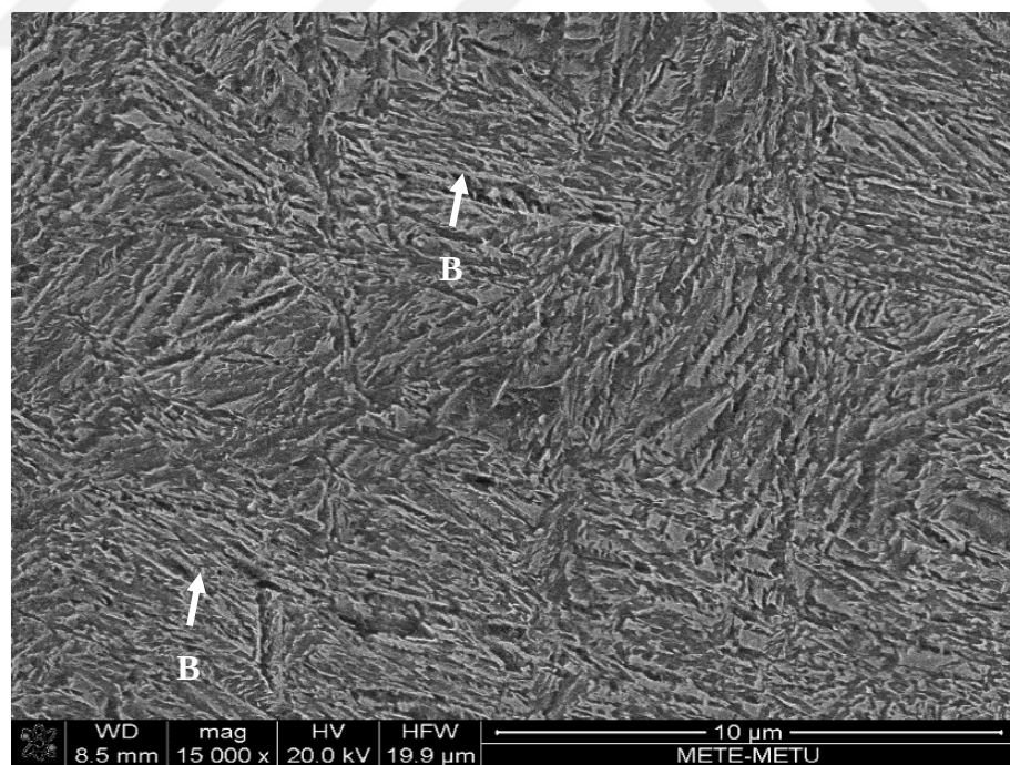
Figure 4.18. SEM micrograph of Mo-IT-230-12.
