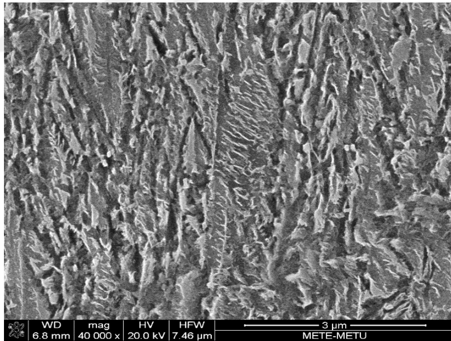
Figure 4.20. SEM micrographs of Mo-IT-230-48.
