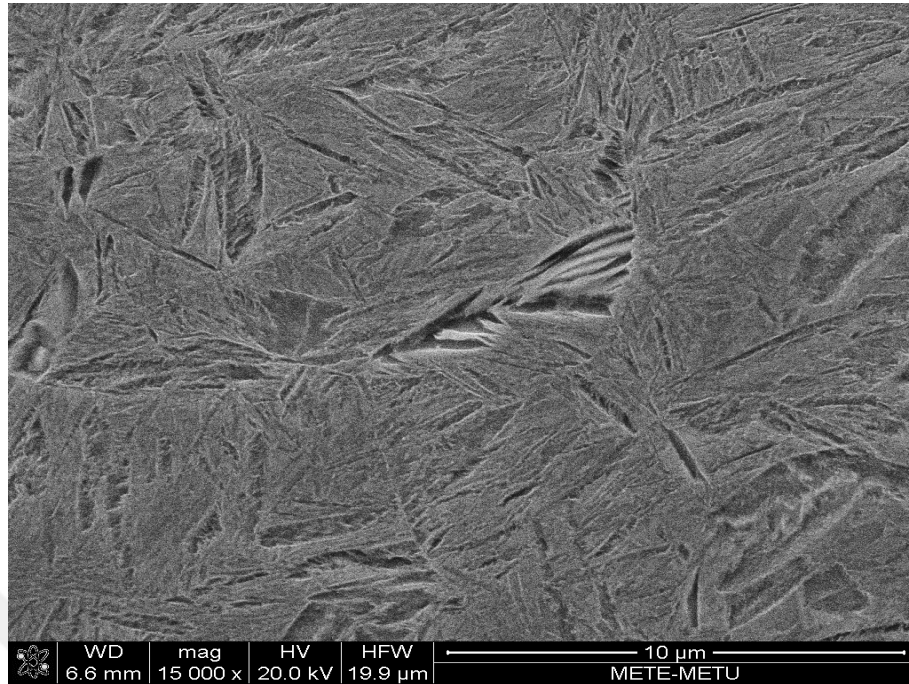
Figure 4.5. SEM micrograph of IT-200-1h.
