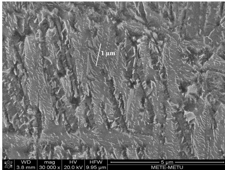
Figure 4.37. SEM micrograph of Mo-IT-280-12. Very thin, elongated carbide precipitation within the sheaves can be seen (white precipitates).
