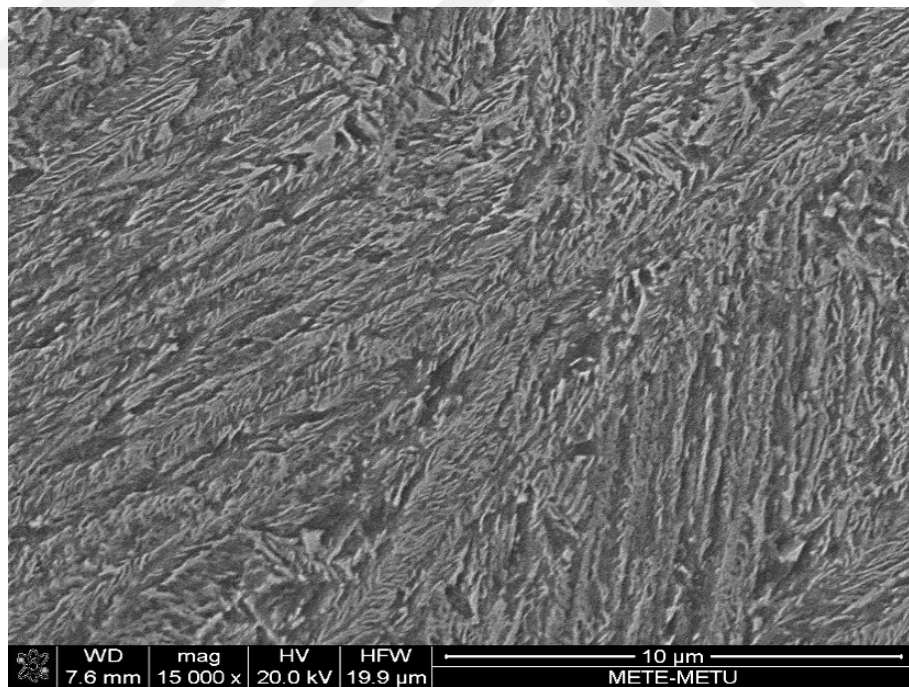
Figure 4.22. SEM micrograph of Mo-IT-280-12.
