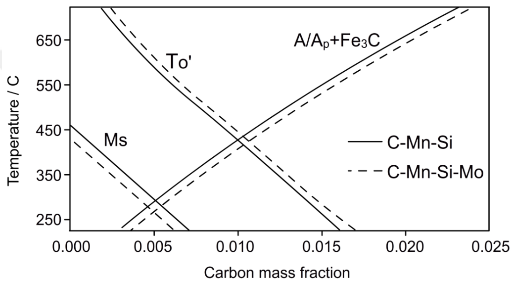
Figure 4.34. The schematic drawing of T_0' curve. At the right of this curve, the bainitic reaction cannot proceed.
