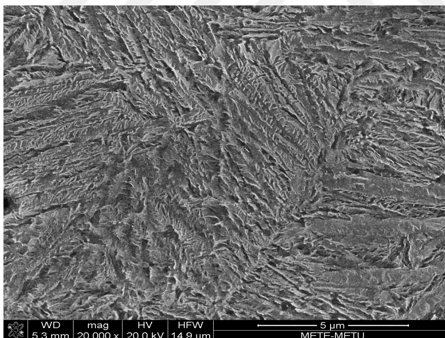
Figure 4.9. SEM micrograph of IT-250-12.
