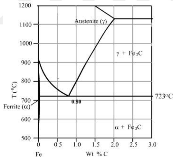
Figure 2.1. Fe-C phase diagram of a eutectoid steel.
