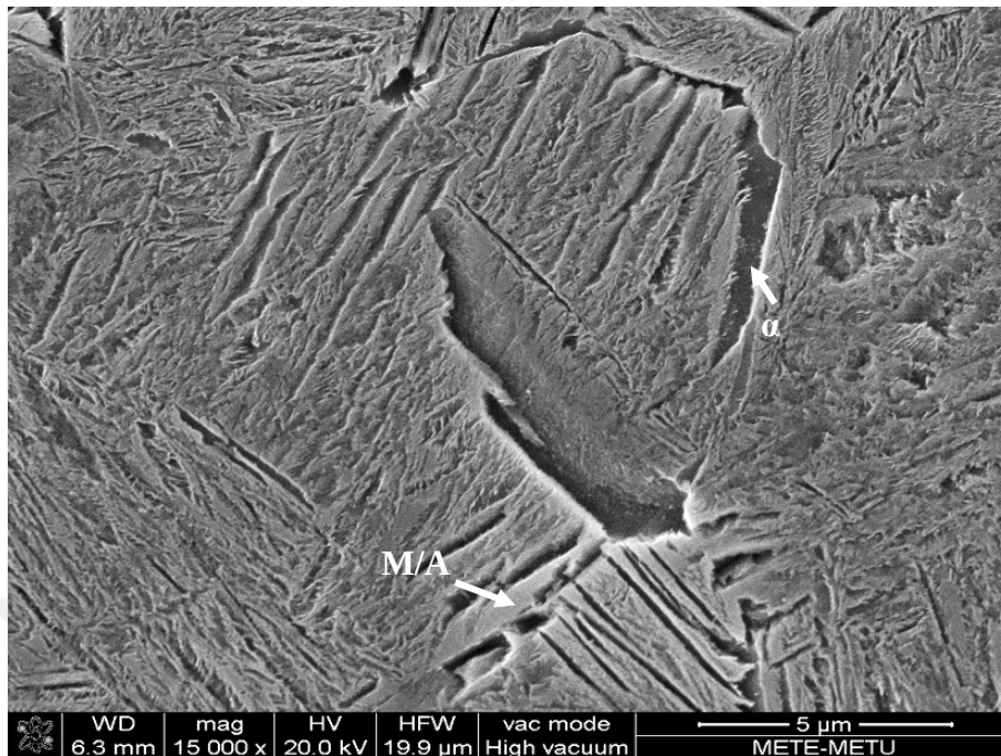
Figure 4.2. SEM micrograph of 900-IT-200-12.
