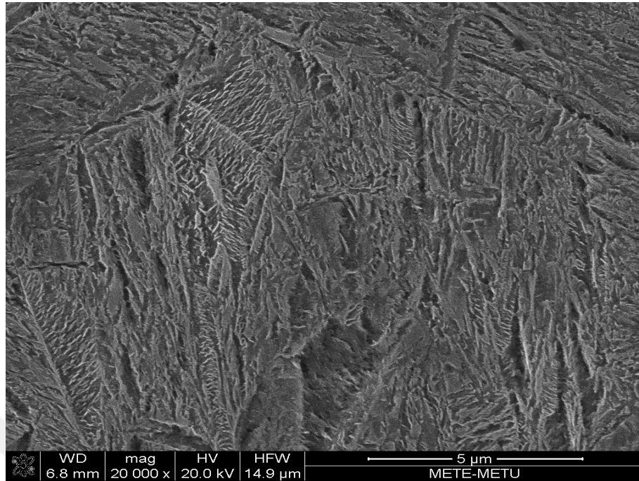
Figure 4.7. SEM micrograph of IT200-24.
