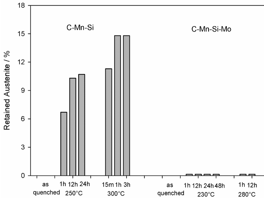
Figure 4.32. The retained austenite contents of all the specimens.
