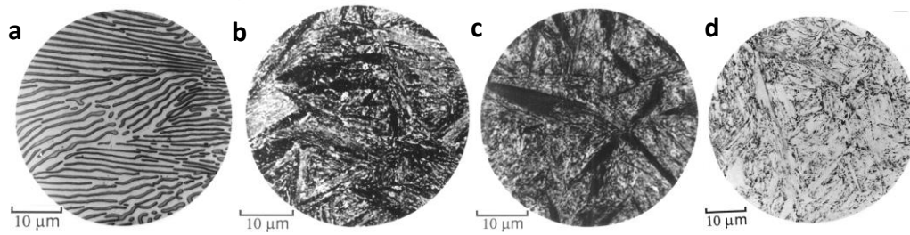
Figure 2.2. Optical micrographs of a eutectoid steel (a) pearlitic structure, (b:c) bainitic structure, (d) martensitic structure [27].
