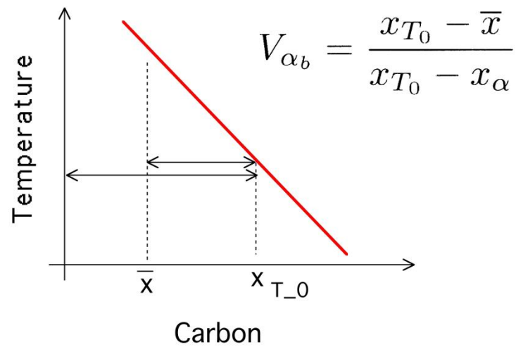
Figure 2.9. Lever rule applied to the T_0 curve to determine the allowable fraction of bainite.
