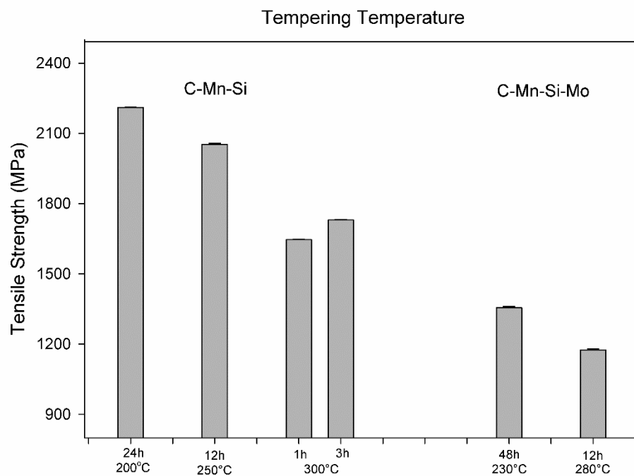
Figure 4.31. Tensile strength values of the isothermal treated C-Mn-Si and C-Mn-Si-Mo alloys.
