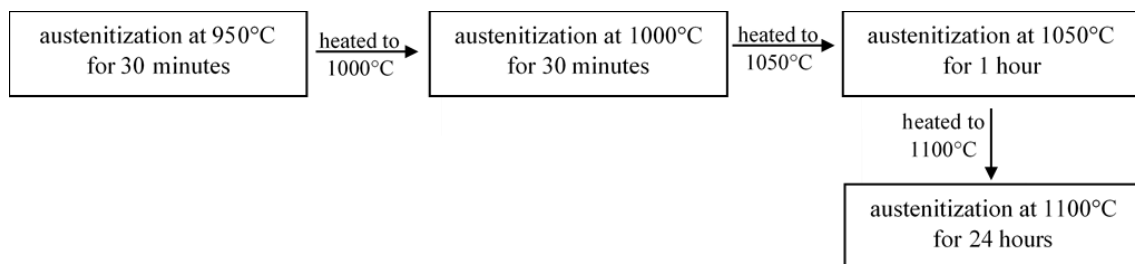
Figure 4.14. Schematic representation of the homogenization process.
