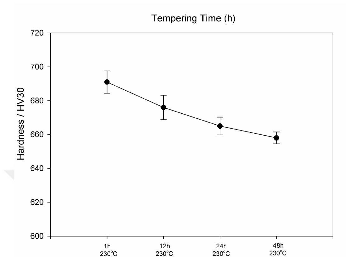
Figure 4.27. Hardness vs. tempering time of C-Mn-Si-Mo alloy.
