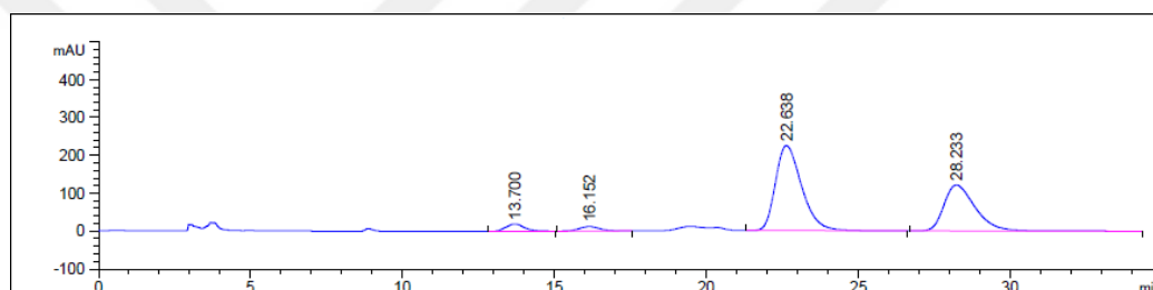
Figure B. 18. HPLC chromatogram of enantiomerically enriched 45h
