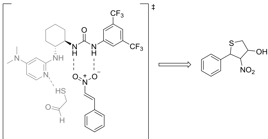
Figure 12. Proposed transition state
