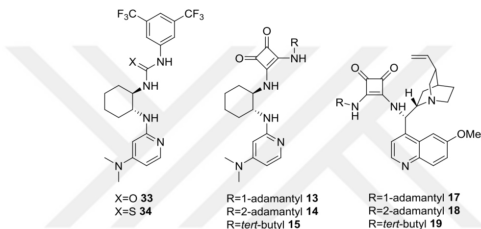
Figure 10. Chiral bifunctional organocatalysts developed by our research group
