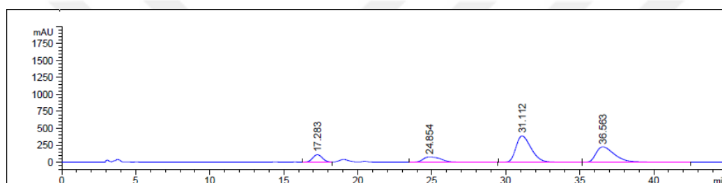
Figure B. 16. HPLC chromatogram of enantiomerically enriched 45g
