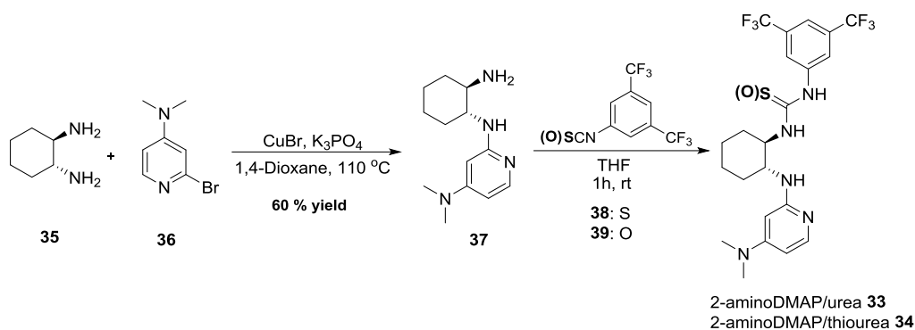
Scheme 17. Synthesis of 2-aminoDMAP/urea and thiourea organocatalysts
