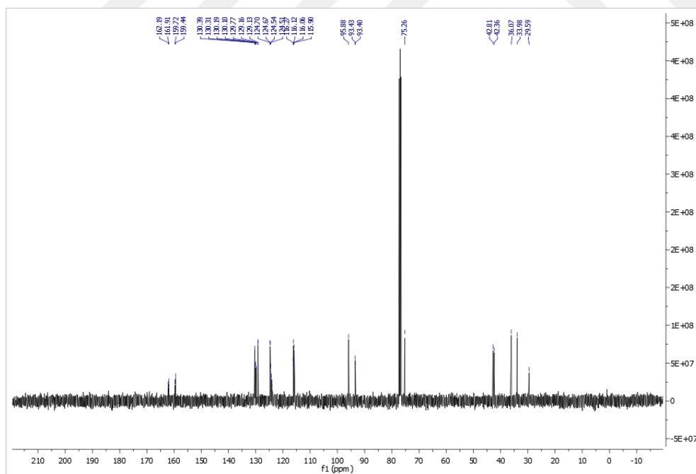
Figure A. 24. 13 C NMR spectrum of compound 45h
