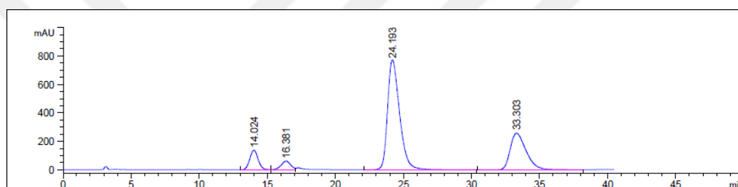
Figure B. 14. HPLC chromatogram of enantiomerically enriched 45f
