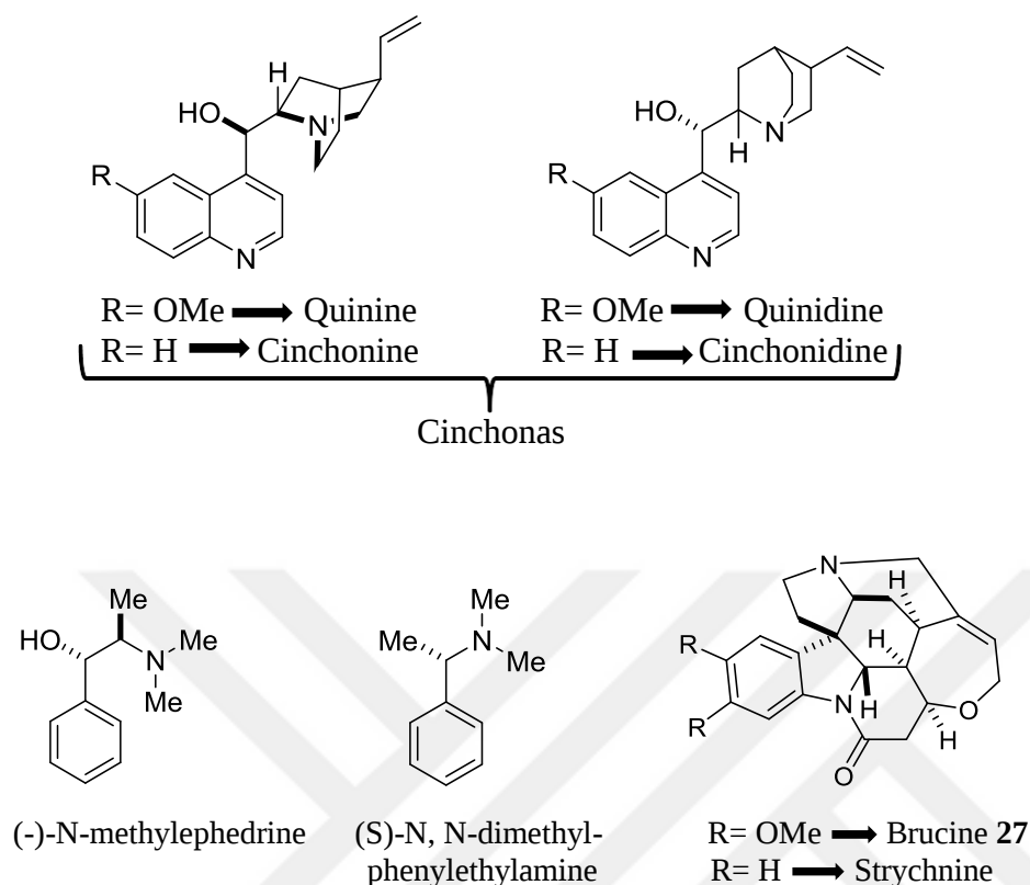
Figure 8. Catalysts screened
