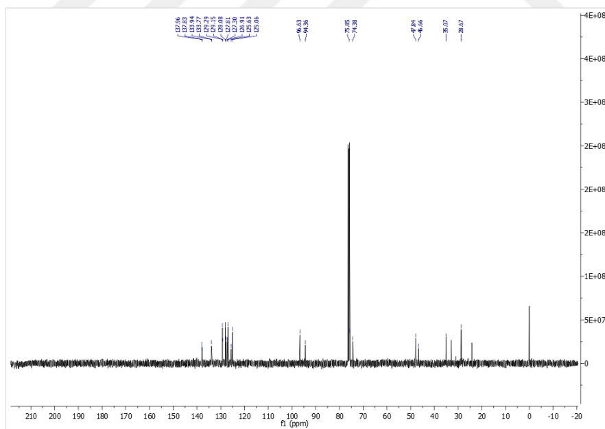
Figure A. 20. ^{13}\text{C} NMR spectrum of compound 45f
