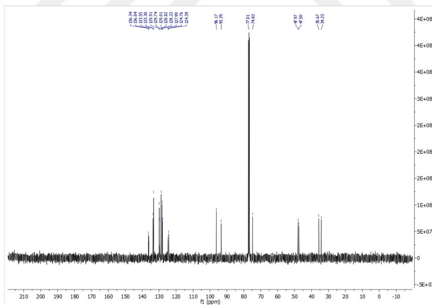
Figure A. 22. ^{13}\text{C} NMR spectrum of compound 45g
