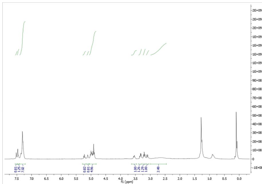
Figure A. 19. ^1\text{H} NMR spectrum of compound 45f
