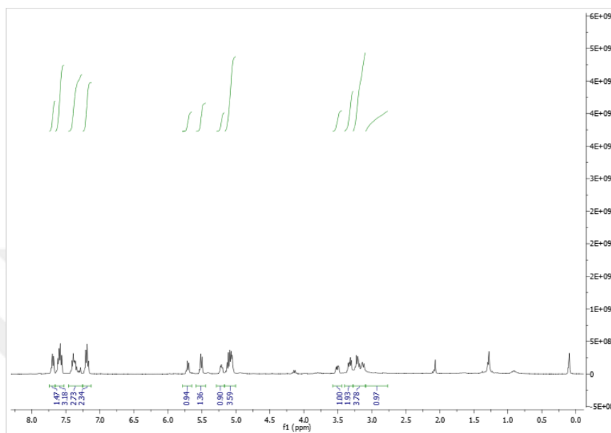
Figure A. 21. ^1\text{H} NMR spectrum of compound 45g
