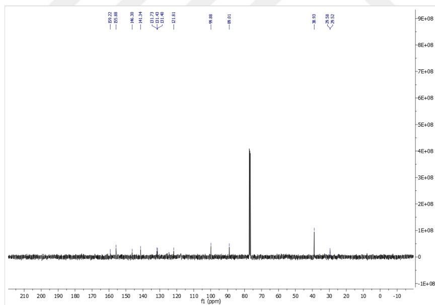
Figure A. 4. ^{13}\text{C} NMR spectrum of compound 33
