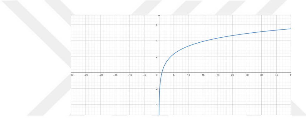
Figure 4.13. \text{Log}_2(X) function.
