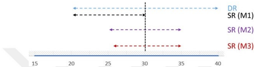
Figure 4.10. Counter example for Suh's formula.
