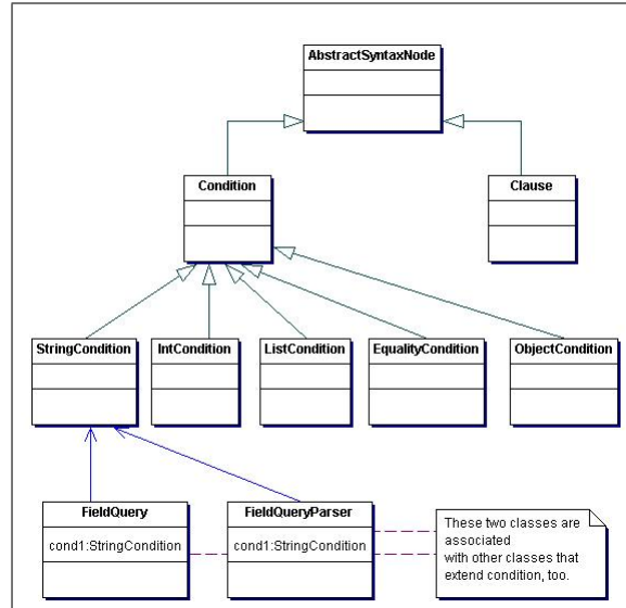
Figure 7.7: The class diagram of field query nodes. A composite pattern was used for arbitrary nesting of query objects.
