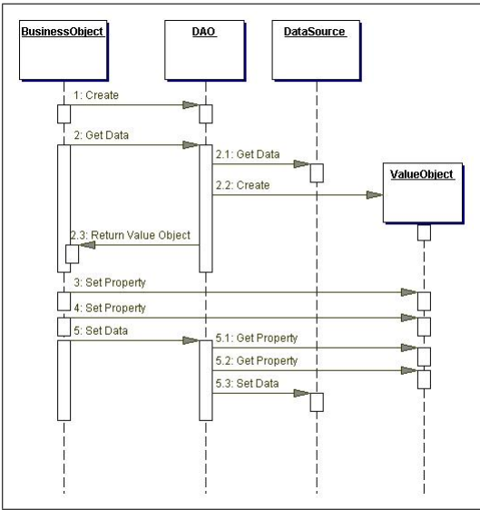
Figure 7.2: DAO pattern allows decoupling business logic from the persistence aspects
