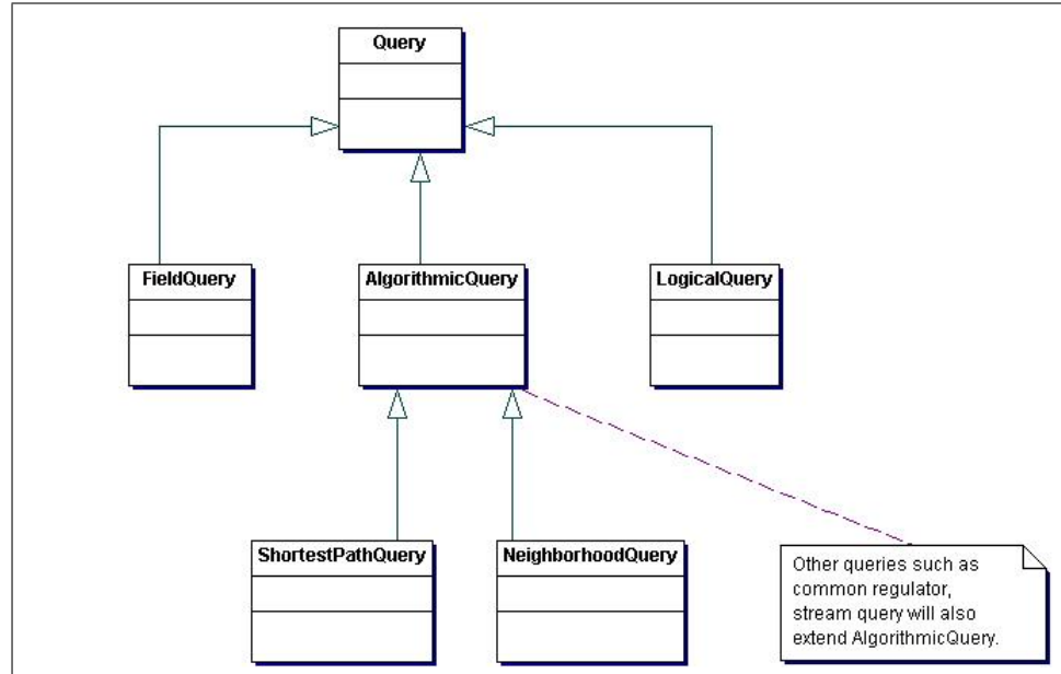
Figure 7.6: An overview of query class relations. Not all algorithmic queries are shown for brevity.
