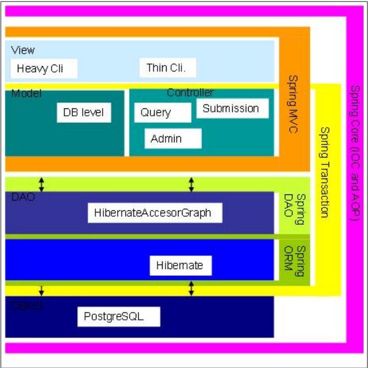
Figure 7.3: Server components within spring framework. Cross cutting concerns, such as transaction damarcation is done via AOP.
