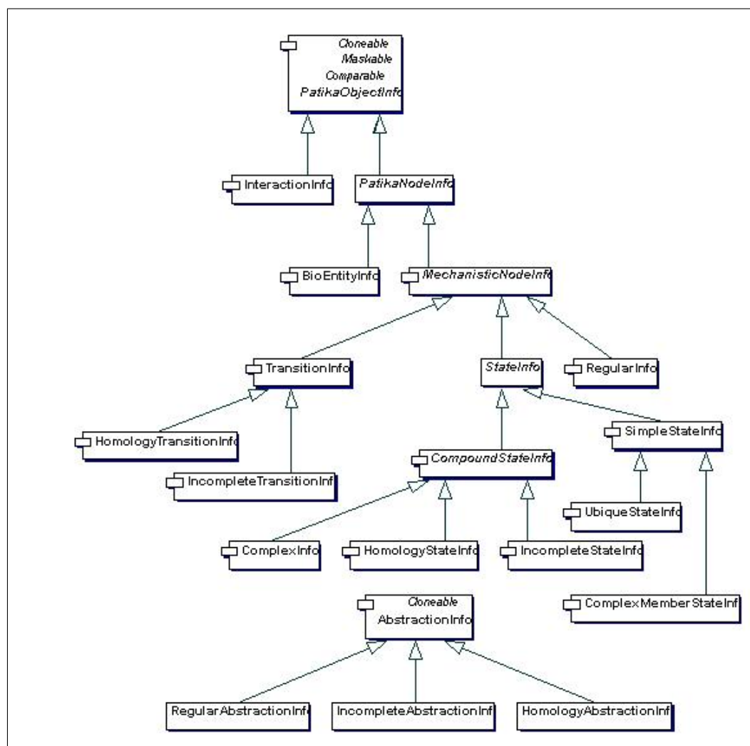
Figure 6.2: Class hierarchy of info objects
