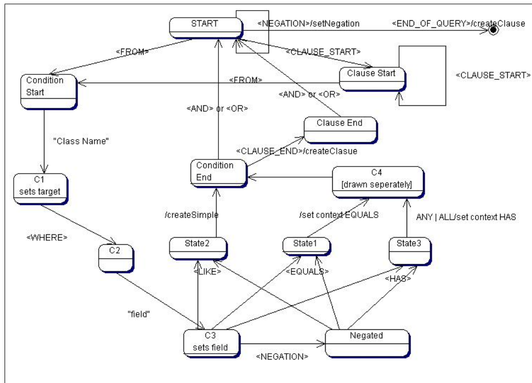
Figure 7.8: General state diagram of fieldQueryParser , for parsing the PATIKA query languages field queries.
