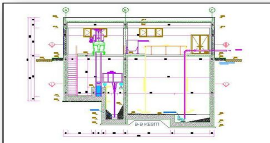
Figure 3.3 Pretreatment units
