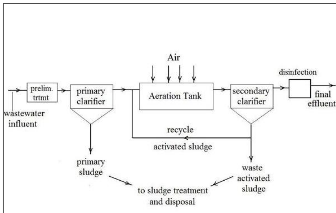
Figure 2.3 Conventional activated sludge process
