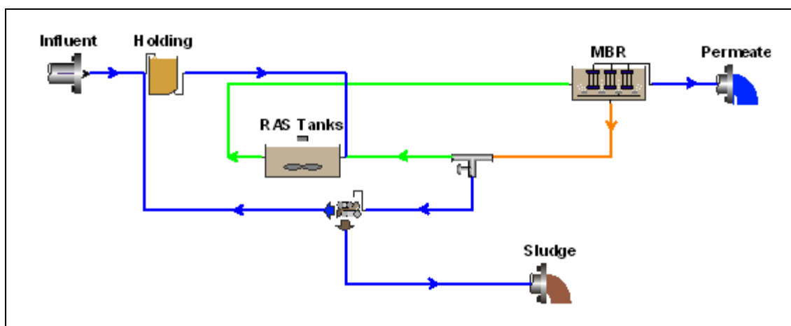
Figure 4.4 The simulation flow diagram of Konacık- MBR system (Alternative 2)
