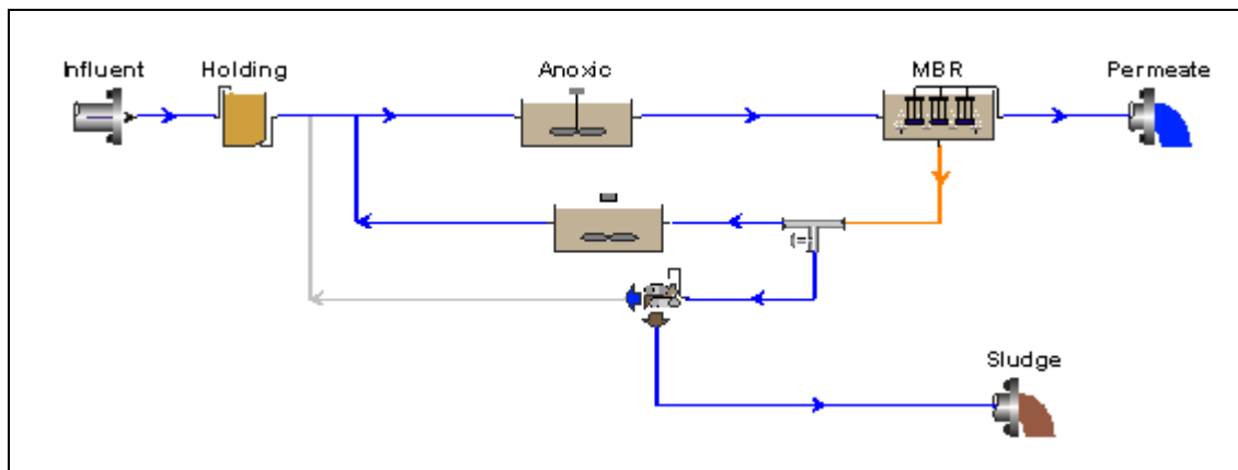
Figure 4.3 The simulation flow diagram of Konacık- MBR system (Alternative 1)
