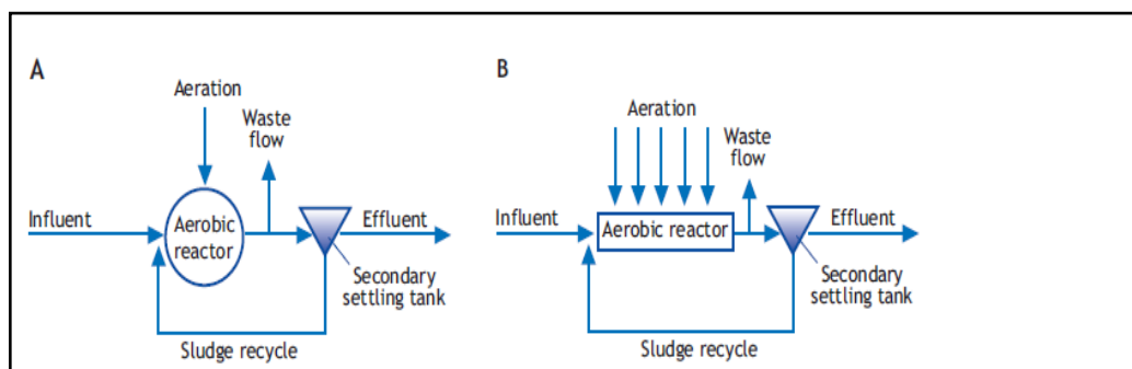
Figure 2.2 Activated sludge systems with (a) a single reactor completely mixed reactor mixing regime, and (b) a flow/intermediate reactor mixing regime (Ekama, 2008, p. 55).
