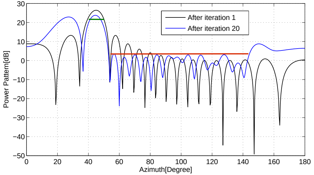
Figure 4.12: Elevation \theta = 0^\circ cut of the power pattern for steering direction (\bar{\theta} = 0^\circ, \bar{\phi} = 45^\circ) computed using the obtained weights after iteration i = 1 (black) and i = 20 (blue). Red line indicates the sidelobe power level \delta_s and green line indicates the main lobe power level \delta .
