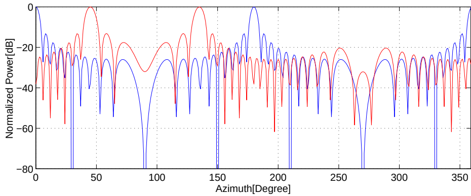
Figure 4.5: Elevation \theta = 90^\circ cut of the power patterns given in Fig.4.3 and Fig.4.4 for steering direction (\bar{\theta} = 90^\circ, \bar{\phi} = 0^\circ) (blue) and (\bar{\theta} = 90^\circ, \bar{\phi} = 45^\circ) (red).
