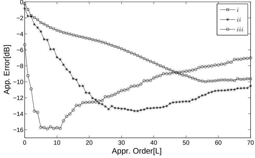
Figure 2.13: Approximation error as a function of approximation order: (i) If no transform is applied (marked with squares); (ii) If only time-frequency translation is applied (marked with stars); (iii) If all the proposed transforms are applied (marked with circles).
