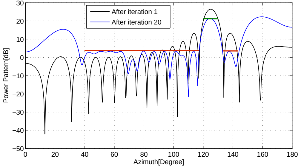
Figure 4.11: Elevation \theta = 0^\circ cut of the power pattern for steering direction (\bar{\theta} = 0^\circ, \bar{\phi} = 125^\circ) computed using the obtained weights after iteration i = 1 (black) and i = 20 (blue). Red lines indicate the sidelobe power level \delta_s and green line indicates the main lobe power level \delta .
