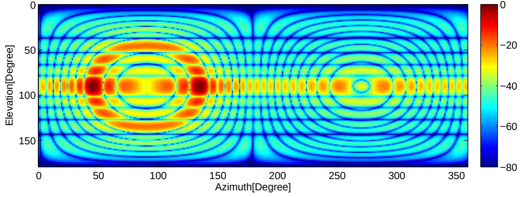
Figure 4.4: Normalized power pattern of the antenna array shown in Fig.4.2 operating at 6 GHz, when the array beam is steered to (\bar{\theta} = 90^\circ, \bar{\phi} = 45^\circ) .
