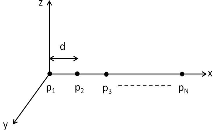
Figure 4.7: Uniform linear array with N = 21 elements. Inter element spacing is d = 0.4\lambda .
