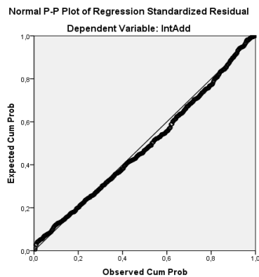
Figure 4.3.1 Normality Histogram
