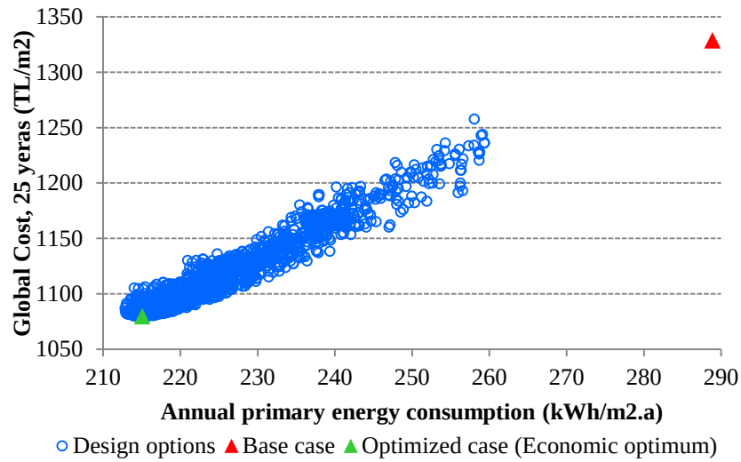
Figure 5.24 : Global cost vs primary energy cloud obtained with Istanbul case.
