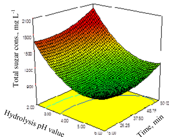
Figure 3.79 Variation of total sugar concentration with time and pH at T=135^\circ\text{C} .
