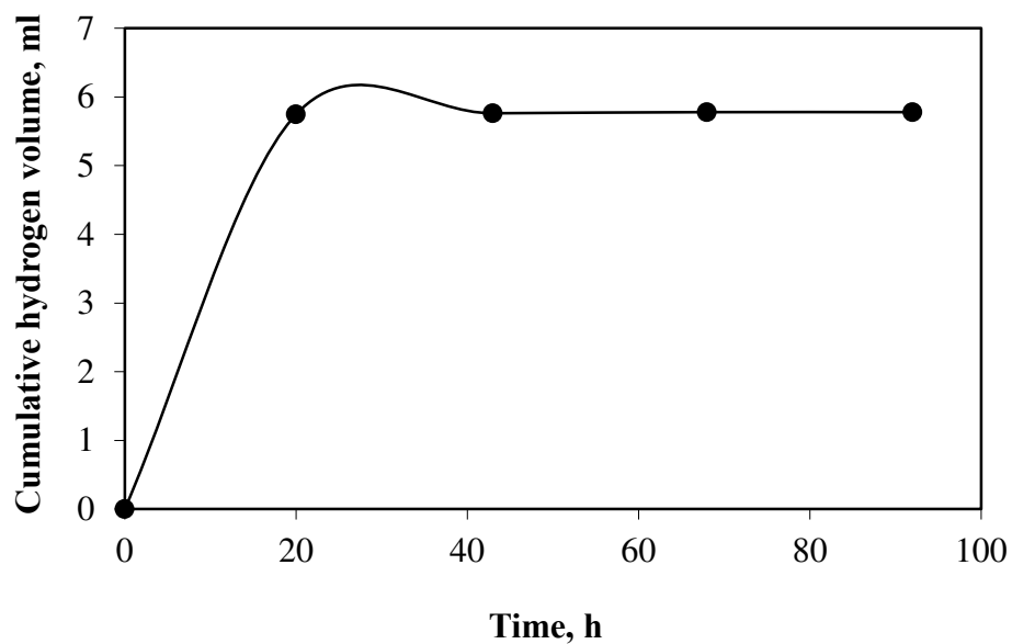
Figure 3.95 Variation of cumulative hydrogen gas volume with time for filtrate at 45^{\circ}\text{C} fermentation temperature.
