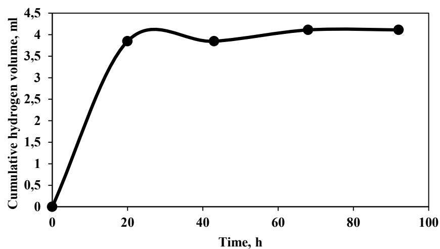
Figure 3.46 Variation of cumulative hydrogen gas volume with time for filtrate obtained at T=60°C and t=60 min hydrolysis conditions.
