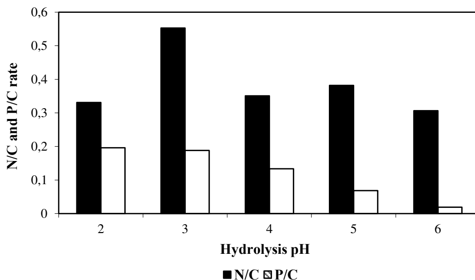
Figure 3.18 Variation of initial N/C and P/C ratios in the filtrate with hydrolysis pH.
