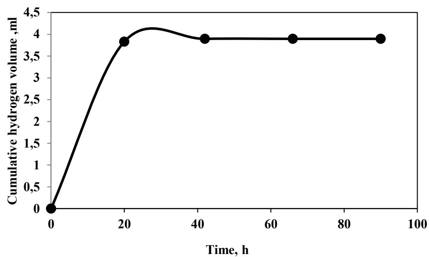
Figure 3.44 Variation of cumulative hydrogen gas volume with time for filtrate obtained at T=100°C and t=45 min hydrolysis conditions.
