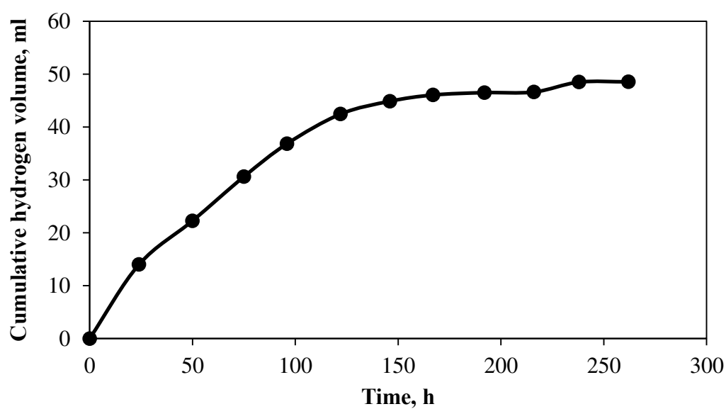
Figure 3.177 Variation of cumulative hydrogen gas volume with time in dark fermentation of sludge \text{TS}=2000 \text{ mg L}^{-1} total sugar concentration.
