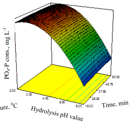
Figure 3.86 Variation of \text{PO}_4\text{-P} concentration with hydrolysis pH and time at T=135^\circ\text{C} .
