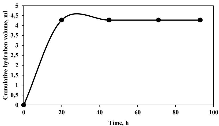
Figure 3.59 Cumulative hydrogen gas volume produced by dark fermentation of sludge hydrolyzed at T=100^{\circ}\text{C} and t=45 min.
