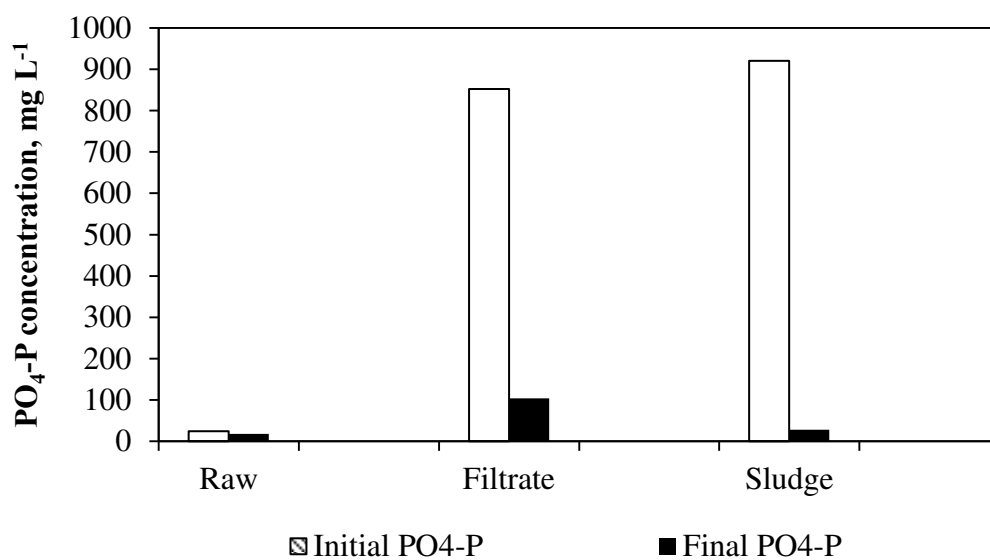
Figure 3.109 Initial and final \text{PO}_4\text{-P} concentrations for different substrates at 55°C fermentation temperature.
