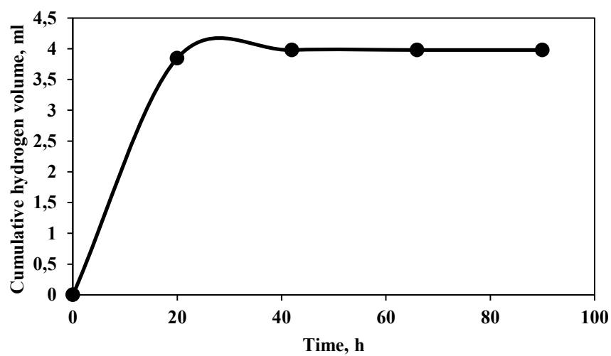
Figure 3.43 Variation of cumulative hydrogen gas volume with time for filtrate obtained at T=60^{\circ}\text{C} and t=45 min hydrolysis conditions.
