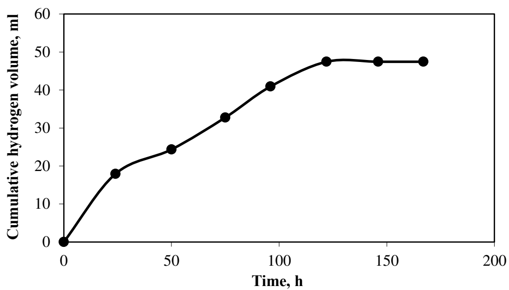
Figure 3.176 Variation of cumulative hydrogen gas volume with time in dark fermentation of filtrate at \text{TS}=2000 \text{ mg L}^{-1} total sugar concentration.
