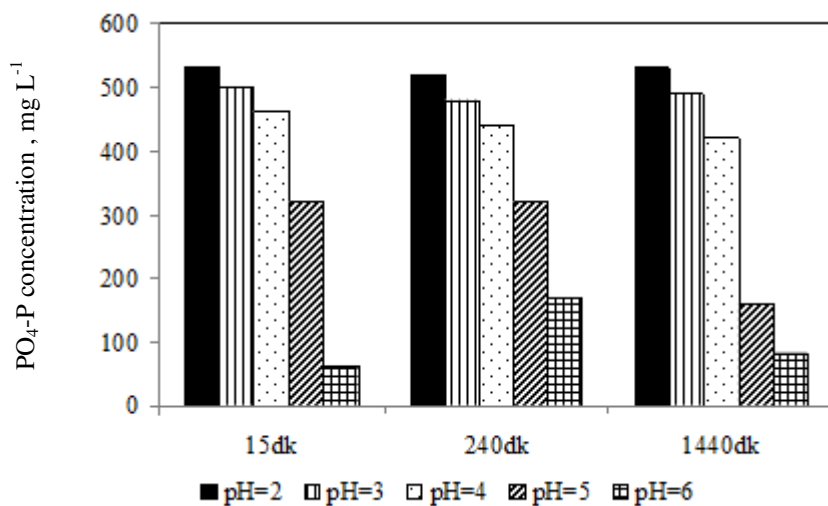
Figure 3.6 Variation of \text{PO}_4\text{-P} concentration with pH and time in single-stage acid hydrolysis of sludge.
