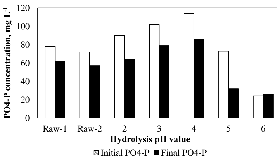
Figure 3.30 Initial and final \text{PO}_4\text{-P} concentrations in hydrogen gas production from sludge hydrolyzed at different pH values.
