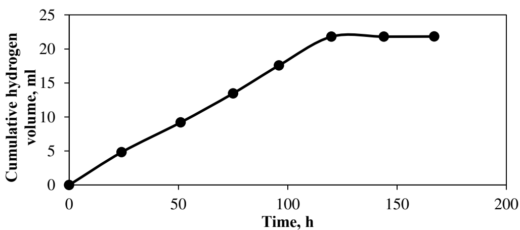
Figure 3.181 Effect of argon sparging on cumulative hydrogen gas volume of sludge hydrolyzed by single-stage heat treatment.
