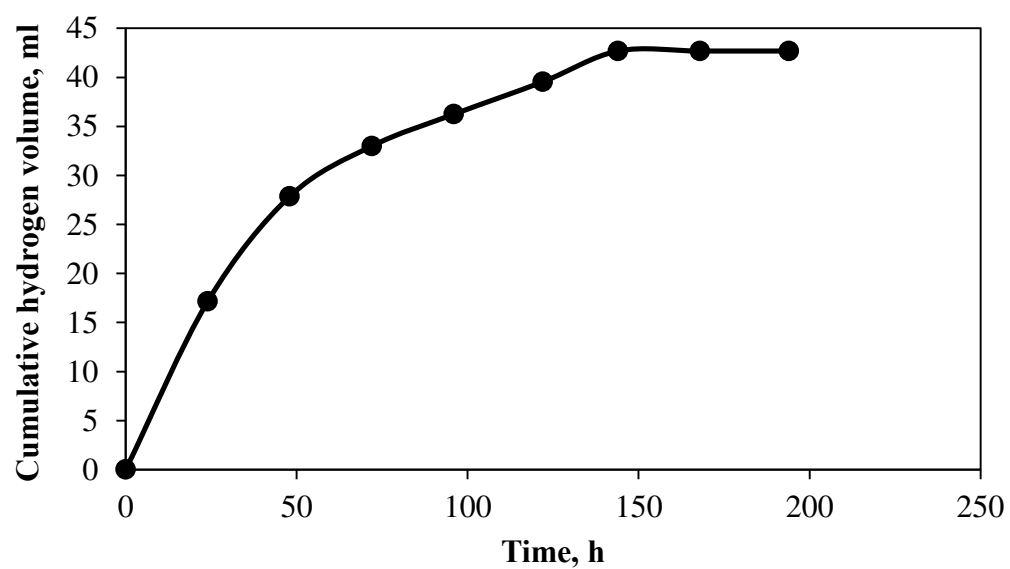
Figure 3.152 Variation of cumulative hydrogen gas volume with time in dark fermentation of sludge at 6 g L -1 initial biomass concentration.
