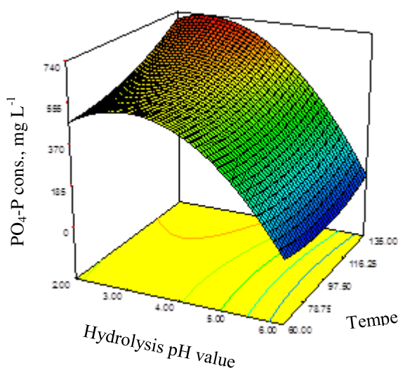
Figure 3.85 Variation of \text{PO}_4\text{-P} concentration with hydrolysis pH and temperature at t=60 min
