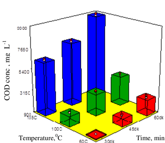
Figure 3.34 Variation of COD concentration with hydrolysis time and temperature.
