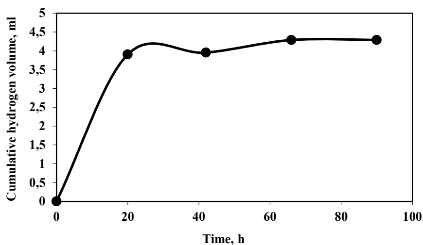
Figure 3.42 Variation of cumulative hydrogen gas volume with time for filtrate obtained at T=135^{\circ}\text{C} and t=30 min hydrolysis conditions.
