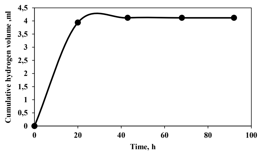
Figure 3.47 Variation of cumulative hydrogen gas volume with time for filtrate obtained at T=100°C and t=60 min hydrolysis conditions.
