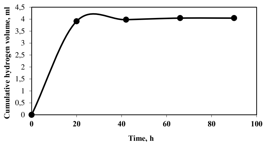
Figure 3.40 Variation of cumulative hydrogen gas volume with time for filtrate obtained at T=60^{\circ}\text{C} and t=30 min hydrolysis conditions.
