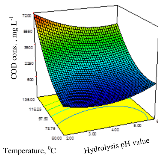
Figure 3.75 Variation of COD concentration with temperature and pH at t=60 min hydrolysis period.
