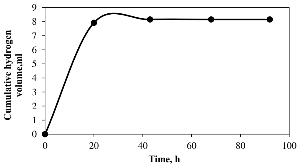
Figure 3.95 Variation of cumulative hydrogen gas volume with time for filtrate at 45^{\circ}\text{C} fermentation temperature.
