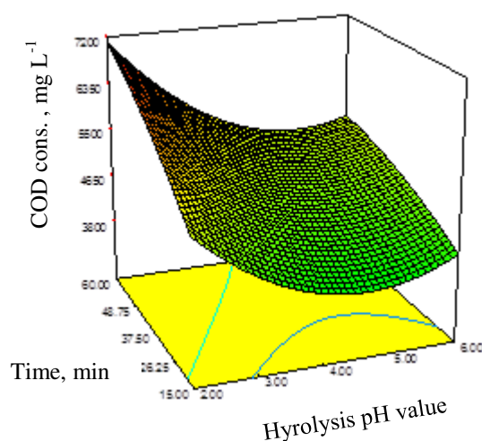
Figure 3.76 Variation of COD concentration with time and pH at T=135 °C hydrolysis temperature.
