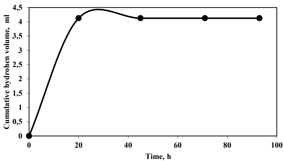
Figure 3.55 Cumulative hydrogen gas volume produced by dark fermentation of sludge hydrolyzed at T=60^{\circ}\text{C} and t=30 min.
