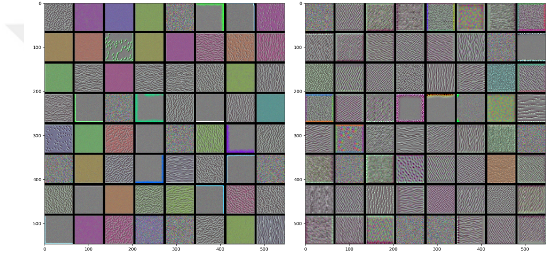
Figure 2.5: Visualization of convolutional filters of block1_conv1 and block2_conv1 layers of the VGG16 model
