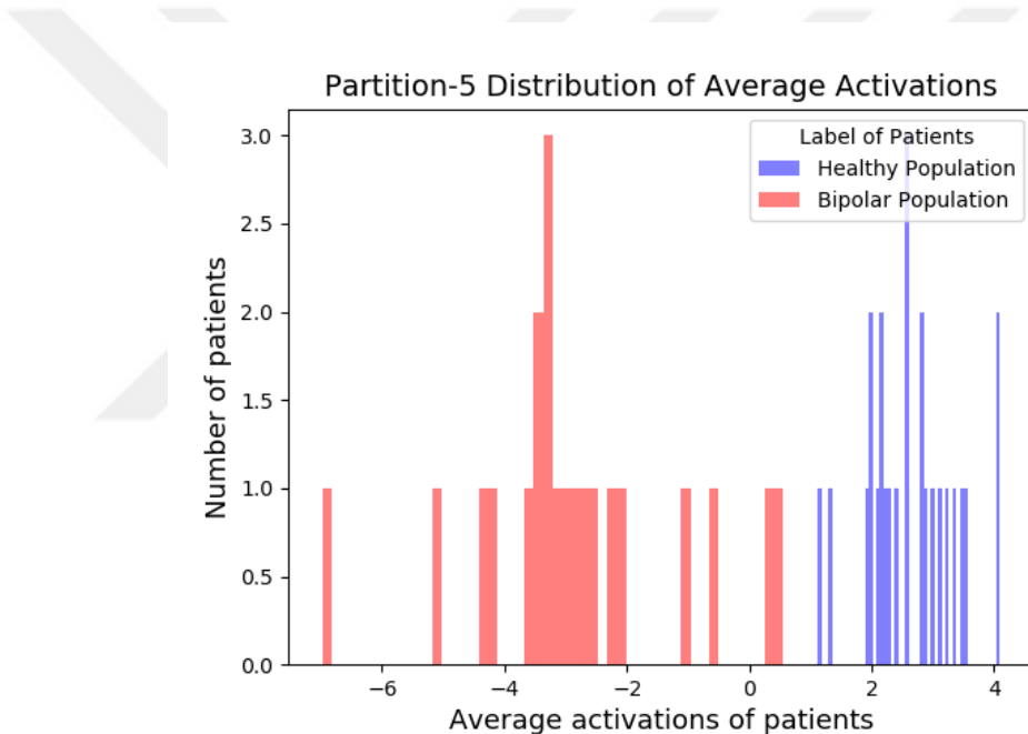
Figure 5.9: The histogram plot of average activations of Task 2 belonging to the ResNet model with 24-channel data
