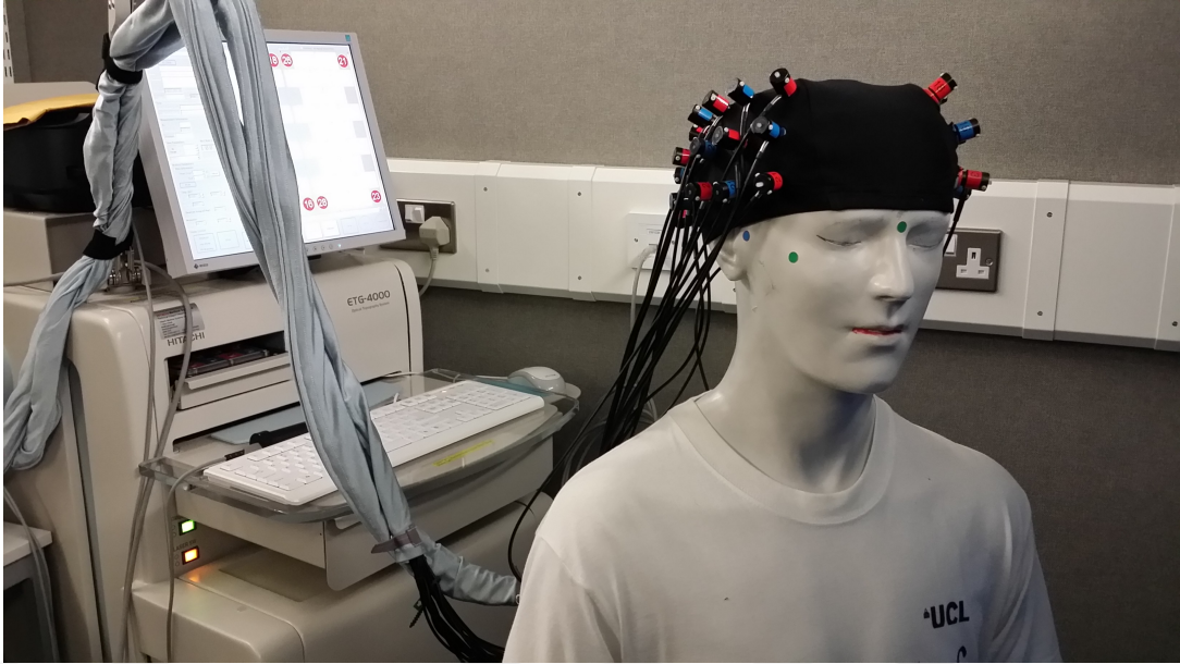
Figure 3.2: Hitachi ETG-4000 optical imaging system to be used for fNIRS measurements [30]
