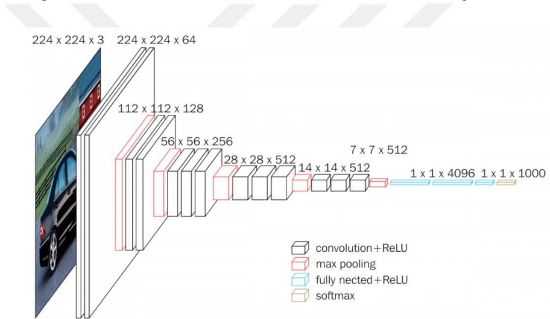
Figure 4.2: The VGG16 network, which is the most common CNN architecture
