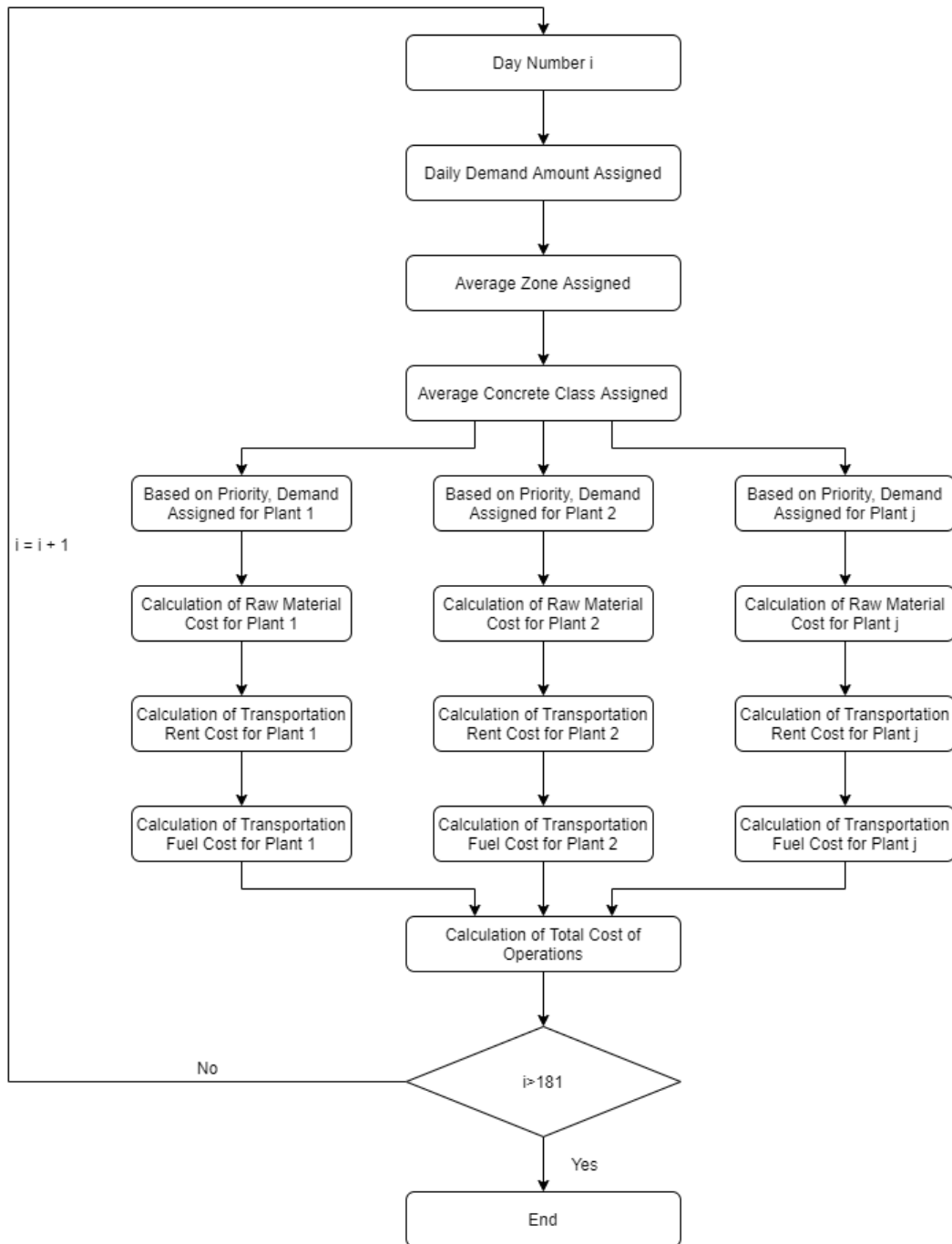
Figure 3.2 The Simulation Algorithm for the Second Run
