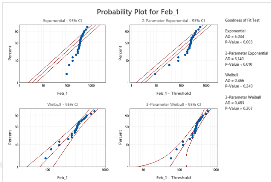
Figure B. 5 Probability Plots of February Demand Data-2
