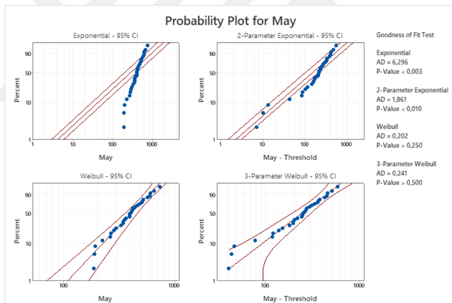
Figure B. 16 Probability Plots of May Demand Data-2
