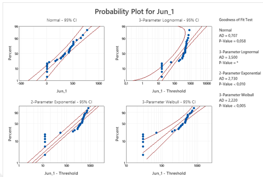
Figure B. 19 Probability Plots of June Demand Data-1
