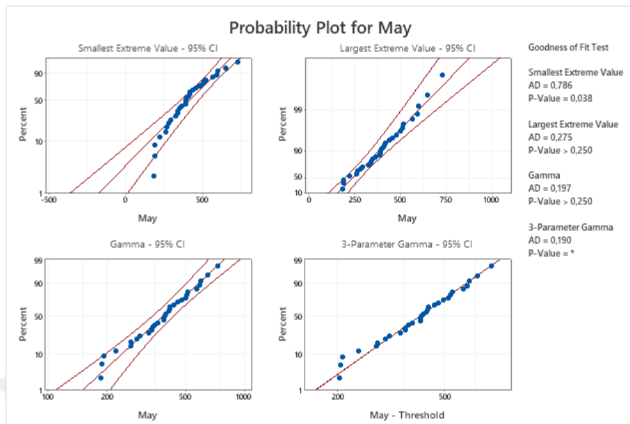
Figure B. 17 Probability Plots of May Demand Data-3
