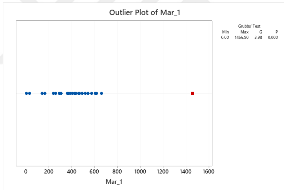
Figure A. 8 Outlier Plot of March (Second Test)
