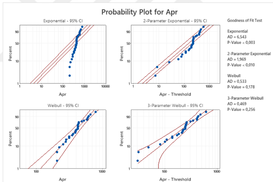
Figure B. 12 Probability Plots of April Demand Data-2
