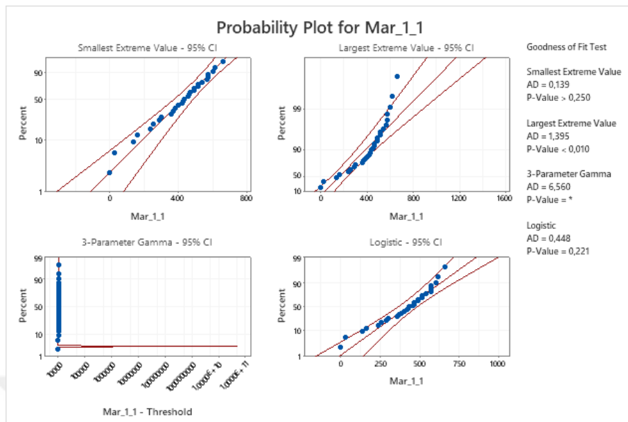
Figure B. 9 Probability Plots of March Demand Data-2
