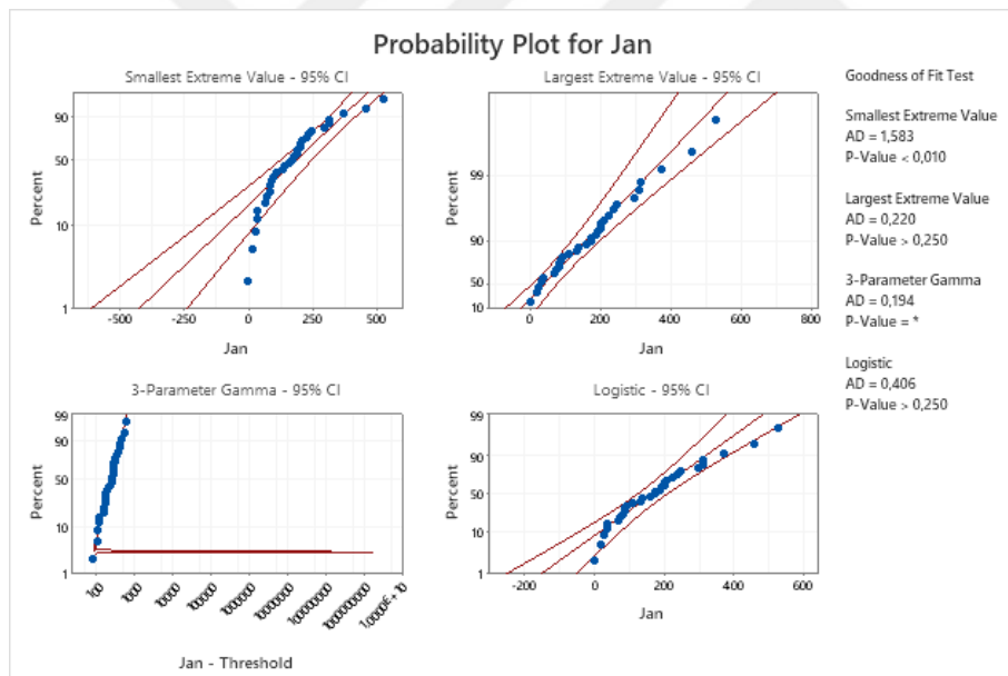
Figure B. 2 Probability Plots of January Demand Data-2
