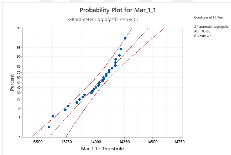
Figure B. 10 Probability Plots of March Demand Data-3
