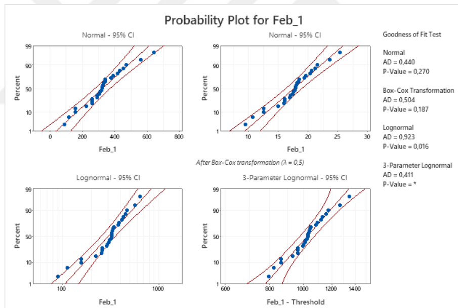
Figure B. 4 Probability Plots of February Demand Data-1
