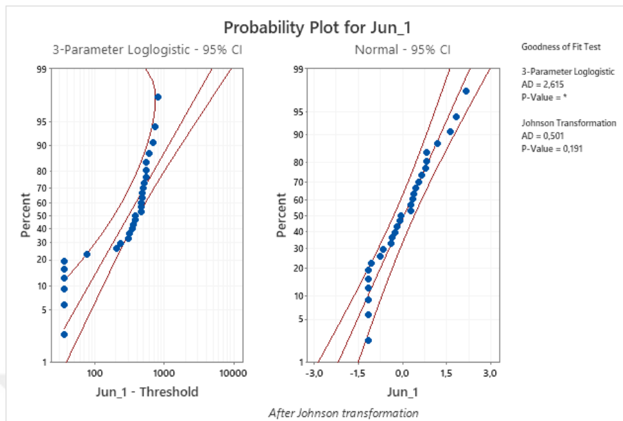
Figure B. 21 Probability Plots of June Demand Data-3
