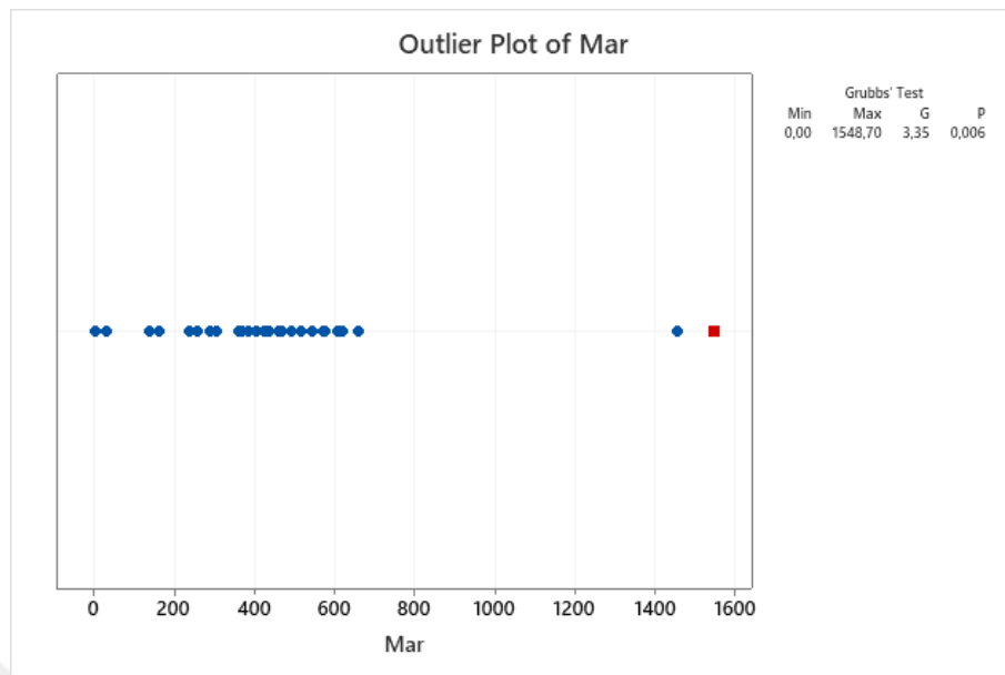
Figure A. 3 Outlier Plot of March (First Test)
