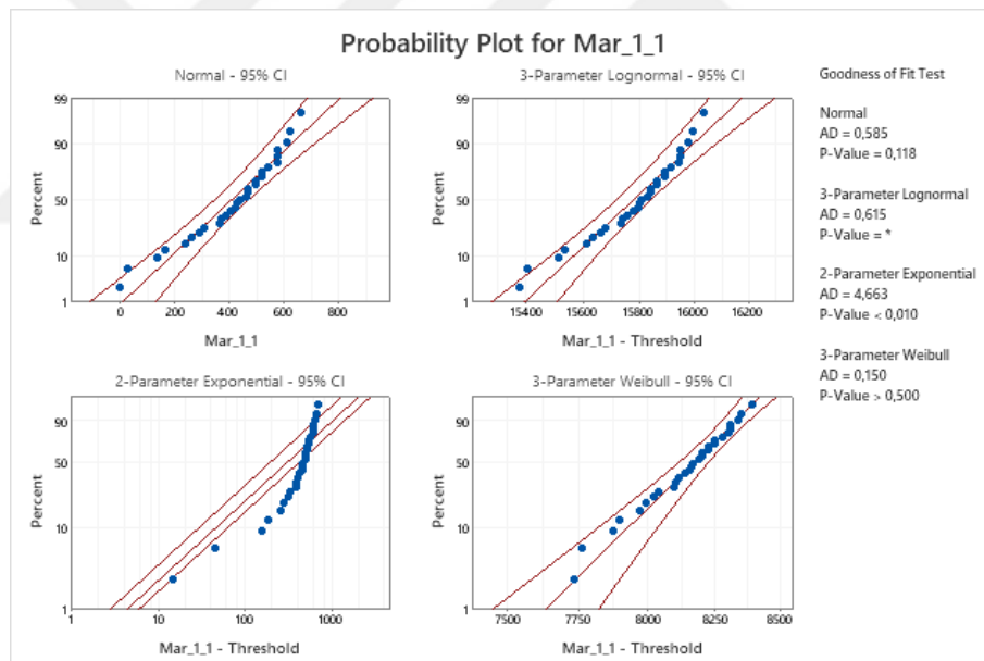
Figure B. 8 Probability Plots of March Demand Data-1
