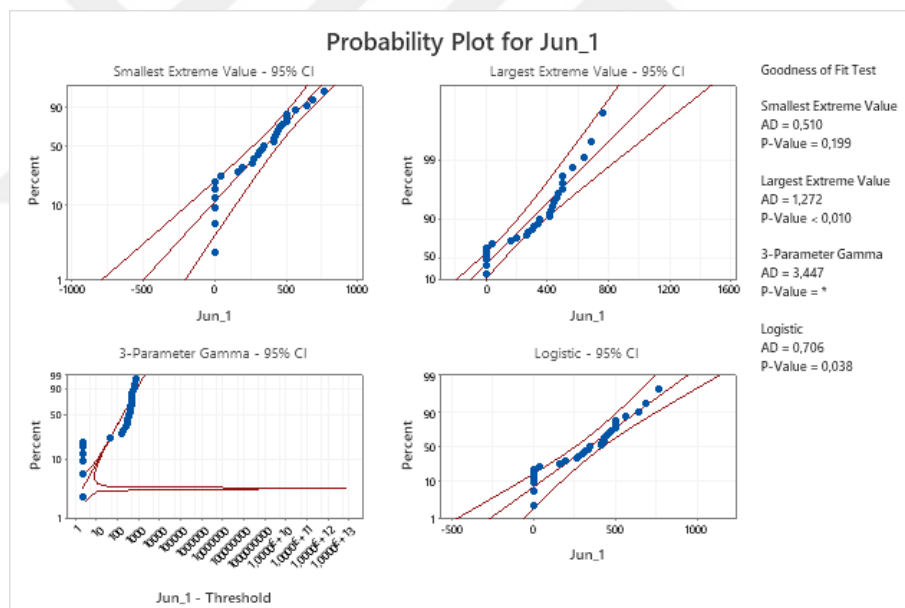
Figure B. 20 Probability Plots of June Demand Data-2
