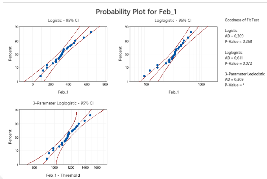
Figure B. 7 Probability Plots of February Demand Data-4
