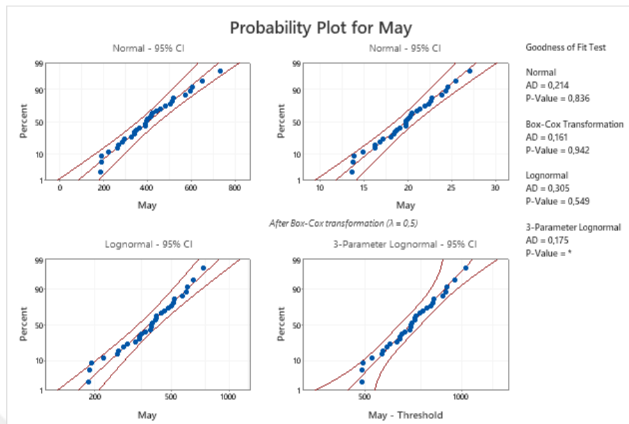
Figure B. 15 Probability Plots of May Demand Data-1
