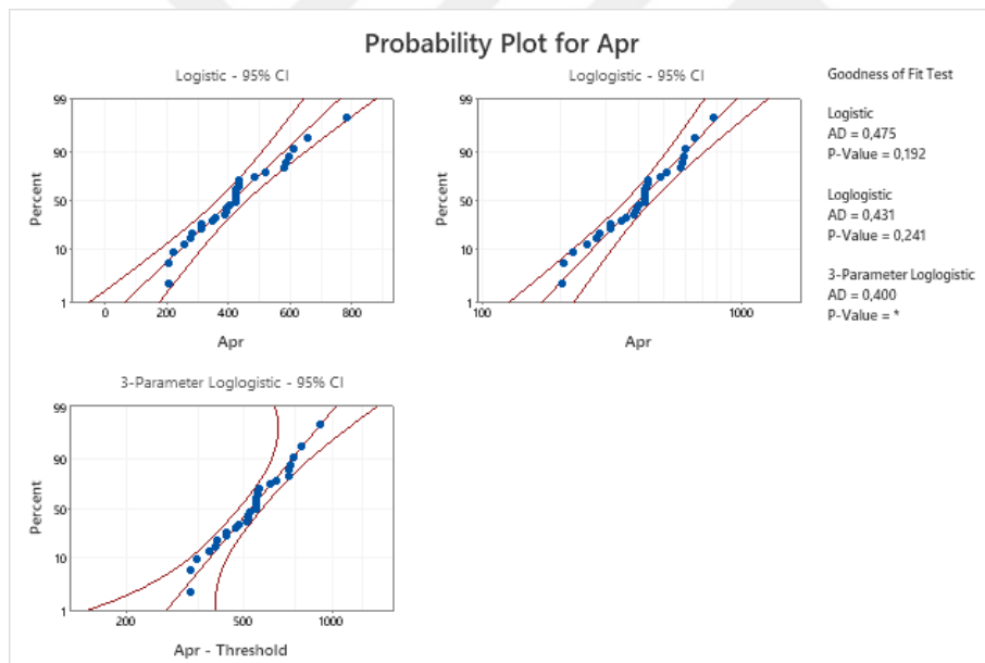
Figure B. 14 Probability Plots of April Demand Data-4
