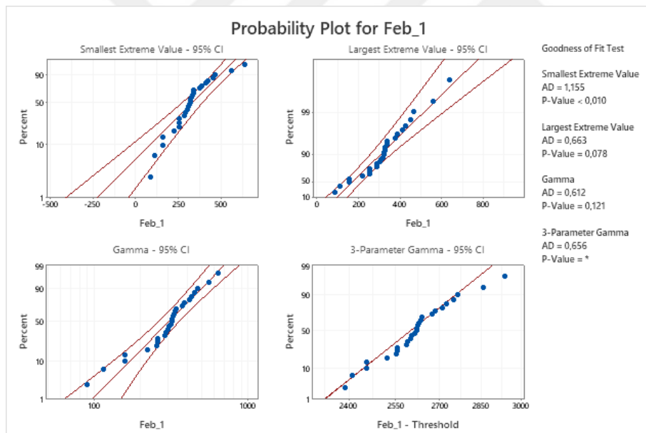
Figure B. 6 Probability Plots of February Demand Data-3
