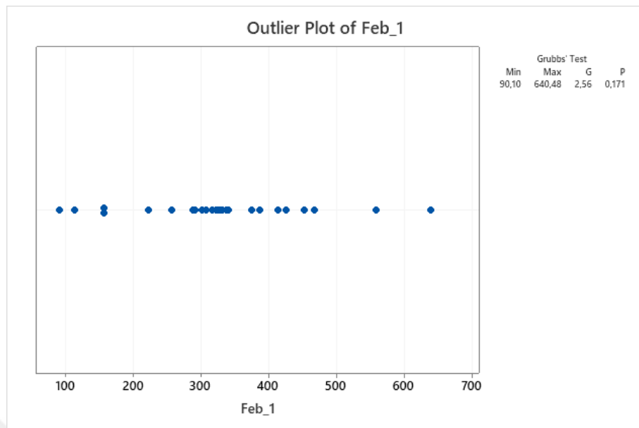
Figure A. 7 Outlier Plot of February (Second Test)
