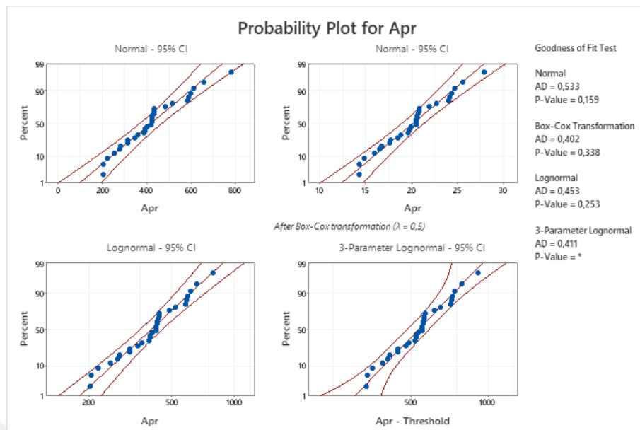
Figure B. 11 Probability Plots of April Demand Data-1
