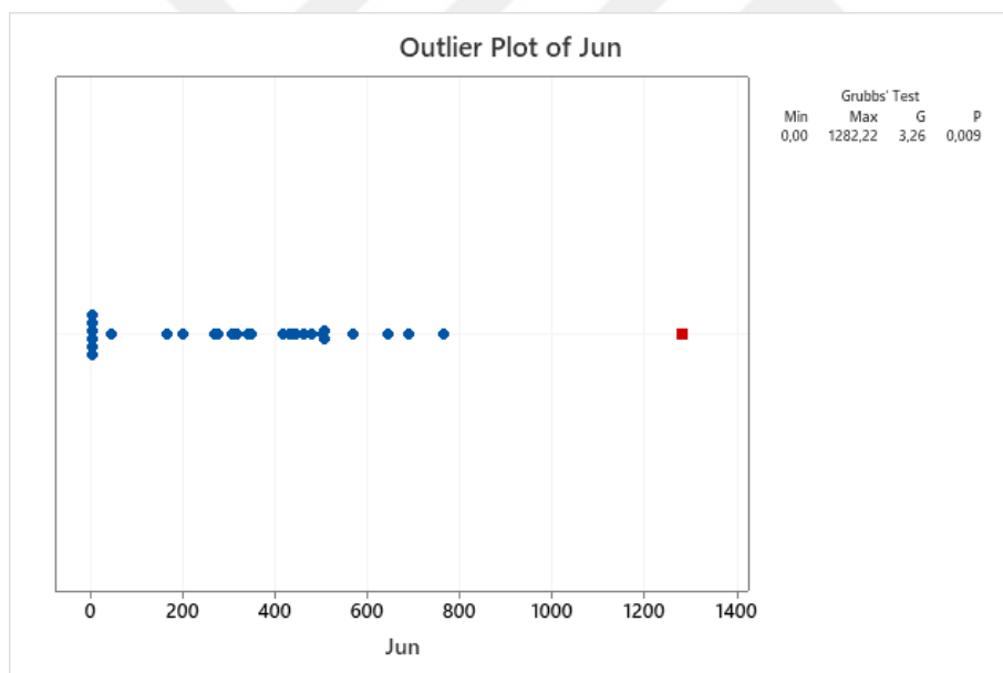
Figure A. 6 Outlier Plot of June (First Test)
