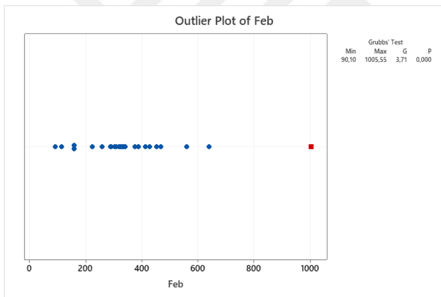
Figure A. 2 Outlier Plot of February (First Test)
