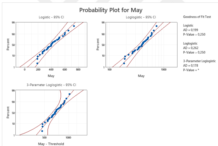
Figure B. 18 Probability Plots of May Demand Data-4
