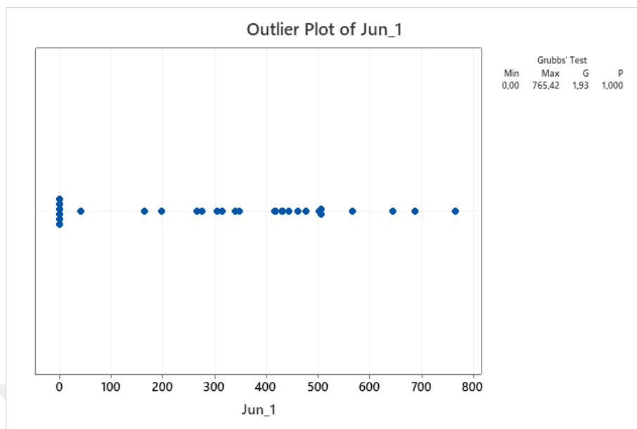
Figure A. 9 Outlier Plot of June (Second Test)
