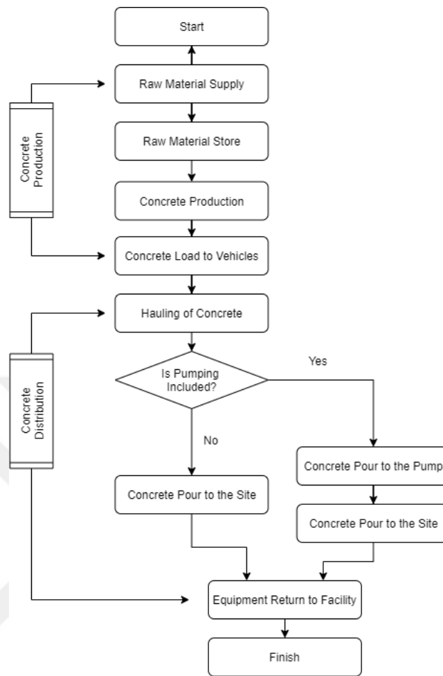
Figure 2.1 Lifecycle of Concrete
