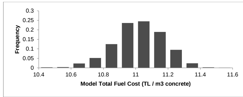
Figure 4.6 Fuel Cost Histogram of the Modified Case Simulation
