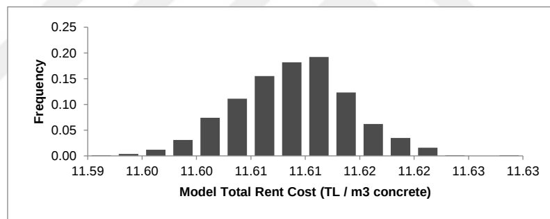
Figure 4.7 Truck-Mixer Rental Cost Histogram of the Modified Case
