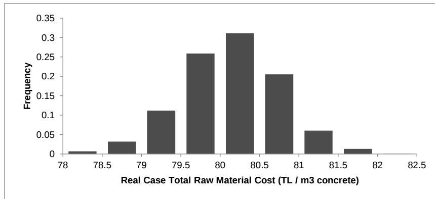
Figure 4.2 Raw Material Cost Histogram of the Real Case Simulation
