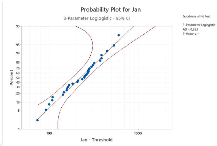
Figure B. 3 Probability Plots of January Demand Data-3
