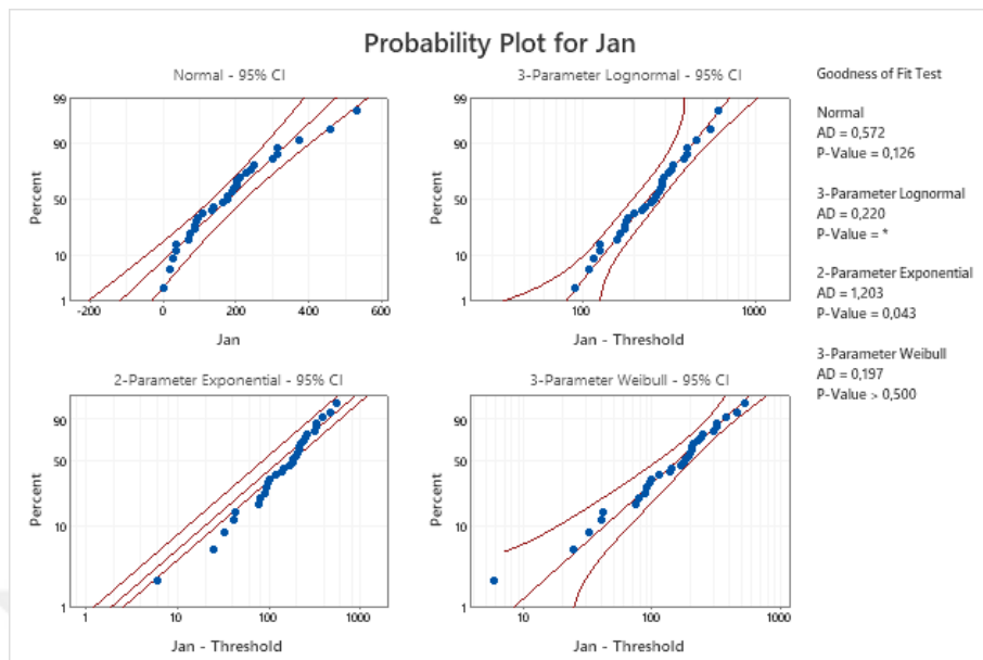
Figure B. 1 Probability Plots of January Demand Data-1
