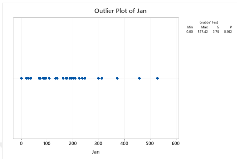
Figure A. 1 Outlier Plot of January (First Test)
