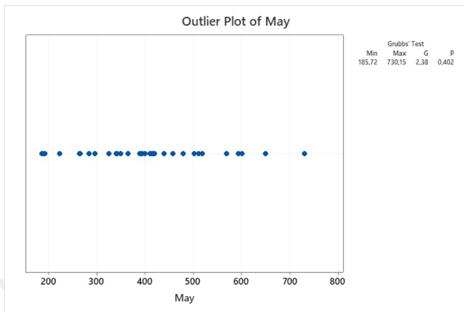
Figure A. 5 Outlier Plot of May (First Test)
