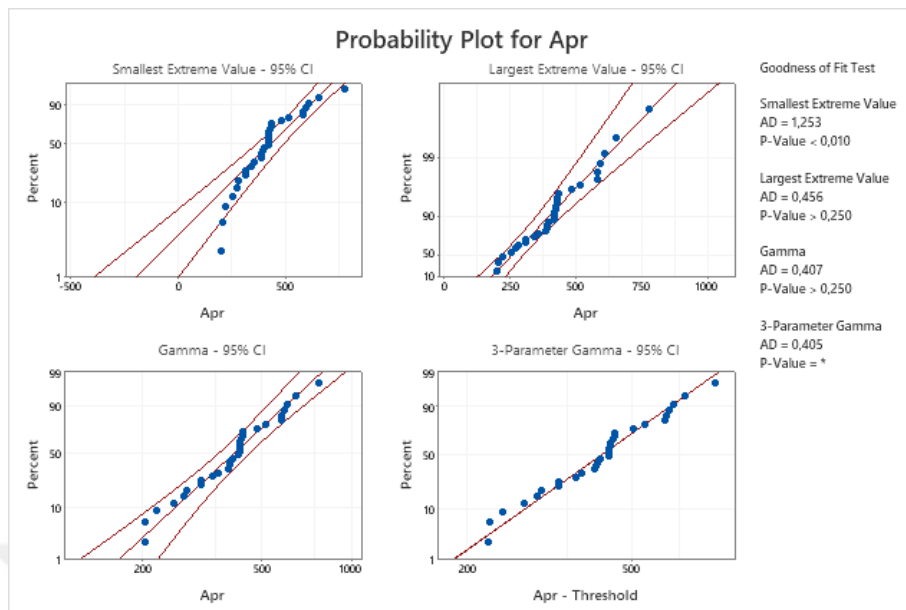
Figure B. 13 Probability Plots of April Demand Data-3
