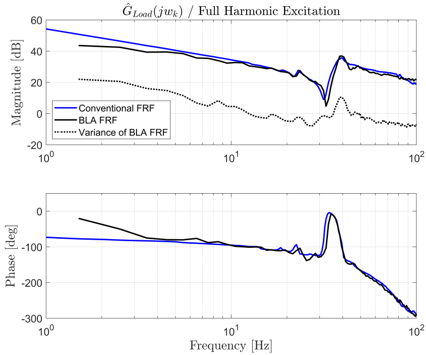
Figure 3.8: The nonparametric model obtained using BLA from torque input to motor speed output (a), and load speed output (b) with the full harmonic random phase multisine excitation.
