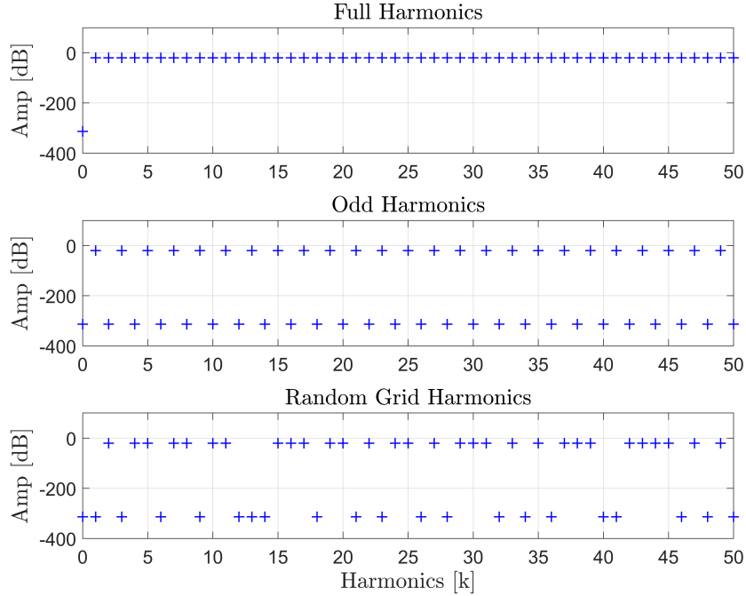
Figure 3.5: Harmonic contents of different random phase multisine excitation signals.
