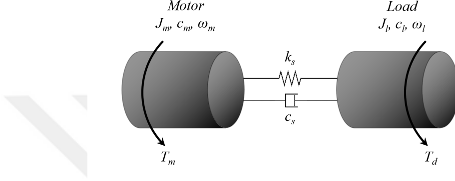
Figure 2.3: System representation with motor-load inertias and elastic driveline of the rotational platform.
