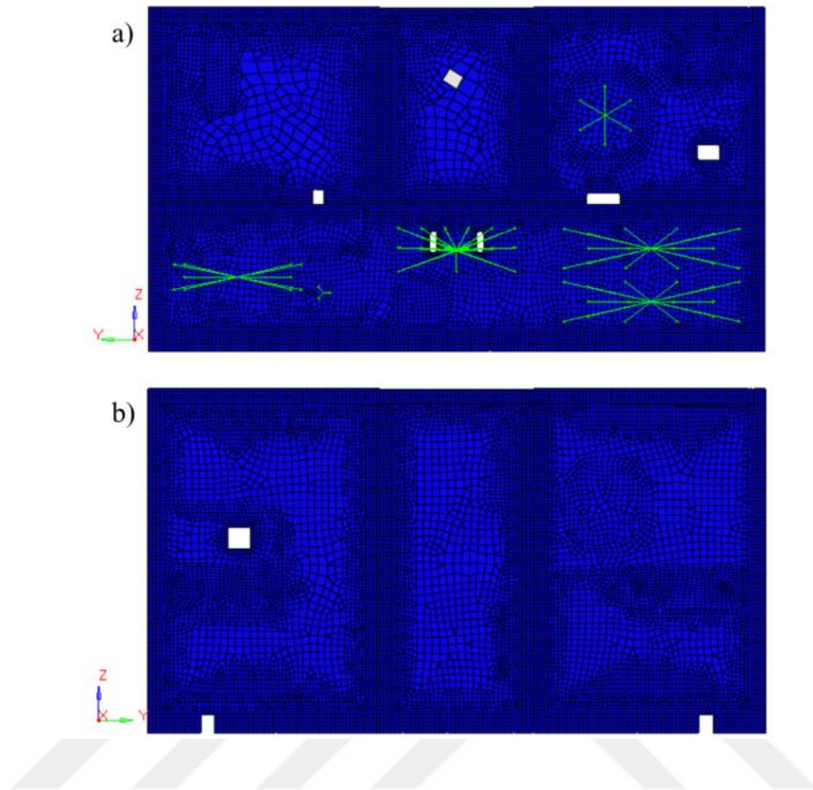
Figure 3.19. The FEM of (a) West and (b) East Service Panels
