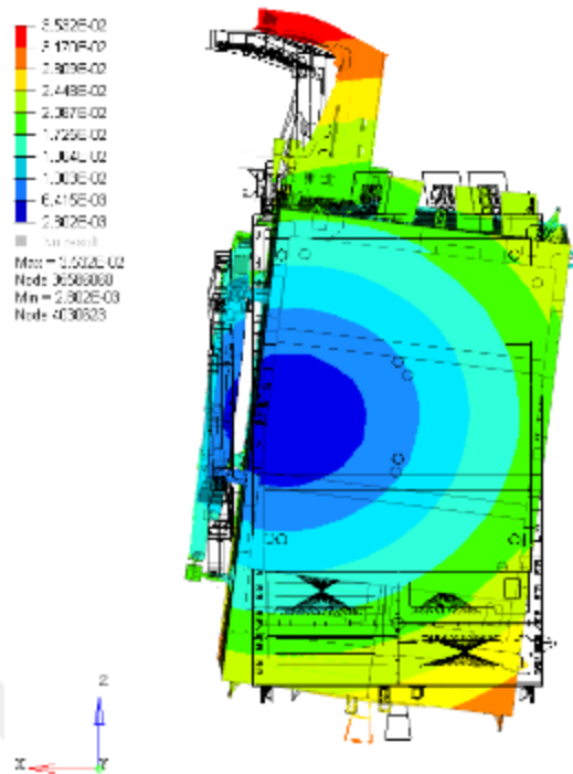
Figure 3.27. Free Boundary Condition Rotational Y Result
