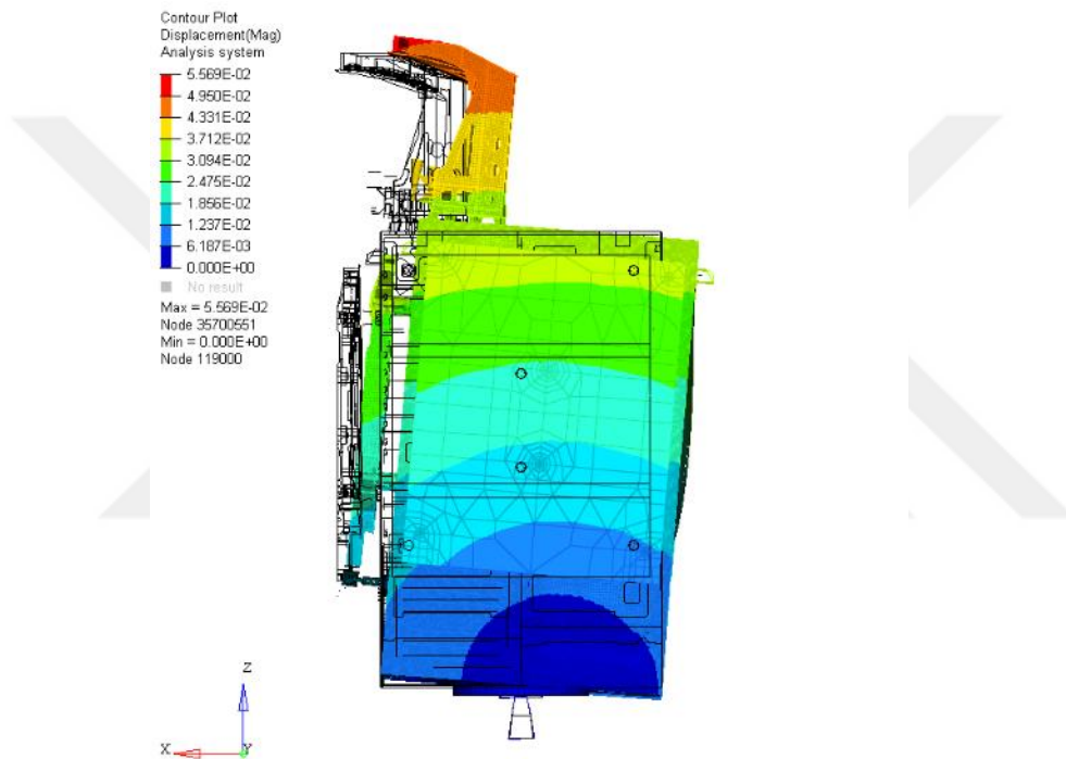
Figure 5.2. Global X Wise Bending Mode of the Satellite
