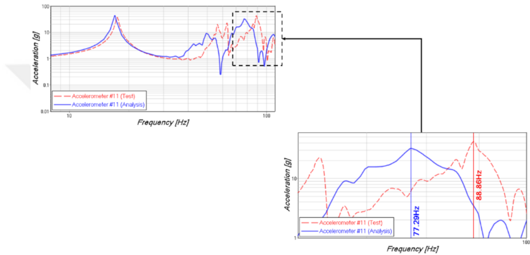
Figure 6.6. Detailed View of Reflector Bending Mode Response of Test and Analysis
