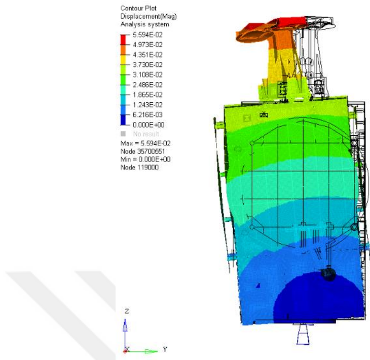
Figure 5.3. Global Y Wise Bending Mode of the Satellite
