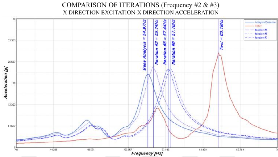
Figure 6.15. The Detailed Comparison of Iteration #3, #5 and #6 for Frequency #2 and #3
