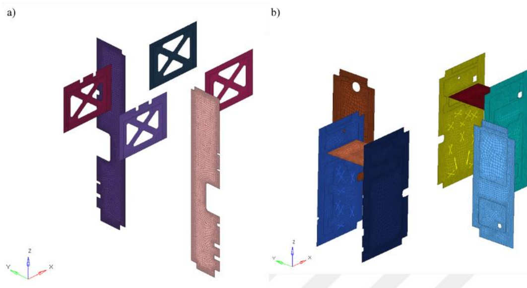
Figure 3.11. The FEM of (a) the Communication and (b) Service Shear Panels
