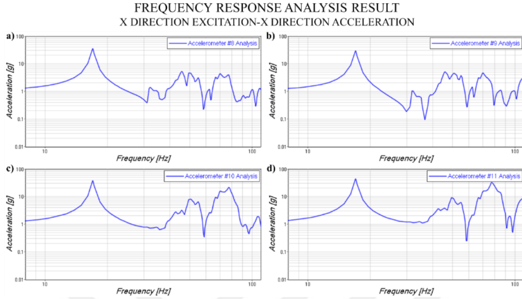
Figure 5.8. Frequency Response Analysis Transfer Function Result of Accelerometer (a) #8, (b) #9, (c) #10 and (d) #11
