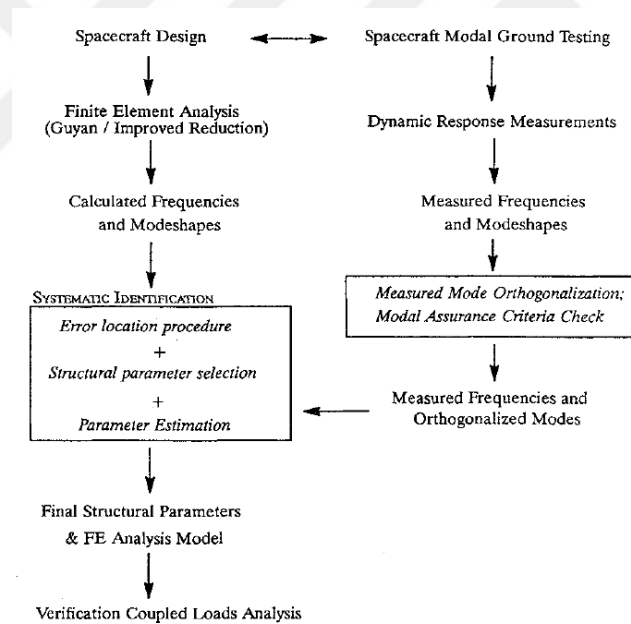
Figure 2.21. Analysis/Test Correlation for Spacecraft structures [20]
