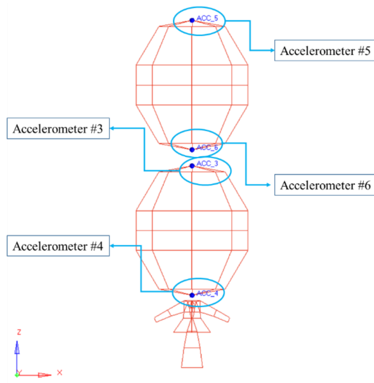
Figure 4.4. The Accelerometer Locations on Upper and Lower Tanks
