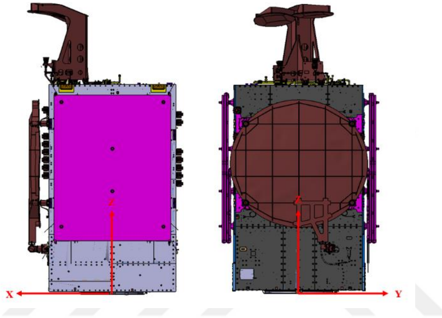
Figure 3.1. Coordinate System of the Satellite
