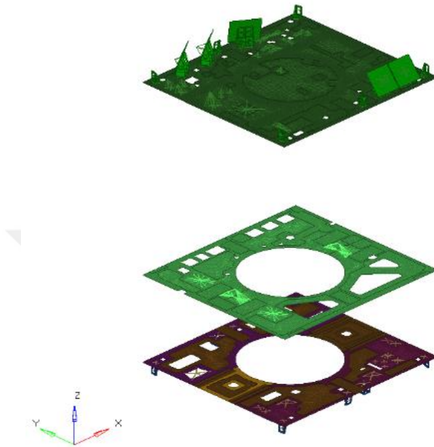
Figure 3.12. The FEM of Satellite Decks
