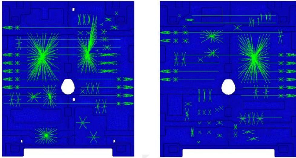
Figure 3.15. The FEM of South and North Communication Panels
