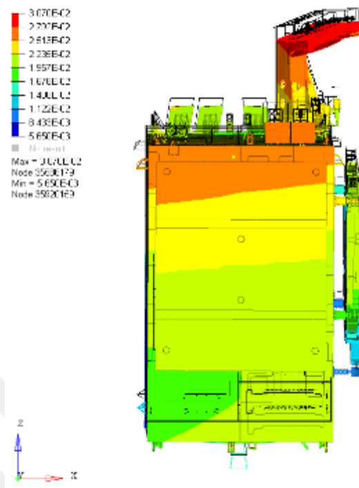
Figure 3.25. Free Boundary Condition Translational Z Result
