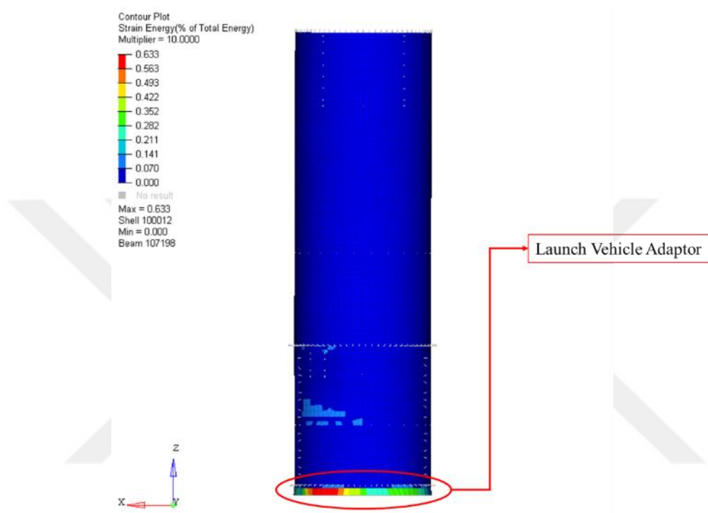
Figure 6.9. The Strain Energy Contour Plot at 16.95Hz
