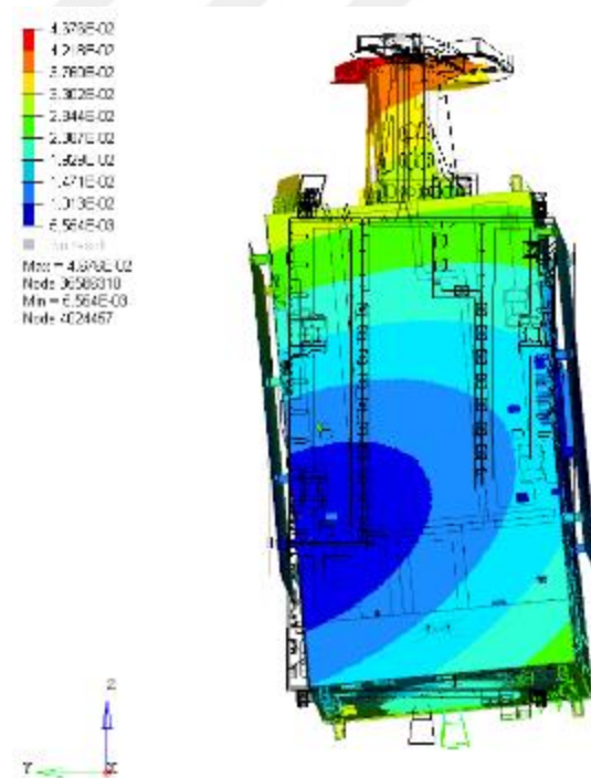
Figure 3.26. Free Boundary Condition Rotational X Result
