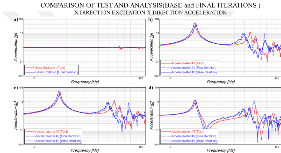
Figure 6.17. Test and Analysis (Base and Final Iterations) Transfer Function Comparison of (a) Base Excitation, Accelerometer (b) #1, (c) #2 and (d) #7
