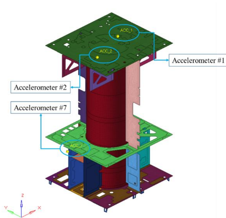
Figure 4.3. The Accelerometer Locations on Primary Structure
