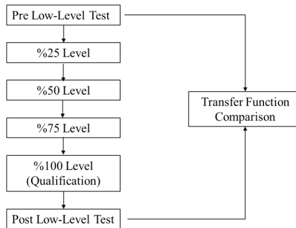
Figure 4.6. The Sine Vibration Test Steps
