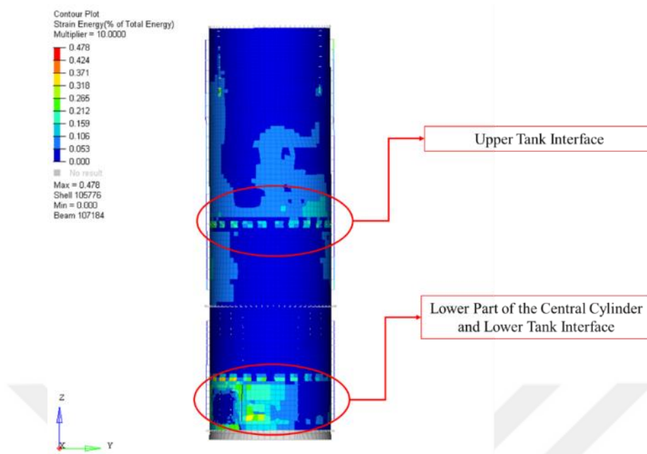
Figure 6.10. The Strain Energy Contour Plot at 48.26Hz
