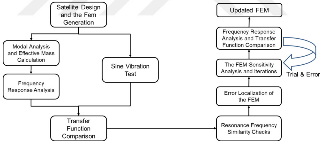
Figure 1.1. General Methodology of the Study
