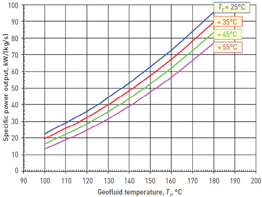
Figure 4.3 : Specific power output [in kW/(kg/s)] for low-to moderate- temperature geofluids as a function of inlet ( T_1 ) and Outlet ( T_2 ) temperatures shown in °C (MIT, 2006).
