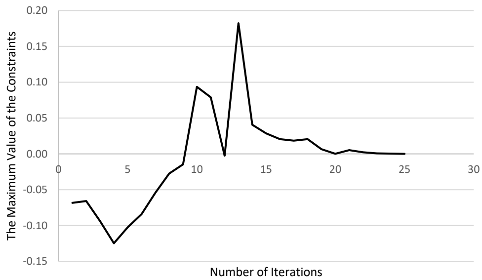
Figure 8-20 The Maximum Value of the Constraints vs Number of Iterations for Wing v2_3
