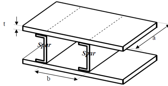
Figure 3-5 Dimensions for Buckling Analyses [27]
