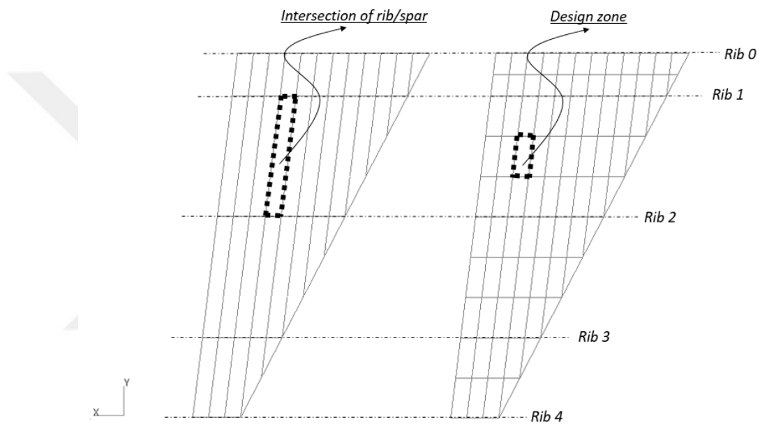
Figure 6-4 Representation of the Design Zones for v1_2
