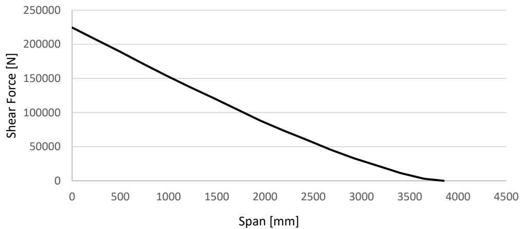
Figure 5-7 Shear Force Distribution using MSC FLDS
