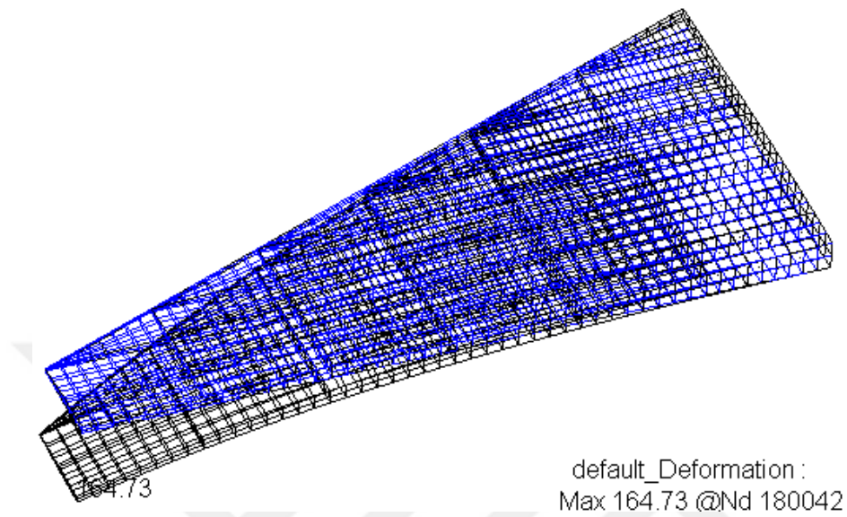
Figure 8-3 Max. Tip Displacement of Wing v1_1 with Finer Mesh
