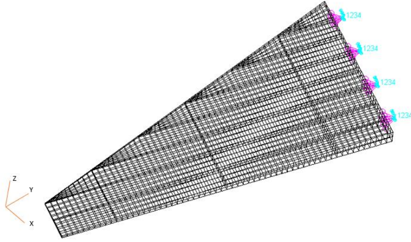
Figure 4-6 Boundary Conditions of the Wing v1_1
