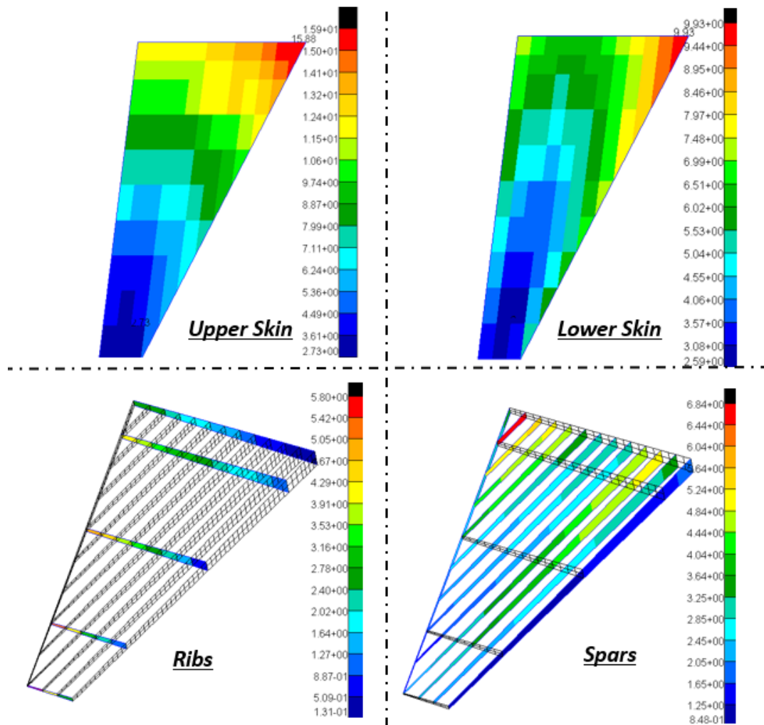
Figure 7-5 Thickness Plots of the Wing v1_2 using Quadratic 2D Shape Function
