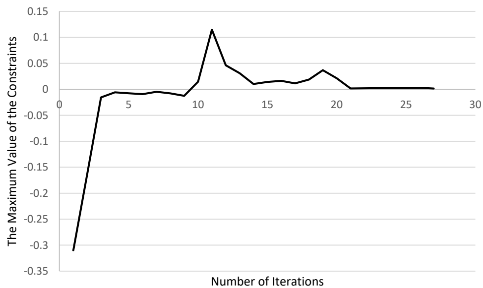
Figure 7-12 The Maximum Value of the Constraints vs Number of Iterations with Starting from the Minimum Design Variables
