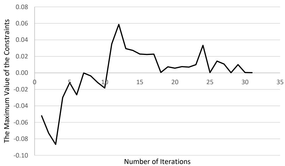
Figure 8-21 The Maximum Value of the Constraints vs Number of Iterations for Wing v3_1
