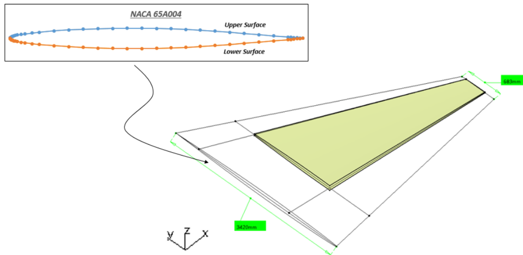
Figure 4-1 Airfoil Profile and the Outer Geometry of the Wing
