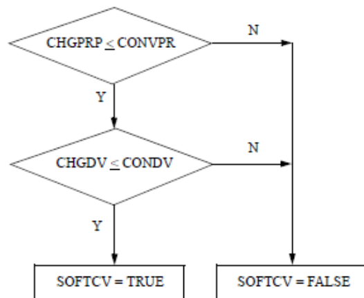
Figure 2-4 Logic for the Soft Convergence Decision [12]
