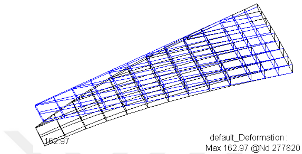
Figure 8-1 Max. Tip Displacement of Wing v1_1 with Coarse Mesh
