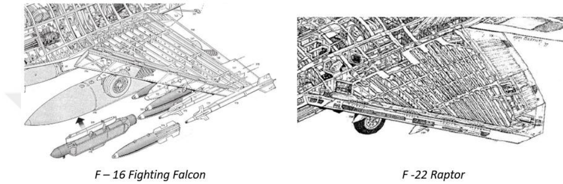
Figure 3-4 Representation for Multi-Spar Configuration [25], [26]
