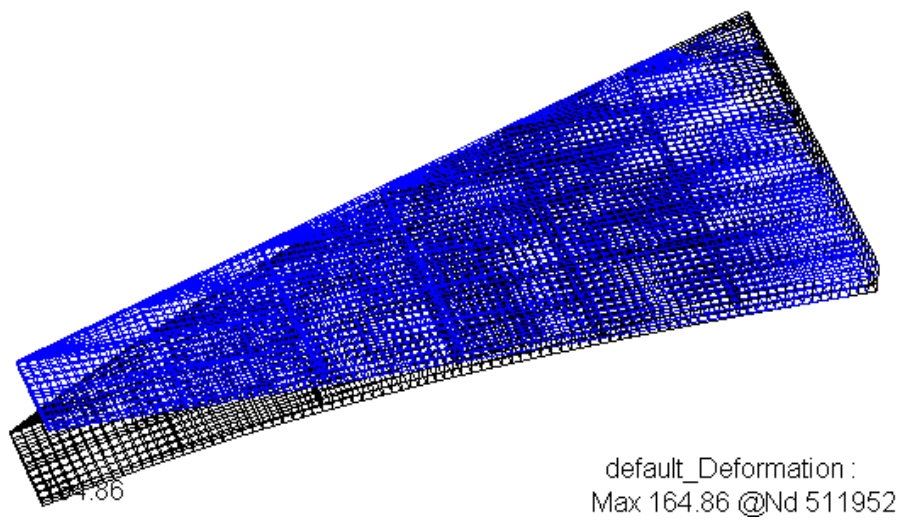
Figure 8-4 Max. Tip Displacement of Wing v1_1 with the Finest Mesh
