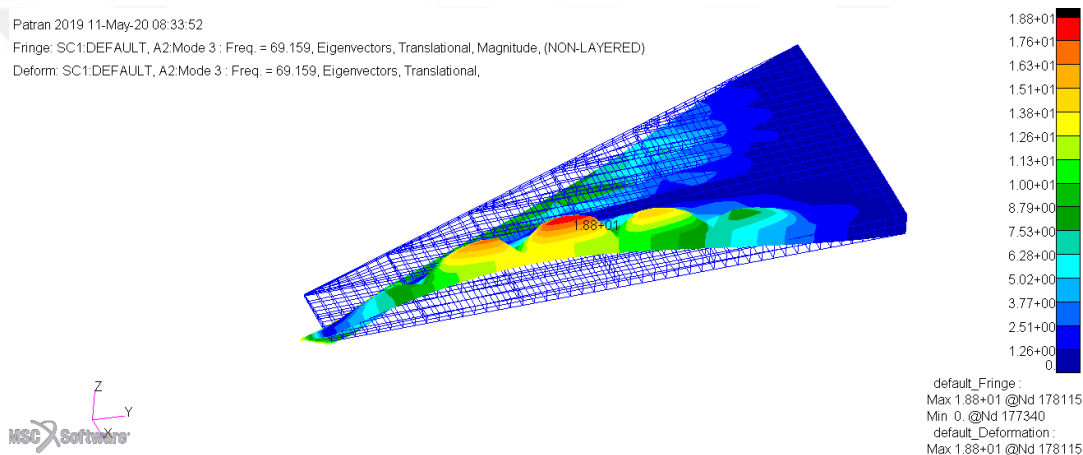
Figure 4-9 The First Torsion Mode Shape of the Wing v1_1
