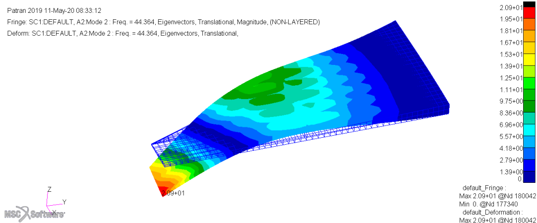
Figure 4-8 Bending-Torsion Coupling Mode Shape of the Wing v1_1
