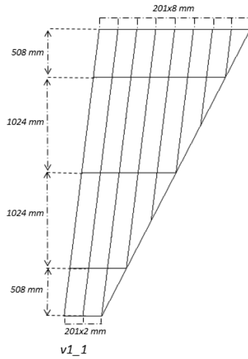
Figure 3-7 The First Candidate of Family 1 (v1_1)
