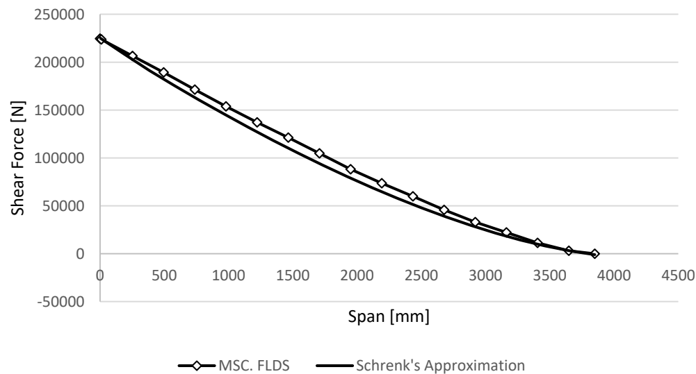
Figure 5-12 Comparison of Two Method for the Shear Force Distribution
