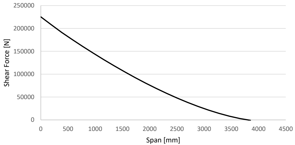
Figure 5-10 Shear Force Distribution along Wing Span using Schrenk's Approximation
