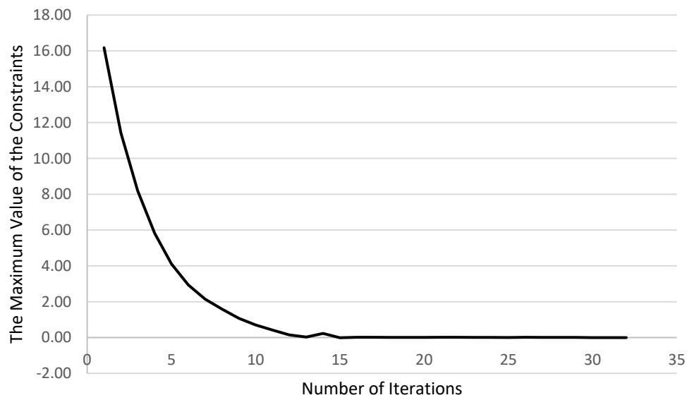
Figure 7-12 The Maximum Value of the Constraints vs Number of Iterations with Starting from the Minimum Design Variables
