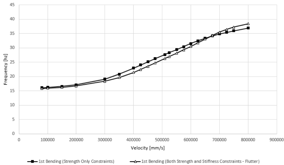
Figure 7-19 Velocity – Frequency Curves Before and After Optimization with Both Strength and Stiffness (Flutter) Constraint
