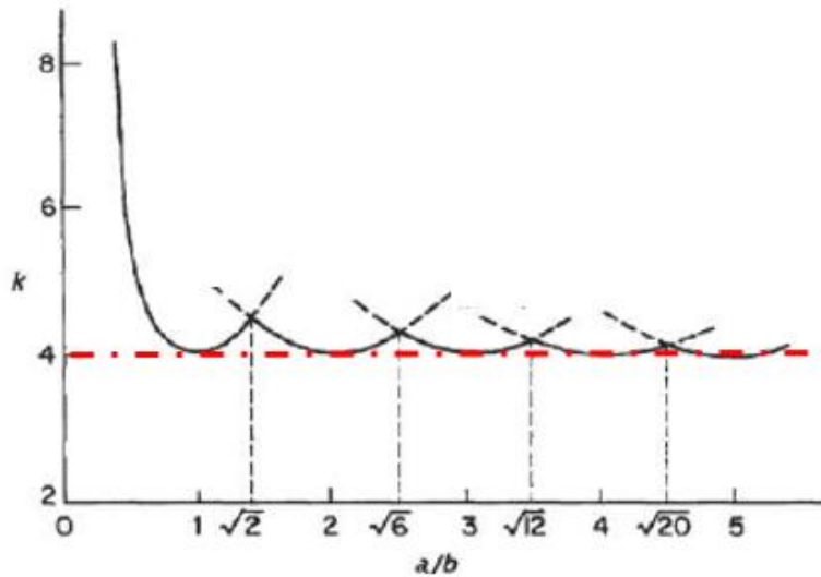
Figure 3-6 The Distribution of Buckling Coefficient for Simply Supported Conditions [28]
