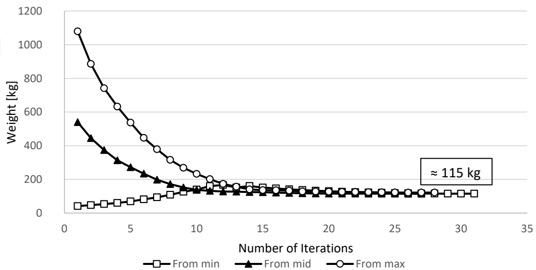
Figure 7-10 Convergence History for Wing v1_2 with Strength-Only Constraints
