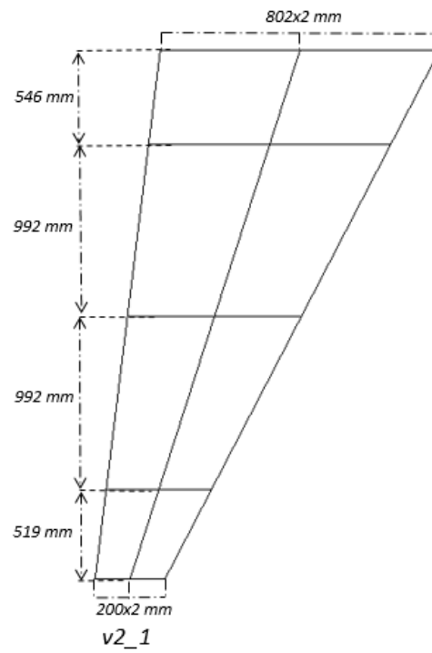
Figure 3-9 The First Candidate of Family 2 (v2_1)
