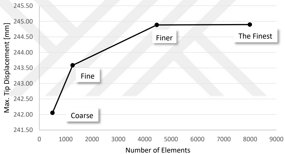
Figure 8-9 Mesh Convergence Results for Wing v3_1
