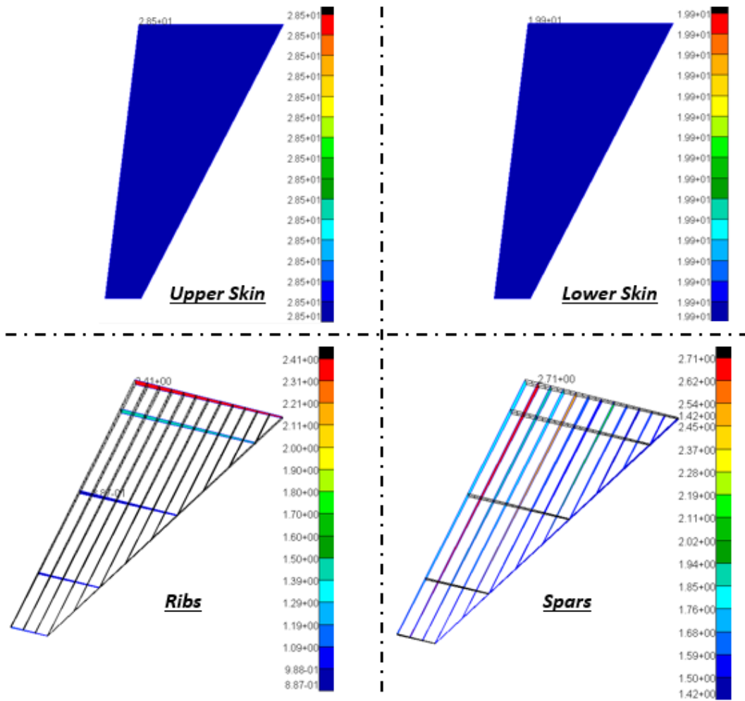
Figure 7-2 Thickness Plots of the Wing v1_2 using Constant Shape Function
