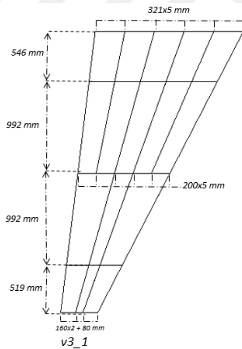
Figure 3-12 The First Candidate of Family 3 (v3_1)
