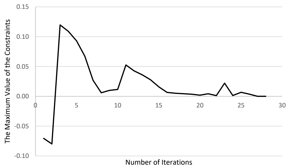
Figure 8-22 The Maximum Value of the Constraints vs Number of Iterations for Wing v3_2
