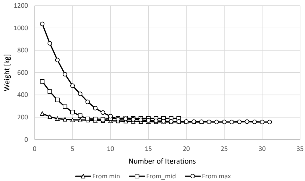
Figure 8-15 Convergence History for Wing v3_1 with Strength-Only Constraints
