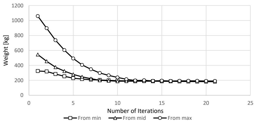
Figure 8-11 Convergence History for Wing v1_1 with Strength-Only Constraints
