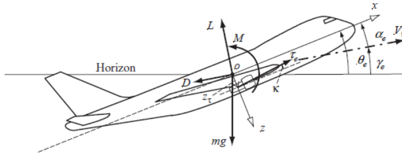
Figure 5-3 Longitudinal Forces Acting on the Aircraft [45]
