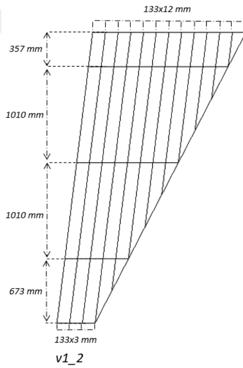
Figure 3-8 The Second Candidate of Family 1 (v1_2)
