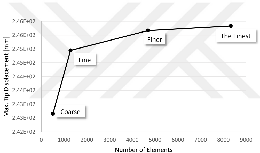
Figure 8-10 Mesh Convergence Results for Wing v3_2
