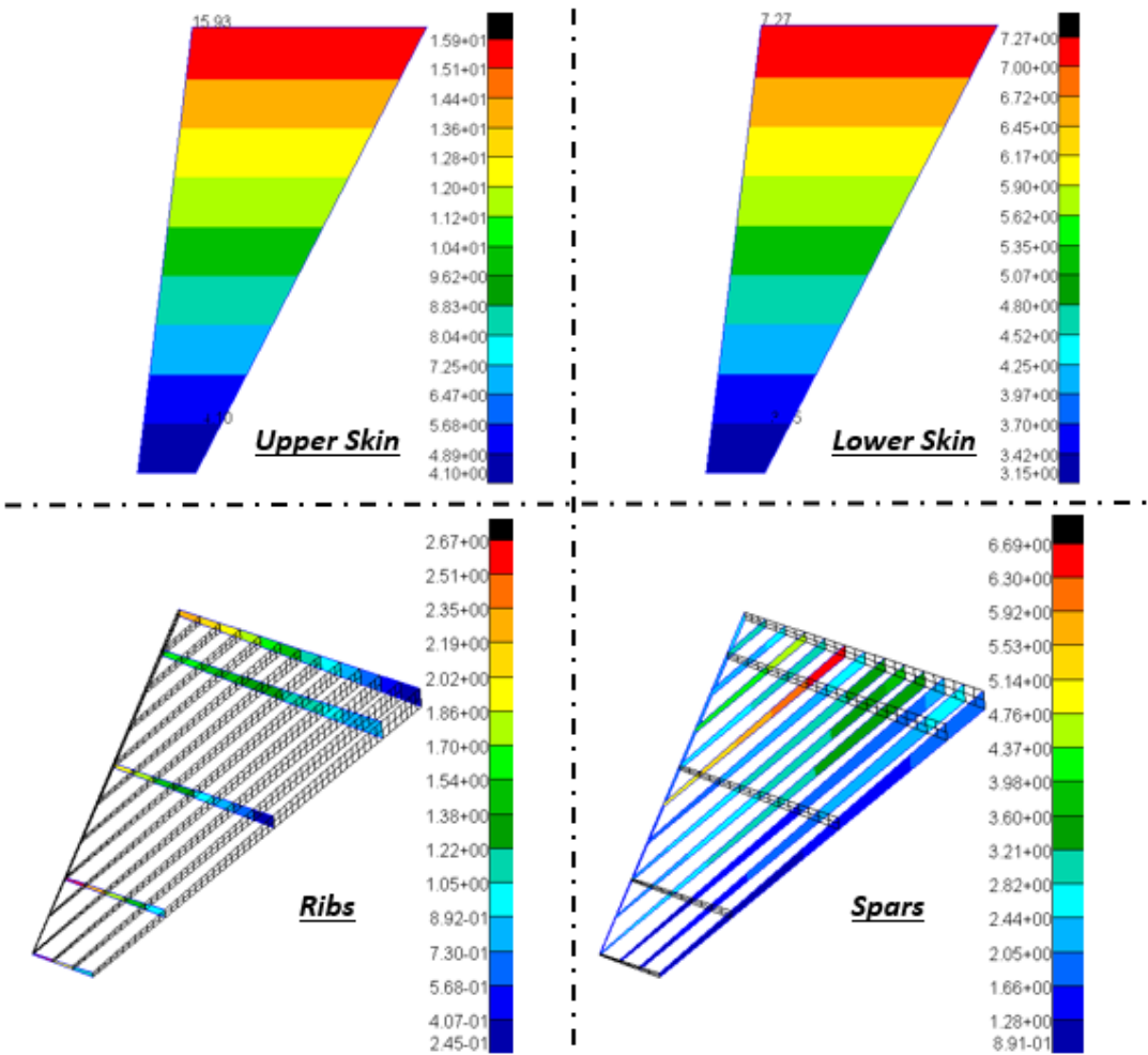
Figure 7-3 Thickness Plots of the Wing v1_2 using Linear Shape Function
