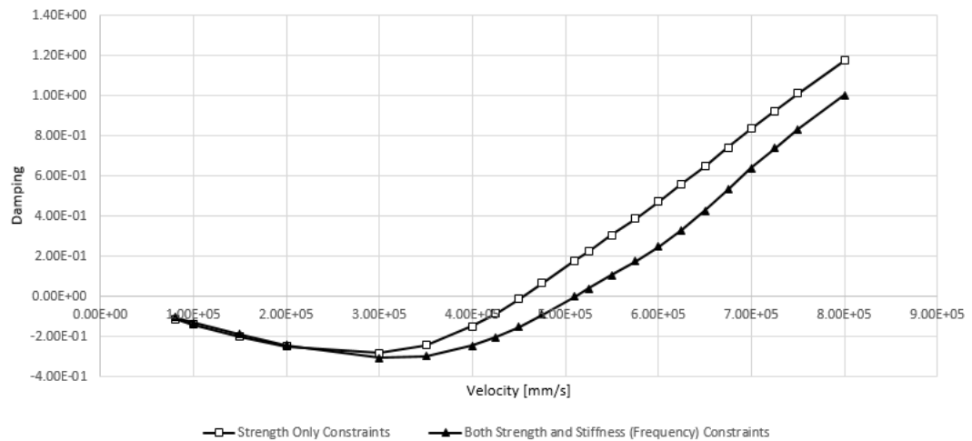
Figure 7-20 Velocity – Damping Curves Before and After Optimization with Both Strength and Stiffness (Frequency) Constraints
