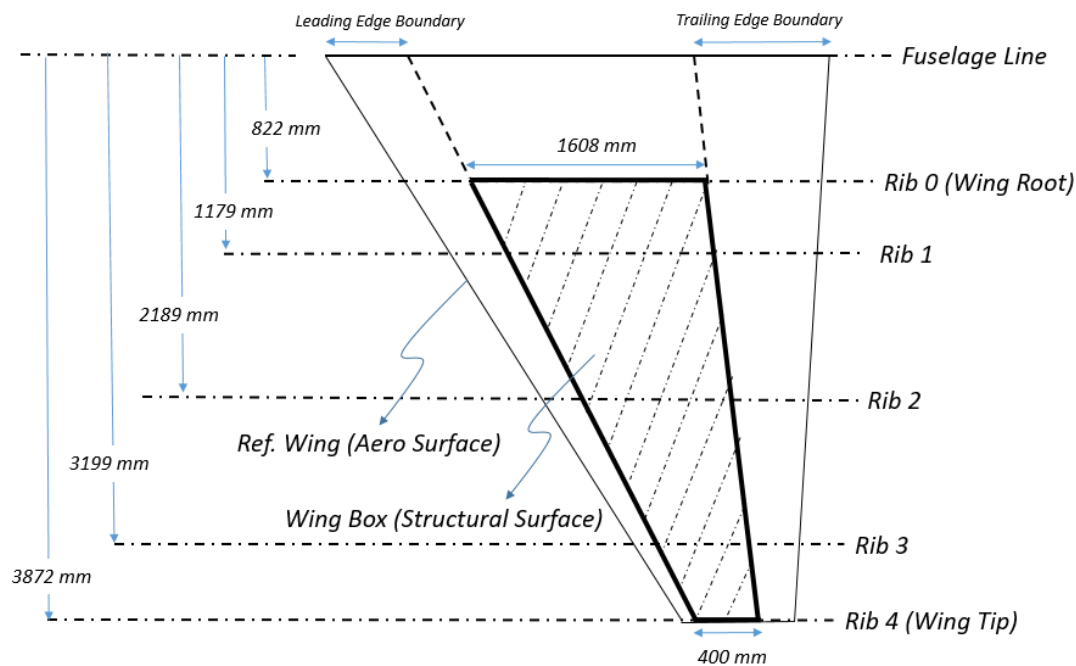
Figure 3-1 General Structural and Aerodynamic Borders of Wing Geometry
