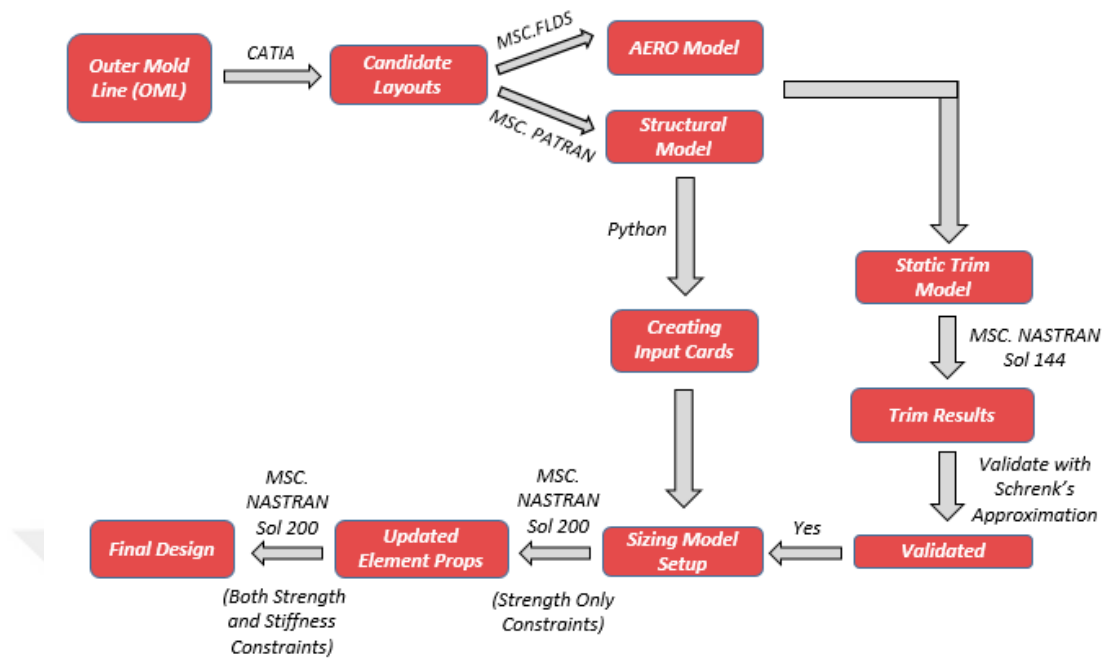
Figure 6-5 Analysis Process Applied to Each Wing
