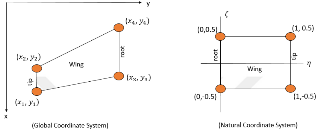
Figure 6-2 An Isoparametric Element in two Different Coordinate Systems
