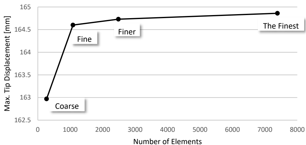
Figure 4-3 Mesh Convergence Results for Wing v1_1
