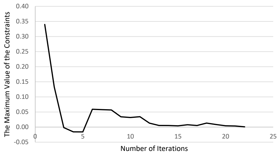
Figure 8-17 The Maximum Value of the Constraints vs Number of Iterations for Wing v1_1
