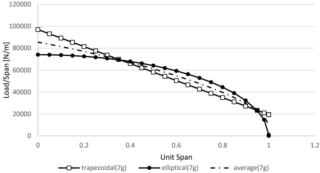
Figure 5-9 Lift Distribution along Unit Span with Schrenk's Approximation
