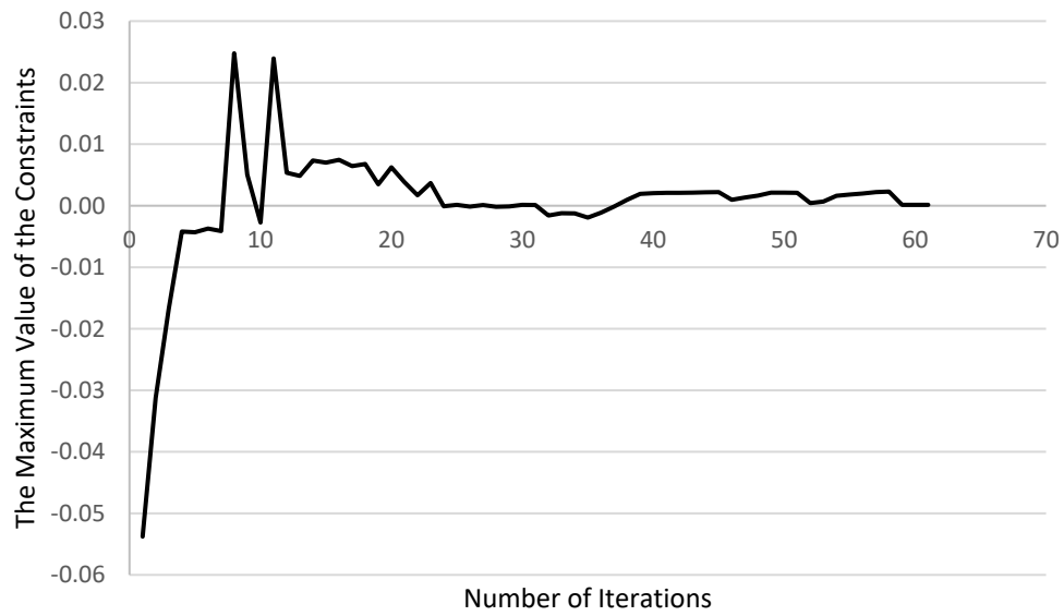
Figure 8-18 The Maximum Value of the Constraints vs Number of Iterations for Wing v2_1
