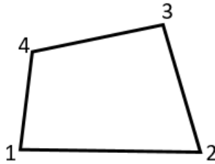
Figure 6-3 Numbering Sketch for Quadrangle Isoparametric Element
