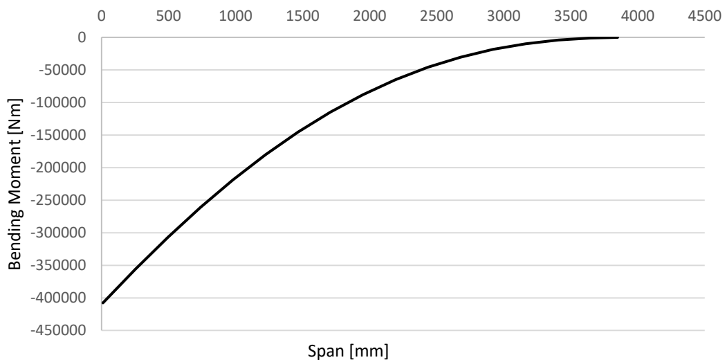
Figure 5-8 Bending Moment Distribution using MSC FLDS
