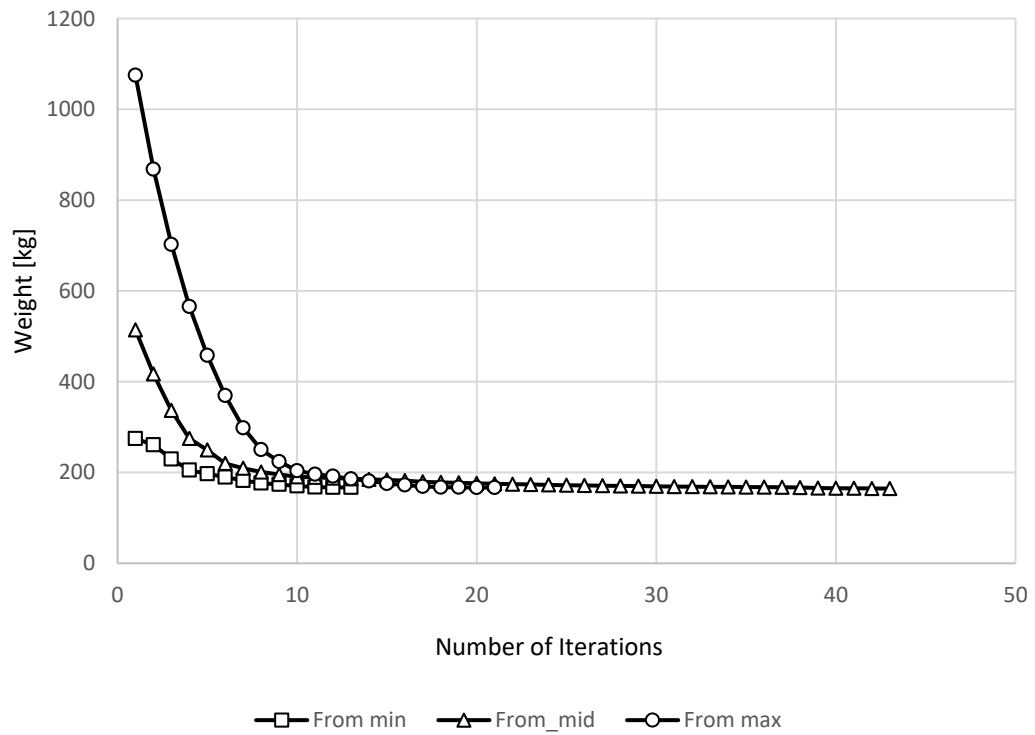
Figure 8-14 Convergence History for Wing v2_3 with Strength-Only Constraints
