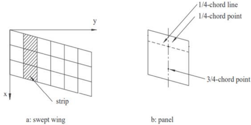
Figure 5-1 Surface Representation by Quadrilateral Elements [41]
