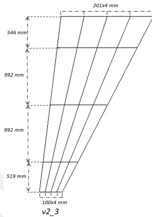
Figure 3-11 The Third Candidate of Family 2 (v2_3)
