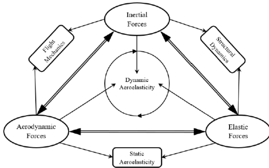
Figure 2-7 Collar's Aeroelasticity Triangle [17]
