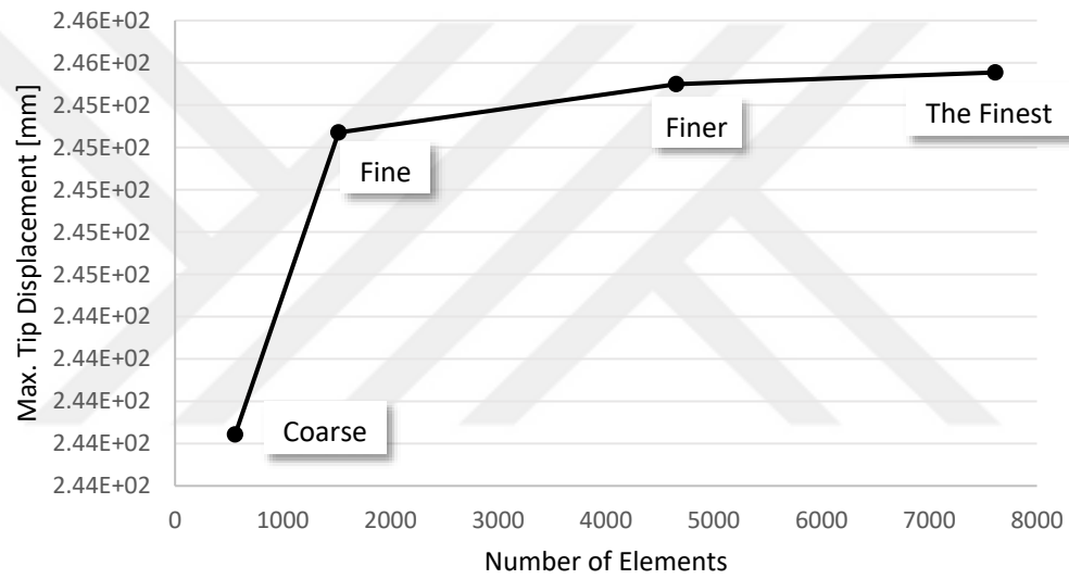
Figure 8-7 Mesh Convergence Results for Wing v2_2
