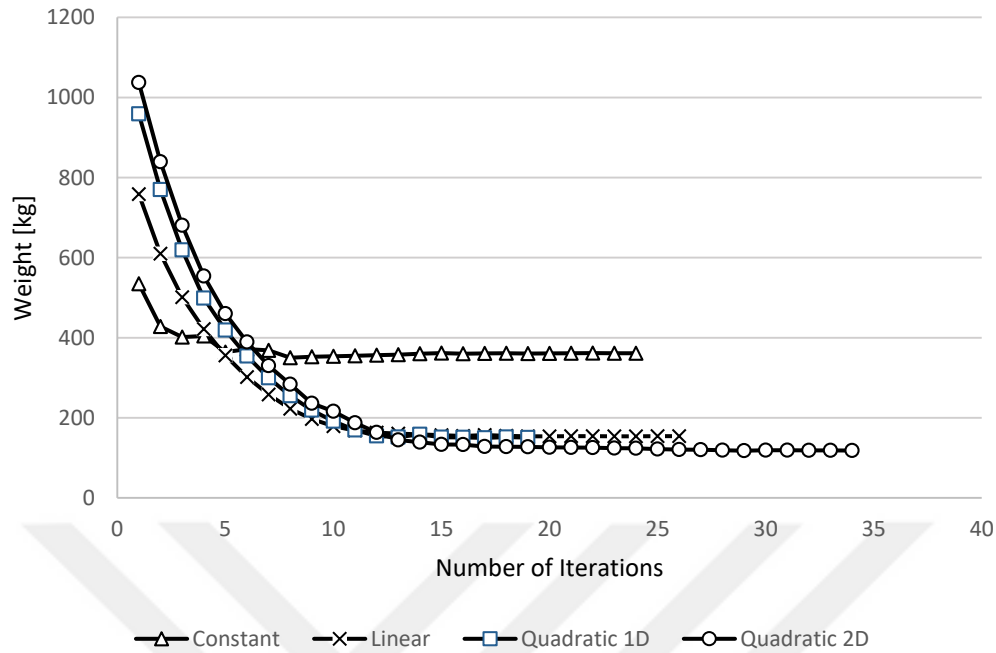
Figure 7-1 Iterations till Converged Results
