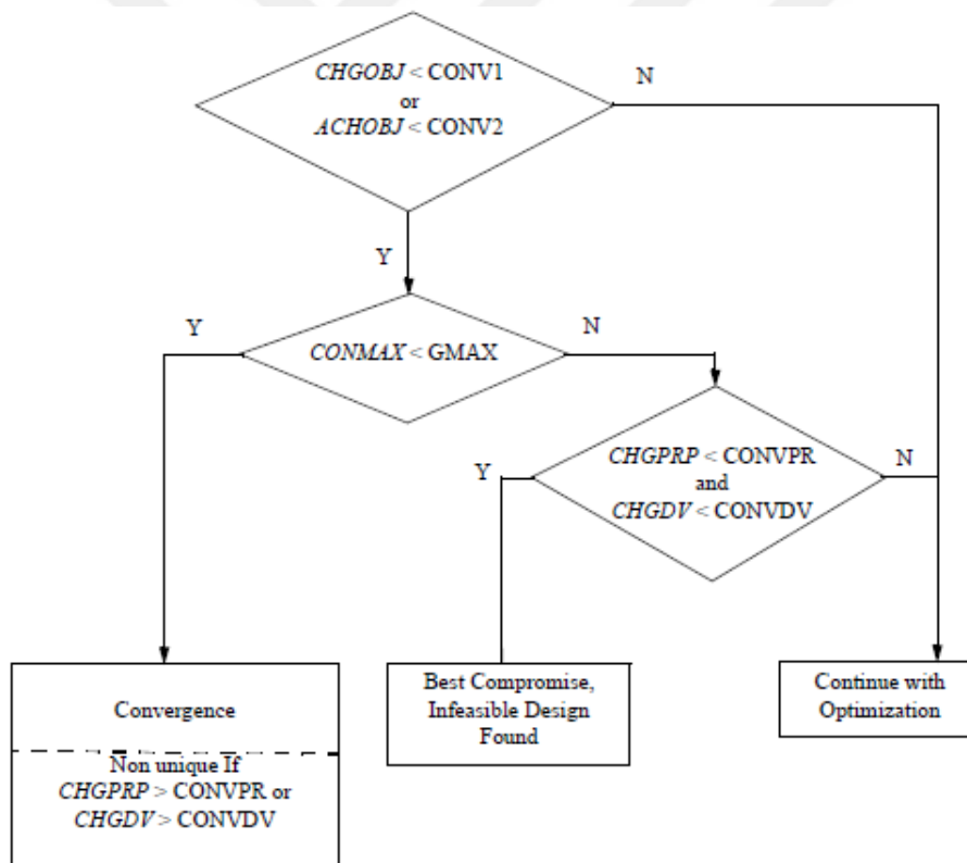
Figure 2-5 Logic for the Hard Convergence Decision [12]
