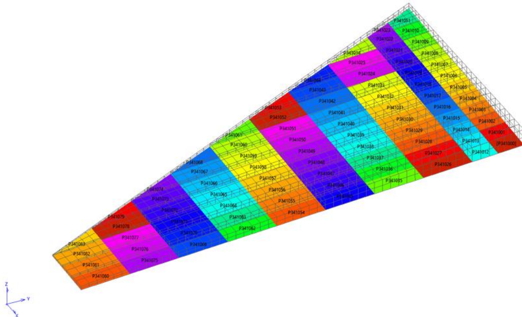
Figure 7-7 Design Zones for Lower Skin of the Wing v1_2
