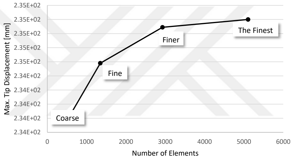
Figure 8-5 Mesh Convergence Results for Wing v1_2
