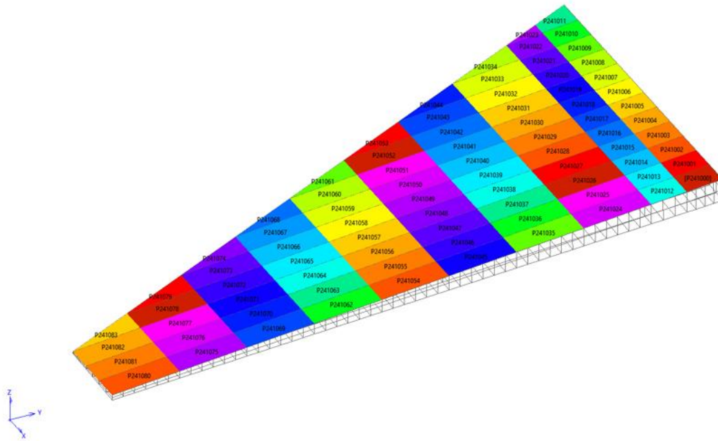
Figure 7-6 Design Zones for Upper Skin of the Wing v1_2
