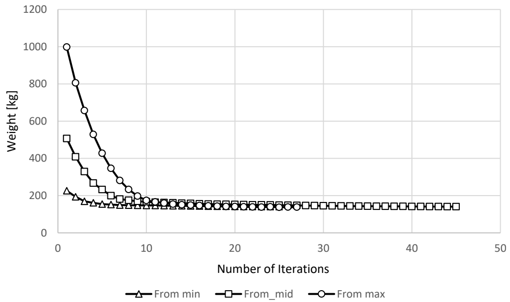
Figure 8-16 Convergence History for Wing v3_2 with Strength-Only Constraints
