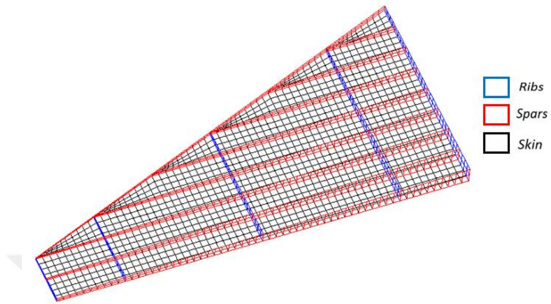
Figure 4-5 Main Structural Components of the Wing v1_1
