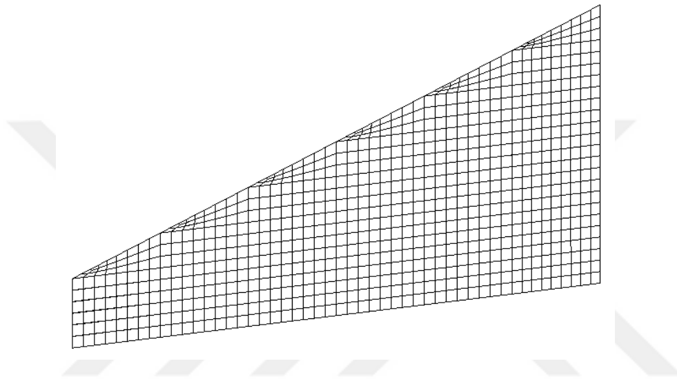
Figure 4-4 Finite Element Model of the Wing v1_1 (Top view)
