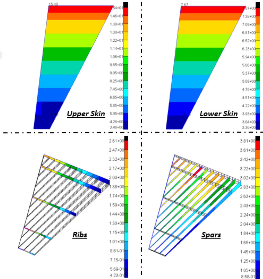
Figure 7-4 Thickness Plots of the Wing v1_2 using Quadratic 1D Shape Function
