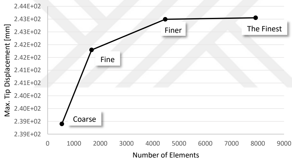
Figure 8-8 Mesh Convergence Results for Wing v2_3
