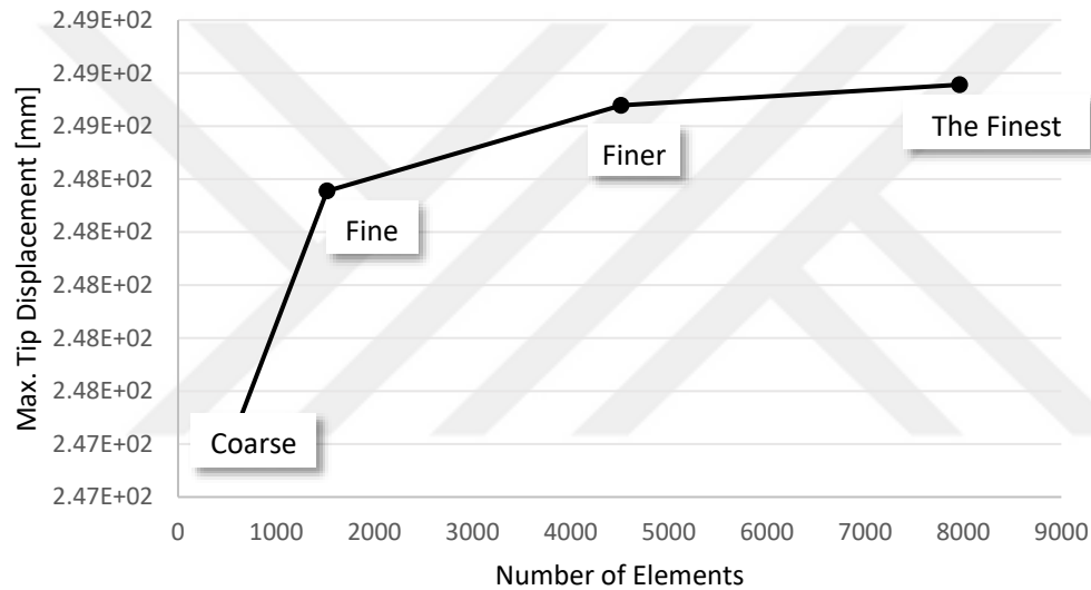
Figure 8-6 Mesh Convergence Results for Wing v2_1
