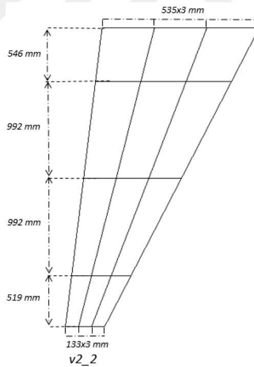
Figure 3-10 The Second Candidate of Family 2 (v2_2)
