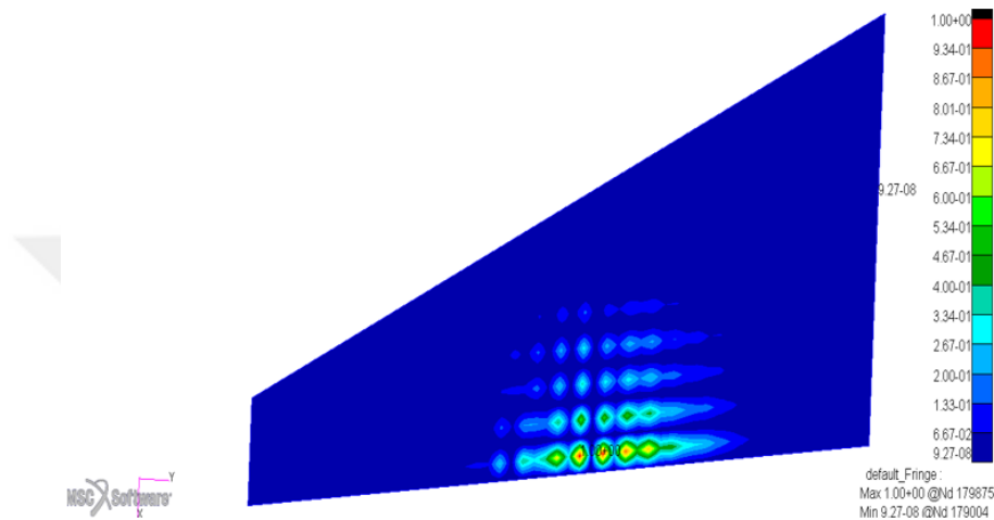
Figure 7-15 Minimum Buckling Eigenvalues for the Upper Skin after the Optimization
