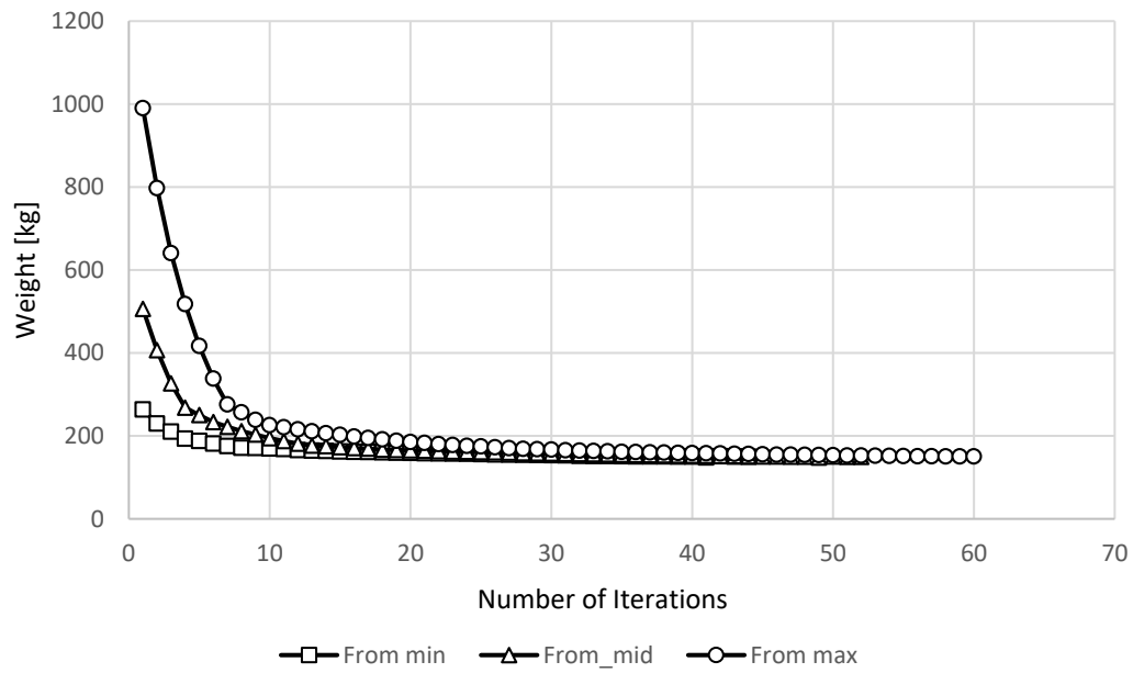
Figure 8-13 Convergence History for Wing v2_2 with Strength-Only Constraints
