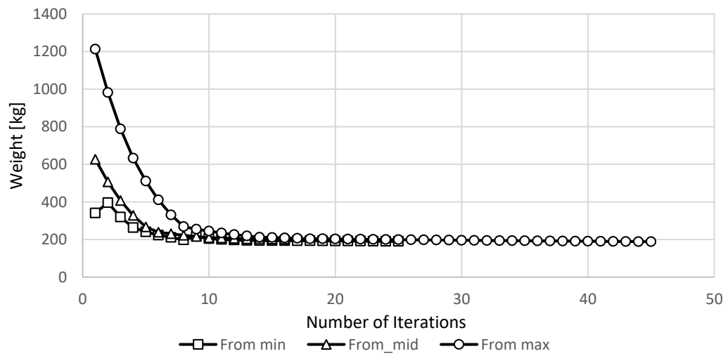
Figure 8-12 Convergence History for Wing v2_1 with Strength-Only Constraints
