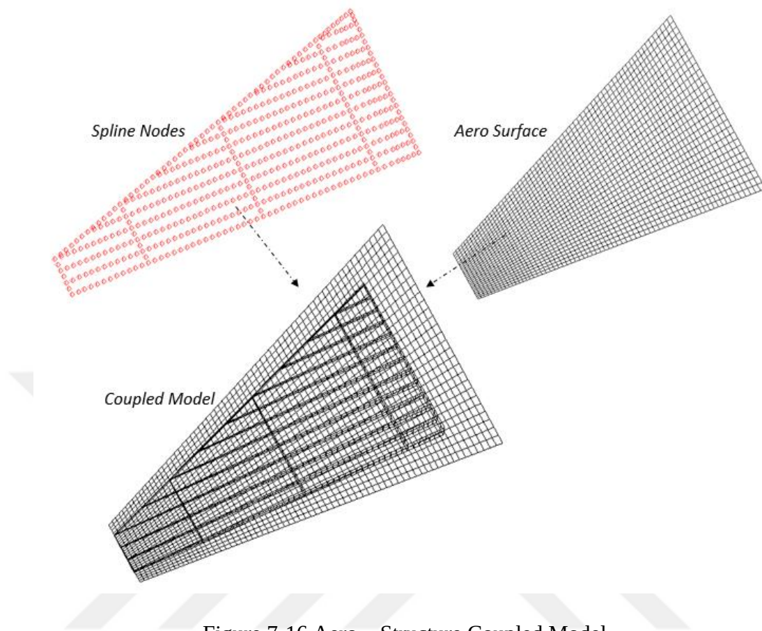
Figure 7-16 Aero – Structure Coupled Model
