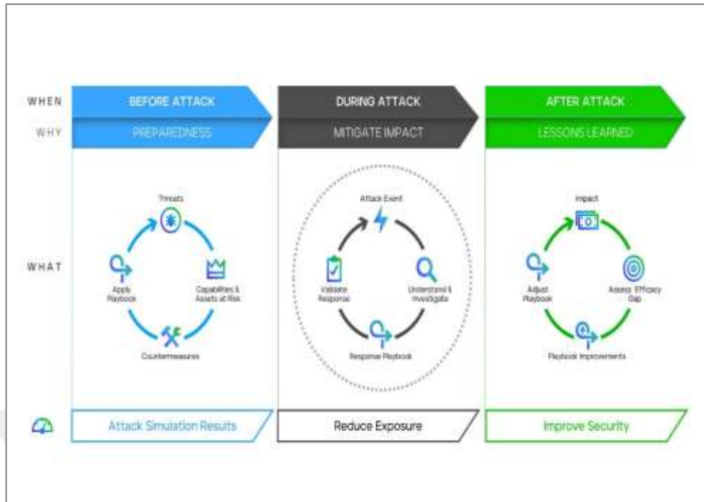
Figure 2.5: Adaptive Defense.
