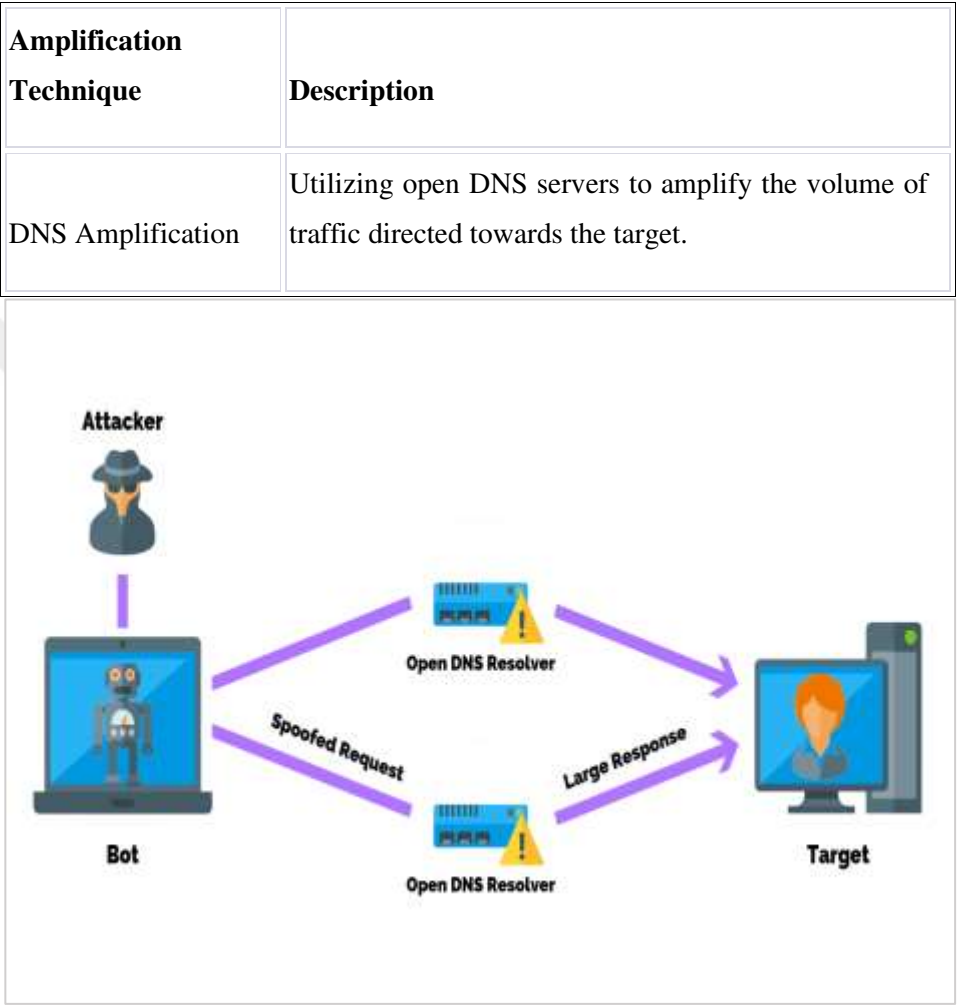
Figure 2.16: DNS Amplification.
