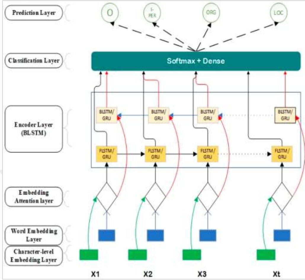
Figure 2.14: BRNN.
