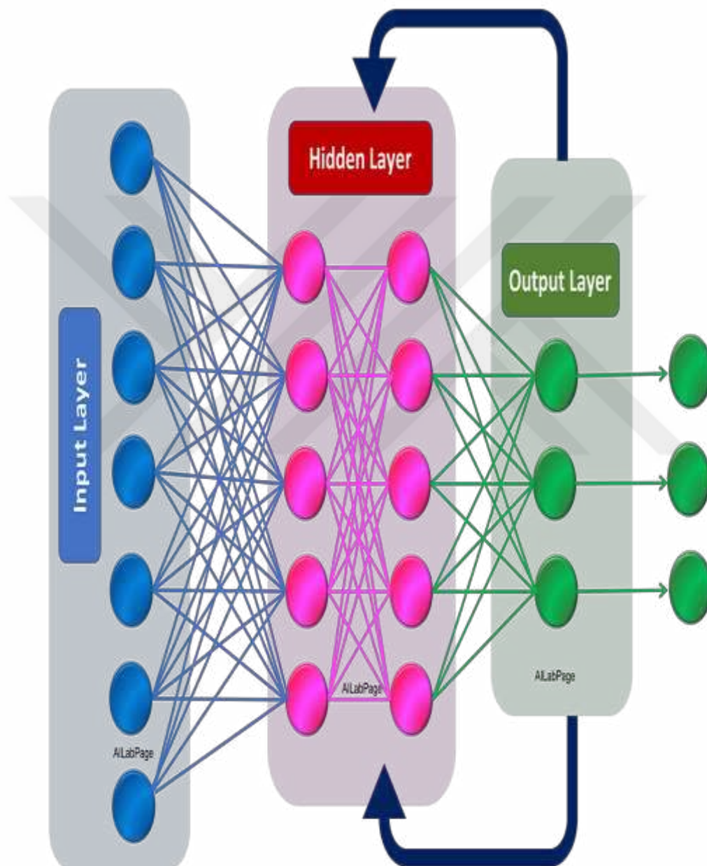
Figure 2.13: Simple RNN.
