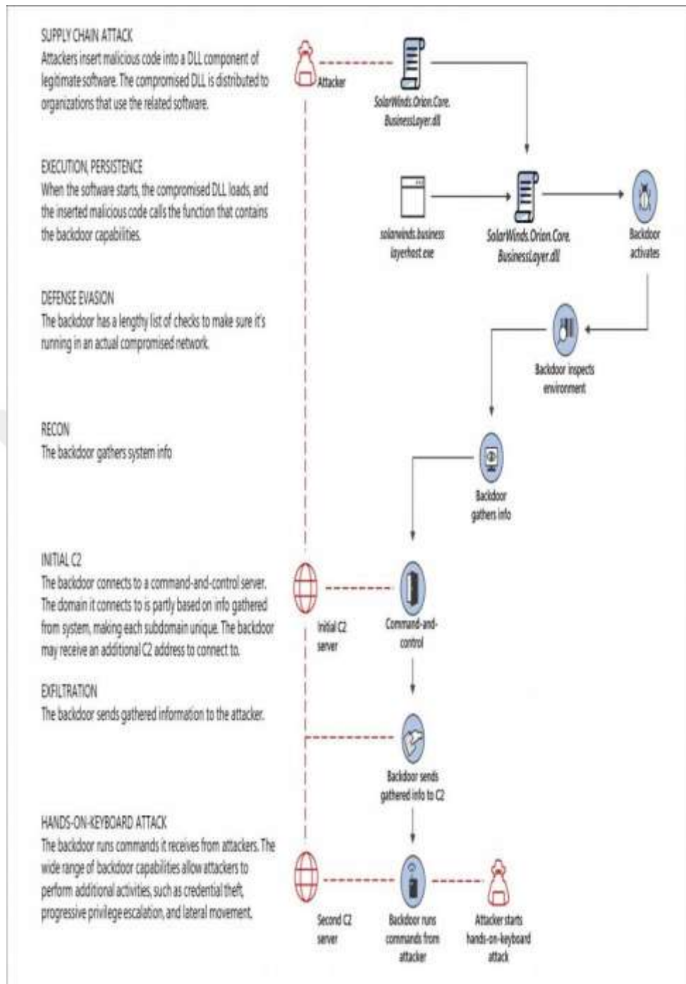
Figure 2.2: Solarwinds Example.
