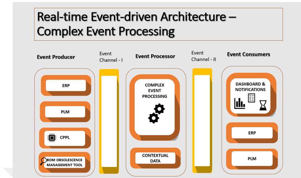
Figure 5.1 Architecture for CEP to administer OM processes in the Company
