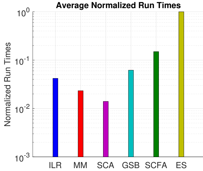
Figure 4.10: Average Complexity Comparison (K, N, L) = (3, 3, 2) .
