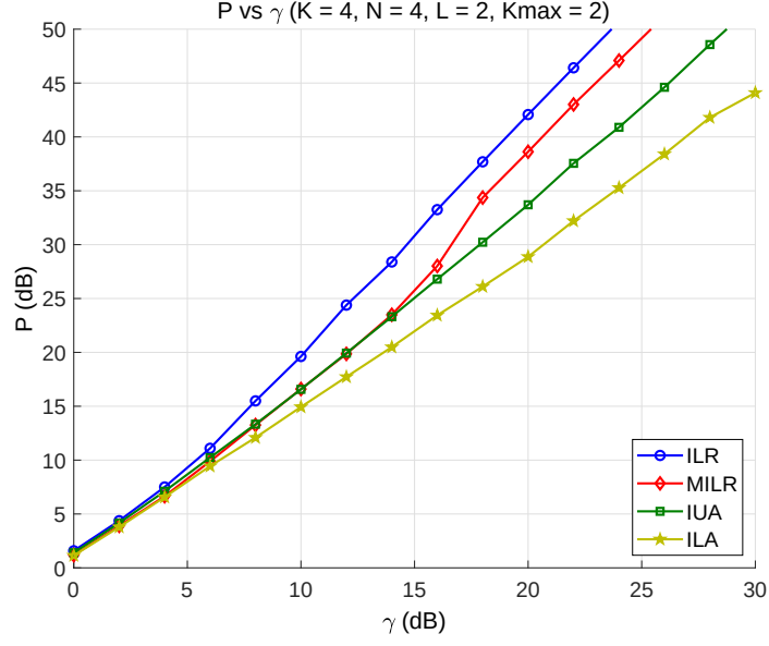
Figure 3.2: P vs \gamma . K = 4, N = 4, L = 2, K_{\max} = 2 .
