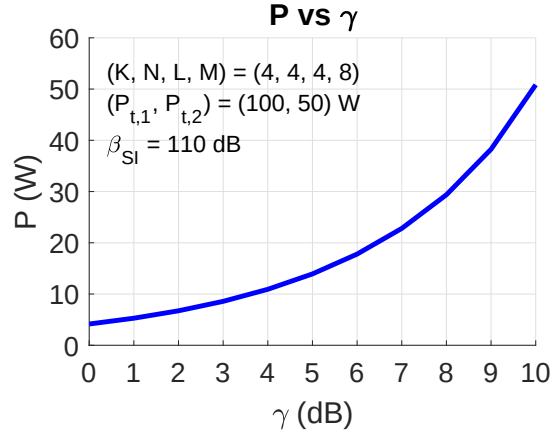
Figure 7.2: P vs \gamma , (K, N, L, M) = (4, 4, 4, 8) , (P_{t,1}, P_{t,2}) = (100, 50) W, \beta_{SI} = 110 dB.
