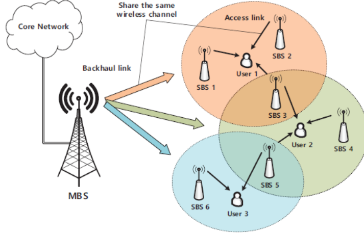
Figure 2.3: A typical full-duplex IAB system diagram [14].
