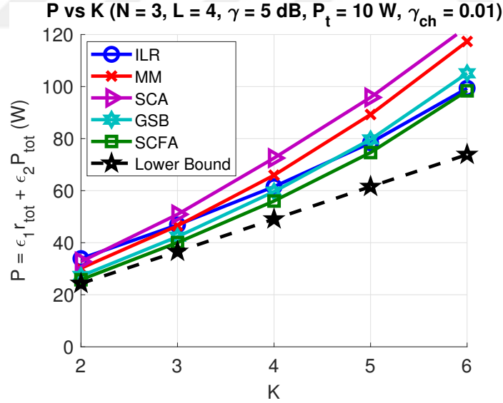
Figure 4.3: P vs K . N = 3, L = 4, \gamma = 5\text{ dB}, P_t = 10\text{W}, \gamma_{\text{ch}} = 0.01 .
