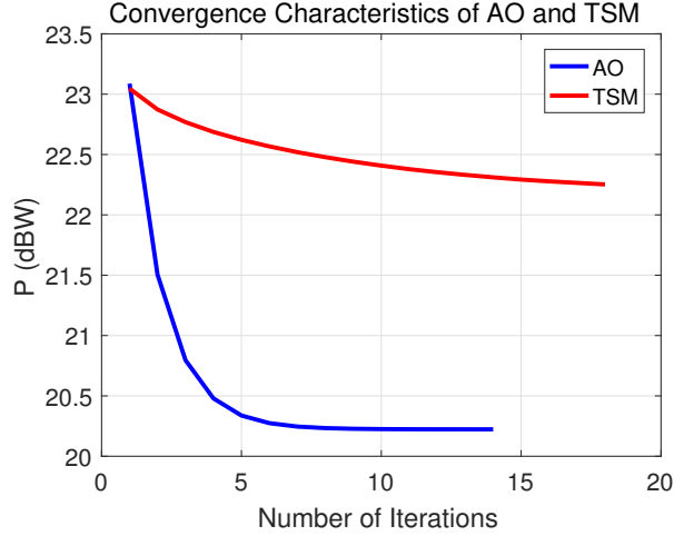
Figure 6.1: Convergence characteristics of AO and TSM.
