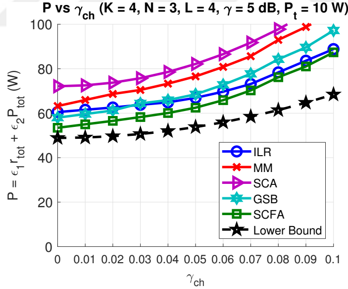
Figure 4.6: P vs \gamma_{ch} . K = 4, N = 3, L = 4, \gamma = 5 dB, P_t = 10 W.
