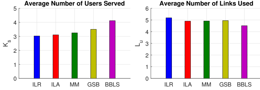
Figure 5.2: Average Number of UEs Served (Left) and Average Number of Links Used (Right).
