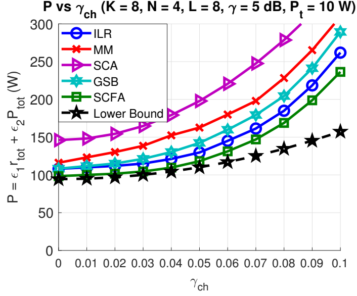
Figure 4.7: P vs \gamma_{ch} . K = 8, N = 4, L = 8, \gamma = 5 dB, P_t = 10 W.
