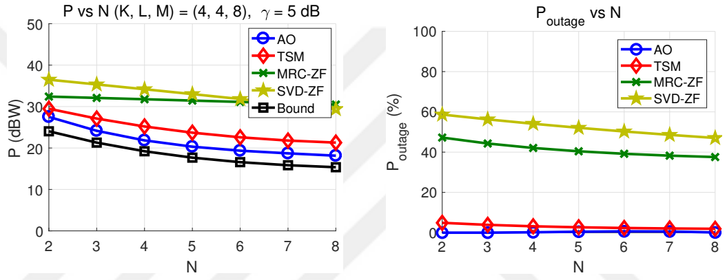
Figure 6.4: P and P_{\text{outage}} vs N . (K, L, M) = (4, 4, 8) , \gamma = 5 dB, \gamma_{\text{ch}} = 0.01 .
