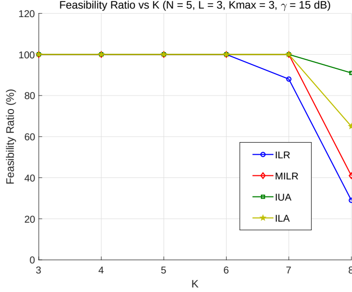
Figure 3.4: Feasibility Ratio vs K . N = 5, L = 3, K_{\max} = 3, \gamma = 15 dB.
