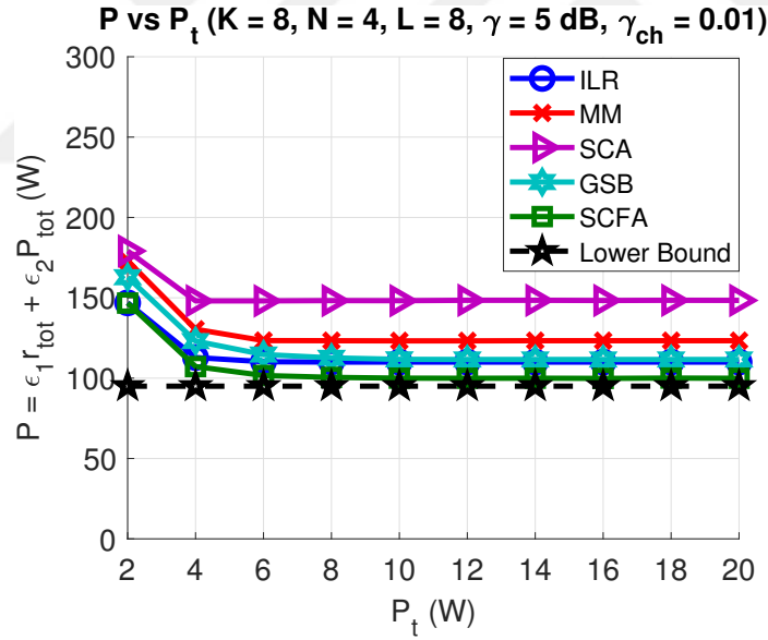
Figure 4.9: P vs P_t . K = 8, N = 4, L = 8, \gamma = 5 \text{ dB}, \gamma_{\text{ch}} = 0.01 .
