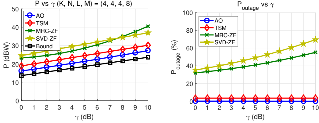
Figure 6.2: P and P_{\text{outage}} vs \gamma . ( K, N, L, M ) = (4, 4, 4, 8), \gamma_{\text{ch}} = 0.01 .
