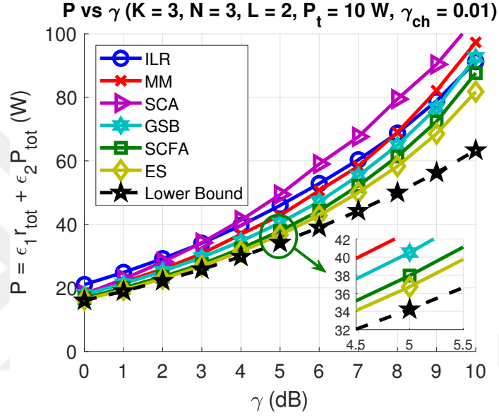
Figure 4.1: P vs \gamma . K = 3, N = 3, L = 2, P_t = 10\text{W}, \gamma_{\text{ch}} = 0.01 .
