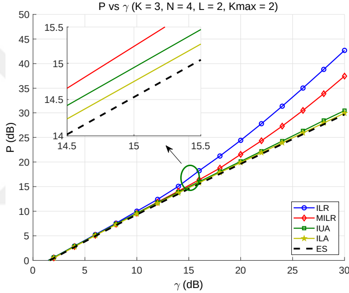
Figure 3.1: P vs \gamma . K = 3, N = 4, L = 2, K_{\max} = 2 .
