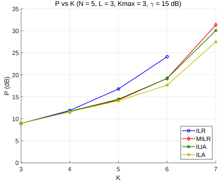
Figure 3.3: P vs K . N = 5, L = 3, K_{\max} = 3, \gamma = 15 dB.
