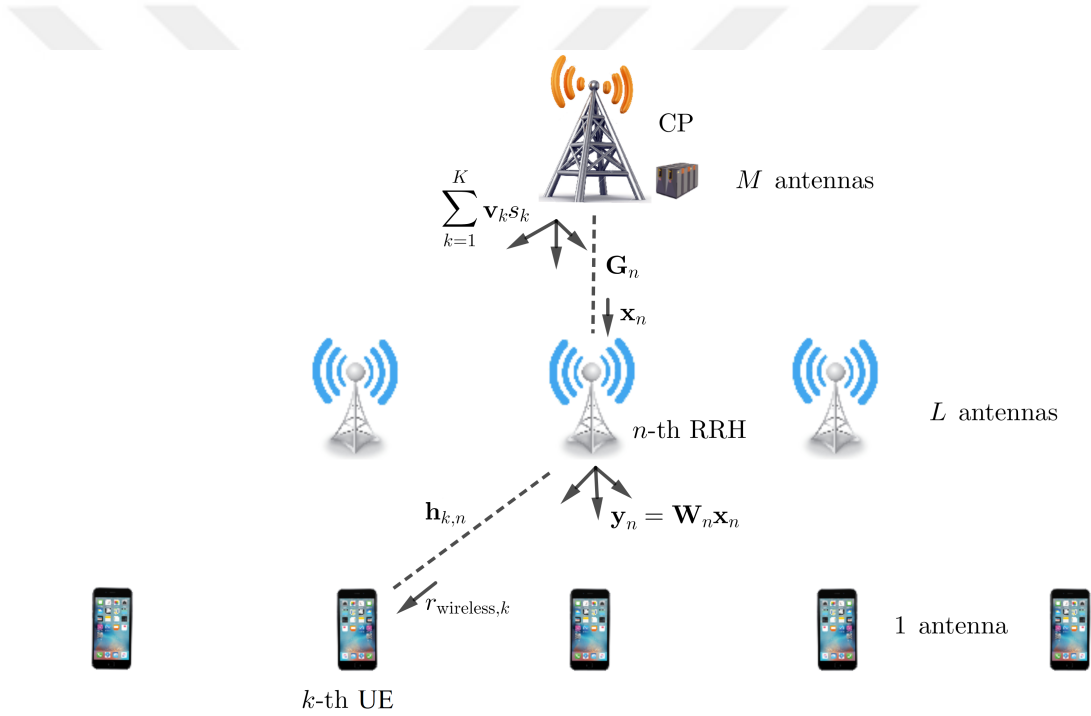
Figure 2.2: Block Diagram of Downlink C-RAN with Wireless Fronthaul.
