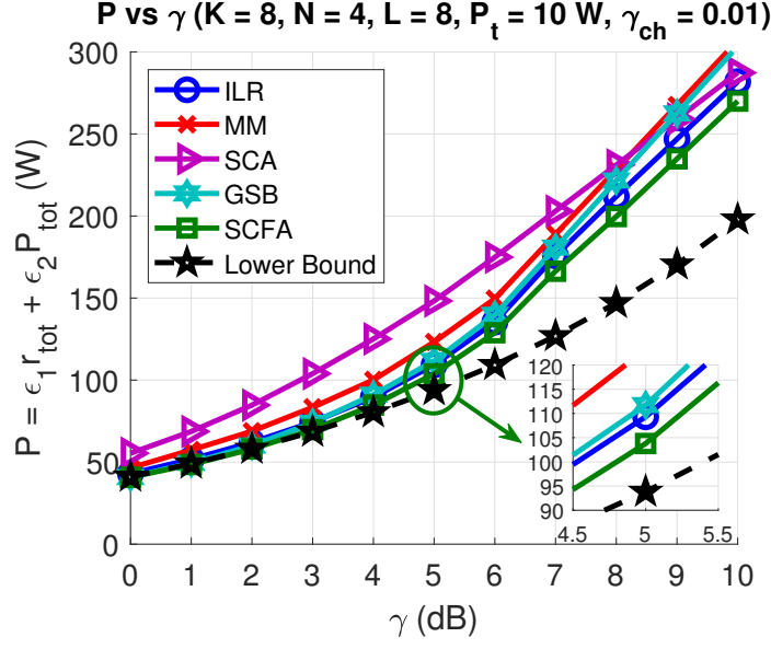
Figure 4.2: P vs \gamma . K = 8, N = 4, L = 8, P_t = 10\text{W}, \gamma_{\text{ch}} = 0.01 .
