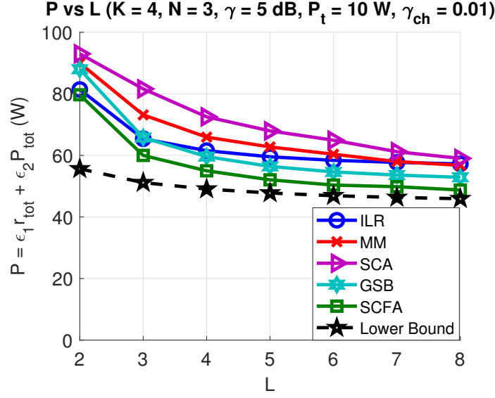
Figure 4.5: P vs L . K = 4, N = 3, \gamma = 5 dB, P_t = 10 W, \gamma_{ch} = 0.01 .
