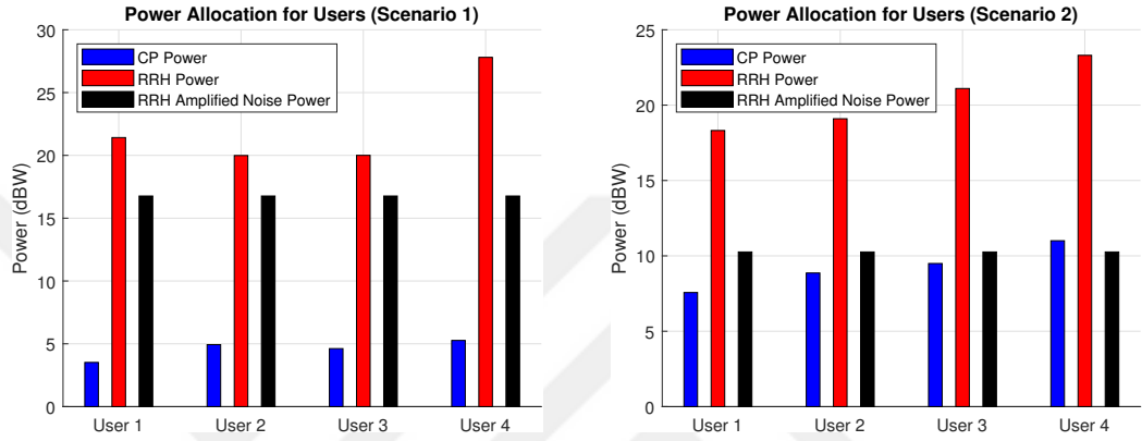
Figure 6.10: Power Allocations for Scenario 1 (left) and Scenario 2 (right).
