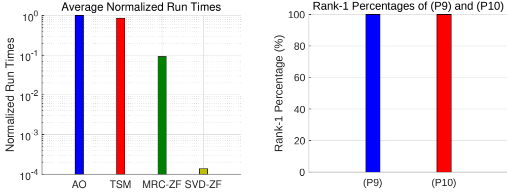
Figure 6.8: Average Complexity Comparison (left) and Rank-1 Percentages of (P9) and (P10) (right).
