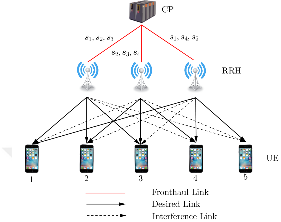
Figure 2.1: A block diagram of a downlink C-RAN with wired fronthaul.
