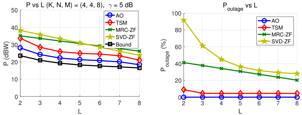
Figure 6.5: P and P_{\text{outage}} vs L . (K, N, M) = (4, 4, 8) , \gamma = 5 dB, \gamma_{\text{ch}} = 0.01 .
