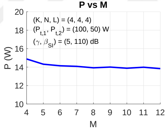
Figure 7.5: P vs M , (K, N, L) = (4, 4, 4) , (P_{t,1}, P_{t,2}) = (100, 50) W, (\gamma, \beta_{SI}) = (5, 110) dB.
