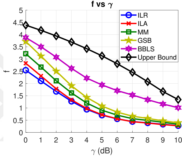
Figure 5.1: Average f vs \gamma .
