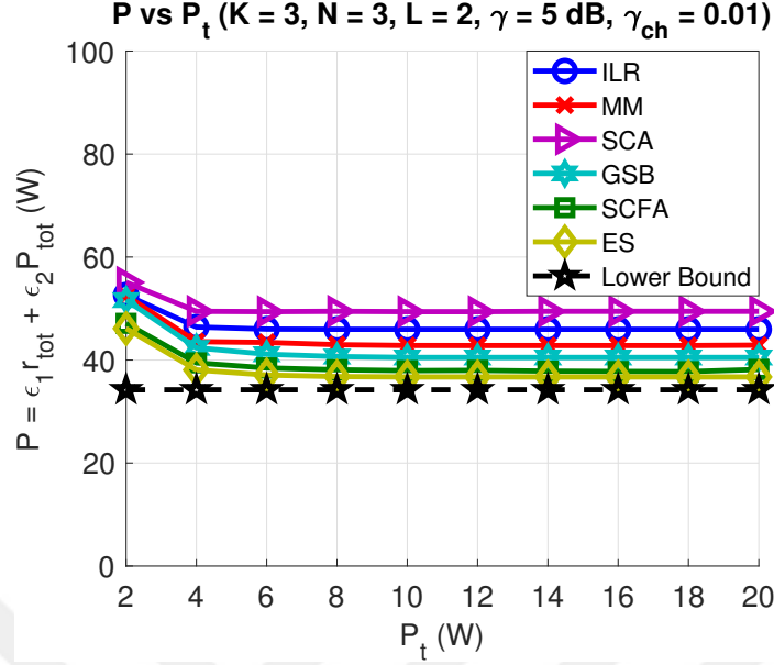
Figure 4.8: P vs P_t . K = 3, N = 3, L = 2, \gamma = 5 \text{ dB}, \gamma_{\text{ch}} = 0.01 .
