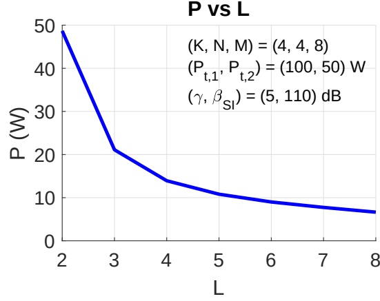
Figure 7.4: P vs L , (K, N, M) = (4, 4, 8) , (P_{t,1}, P_{t,2}) = (100, 50) W, (\gamma, \beta_{SI}) = (5, 110) dB.
