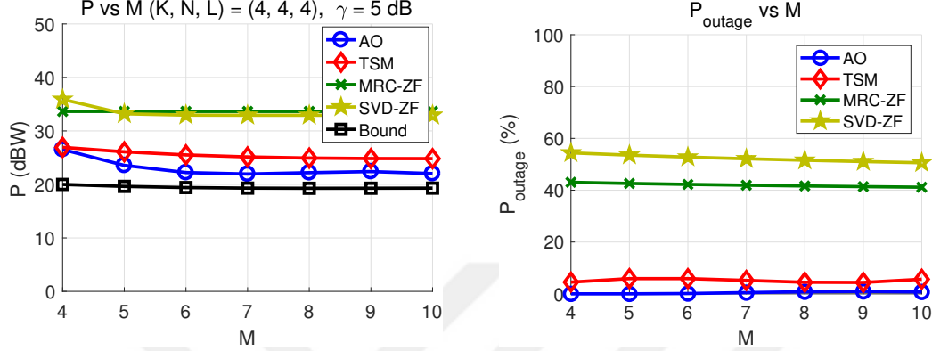
Figure 6.6: P and P_{\text{outage}} vs M . (K, N, L) = (4, 4, 4) , \gamma = 5 dB, \gamma_{\text{ch}} = 0.01 .
