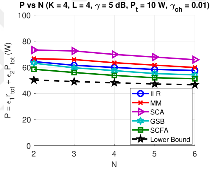
Figure 4.4: P vs N . K = 4, L = 4, \gamma = 5 dB, P_t = 10 W, \gamma_{ch} = 0.01 .
