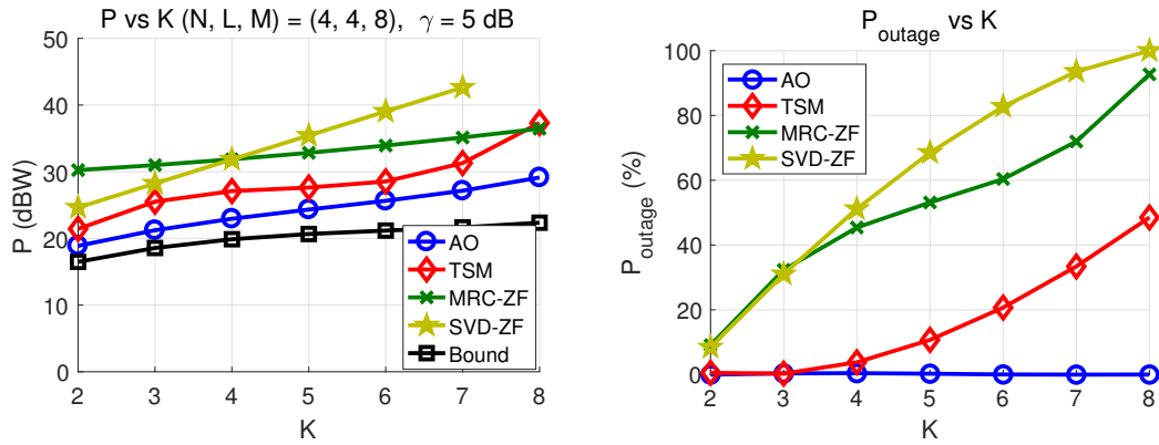
Figure 6.3: P and P_{\text{outage}} vs K . ( N, L, M ) = (4, 4, 8), \gamma = 5 dB, \gamma_{\text{ch}} = 0.01 .
