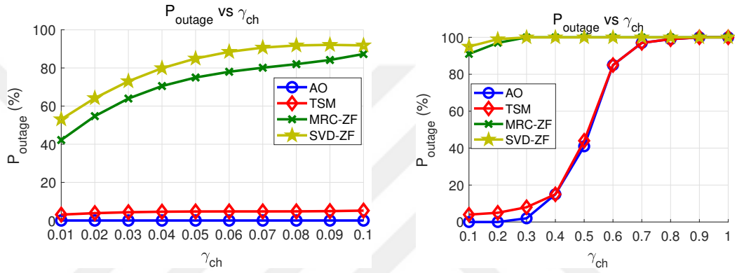
Figure 6.7: P_{\text{outage}} vs \gamma_{\text{ch}} . (K, N, L, M) = (4, 4, 4, 8) , \gamma = 5 dB.
