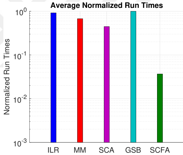
Figure 4.11: Average Complexity Comparison (K, N, L) = (8, 4, 8) .
