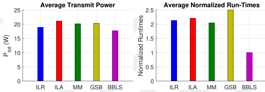
Figure 5.3: Average Transmit Power (Left) and Average Normalized Run-Times (Right).
