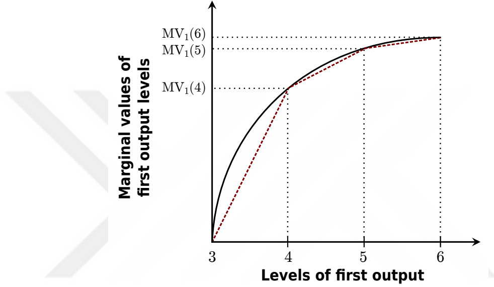
Figure 5.1: Concave marginal value function and its piecewise linear approximation
