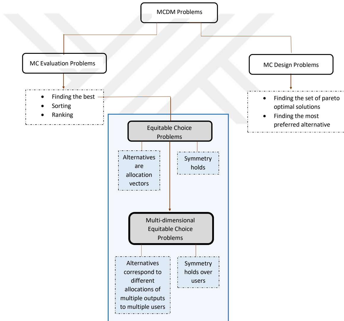
Figure 3.1: Summary of the MCDM problems
