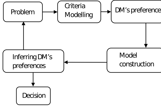
Figure 3.2: Underlying setting of the UTA and the convex cone methods [1]
