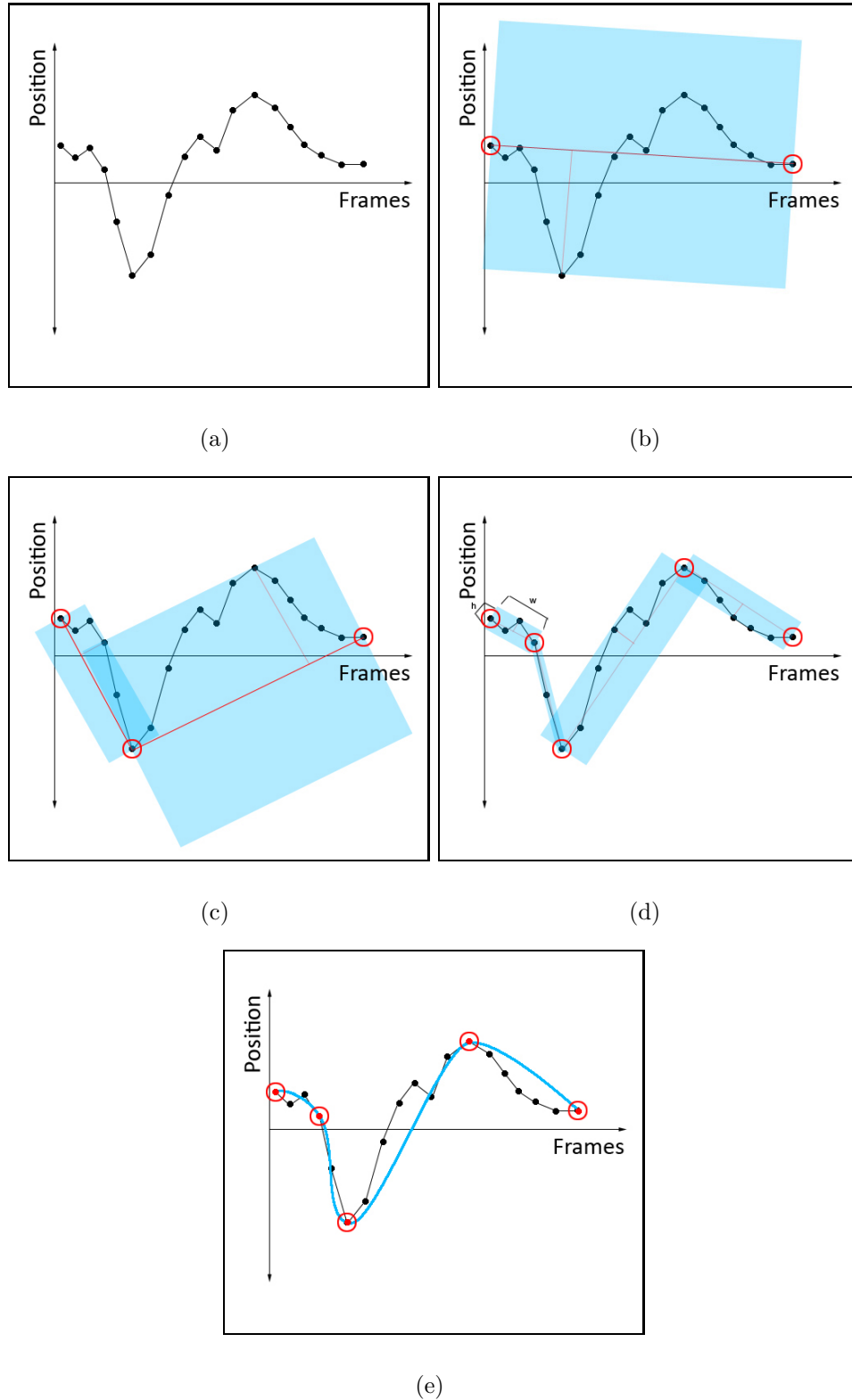
Figure 3.8: The application of the curve simplification algorithm: (a) the initial curve; (b) the first step; (c) the second step; (d) the third step; (e) the final result.
