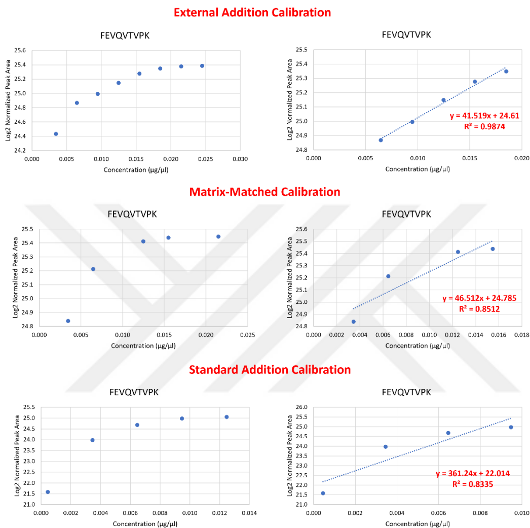
Figure 3.11. The linearity of unique peptide FEVQVTVPK in formic acid, bovine serum and human serum samples
