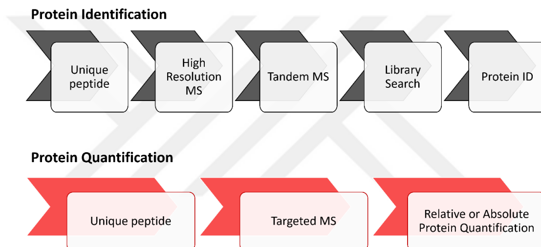
Figure 1.3. The following steps for protein identification and protein quantification in proteomics
