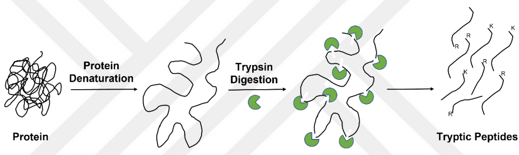
Figure 1.6. The illustration of protein digestion steps with trypsin enzyme
