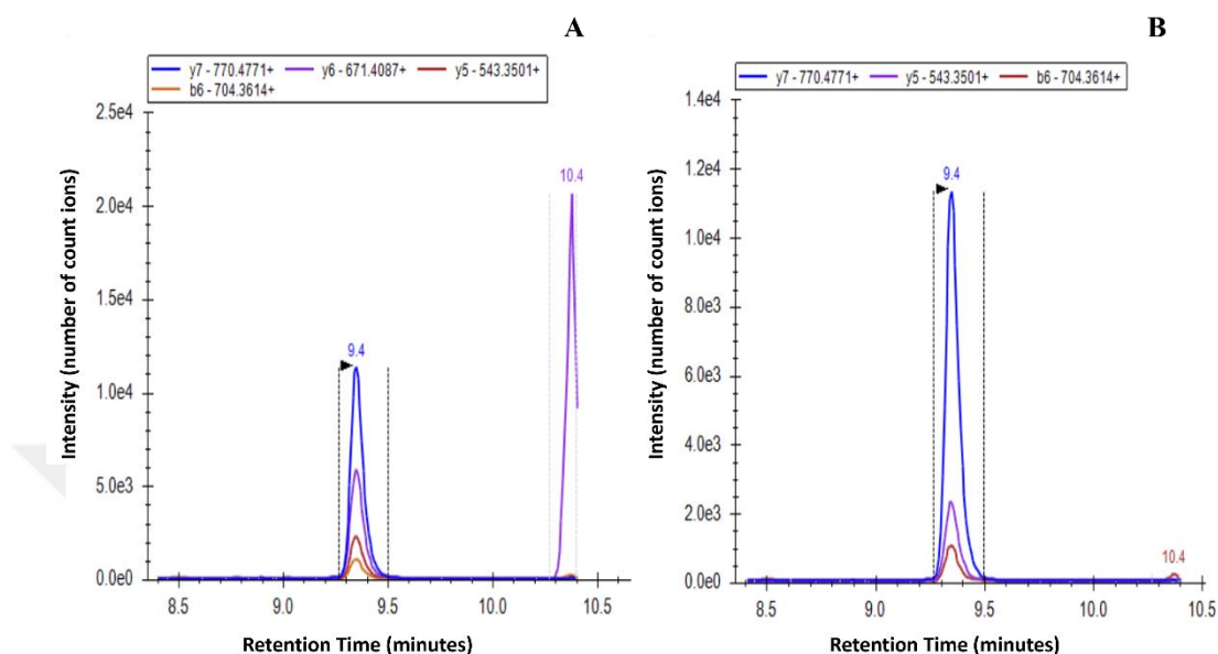
Figure 3.6. The representation of interference filtration on the unique peptide FEVQVTVPK in Skyline software A. The peak of the unique peptide is suppressed by interference. B. The interference eliminated version of the chromatogram
