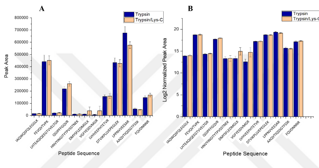
Figure 3.14. The error column plots of all unique peptides in six serum digest replicates for both enzymes. A. The plot of obtained peak areas of unique peptides for both enzymes. B. The plot of log2 normalized peak areas of unique peptides for both enzymes.
