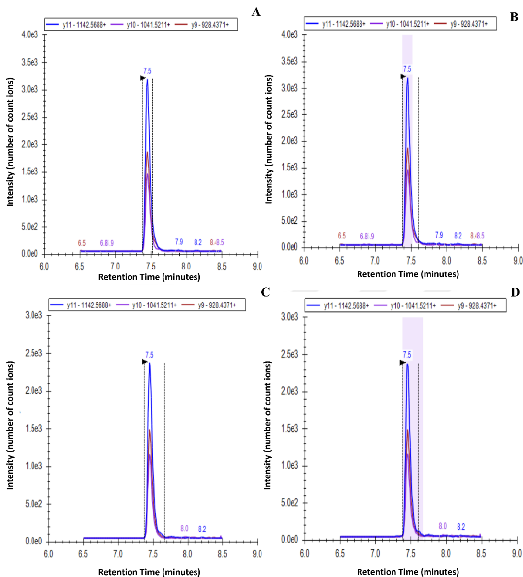
Figure 3.7. The interpretation of reintegration on one of the unique peptides AAQVTIQSSGTFSSK in Skyline software. A. The auto-integrated peak of the peptide in the serum sample. B. The reintegrated peak of the peptide in the serum sample. C. The auto-integrated peak of the peptide in the A2MG protein standard sample. D. The reintegrated peak of the peptide in the A2MG protein standard sample.
