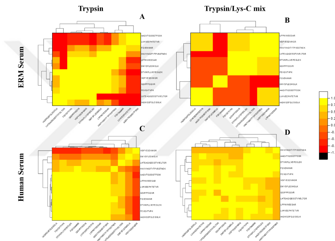
Figure 3.22. A heatmap with a dendrogram plot highlighting the association of A2MG unique peptides in standard human serum and ERM certified human serum samples with the participation of different enzymes A . The correlation of trypsin digested ERM serum. B . The correlation of trypsin/Lys-C mixture digested ERM serum samples. C . The correlation of trypsin digested standard human serum. D . The correlation of trypsin/Lys-C mixture digested human serum samples.
