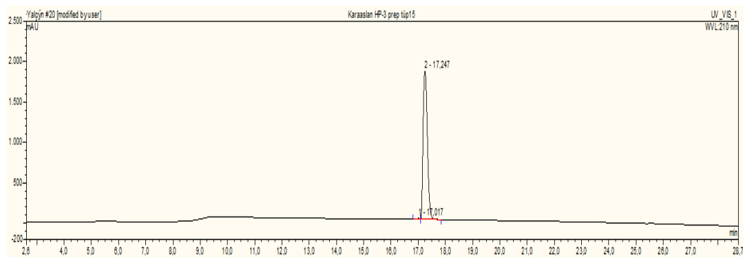
Figure 4.11. HPLC chromatogram of TFLLR (Internal Standard)
