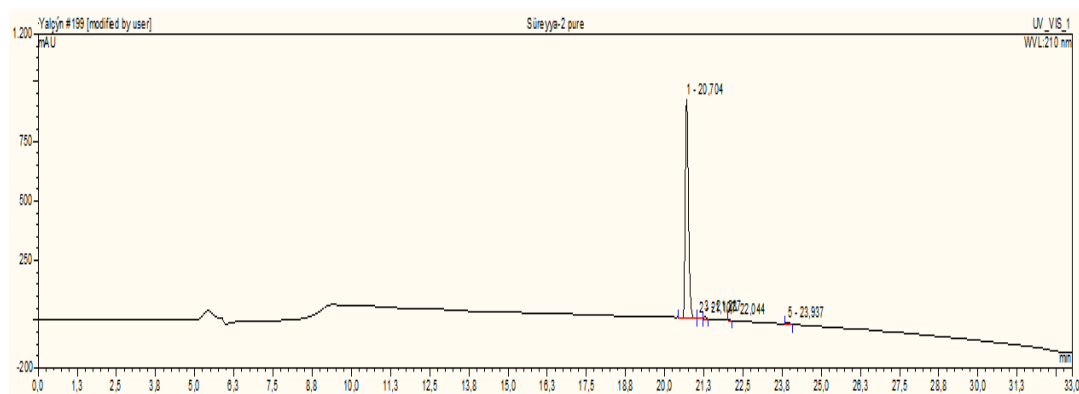
Figure 4.3. HPLC chromatogram of DMYSFLEDMLK
