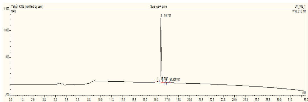
Figure 4.7. HPLC chromatogram of VGFYESDVMGR
