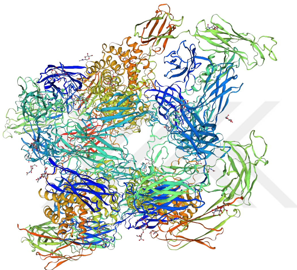
Figure 1.12. The 3D structure of A2MG from ExPasy Swiss Model Database
