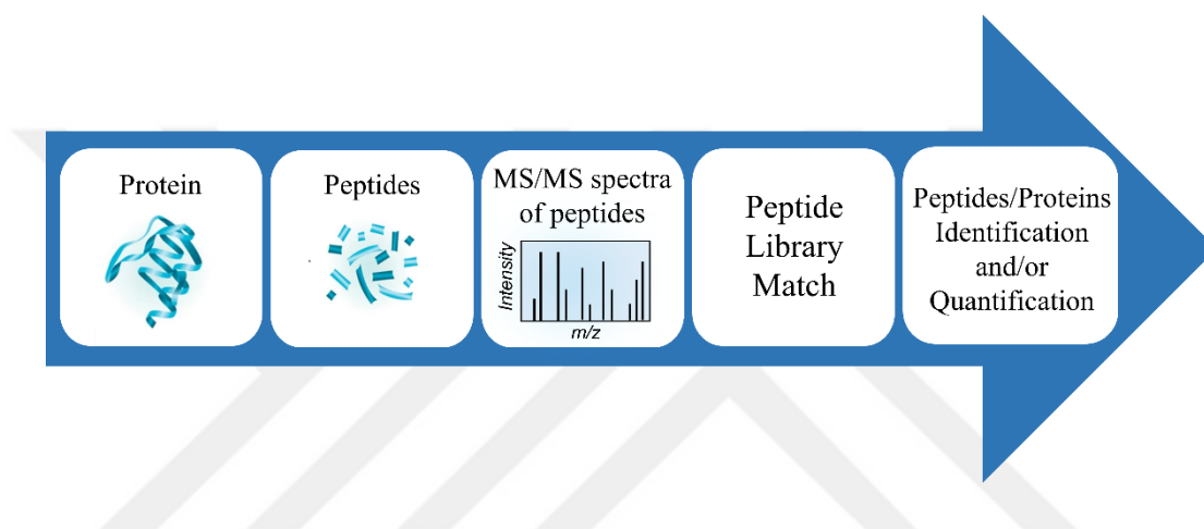
Figure 1.5. The representation of peptide-centric approach in proteomics. The figure is regenerated from "Proteomics: Technologies and Their Applications" by Aslam, B., Basit, M., Nisar, M. A., Khurshid, M., Rasool, M. H., 2017, Journal of Chromatographic Science , 55(2) 182–196.
