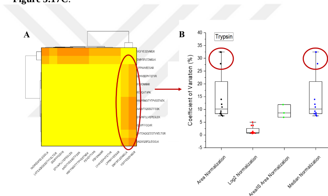
Figure 3.18. The oppositely correlated peptides in Figure 3.17C with the highlighted CV values A . The peptide correlation due to trypsin digestion in Figure 3.17C. The oppositely correlated peptides are highlighted. B . The CV values of these peptides are highlighted.
