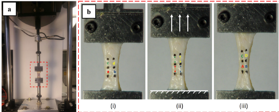
Figure 1.4: The experimental setup of the uniaxial testing machine (a) and close ups of a transverse sample under various stages of tension (b) including before loading (i), during loading (ii) and at maximum stretch of the test, modified from Cooney et al. [14].
