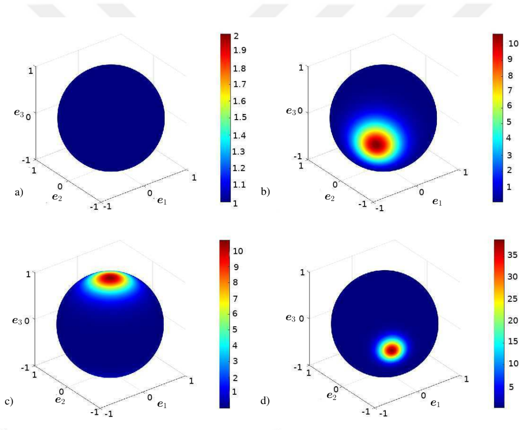
Figure 3.4: Representation of von-Mises distribution function for different parameter set; (a) b = 0, \Theta = 0^\circ, \Phi = 0^\circ (isotropic case) (b) b = 3, \Theta = 90^\circ, \Phi = 45^\circ , (c) b = 3, \Theta = 0^\circ, \Phi = 0^\circ , (d) b = 10, \Theta = 90^\circ, \Phi = 60^\circ .
