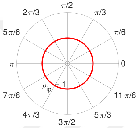
(c) One family of fibers distribution based on UT dataset for lineal alba [14].
