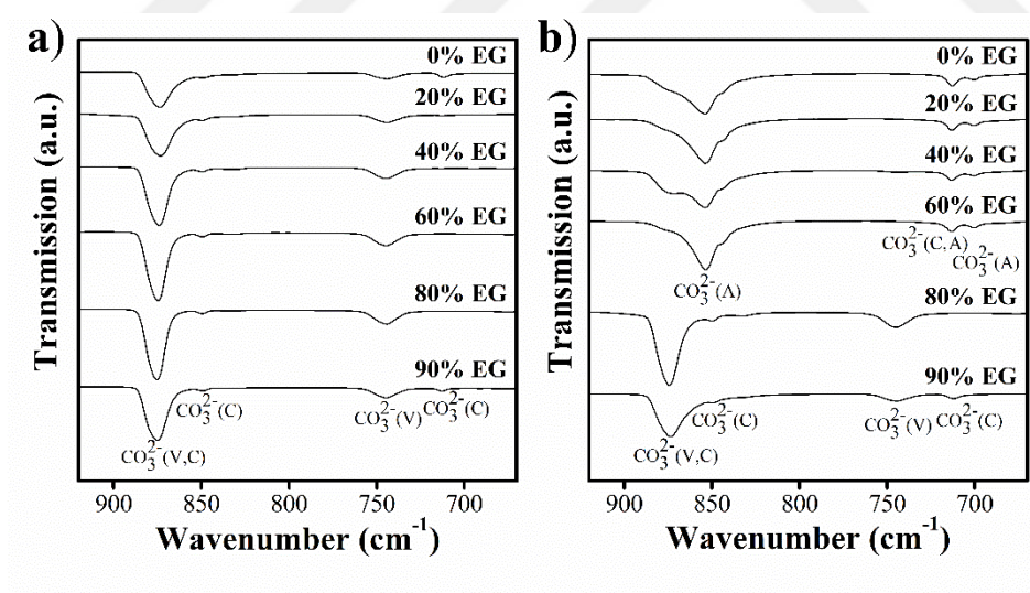
Figure 3.2. FTIR spectra of \text{CaCO}_3 particles synthesized using 0%, 20%, 40%, 60%, 80% and 90% EG at a) 25 °C and b) 70 °C. ‘V’, ‘A’ and ‘C’ denote peaks corresponding to vaterite, aragonite and calcite polymorphs, respectively.
