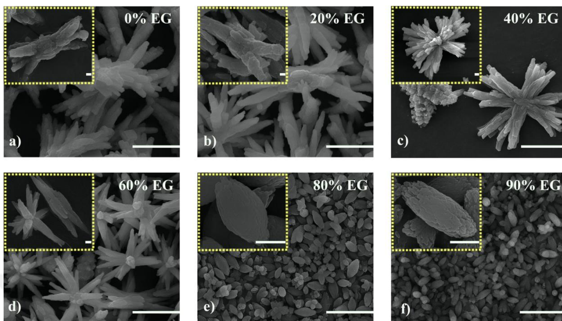
Figure 3.4. SEM micrographs of \text{CaCO}_3 particles synthesized at 70 °C using a) 0%, b) 20%, c) 40%, d) 60%, e) 80% and f) 90% EG concentrations. Scale bars are 10 \mu\text{m} . Insets show higher magnification micrographs of \text{CaCO}_3 particles and their scale bars are 1 \mu\text{m} .
