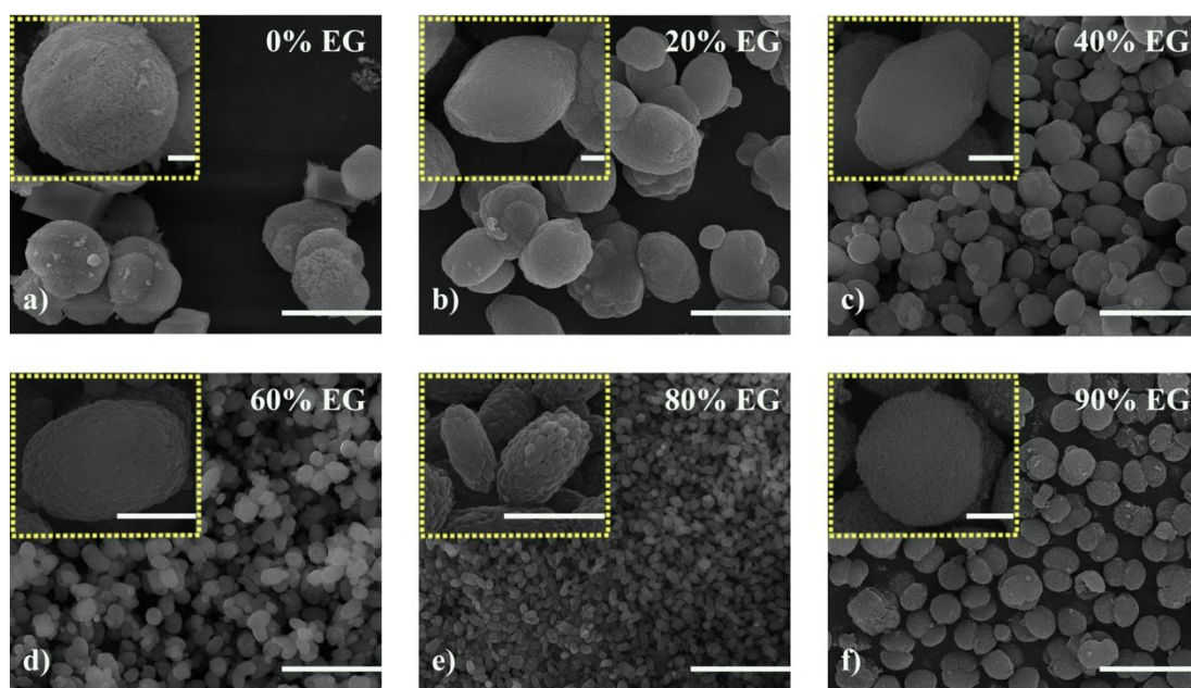
Figure 3.3. SEM micrographs of \text{CaCO}_3 particles synthesized at 25 °C using a) 0%, b) 20%, c) 40%, d) 60%, e) 80% and f) 90% EG concentrations. Scale bars are 10 \mu\text{m} . Insets show higher magnification micrographs of \text{CaCO}_3 particles and their scale bars are 1 \mu\text{m} .
