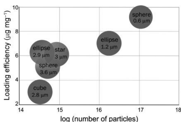
Figure 1.5. Loading capacity of \text{CaCO}_3 particles having different morphologies and sizes. The capacity values were represented in \mu\text{g} of dye per \text{mg} of the particles for the same total particle weight [45].
