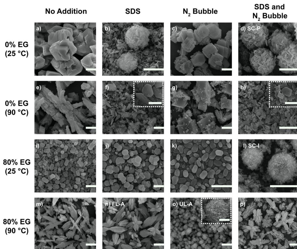
Figure 6.1. SEM micrographs of \text{CaCO}_3 particles prepared using a-d) 0% EG (25 °C), e-h) 0% EG (90 °C), i-l) 80% EG (25 °C) and m-p) 80% EG (90 °C) precursor solutions. a, e, i and m) have neither SDS nor \text{N}_2 bubbling, b, f, j and n) have SDS addition only, c, g, k and o) have \text{N}_2 bubbling only and d, h, l and p) have both SDS and \text{N}_2 bubbling. Platelet shaped spherical calcite (SC-P), irregular shaped spherical calcite (SC-I), flower-like aragonite (FL-A) and urchin-like aragonite (UL-A) particles are highlighted in the figure. Insets show higher magnification micrographs of the particles. Scale bars are 5 \mu\text{m} and 1 \mu\text{m} for lower and higher magnification micrographs, respectively.
