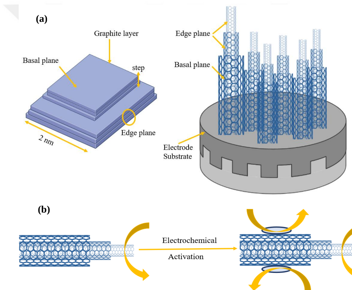
Figure 3.8 Electrochemistry of carbon nanotubes is similar to that of graphite, Redesigned based on (Pumera 2009)
