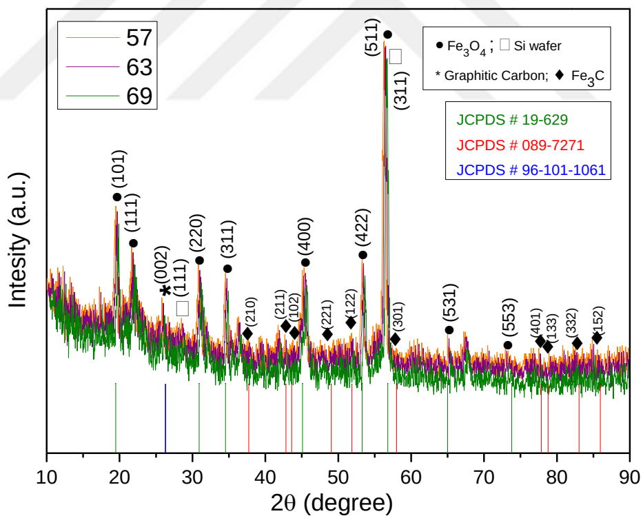
Figure 5.29 X-ray diffraction (XRD) graph of the 7-minute samples
