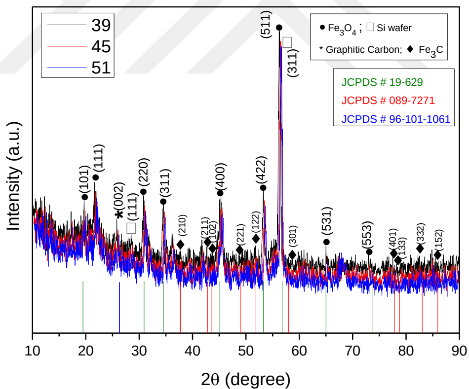
Figure 5.28 X-ray diffraction (XRD) graph of the 5-minute samples
