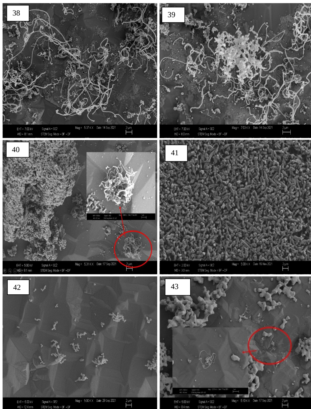
Figure 5.12 SEM images at x5K magnification of samples applied 6 wt.% catalysts and 5 min growth time.
