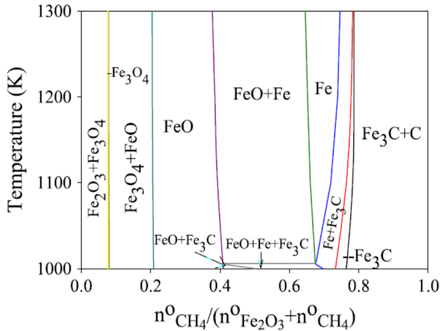
Figure 5.8 Diagram illustrating \text{Fe}_2\text{O}_3 – \text{CH}_4 solid stability in equilibrium with the gas phase as a function of temperature and mole fraction of \text{CH}_4 (Altay and Eroglu 2013).
