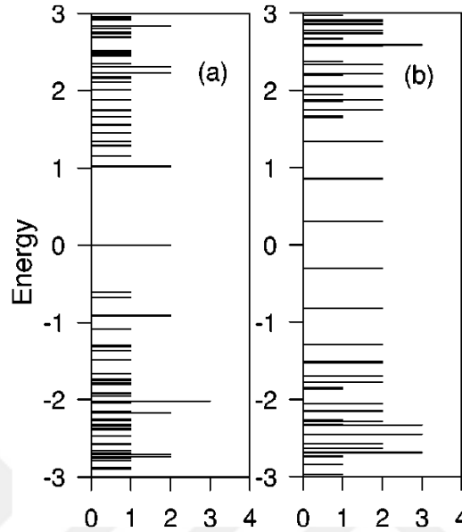
Figure 2.16 Energy-level structure based on nanotube HOMO and LUMO. The length of the line is related to the energy level's degeneracy. The undegenerated levels have the shortest line. (a) (6,4); (b) (6,3) (Wan, Dong, and Xing 1998)
