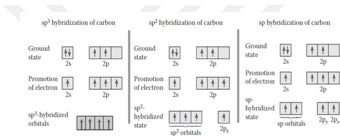
Figure 2.19 A carbon atom's hybridization types (Mathur, Singh, and Pande 2016)
