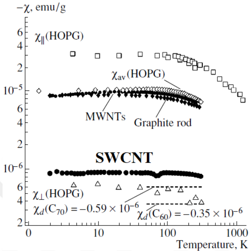
Figure 2.17 Magnetic susceptibility of different carbons measured experimentally. highly oriented pyrolytic graphite (HOPG) in the longitudinal ( c_{||} ) and transverse ( c_{\perp} ) directions, powdered HOPG (cav), a graphite rod, MWNTs, SWCNTs, and fullerenes (Makarova 2004)
