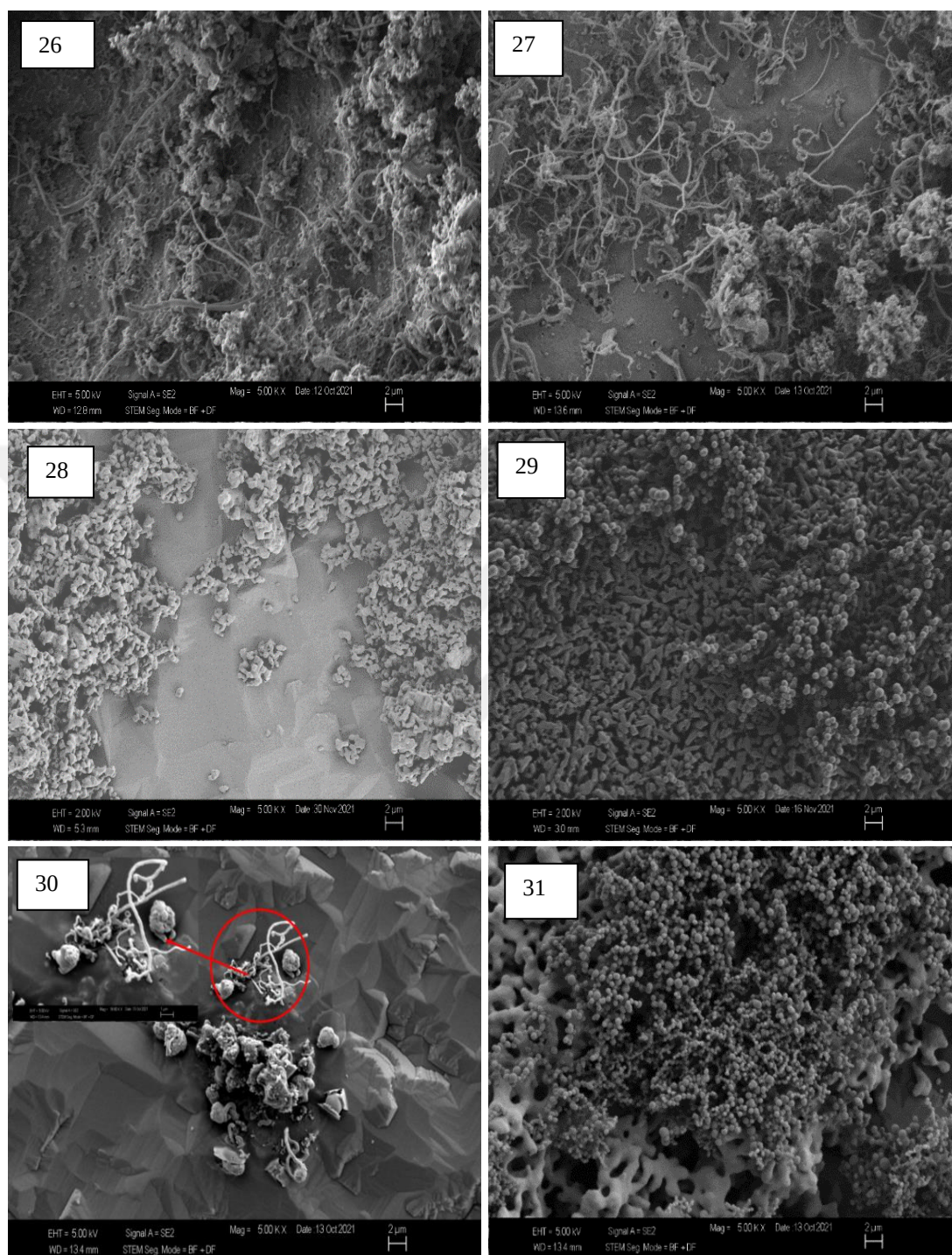
Figure 5.10 SEM images at x5K magnification of samples applied 4 wt.% catalysts and 3 min growth time.
