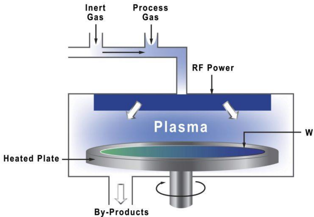
Figure 2.12 Schematic representation of Plasma Enhanced CVD process
