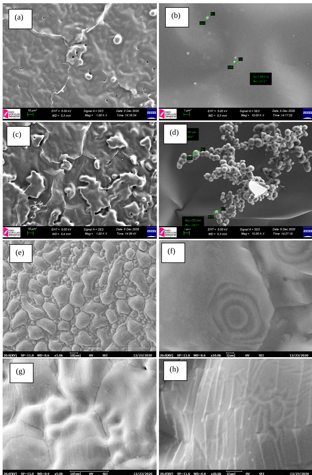
Figure 5.1 SEM Images of samples 1 and 2; Sample 1 (a) at \times 1K , (b) at \times 10K ; Sample 2 (c) at \times 1K , (d) at \times 10K magnification; Sample 3 (e) at \times 1K , (f) at \times 10K ; Sample 4 (g) at \times 5K , (h) at \times 20K magnification.
