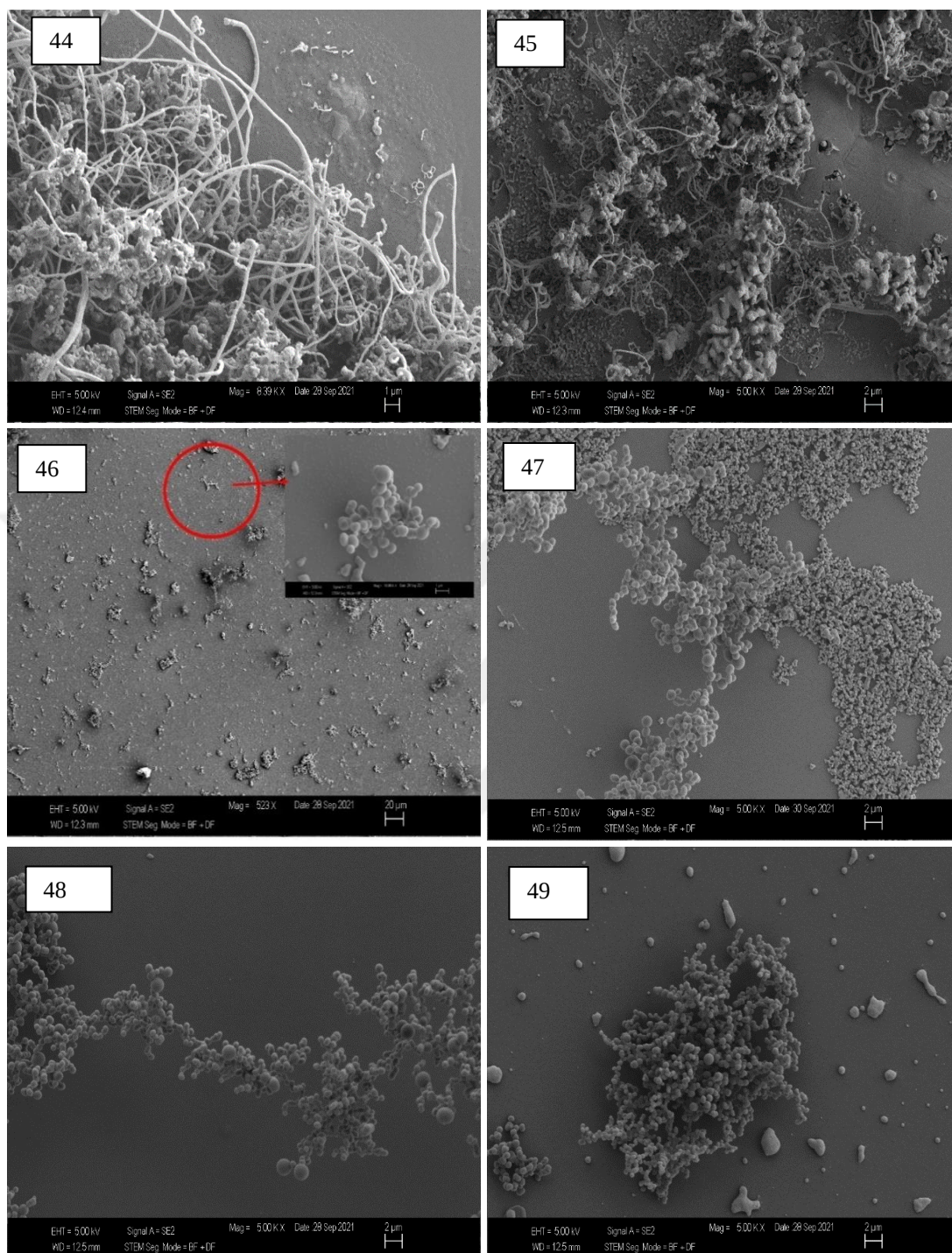
Figure 5.13 SEM images at x5K magnification of samples applied 4 wt.% catalysts and 5 min growth time.
