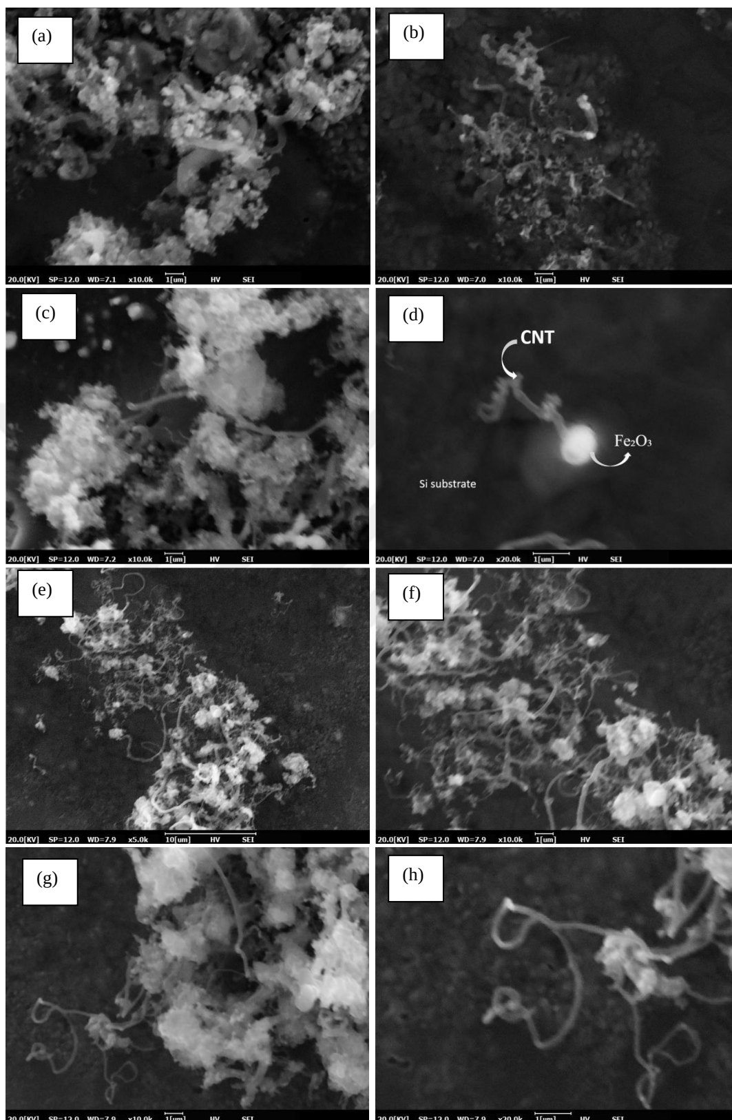
Figure 5.2 SEM Images of samples 5 and 6; Sample 5 (a,b and c) at \times 10K , (d) at \times 20K magnification; Sample 6; (e) at \times 5K , (f, and g) at \times 10K , (h) at \times 20K magnification
