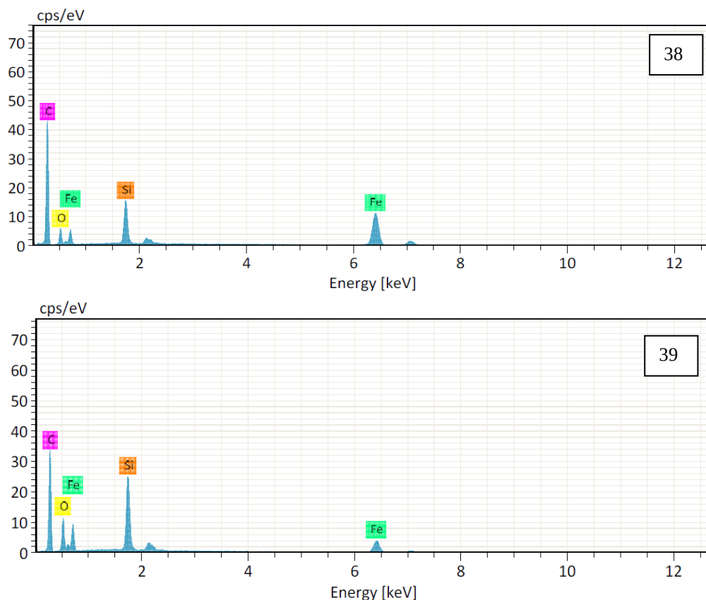
Figure 5.18 EDX spectrum of Samples 38 and 39
