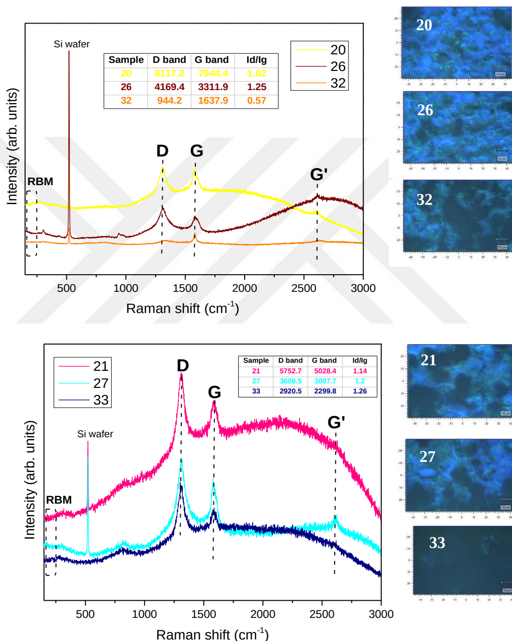
Figure 5.24 Raman spectrum of the 3-minute samples.
