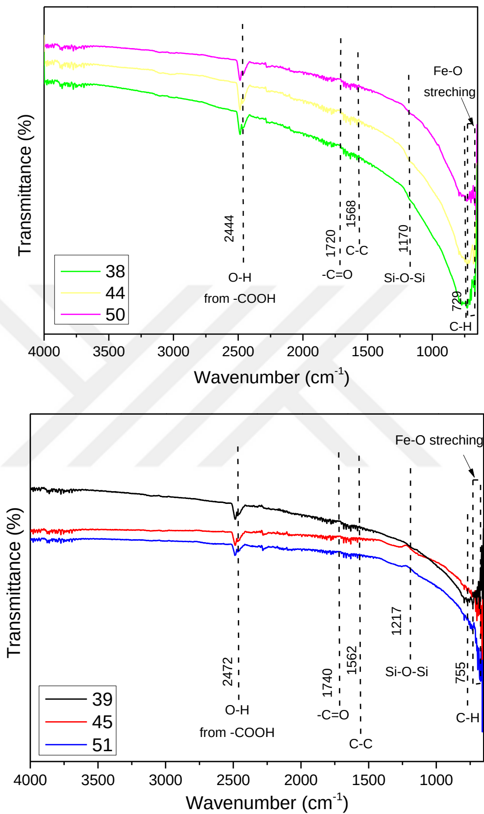
Figure 5.22 FT-IR spectra of the 5-minute samples
