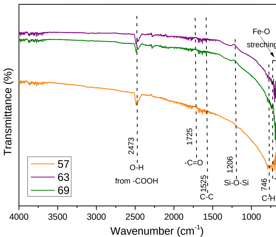
Figure 5.23 FT-IR spectra of the 7-minute samples
