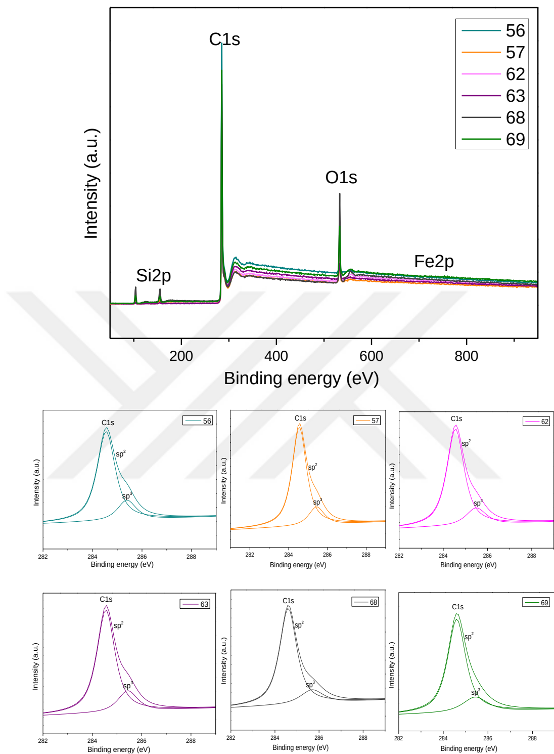
Figure 5.32 XPS Survey spectra and the deconvoluted C 1s spectra of the 7-minute samples.
