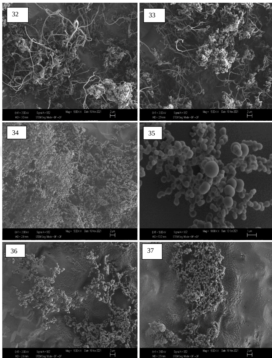
Figure 5.11 SEM images at x5K magnification of samples applied 2 wt.% catalysts and 3 min growth time.
