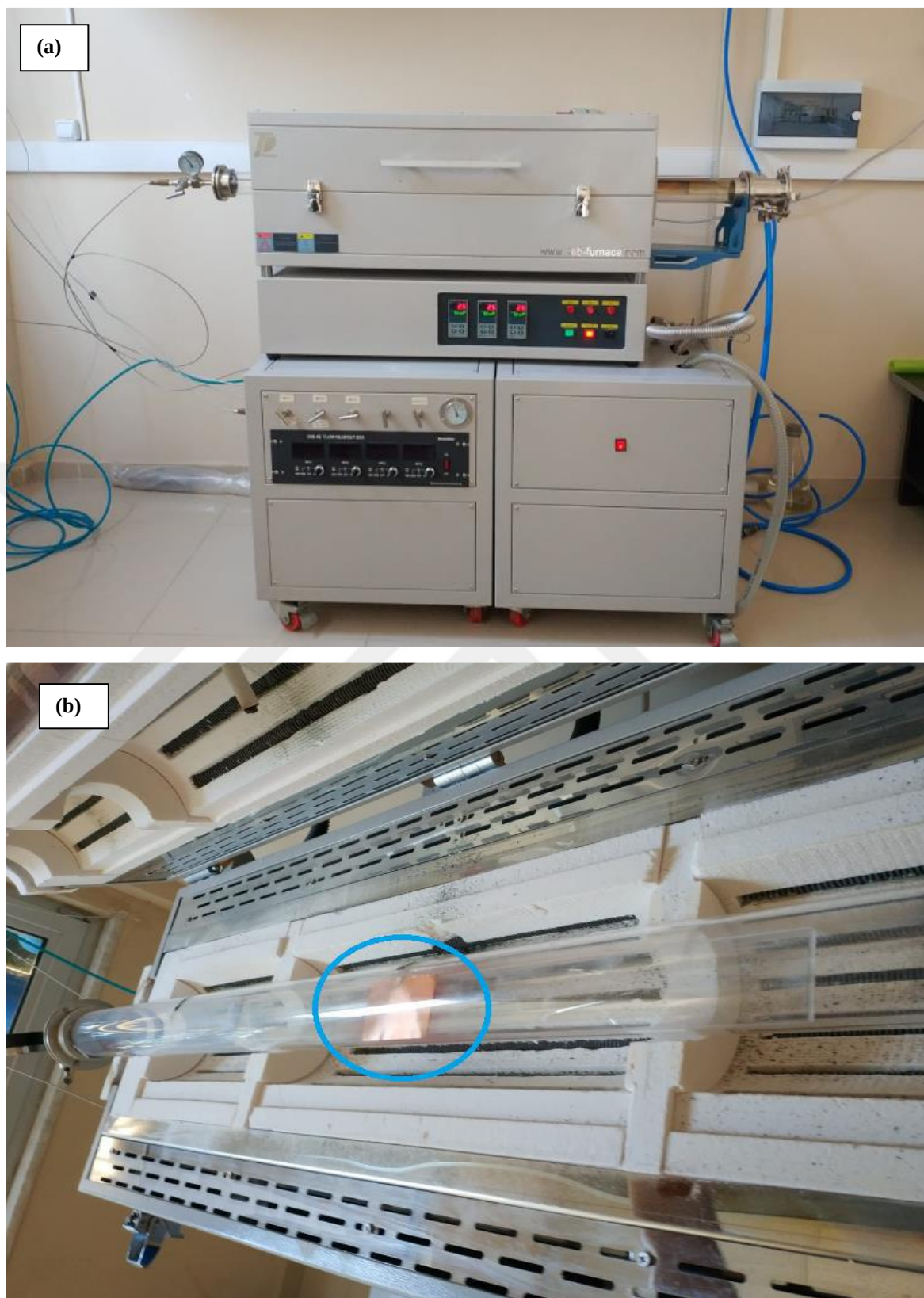
Figure 4.4 The CVD System, Zhengzhou Protech technology Co. Ltd-PT 1200-CVD, (Smart Materials's Lab., IKCU); (a) External view of the system, (b) Active reaction zone.
