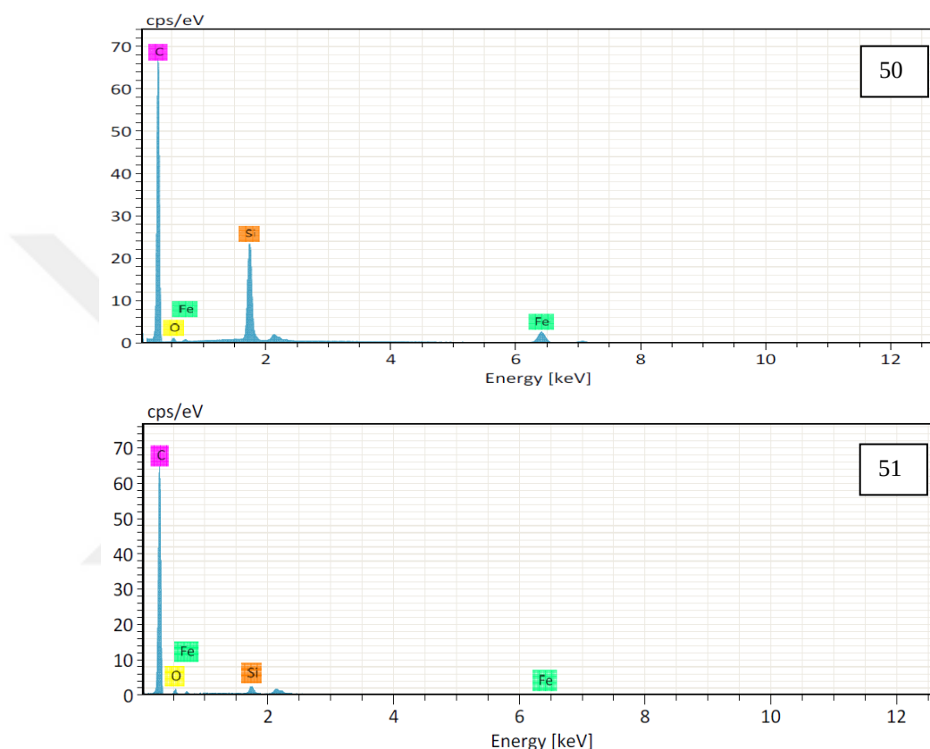
Figure 5.20 EDX spectrum of Samples 50 and 51
