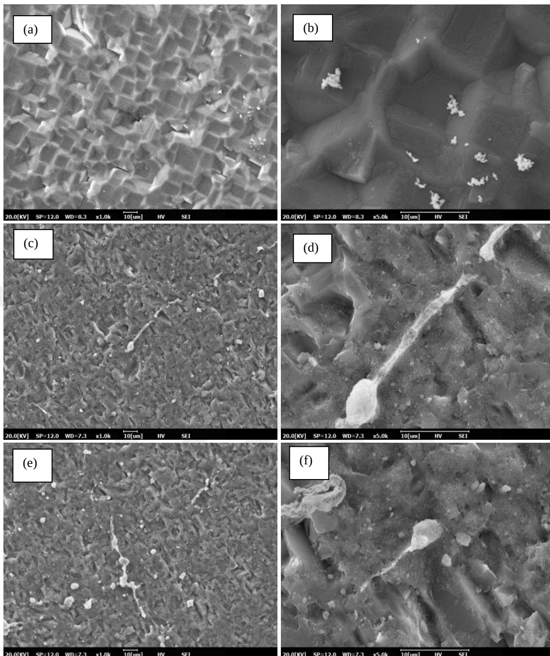
Figure 5.5 SEM Images of samples 11, and 12 at different magnifications and locations; Sample 11 (a) x1K, (b) x5K; Sample 12 (c) x1K, (d) x5K, (e) x1K, (f) x5K
