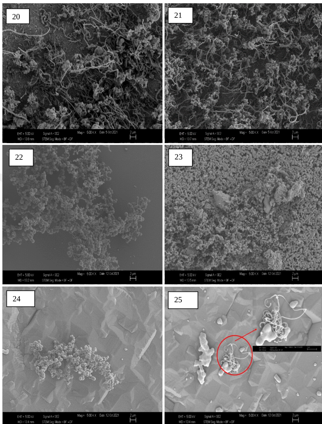
Figure 5.9 SEM images at x5K magnification of samples applied 6 wt.% catalysts and 3 min growth time.
