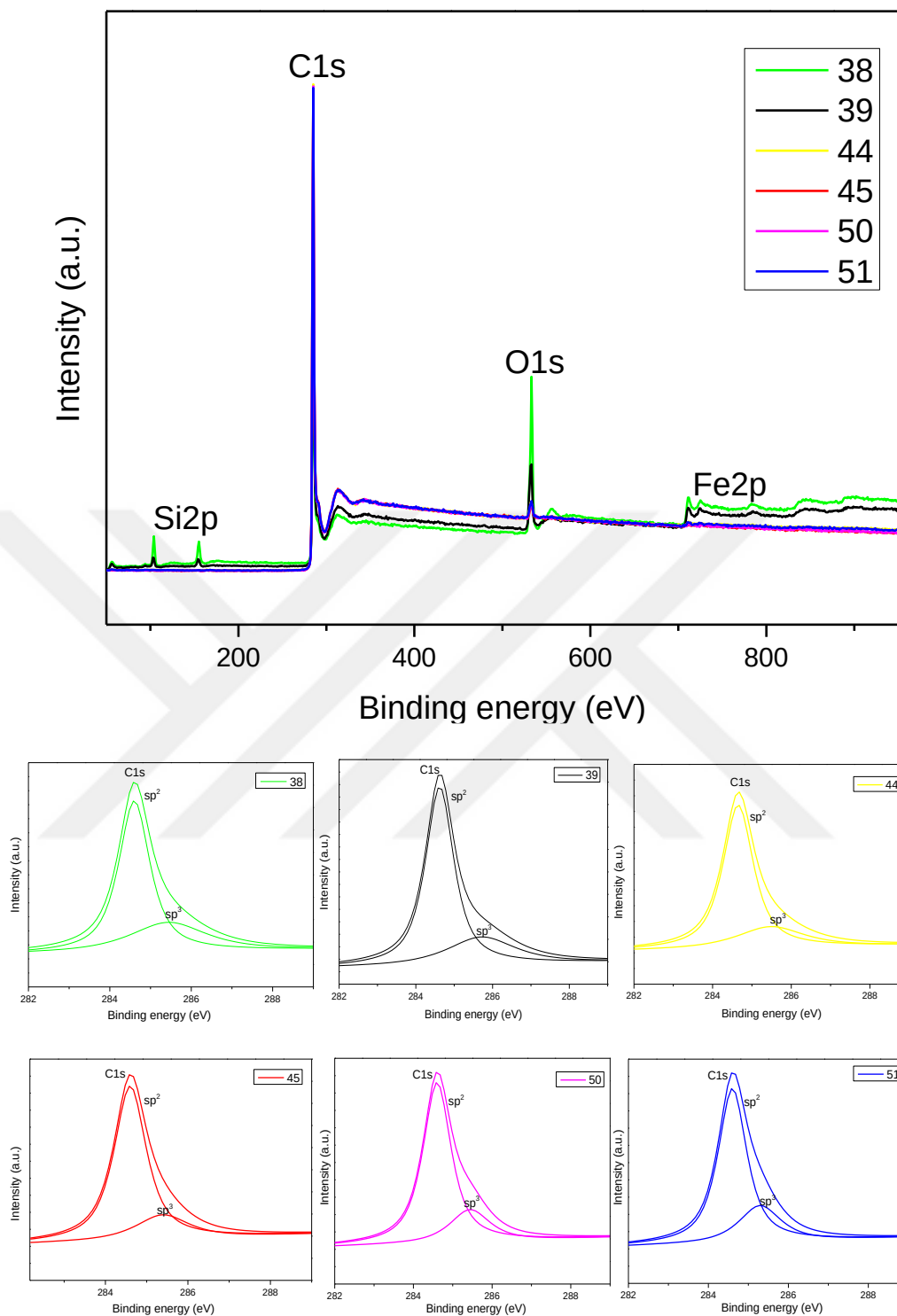
Figure 5.31 XPS Survey spectra and the deconvoluted C 1s spectra of the 5-minute samples.
