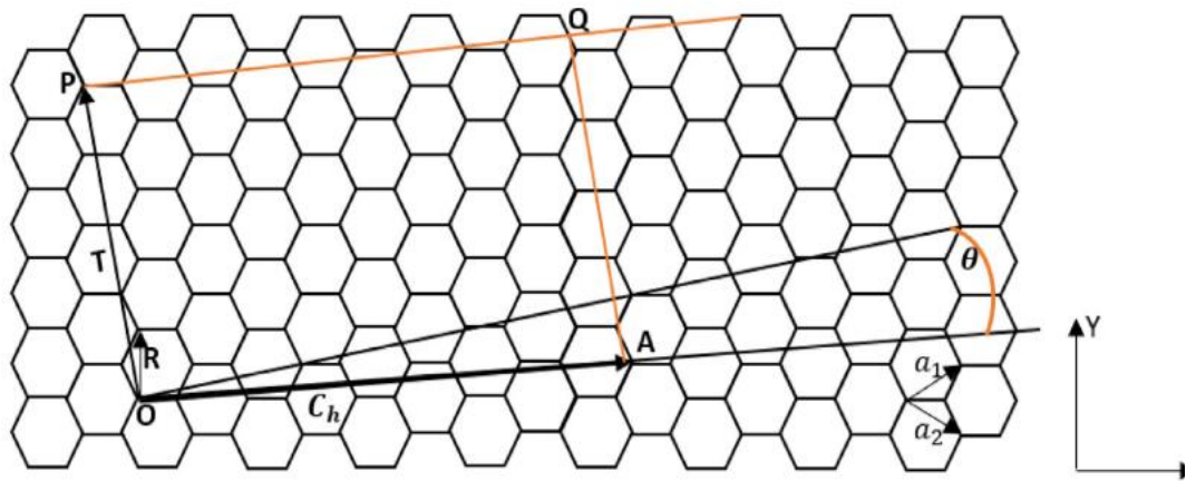
Figure 2.3 An unrolled graphene sheet from which SWCNT is formed by joining the PQ and OA sides of the OAQP rectangle (Garg et al., 2021)
