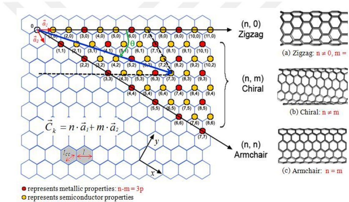
Figure 2.4 Different types of SWCNTs (Attaf 2015)
