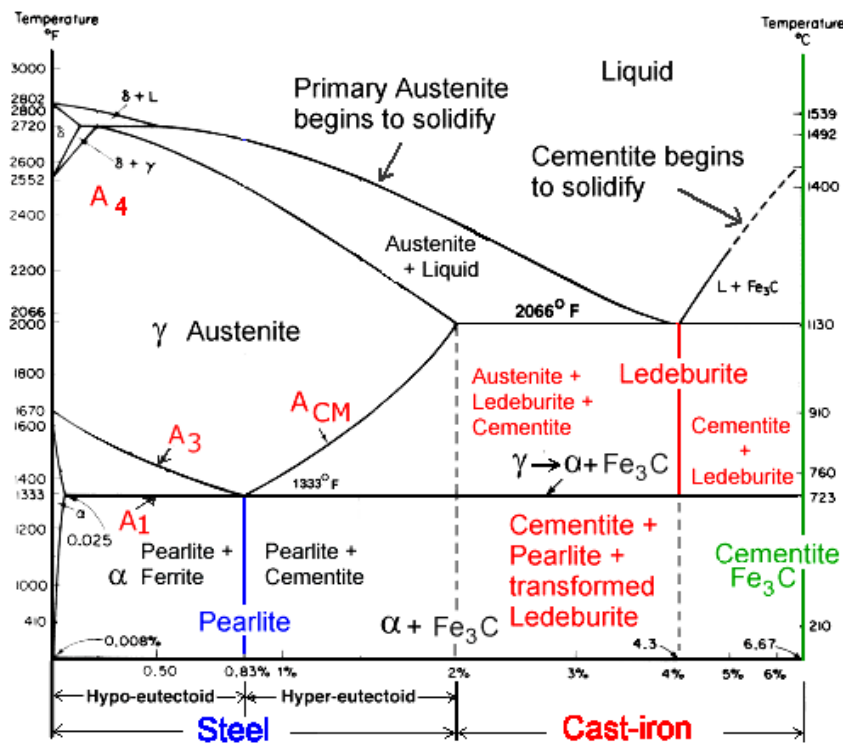
Figure 5.7 Iron-carbon equilibrium diagram(Ho Okamoto 1992)
