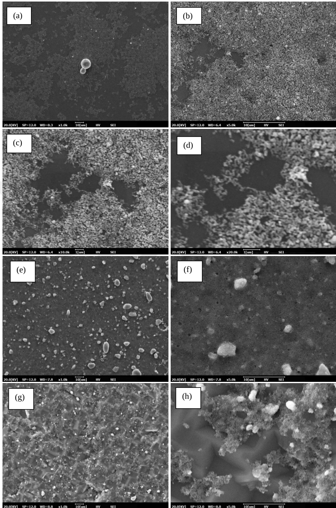
Figure 5.4 SEM Images of samples 9 and 10 at different magnifications and locations; Sample 9 (a) x1K, (b) x5K, (c) x10K, (d) x20K; Sample 10; (e) x1K, (f) x5K, (g) x1K, (h) x5K.
