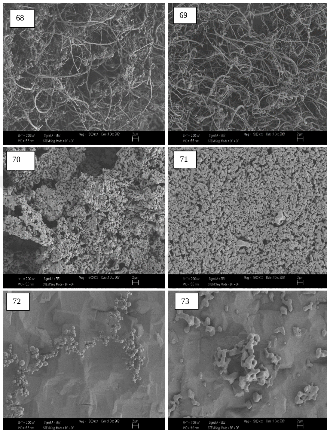
Figure 5.17 SEM images at x5K magnification of samples applied 2 wt.% catalysts and 7 min growth time.
