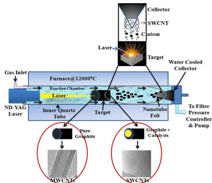
Figure 2.8 Schematic representation of the CNTs synthesis via laser ablation method (R. Das et al., 2016)
