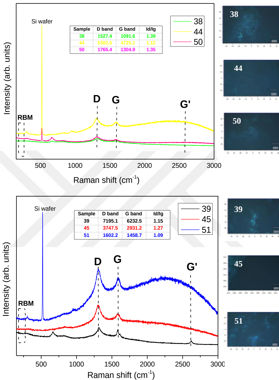
Figure 5.25 Raman spectrum of the 5-minute samples.
