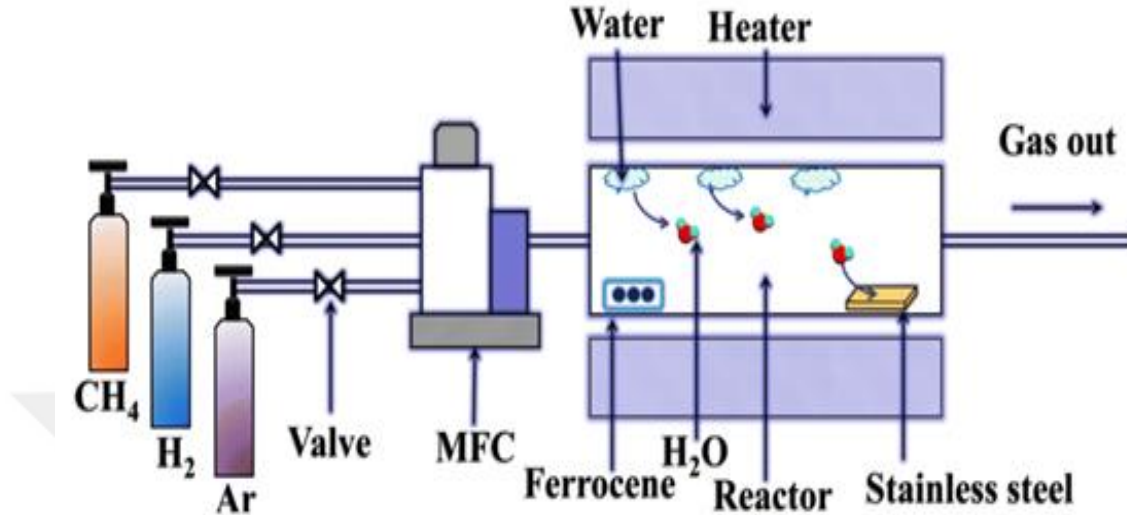
Figure 2.13 Schematic representation of WACVD process (F. Wu et al., 2019)
