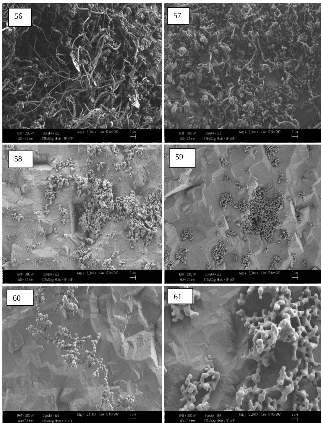
Figure 5.15 SEM images at x5K magnification of samples applied 6 wt.% catalysts and 7 min growth time.
