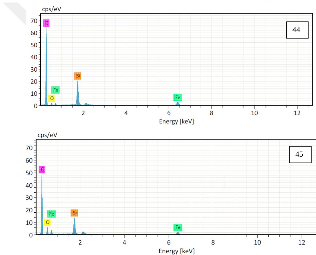
Figure 5.19 EDX spectrum of Samples 44 and 45
