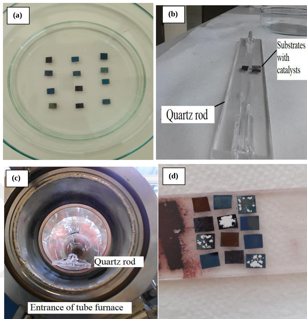
Figure 4.6 (a) Catalyst supported substrates, (b) Placing catalyst supported substrates on quartz rod, (c) insertion of the quartz rod into the CVD system, (d) appearance of substrates after CVD treatment
