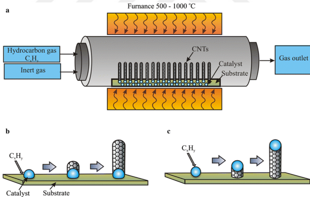
Figure 2.11 Schematic representation of Catalytic CVD process (Zaytseva and Neumann 2016)
