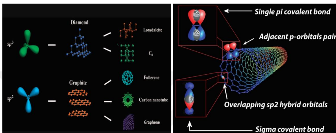
Figure 2.20 Hybridization of carbon structures and schematic representation of bond structure of CNT (Batmunkh, Biggs, and Shapter 2015; Radauscher 2016)
