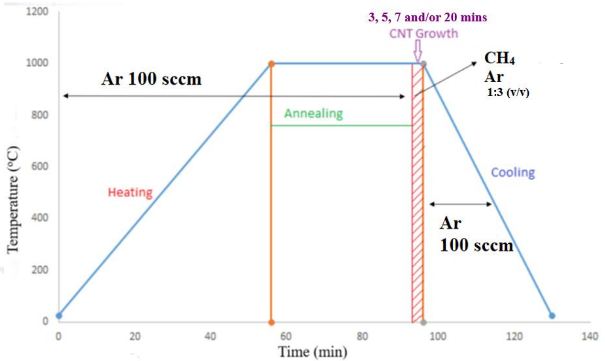
Figure 4.7 CVD process for CNT growth
