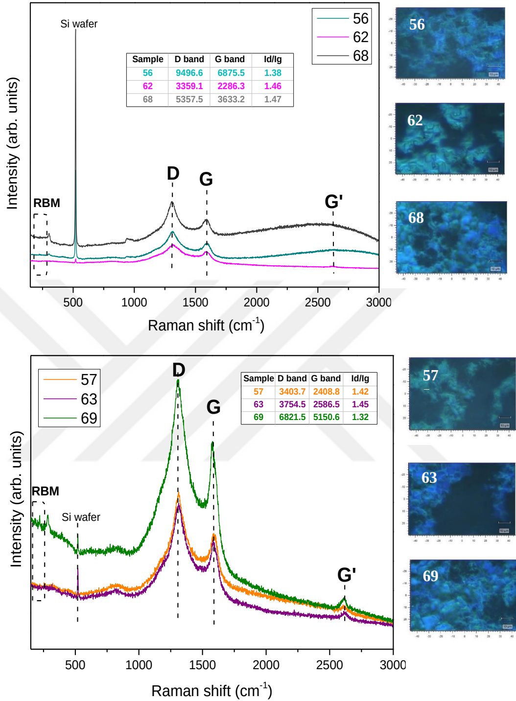
Figure 5. 26 Raman spectrum of the 7-minute samples.
