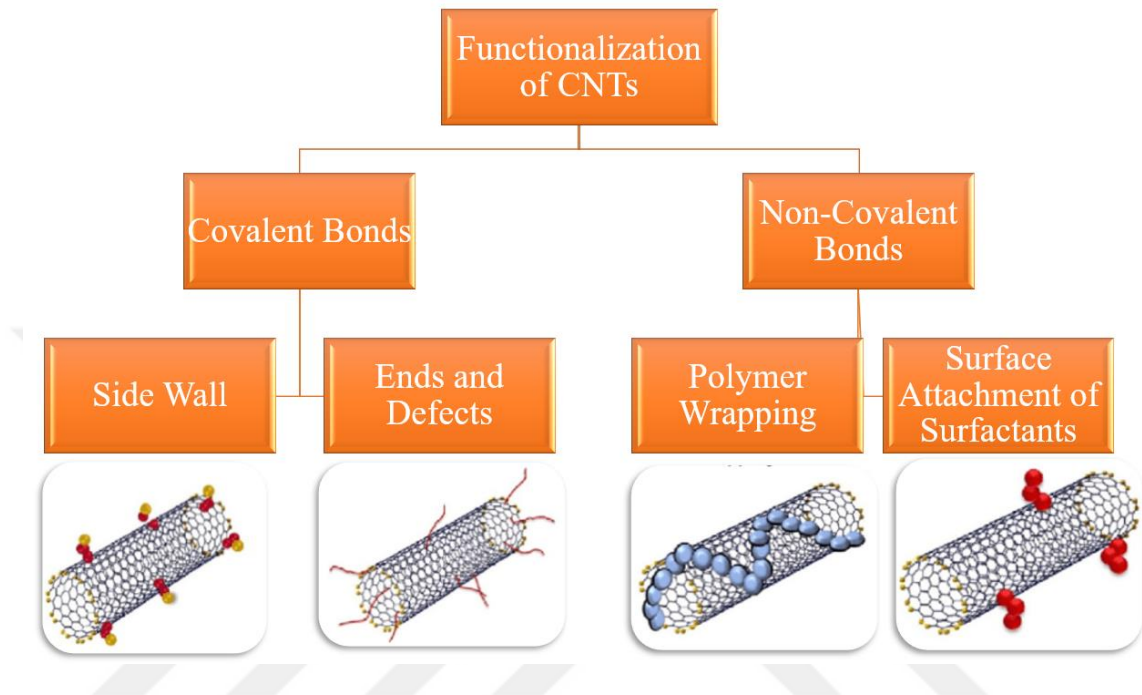
Figure 3.7 Chemical functionalization techniques for CNTs (Jun et al., 2018)
