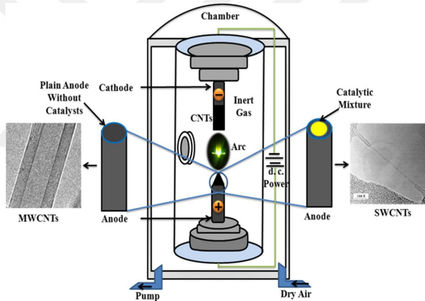
Figure 2.7 Schematic representation of the CNTs synthesis using arc discharge technology (R. Das et al., 2016)
