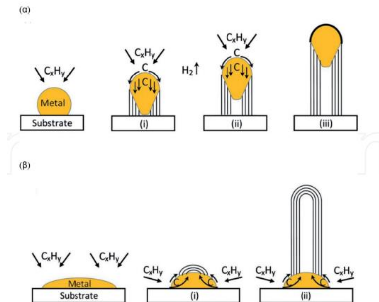
Figure 2.14 Growth Mechanisms of CNTs via CVD
