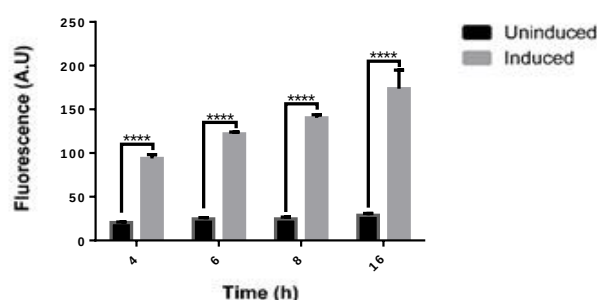
Figure 123. Time-dependent characterization of the pET22b-ABS-ParsR-ArsR-sfGFP-ProD-HucR sensor with 10 \mu M Sodium Arsenate ( \text{Na}_3\text{AsO}_4 ). E. coli PRO cells were grown in LB growth media at 42°C. Experiments were repeated in triplicates, and measurements were taken at 4 th , 6 th , 8 th and 16 th hours after induction. The results were analyzed with two-way analysis of variance (ANOVA) (GraphPad Prism version 9.0.0), the differences between the groups were marked with “*” ( p \leq 0.05 , p \leq 0.01 , p \leq 0.001 and p \leq 0.0001 is represented by “*”, “**”, “***” and “****” respectively). “ns” was used in the groups that did not show significant differences.
