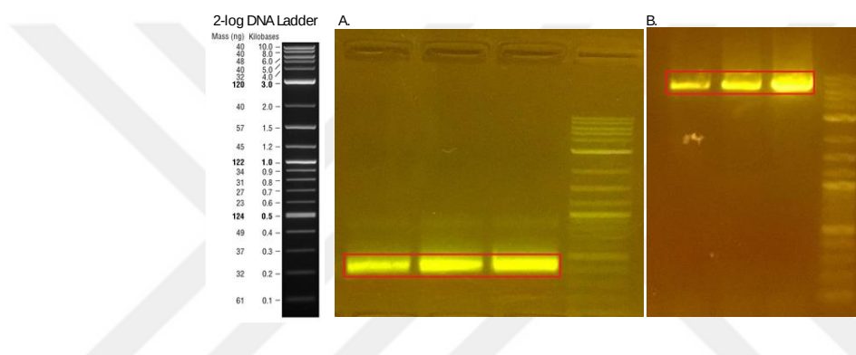
Figure 112. Agarose gel image of the biological parts required for the cloning of the pET22b-ABS-ParsR-ArsR-sfGFP-ProD-HucR vector. A. PCR product of ArsR transcription factor gene region, 434 bp. B. PCR product of the linear pET22b-ABS-ParsR-sfGFP-ProD backbone, 6810 bp
