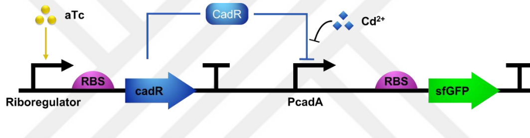
Figure 81. Figure of cadmium biosensor working mechanism. Cadmium biosensor biological parts and working mechanism. CadR transcription factor binds to PcadA promoter in the absence of cadmium ions within the cell. When cadmium ions present, upon release of CadR from PcadA promoter, downstream expression of sfGFP is activated.
