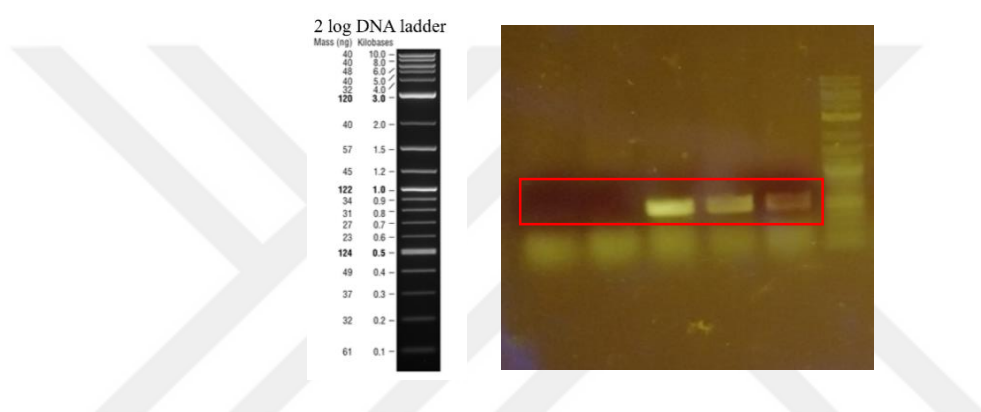
Figure 86. Confirmation of the pZs-PITetO-rioregulator-CadR-KanR vector with colony PCR. A. The bands expected for the PCR amplified PITetO-rioregulator-CadR biological parts were observed at 878 bp.
