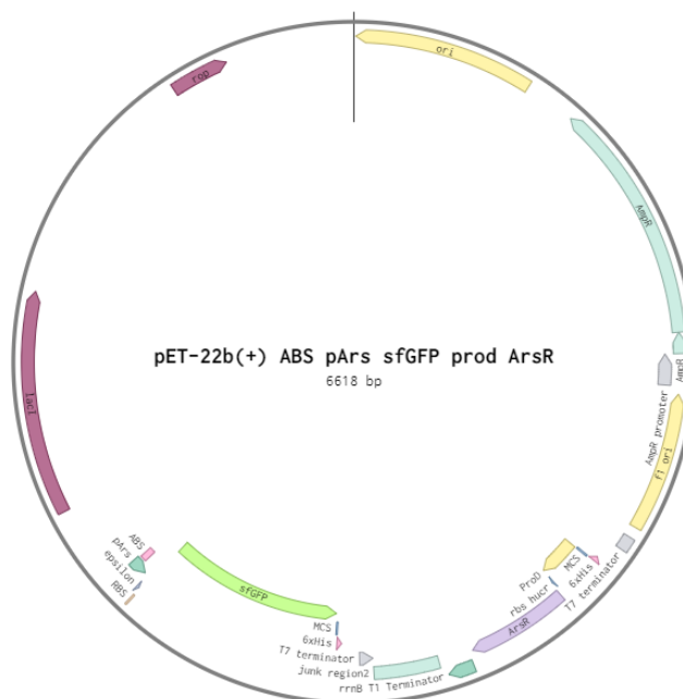
Figure 184. Schematic representation of pET22b -ParsR-sfGFP-ProD-HucR vector.
