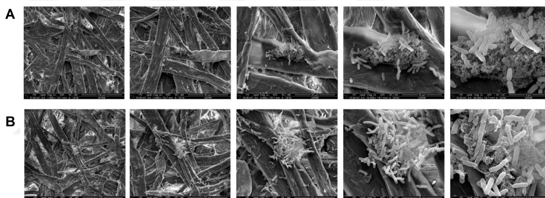
Figure 136. Biofilm mediated immobilization of cells on filter paper assay with Environmental scanning electron microscopy (ESEM). A. Uninduced E.coli PRO cells containing pZa pBAD csgA vector grown in LB overnight with OD 600 0.01. A. 0.2% arabinose and 1mM IPTG induced E.coli PRO cells containing pZa pBAD csgA vector grown in LB overnight with OD 600 0.01 Images are taken with x1000, x2000, x5000, x10000, x20000 magnification from left to right in order.
