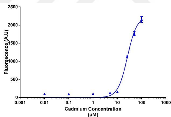
Figure 91. Concentration-dependent characterization of the pET22b-PcadA-RBS30-sfGFP cotransformed with pZs-PITetO-riboregulator-CadR-KanR sensor with \text{Cd}(\text{CH}_3\text{COO})_2 . Experiments were repeated in triplicates, and measurements were taken at the 8 th hour of induction. E. coli cells were grown in chemically defined MOPS buffered minimal growth media.
