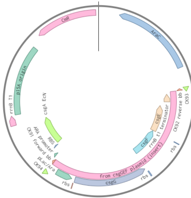
Figure 190. Schematic representation of pZa PBAD csgA pLac/Ara csgGEF vector.
