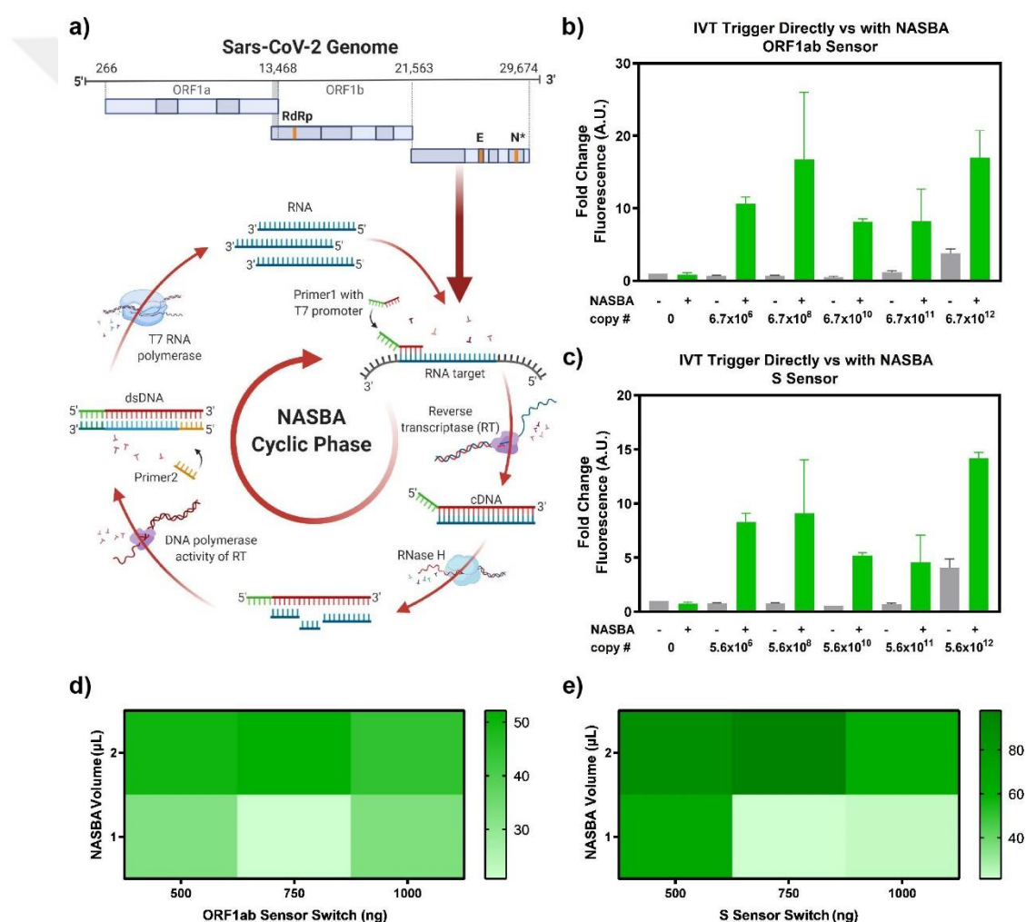
Figure 163. Characterization and optimization of ORF1ab trigger/switch and S trigger/switch couples in TXTL reactions. a) Representation of working principle of NASBA reaction. In vitro transcribed triggers are either added to TXTL reactions directly or after NASBA reactions, measurements at 60th minute are given for b) ORF1ab and c) S trigger/switch couple. The average and SE of duplicate experiments are shown. NASBA volume and switch vector amounts are optimized in TXTL reactions. Reactions were monitored for 120 minutes with 10 minute intervals and endpoint fluorescence measurements of d) ORF1ab and e) S trigger/switch couple are given. Representative average and SE of triplicate experiments are shown.
