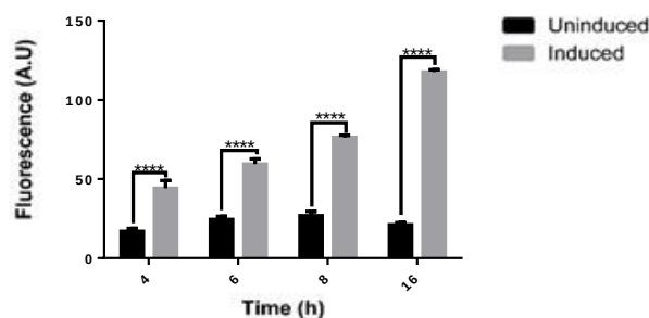
Figure 122. Time-dependent characterization of the pET22b-ABS-ParsR-ArsR-sfGFP-ProD-HucR sensor with 10 \mu M Sodium Arsenate ( \text{Na}_3\text{AsO}_4 ). E. coli PRO cells were grown in LB growth media at 25°C. Experiments were repeated in triplicates, and measurements were taken at 4 th , 6 th , 8 th and 16 th hours after induction. The results were analyzed with two-way analysis of variance (ANOVA) (GraphPad Prism version 9.0.0), the differences between the groups were marked with “*” ( p \leq 0.05 , p \leq 0.01 , p \leq 0.001 and p \leq 0.0001 is represented by “*”, “**”, “***” and “****” respectively). “ns” was used in the groups that did not show significant differences.
