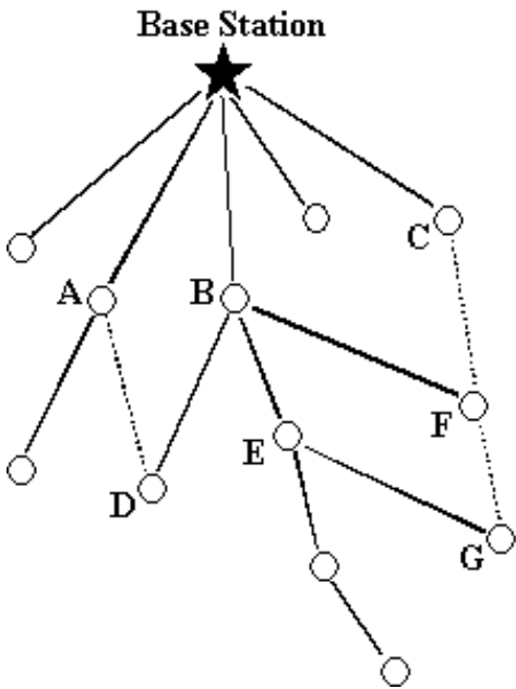
Figure 4.1: Unbalanced tree.
