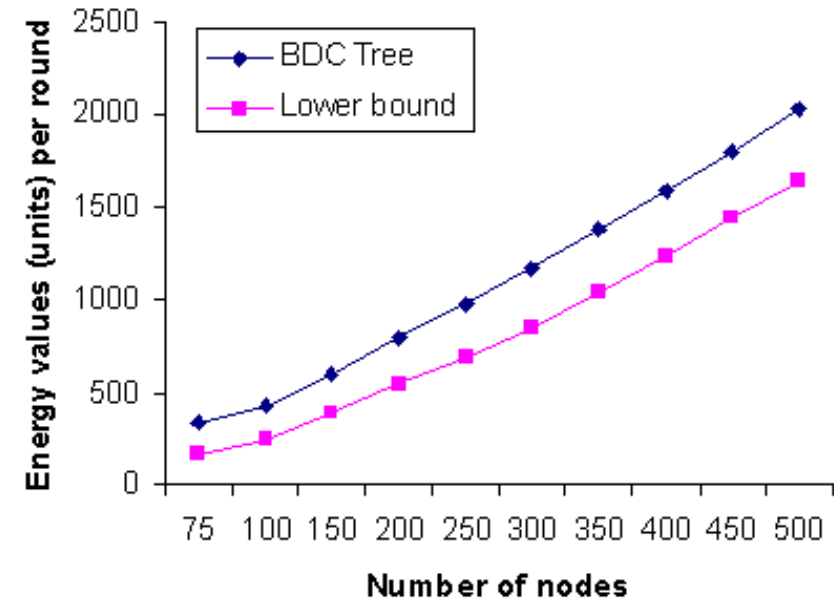
Figure 5.8: Comparison of energy consumptions of BDC Tree with lower bound.
