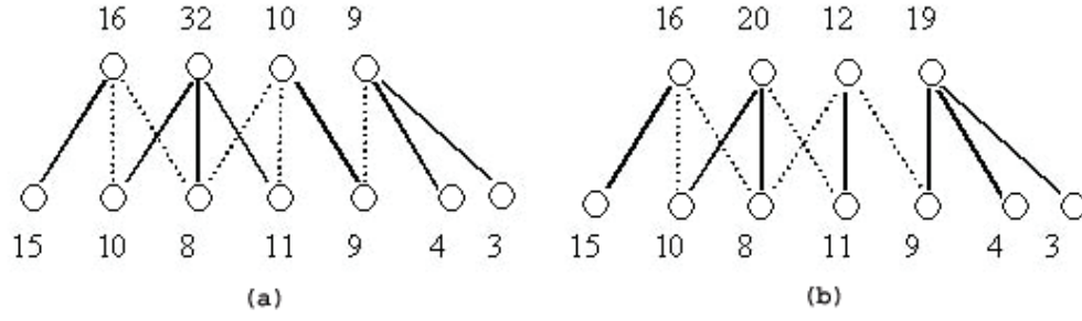
Figure 4.3: a) Unbalanced nodes; b) Balanced nodes
