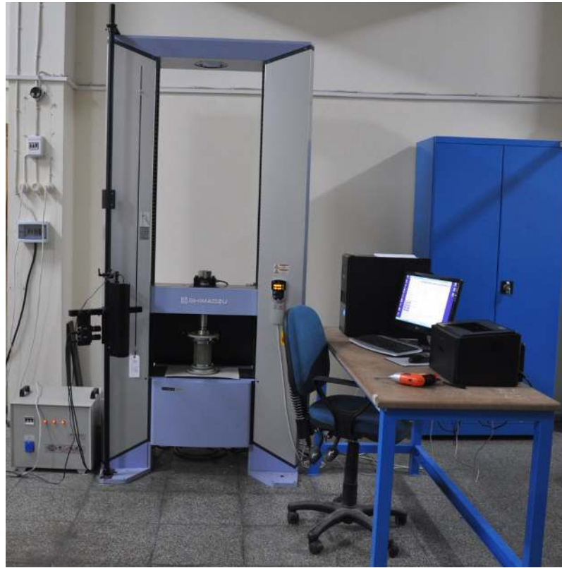
Figure 3.1 A view of the SHIMADZU test machine
