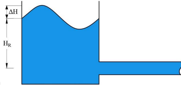
Figure 3.2. Upstream reservoir with variable head
