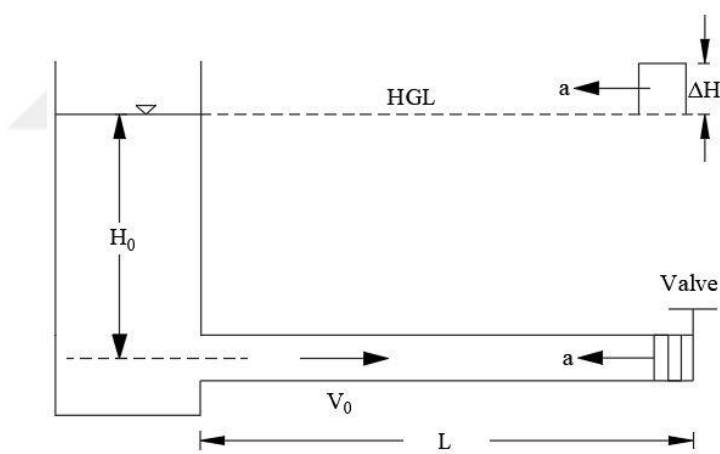
Figure 2.1. The pipeline system with a reservoir at upstream and a suddenly closed valve at downstream, Streeter & Wylie (1967)
