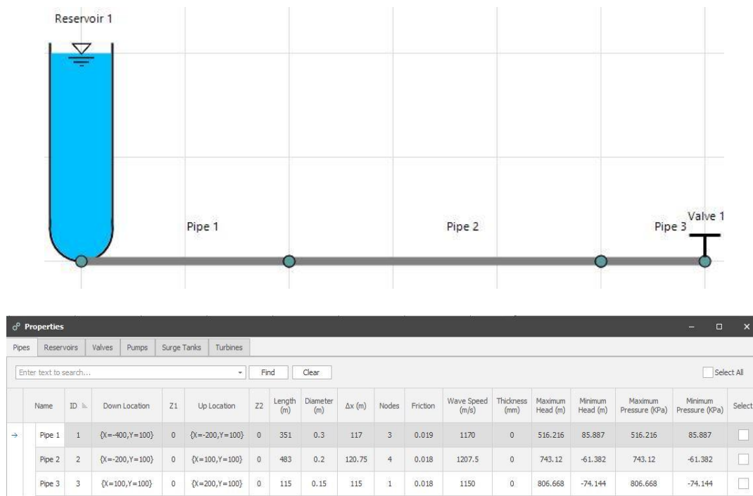
Figure 5.8. S-Hammer schematic view and the properties of the pipes of a case study by Wylie & Streeter
