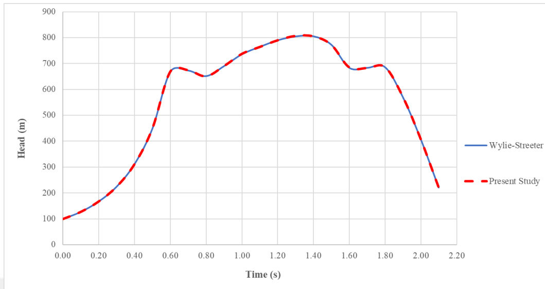
Figure 5.9. H vs. Time comparison at valve end (Wylie-Streeter vs. S-Hammer)
