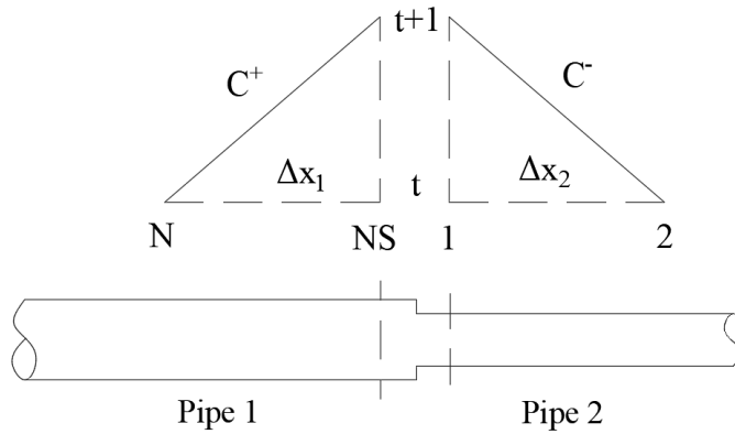
Figure 3.1. Series junction boundary condition
