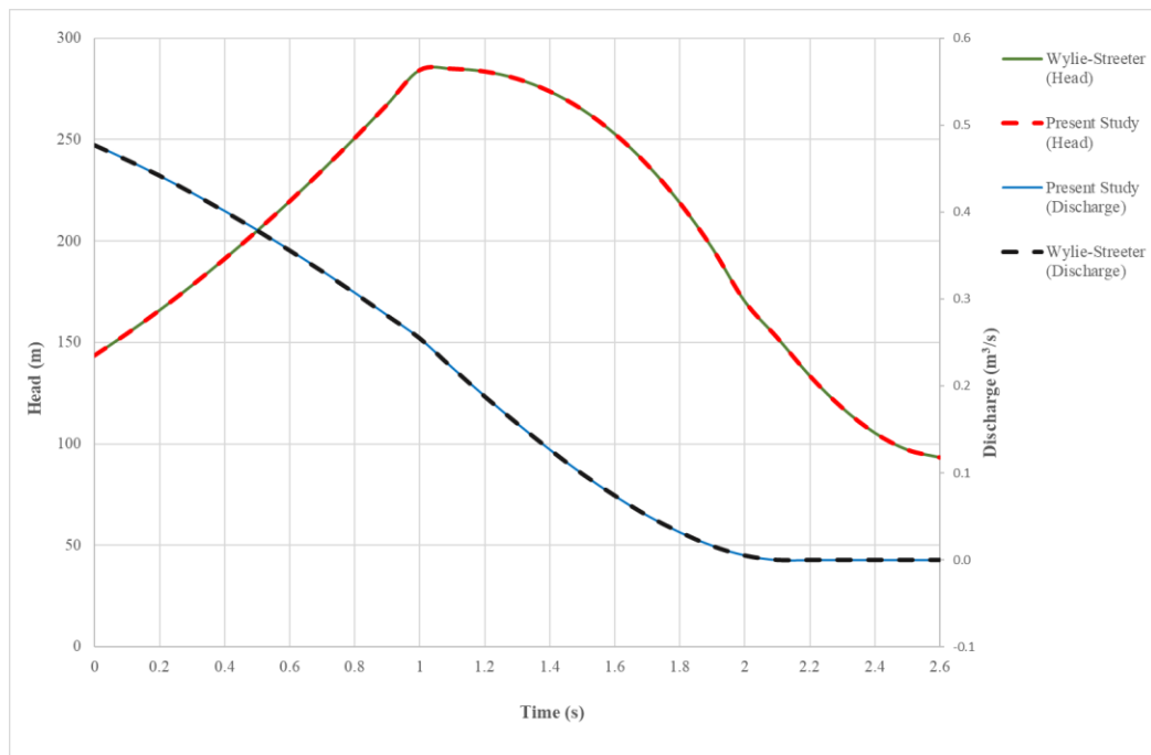
Figure 5.6. Single pipe comparison (H vs. Time) and (Q vs. Time) at valve end
