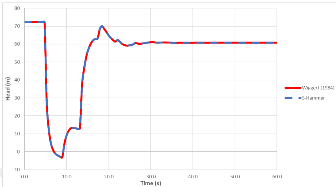
Figure 5.17. H vs. Time chart for pump failure with no discharge valve, at x = 0 m
