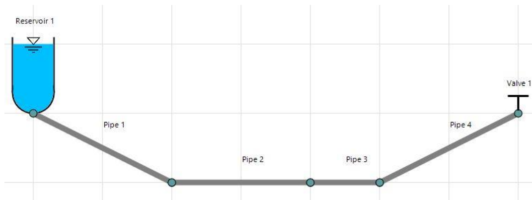
Figure A.3. A sample hydraulic system drawn in S-Hammer
