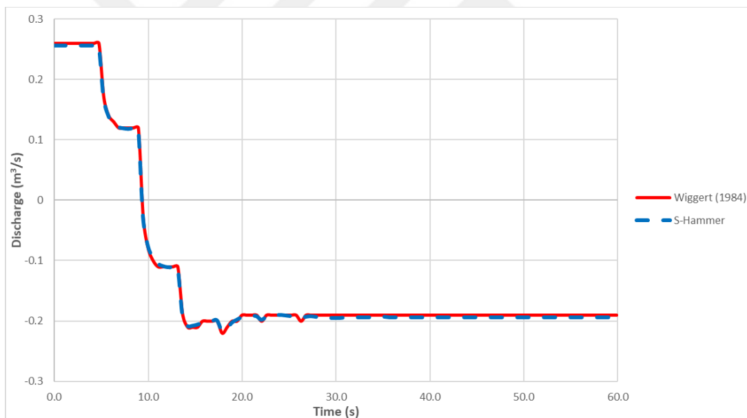
Figure 5.18. Q vs. Time chart for pump failure with no discharge valve, at x = 0 m
