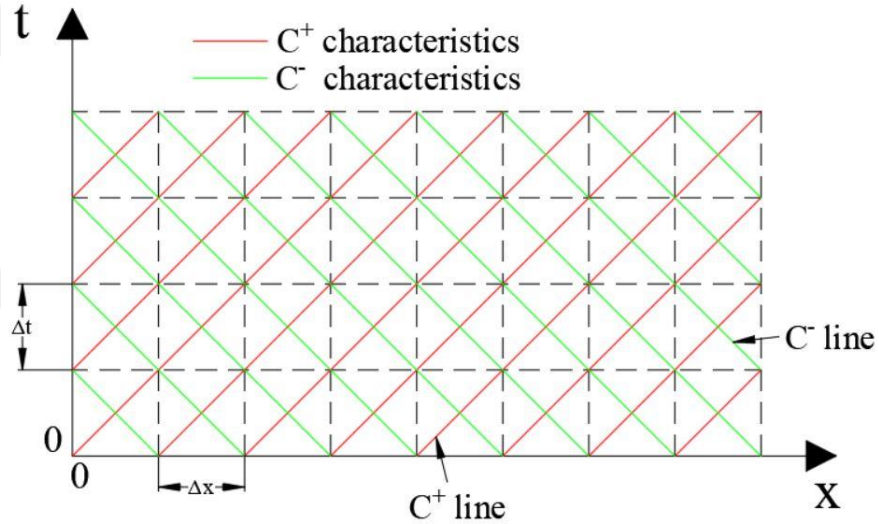
Figure 2.6. Characteristic lines in the x-t plane
