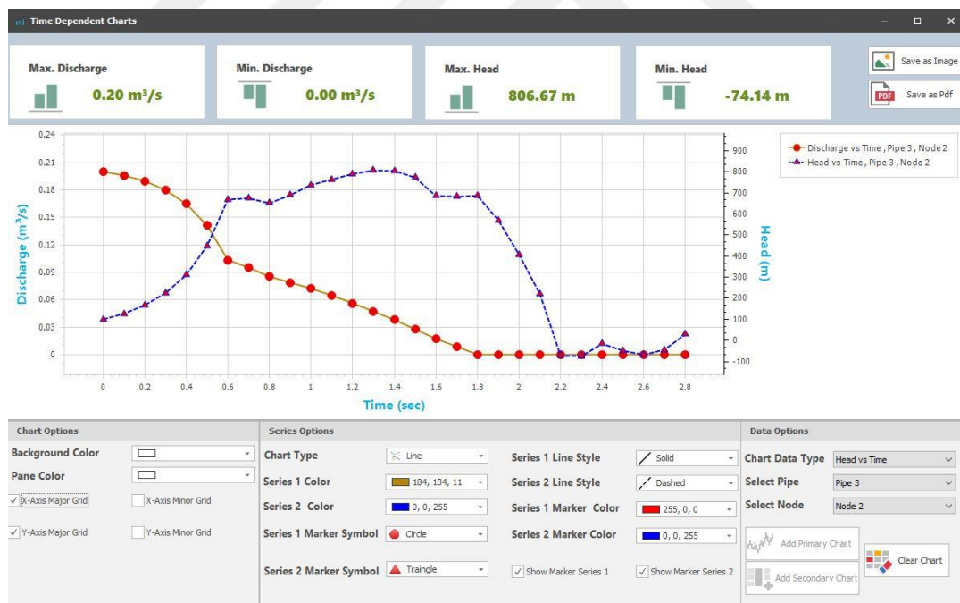
Figure 4.11. Time dependent graphical chart windows form
