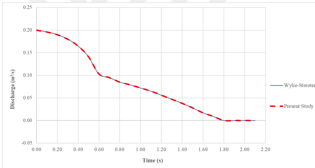
Figure 5.10. Q vs. Time comparison at valve end (Wylie-Streeter vs. S-Hammer)
