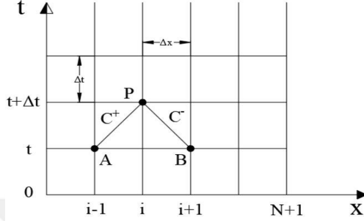
Figure 2.7. Characteristics lines for the nodal solution
