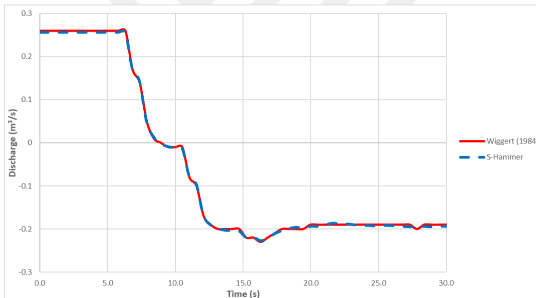
Figure 5.20. Q vs. Time chart for the pump with no discharge valve, at x = 1575 m
