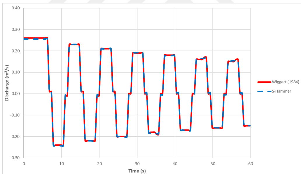
Figure 5.29. Q vs. Time chart for pump failure transient event with a discharge valve closing suddenly, at x = 1575 m
