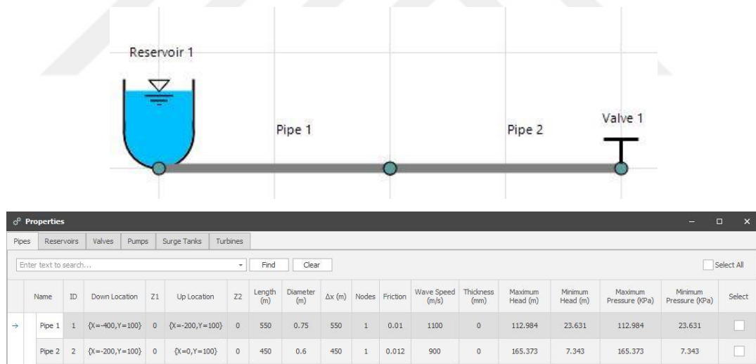
Figure 5.13. S-Hammer view and pipes properties of a case study by Chaudhry
