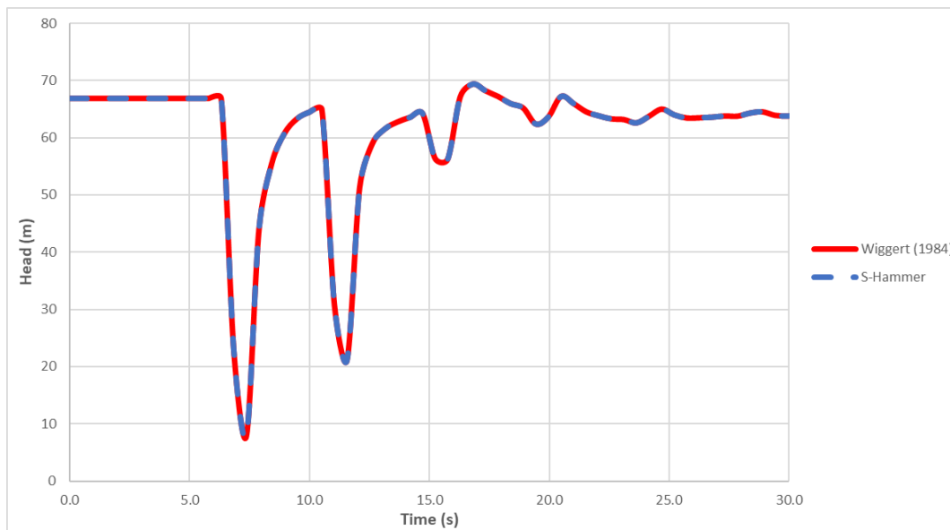
Figure 5.19. H vs. Time chart for the pump with no discharge valve, at x = 1575 m
