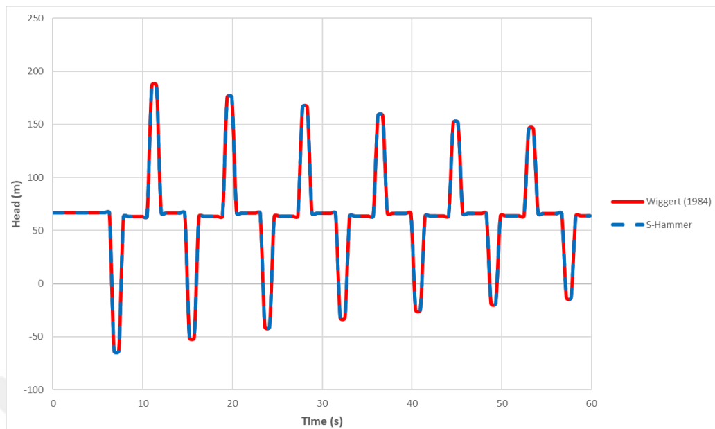
Figure 5.28. H vs. Time chart for pump failure transient event with a discharge valve closing suddenly, at x = 1575 m
