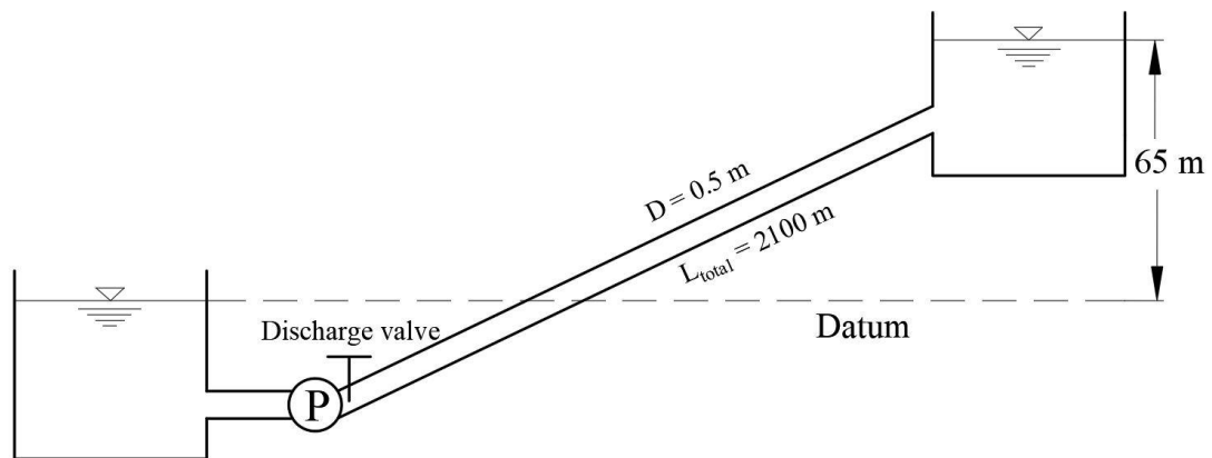
Figure 5.16. The hydraulic model for pump failure transient simulation
