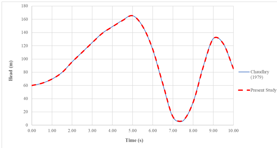
Figure 5.14. H vs. Time at valve end (Chaudhry vs. Present study)
