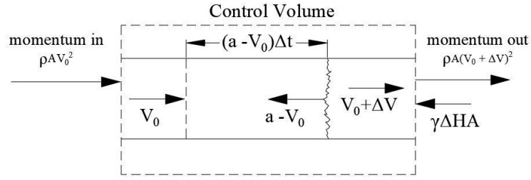
Figure 2.2. Implementation of the momentum equation to the control volume, Streeter & Wylie (1967, 1993)
