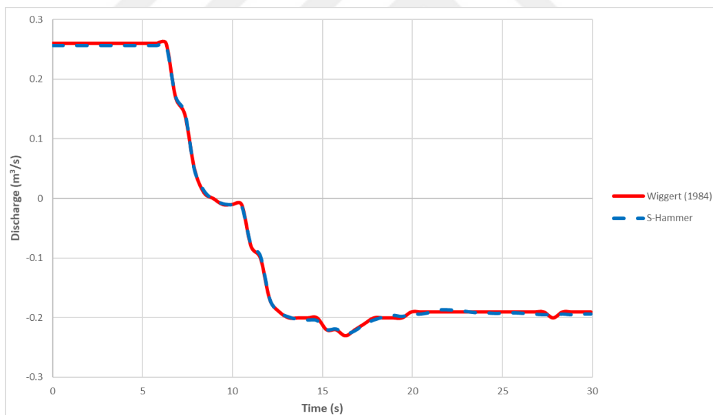
Figure 5.25. Q vs. Time chart for pump failure transient event with a discharge valve and t_c = 8 seconds, at x = 1575 m
