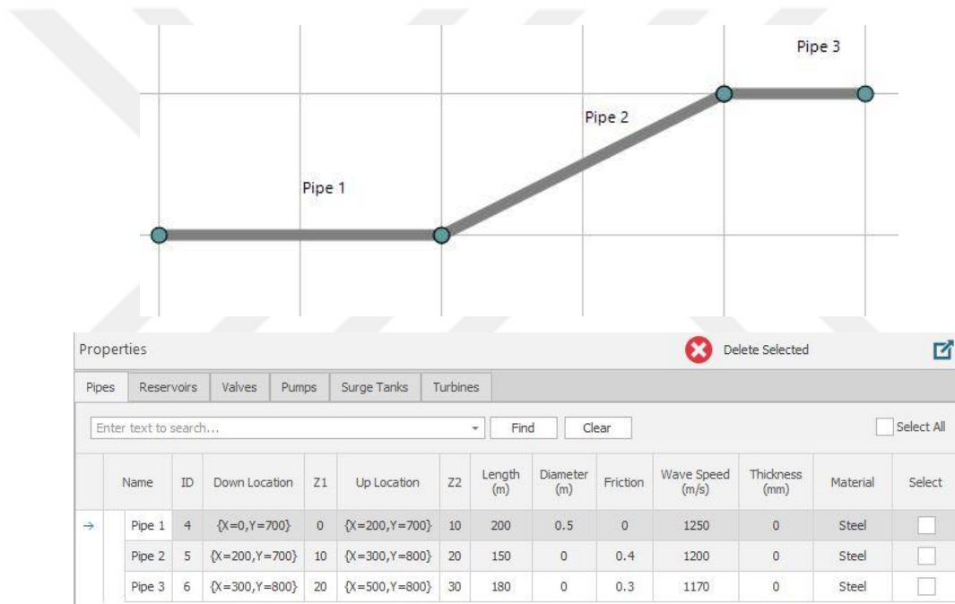
Figure 4.14. A scheme of pipe series and Pipe series property panel in the software
