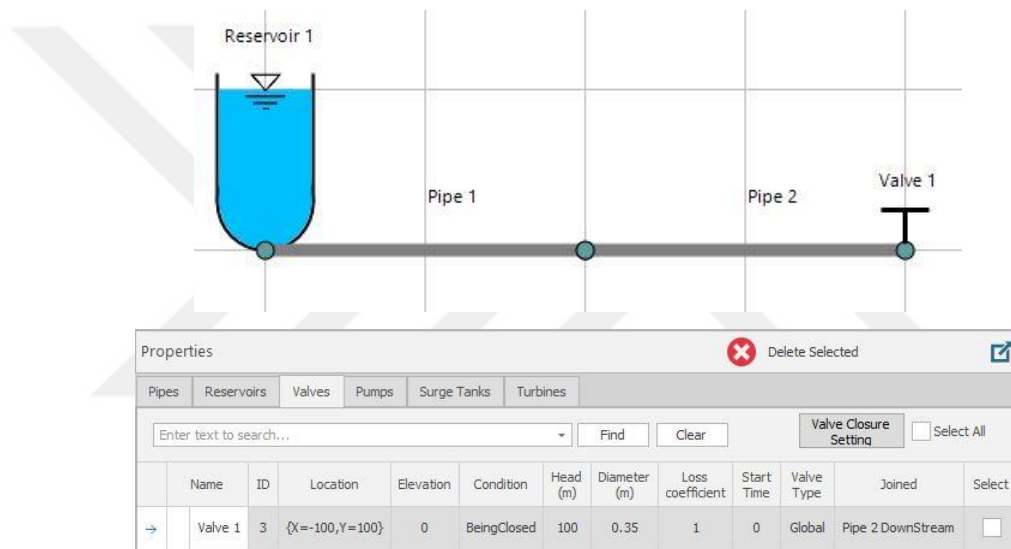
Figure 4.16. Valve objects view and its properties panel
