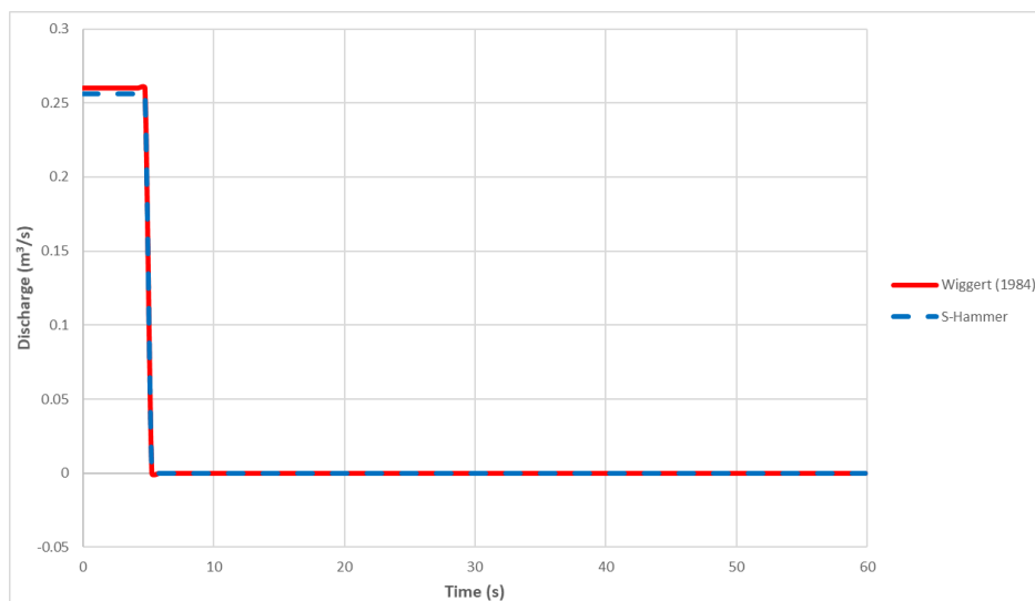
Figure 5.27. Q vs. Time chart for pump failure transient event with a discharge valve closing suddenly at x = 0 m
