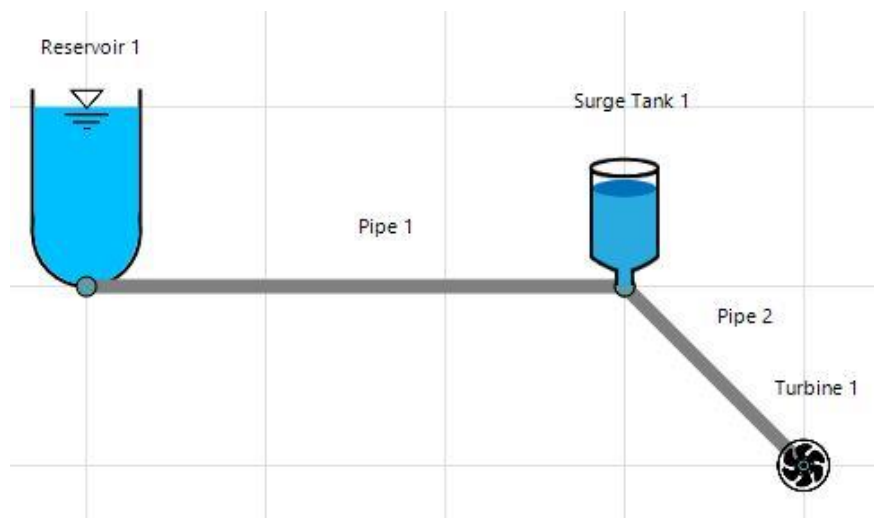
Figure 4.21. Surge tank added to the system in the design stage
