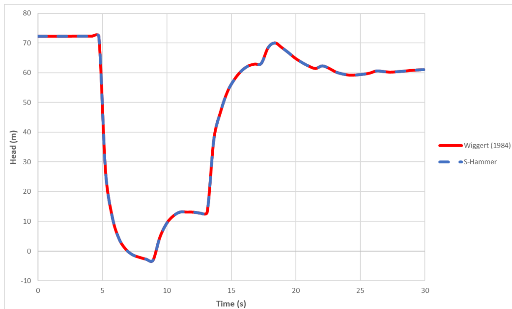
Figure 5.22. H vs. Time chart for pump failure transient event with a discharge valve and t_c = 8 s, at x = 0 m
