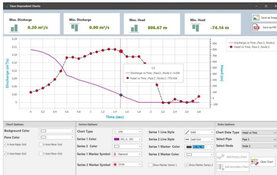
Figure 4.12. A feature of the graphical charts form
