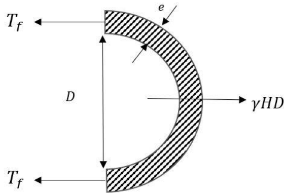
Figure 2.4. Circumferential pipe stress forces because of water hammer
