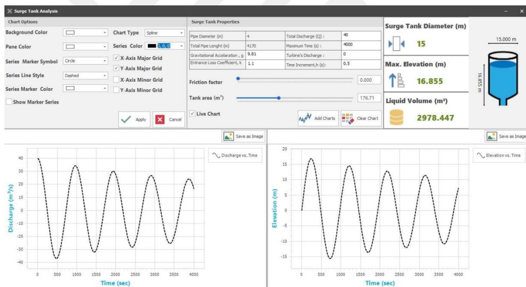
Figure 5.31. Simple surge tank simulations of S-Hammer
