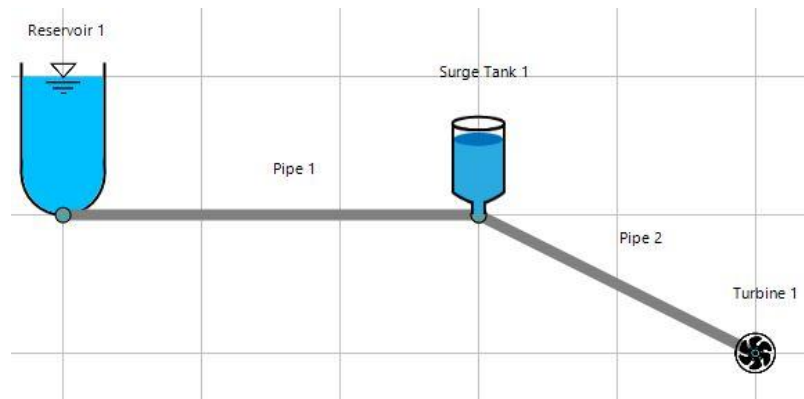
Figure 5.30. Simple surge tank model (Cofcof, 2011)
