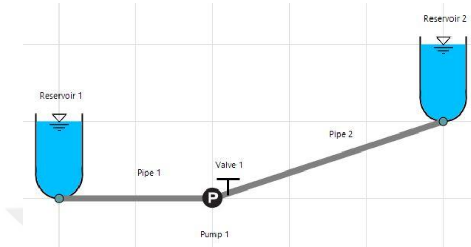
Figure 4.18. A sample of a system pumping water from an upstream lower reservoir to a downstream upper reservoir
