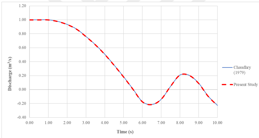
Figure 5.15. Q vs. Time at the reservoir (Chaudhry vs. Present study)
