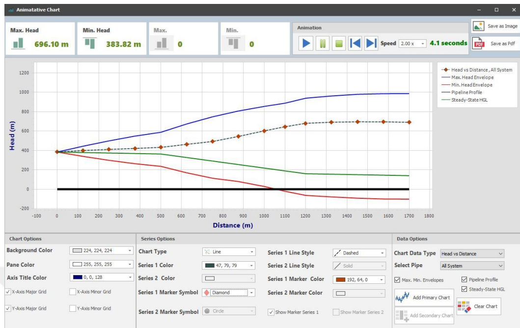
Figure A.12. Animative chart result for the example model
