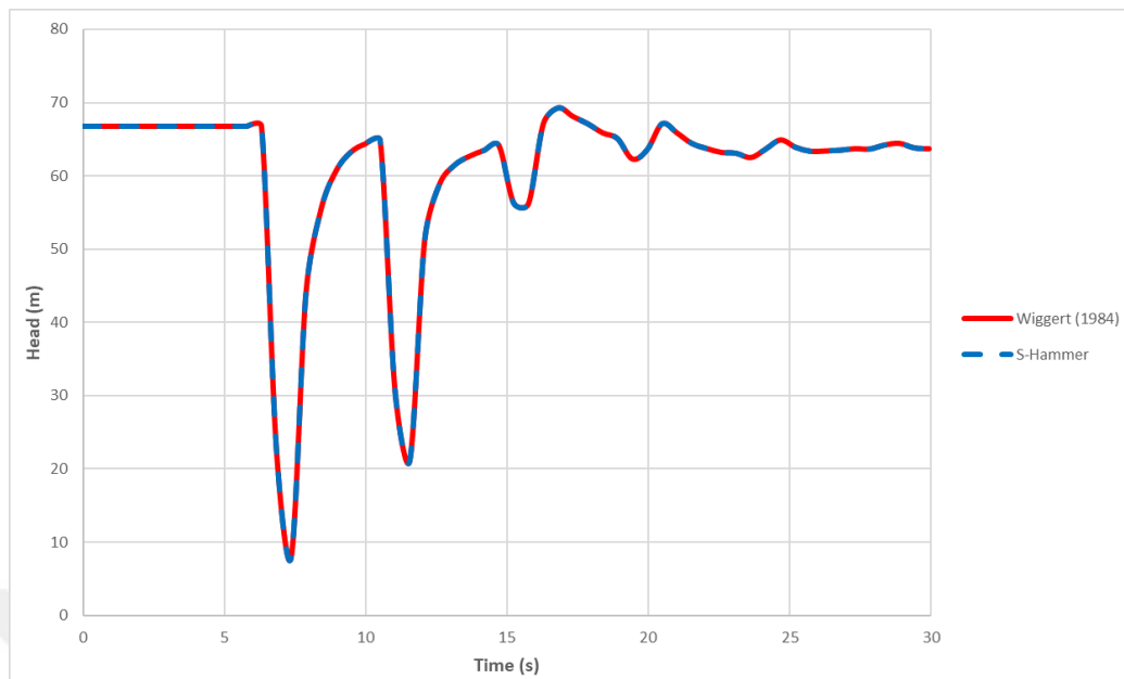
Figure 5.24. H vs. Time chart for pump failure transient event with a discharge valve and t_c = 8 seconds, at x = 1575 m
