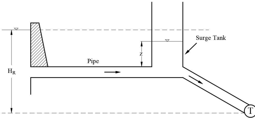
Figure 3.7. Simple surge tank
