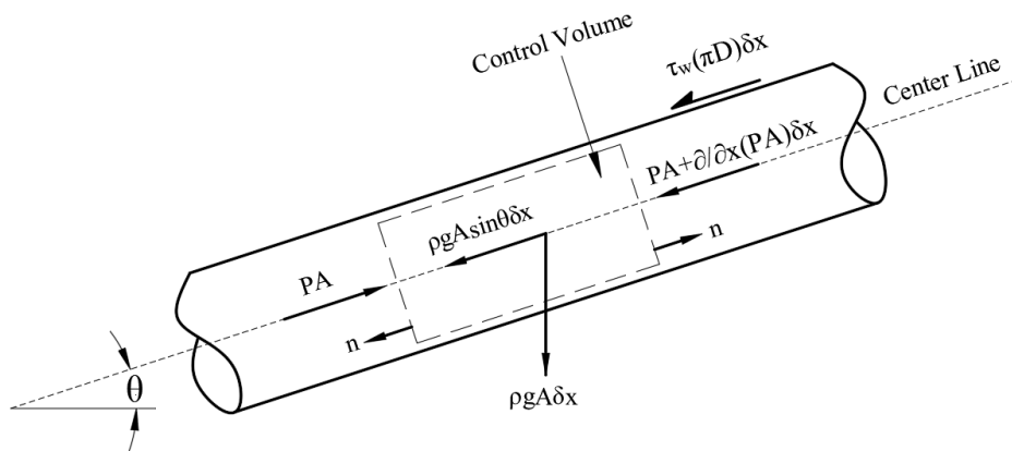
Figure 2.5. Selected control volume for the continuity and momentum equations
