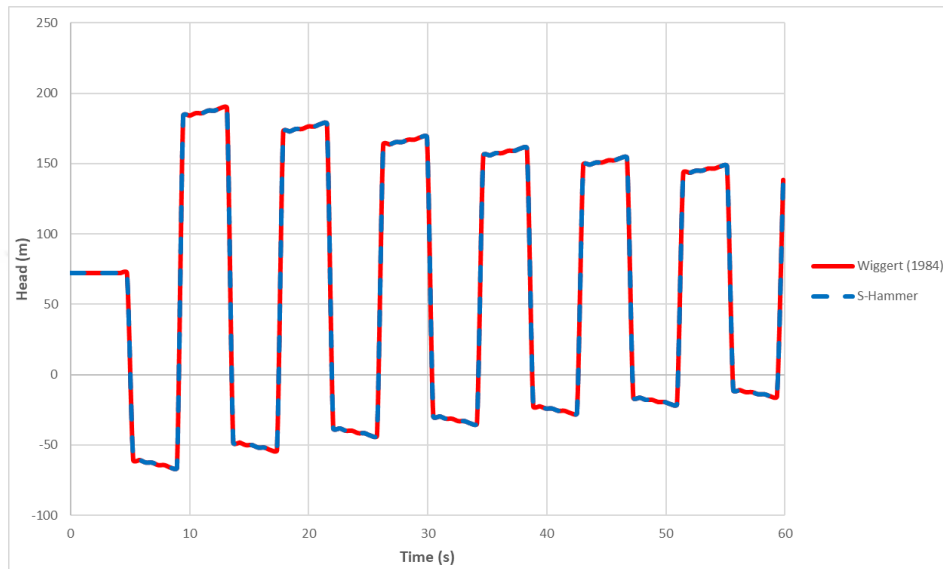
Figure 5.26. H vs. Time chart for pump failure transient event with a discharge valve closing suddenly at x = 0 m
