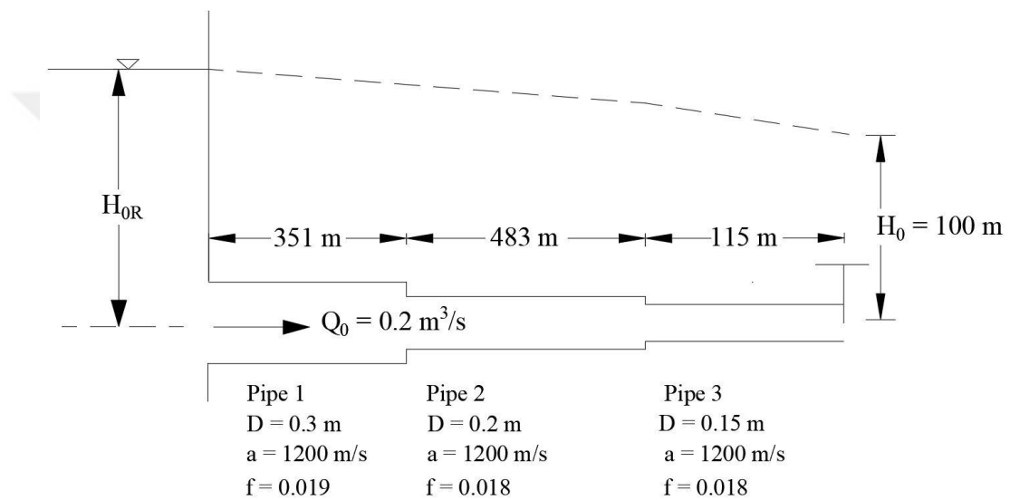
Figure 5.7. Series pipes case study, Wylie and Streeter (1978)
