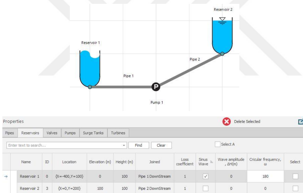
Figure 4.15. symbols of upstream and downstream reservoirs and upstream reservoir object properties panel
