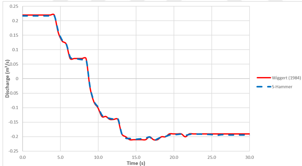
Figure 5.23. Discharge vs. Time chart for pump failure transient event with a discharge valve and t_c = 8 seconds, at x = 0 m
