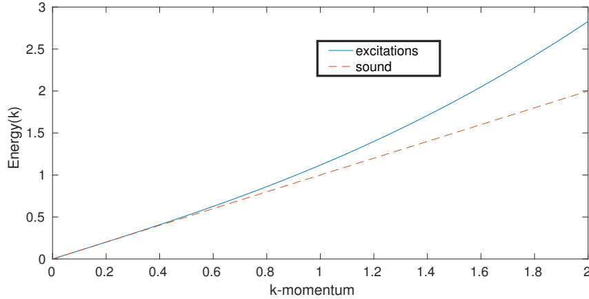
Figure 2.2: Spectrum of Bogoliubov excitations
