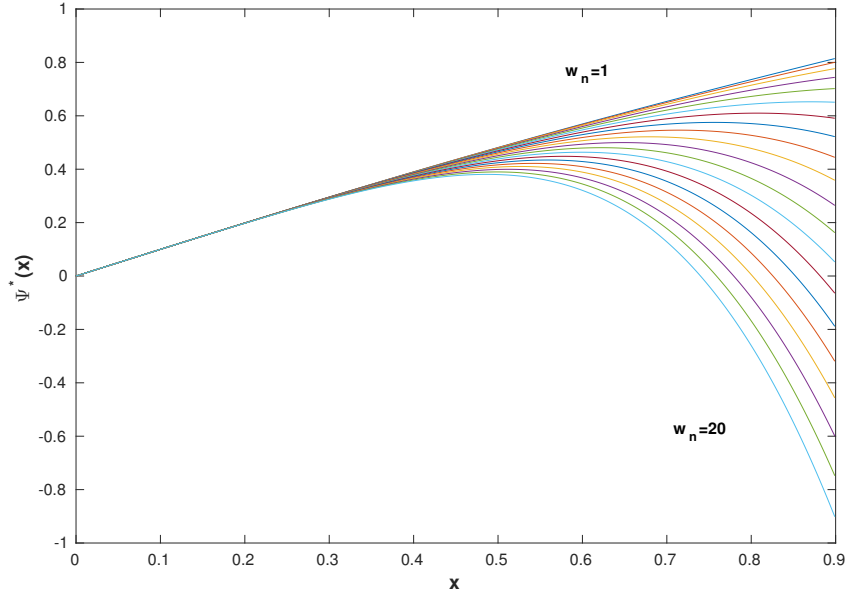
Figure 6.3: \bar{\psi}(x) for first 20 modes
