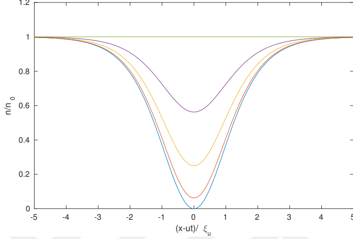
Figure 2.1: The density of a dark soliton for u^2/s^2 = 0, 0.25, 0.5, 0.75 , and 1
