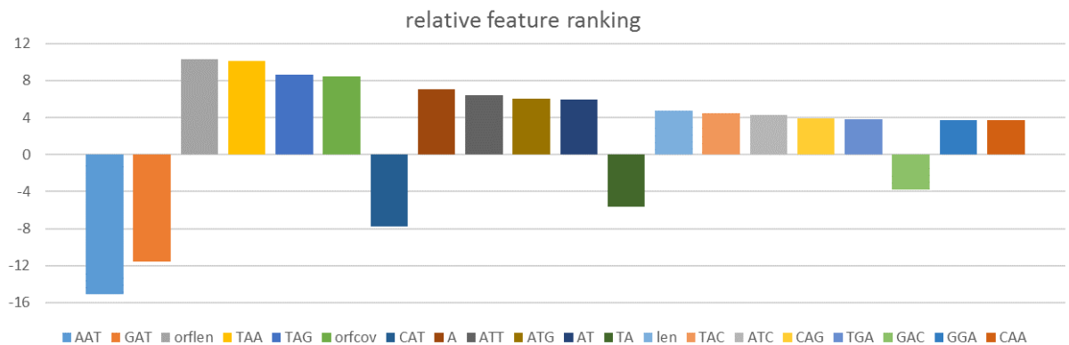
Figure 5.2. Feature ranking of wheat specific prediction model based on logistic regression. Relative feature ranking indicates the coefficient of the features in the decision function.
