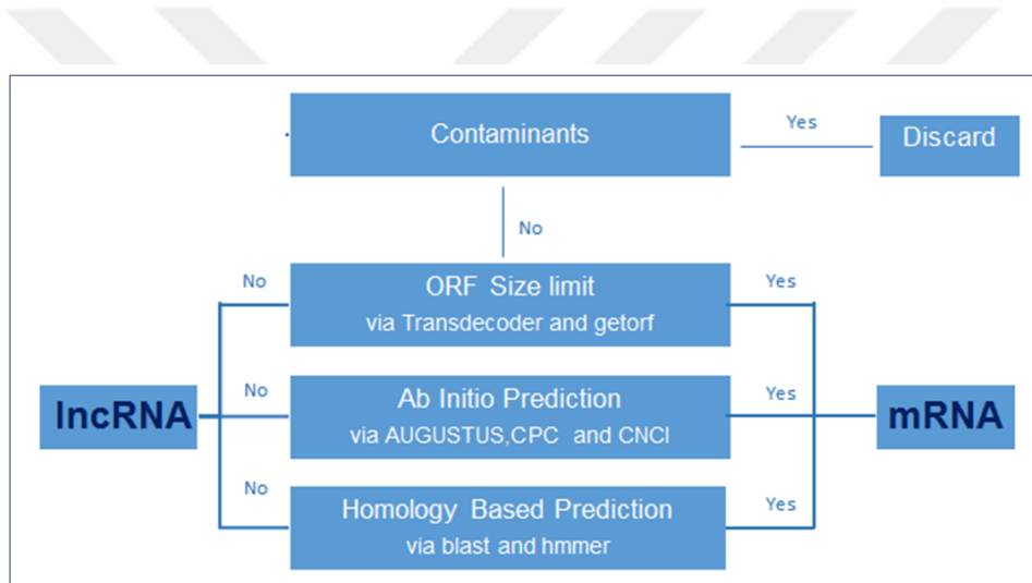
Figure 3.1. The pipeline for the identification and annotation of both coding transcripts and lncRNAs.
