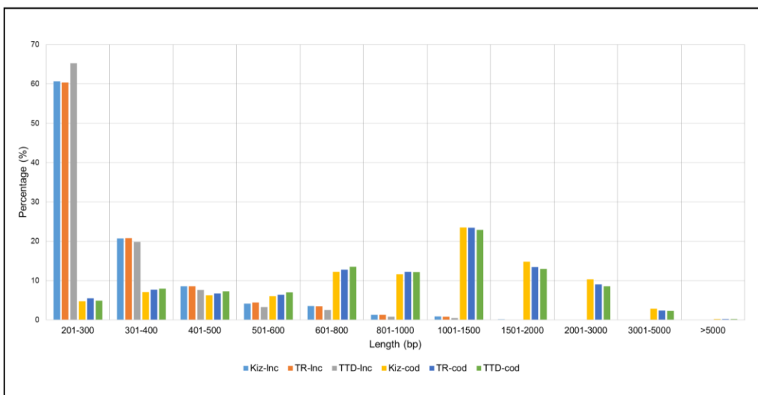
Supplementary Figure 2. Length distribution of lncRNAs and coding transcripts from each T. turgidum variety. (Graph legend: Kiz: Kiziltan, TR: TR39477, TTD: TTD-22; CK: control conditions, DS: drought stressed)
