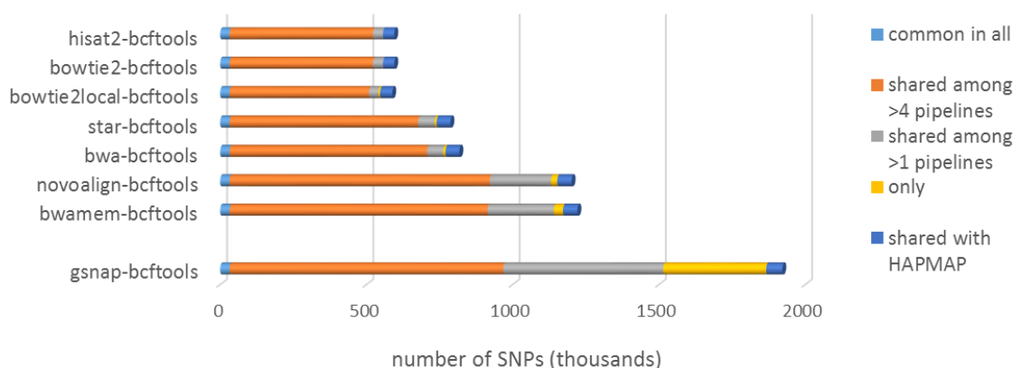
Figure 6.4. Distribution of number of SNPs called using bcftools call function as caller. The selected seven pipeline were separated from remaining gsnap-bcftools pipeline. ‘Shared with HAPMAP’ is additional to the total number of SNPs.
