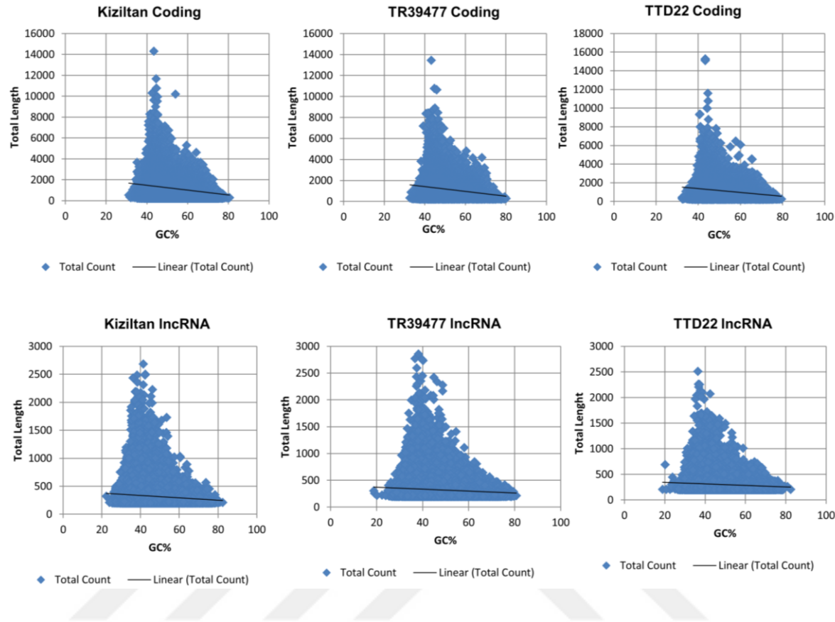
Supplementary Figure 3. Association between GC% content and length of lncRNAs from each T. turgidum variety.
