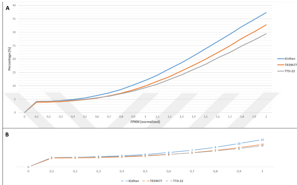
Supplementary Figure 1. The distribution of percent change of the number of transcripts over a set of FPKM cutoffs. Plot of percent change over 0 to 2 FPKM cutoffs (A). Closer look at the graph between the cutoffs of 0 to 1 (B).
