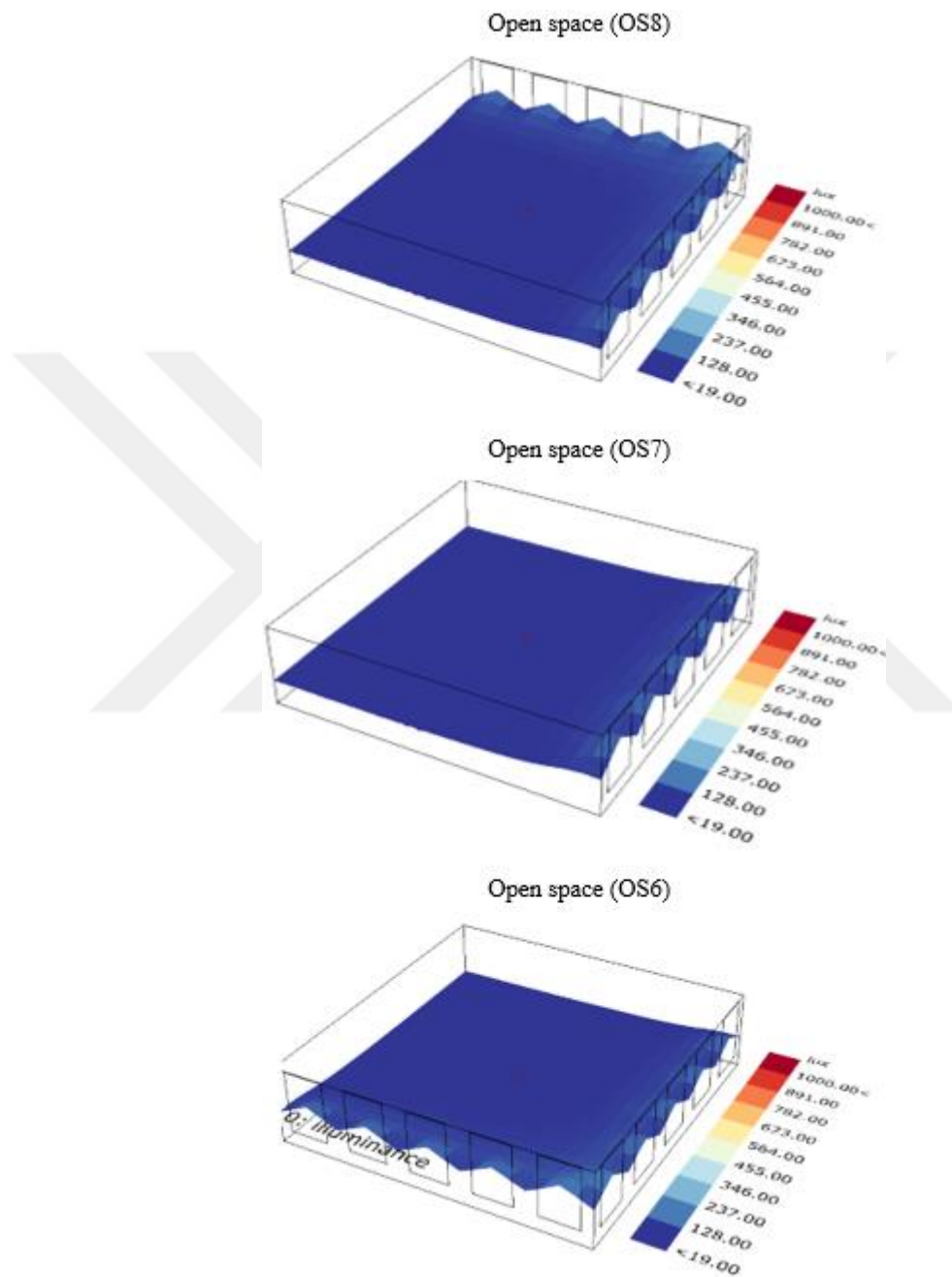
Figure 5.9. Sunlight impact for winter seasons (OS_8_7_6)
