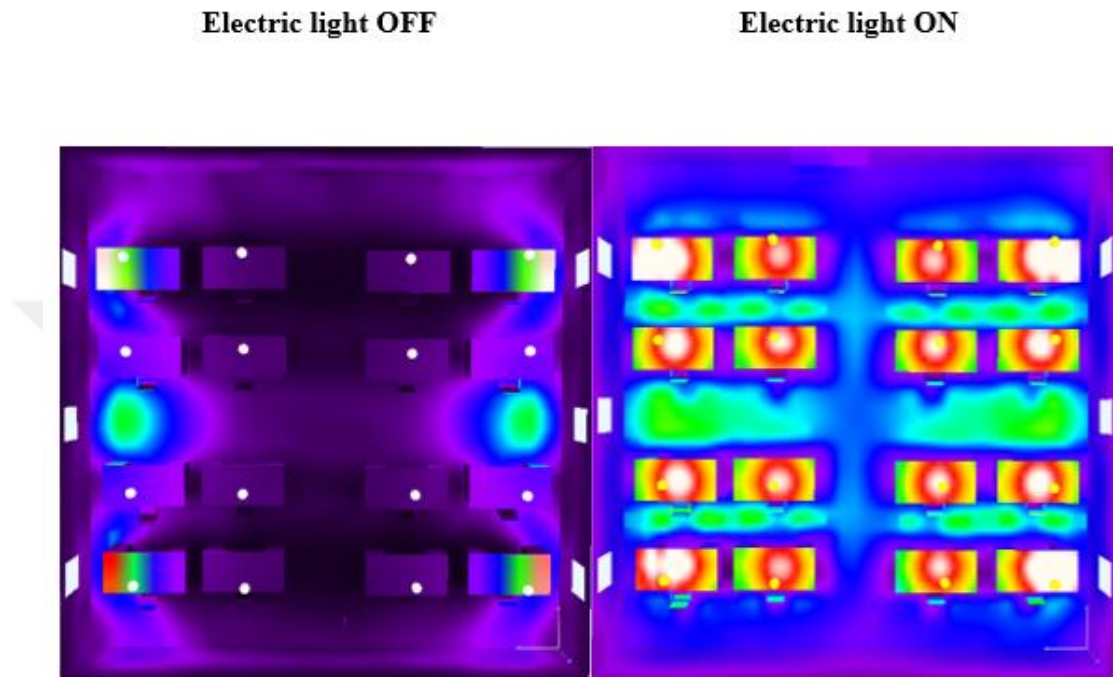
Figure 7.4. Day light impact in the open office
