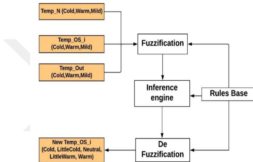
Figure 4.5. Block diagram of fuzzy logic (FL)
