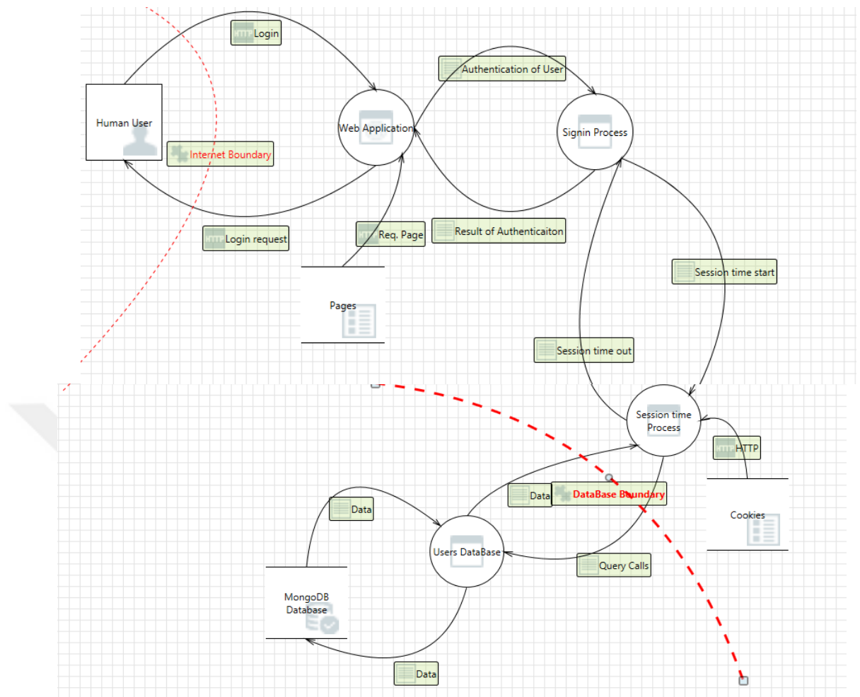
Figure 7.1. Data Flow Diagram
