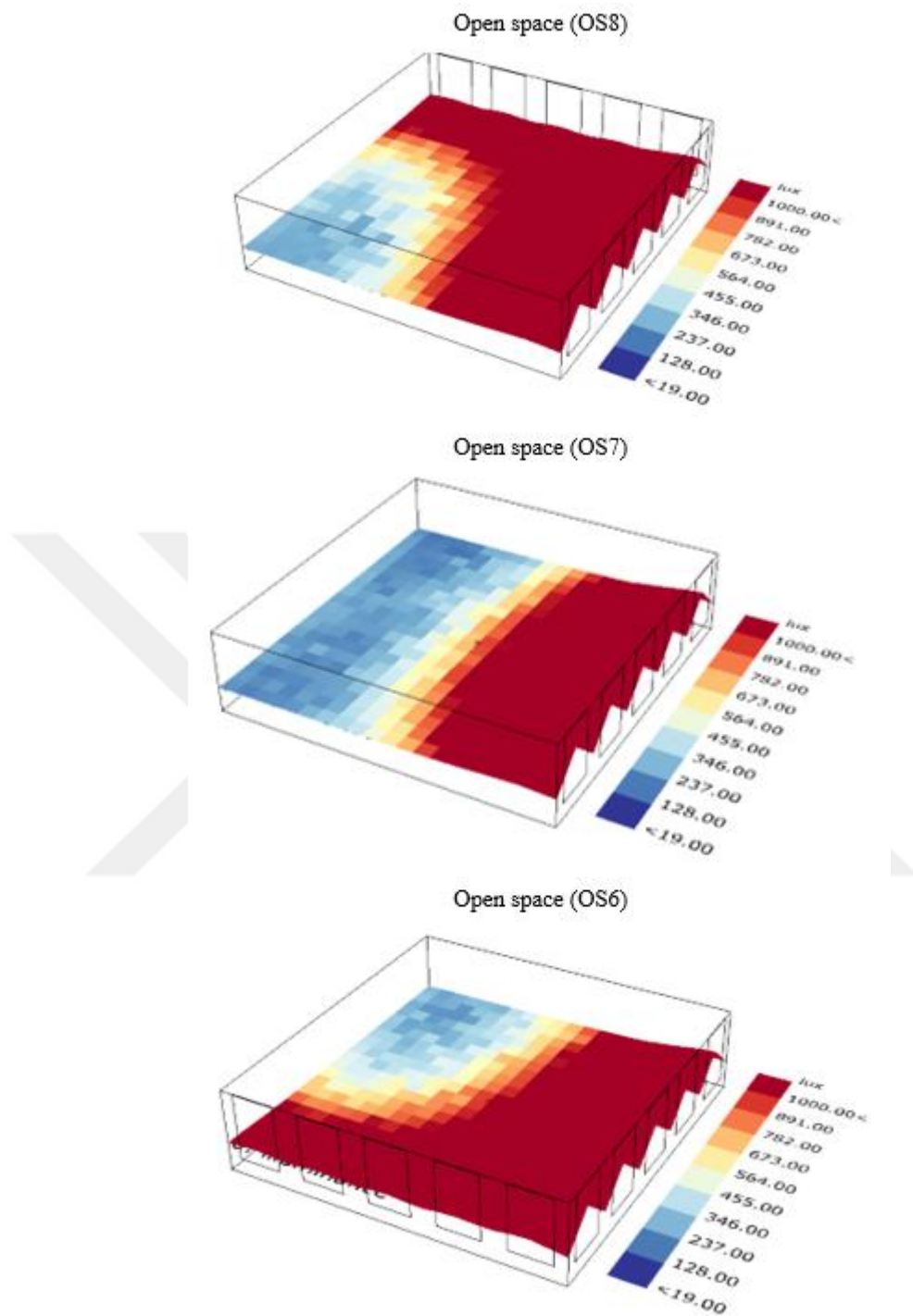
Figure 5.6. Sunlight impact for summer seasons (OS_8_7_6)
