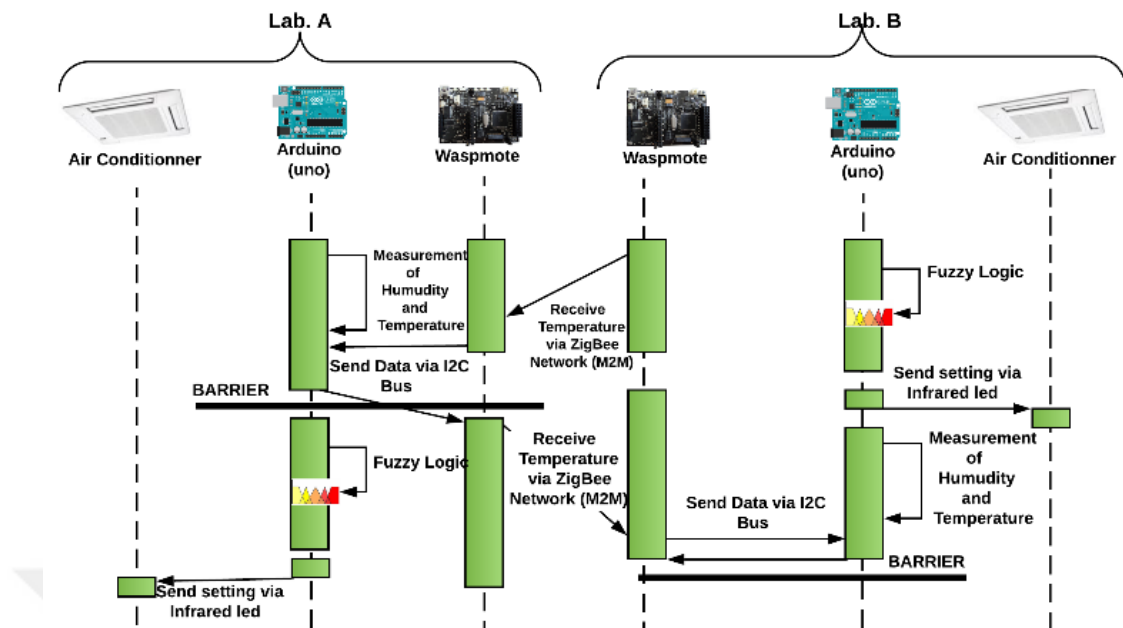
Figure 2.5. Sequence diagram of M2M communication
