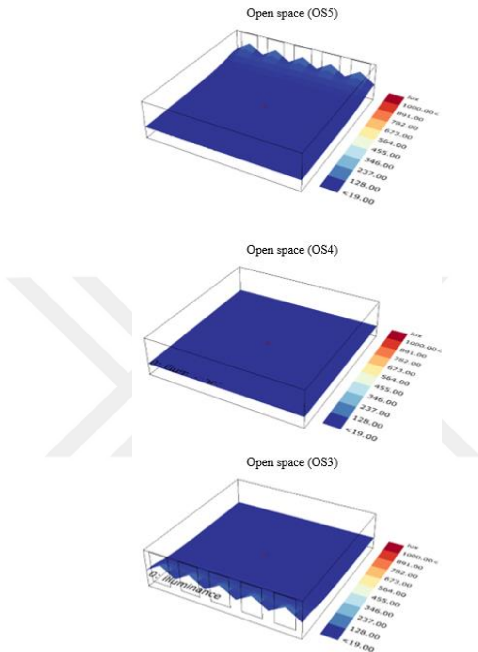
Figure 5.10. Sunlight impact for winter seasons (OS_5_4_3)
