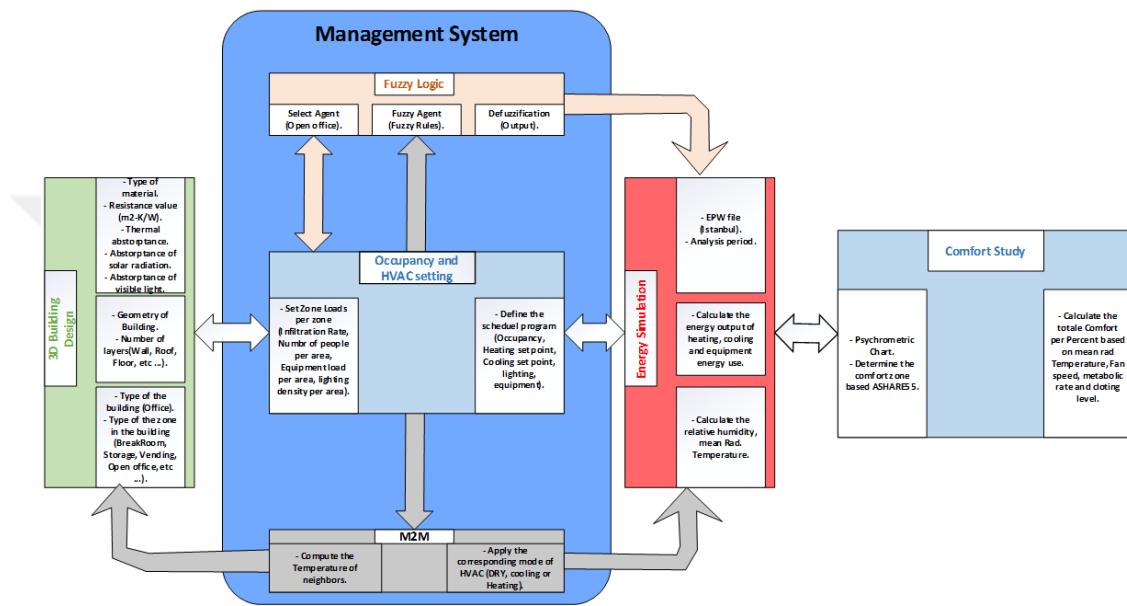
Figure 4.1. Outline of the proposed design
