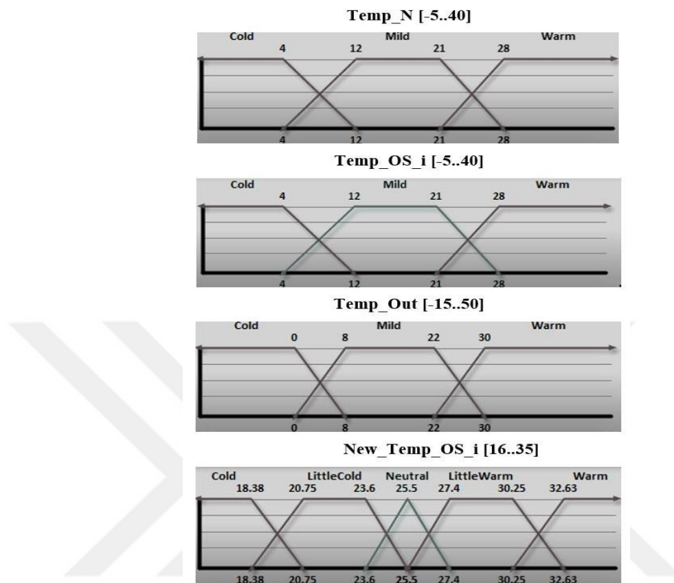
Figure 4.6. Membership functions of Input/Output
