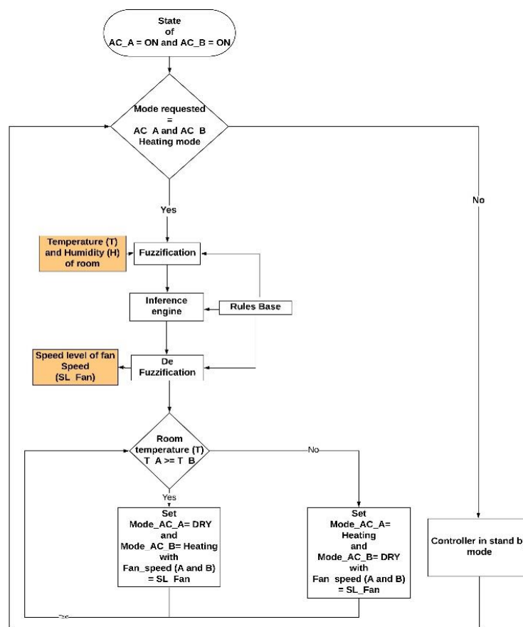
Figure 2.3. Flowchart of the management system
