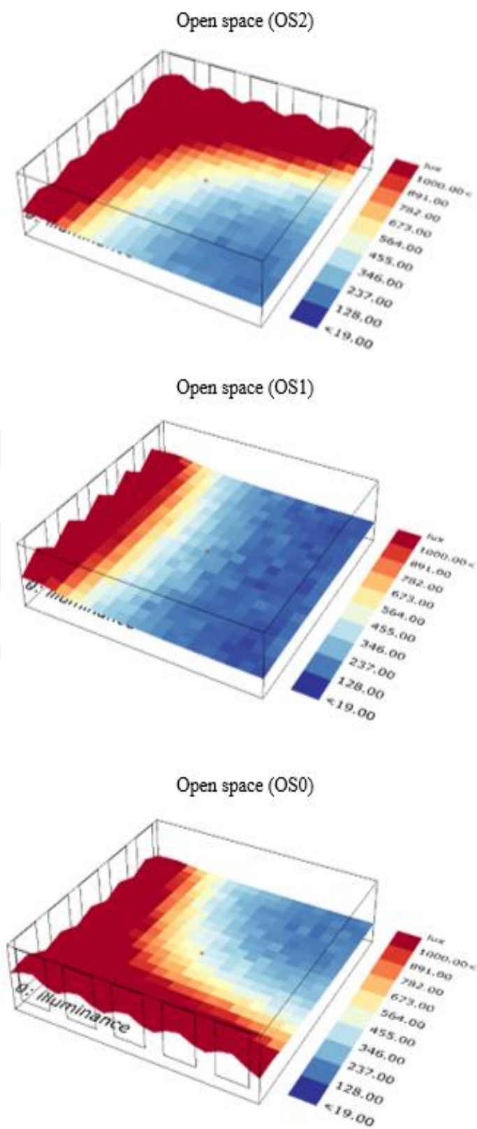
Figure 5.8. Sunlight impact for summer seasons (OS_2_1_0)
