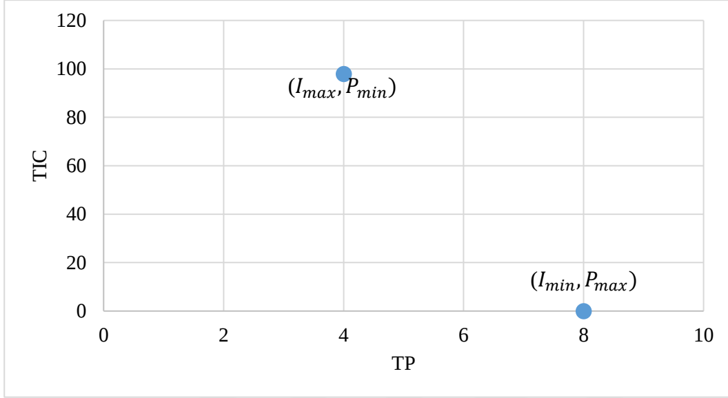
Figure 4.2. Extreme Nondominated Objective Vectors of Example Instance
