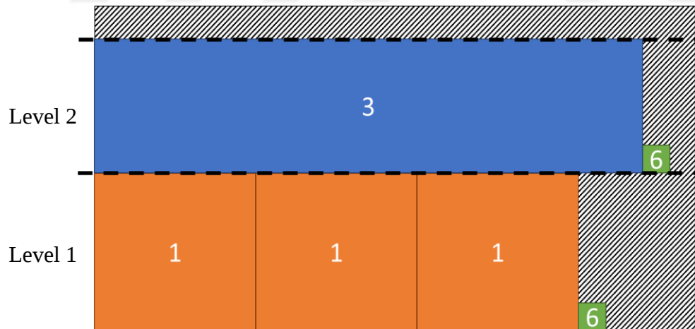
Figure 4.5. Cutting Scheme of Panel 1 at t = 1
