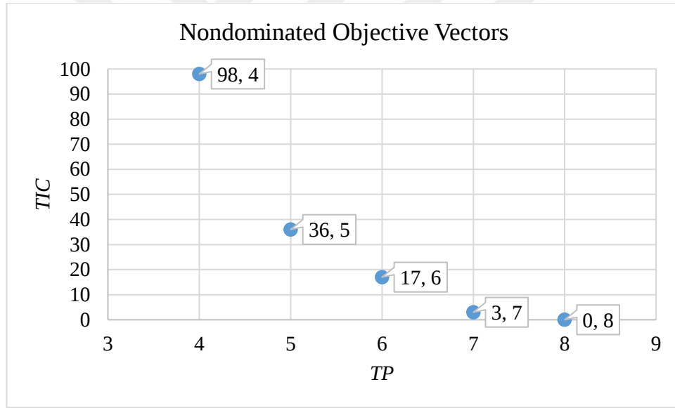
Figure 4.3. All Nondominated Objective Vectors for the Example Instance
