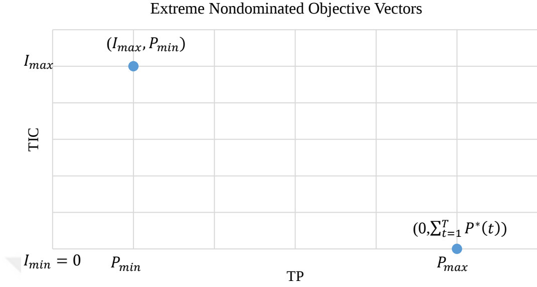
Figure 4.1. Extreme Nondominated Objective Vectors
