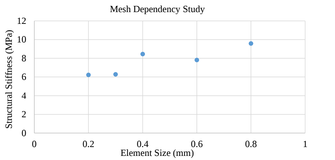
Figure 3.11 - Mesh dependency analysis of the structure.
