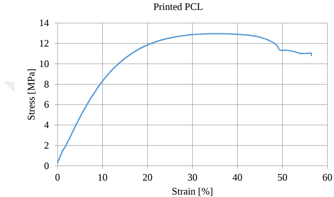
Figure 3.9 - Stress - strain curve of printed PCL.
