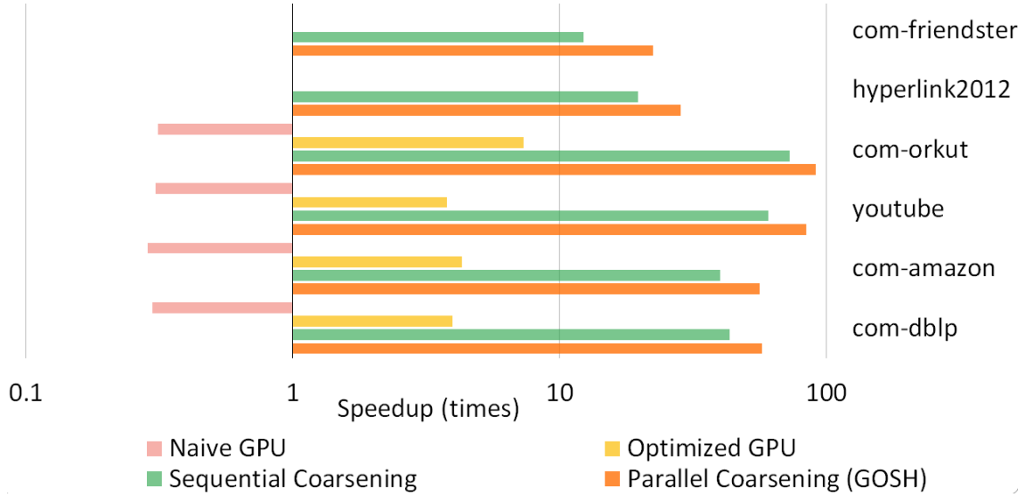
Figure 6.8 The speedups obtained from running intermediate versions of Gosh compared to our multi-core CPU implementation with 16 threads.
