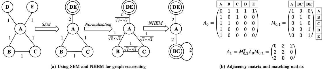
Figure 4.1 MILE Coarsening Strategy
