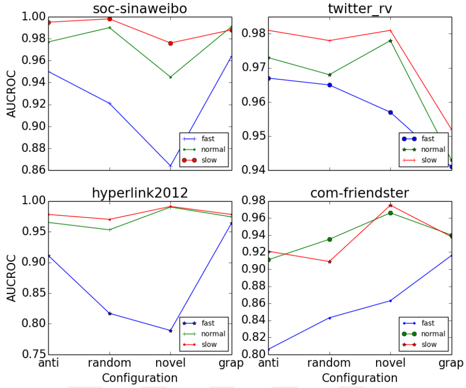
Figure 6.2 Large-scale graph results for different coarsening strategies and configurations.
