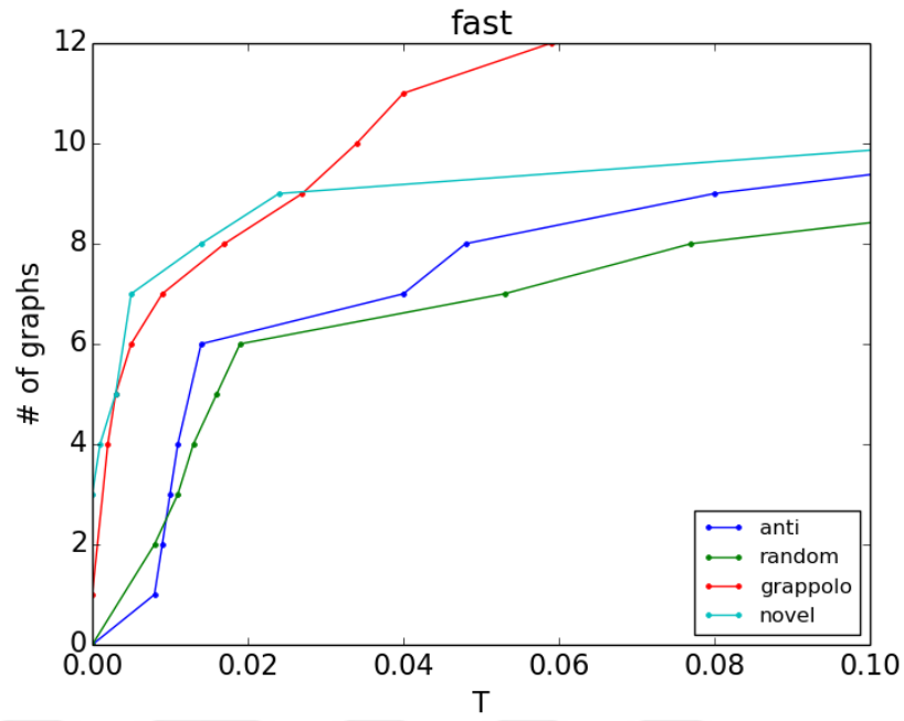
Figure 6.4 Performance profile of Gosh using fast configuration with different coarsening strategies for the entire data-set.
