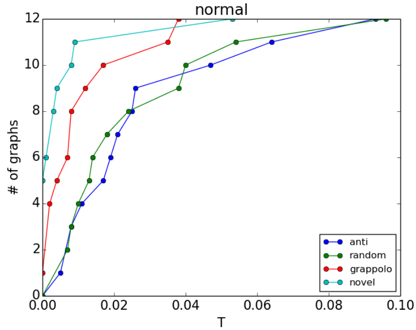
Figure 6.5 Performance profile of Gosh using normal configuration with different coarsening strategies for the entire data-set.
