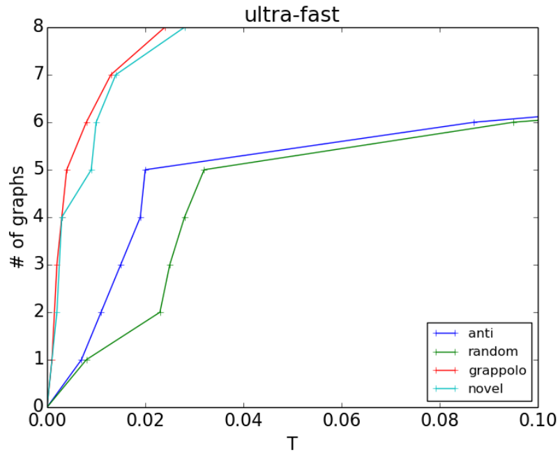
Figure 6.3 Performance profile of Gosh using ultra-fast configuration with different coarsening strategies for the entire data-set.
