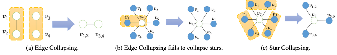
Figure 4.2 HARP Coarsening Strategy
