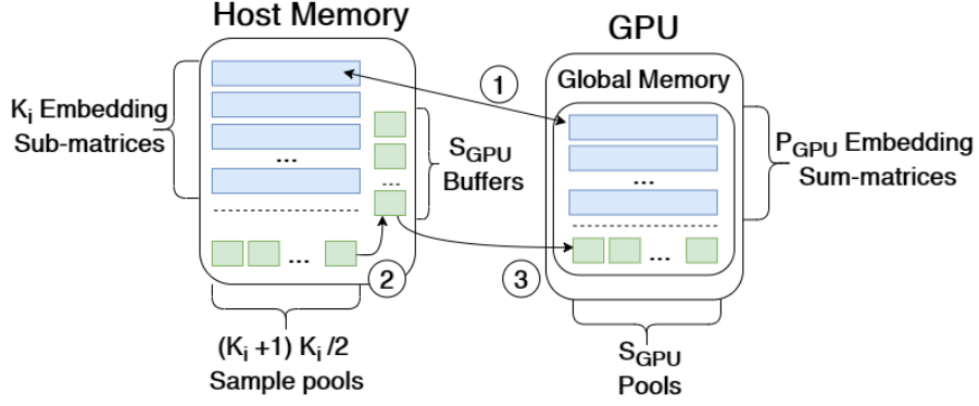
Figure 3.2 Memory model of large graphs algorithm embedding graph G_i . 1) Embedding sub-matrices are copied between the host and GPU as needed, 2) When sample pool S_i^{j,k} is ready, it is copied to an empty buffer. 3) When a sample pool on the GPU is used up, it is replaced by the next sample pool from the buffer.
