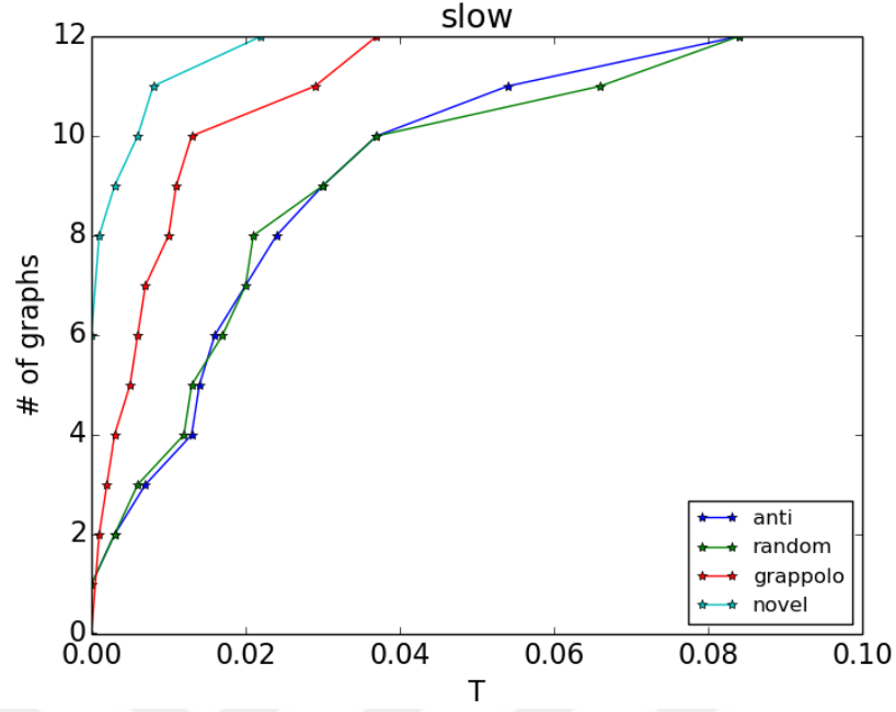
Figure 6.6 Performance profile of Gosh using slow configuration with different coarsening strategies for the entire data-set.
