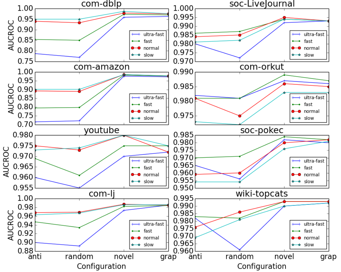
Figure 6.1 Medium-scale graph results for different coarsening strategies and configurations.
