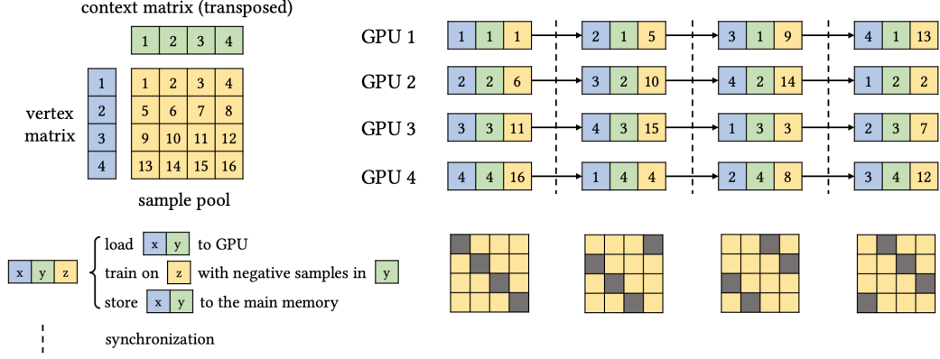
Figure 5.1 GraphVite Embedding with Multiple GPUs (Zhu et al., 2019)
