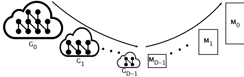
Figure 3.1 Multilevel embedding performed by Gosh : first, the coarsened set of graphs are generated. Then, the embedding matrices are trained until \mathbf{M}_0 is obtained. The original graph is coarsened down into a smaller graph, and then that graph is coarsened, and so on. The smallest graph is then embedded, and its embeddings are projected onto the higher graph, and then that graph is embedded and that continues upwards until the original graph is embedded.
