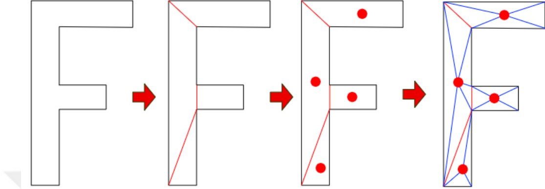
Figure 6.3: Illustration of the surface closure algorithm: from left to right: projected boundary polygon; Planar Straight Line Graph (PSLG) after convex decomposition where red edges are newly added; centroids calculated for each convex polygon; and sub-polygon vertices and centroids of each convex polygon connected with blue edges.
