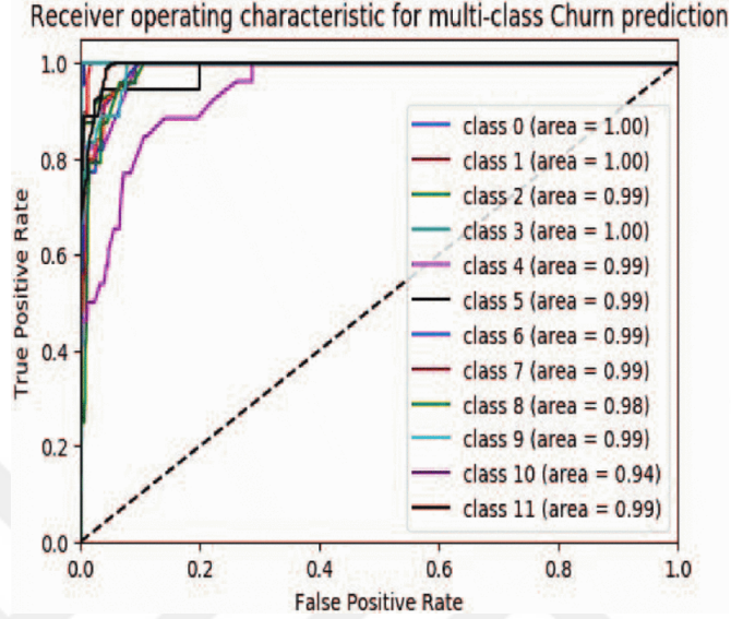
Figure 4.6: Receiver operating characteristics (ROC) for multi-class churn prediction using random forest classifiers
