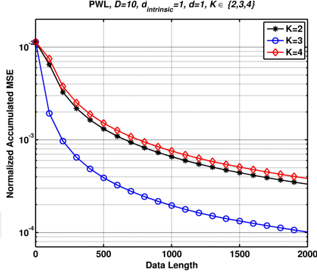
Figure 2.6: Piecewise Linear Prediction on high dimensional, time varying submanifolds using Adaptive Hierarchical Trees. D = 10, d_{\text{intrinsic}} = 1, d = 1 , and K = 2, 3, 4 d = 1, 2, 3 in Fig. 2.7.
