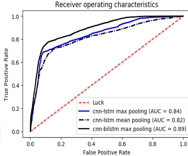
Figure 3.6: Receiver operating characteristics (ROC) for comparison of unidirectional and bidirectional LSTM units and show our results in Fig. 3.6.
