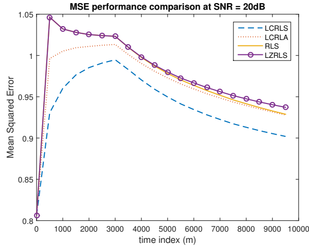
Figure 6.9: MSE analysis of different second order methods.
