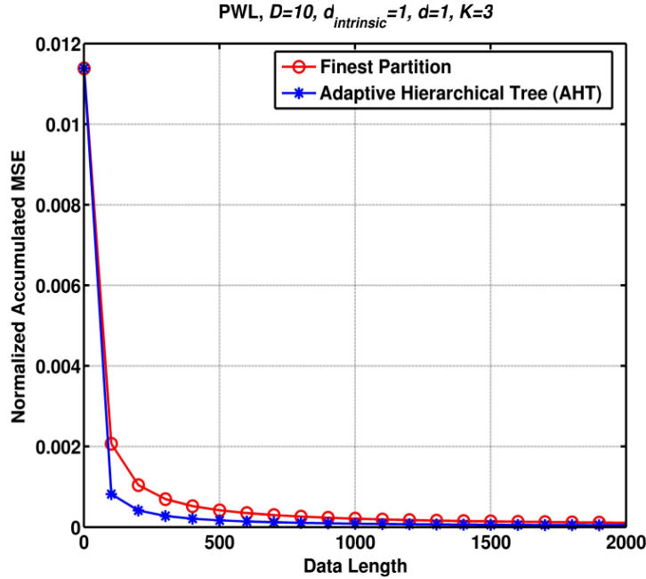
Figure 2.5: Sequential piecewise linear prediction of the desired data \hat{y}[n] of (2.26) with d = 1 and tree depth, K = 3 , sequential piecewise linear predictor with finest partitions on the tree.
