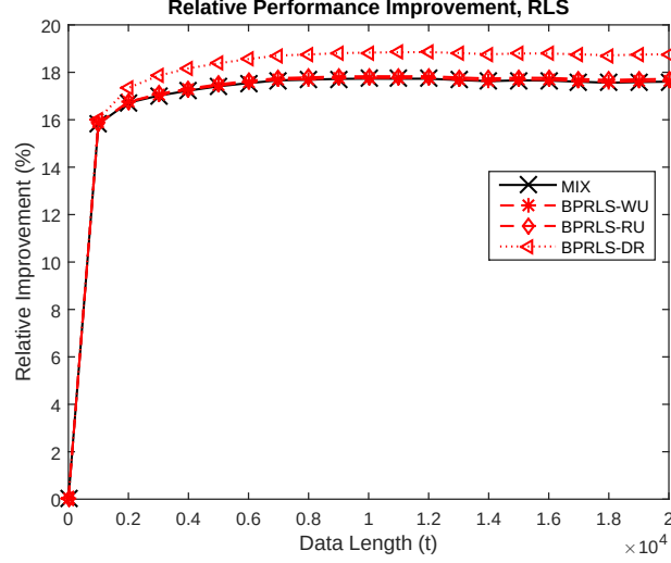
Figure 5.5: The relative improvement in ASE performance of the RLS-based algorithms in the stationary data experiment.
