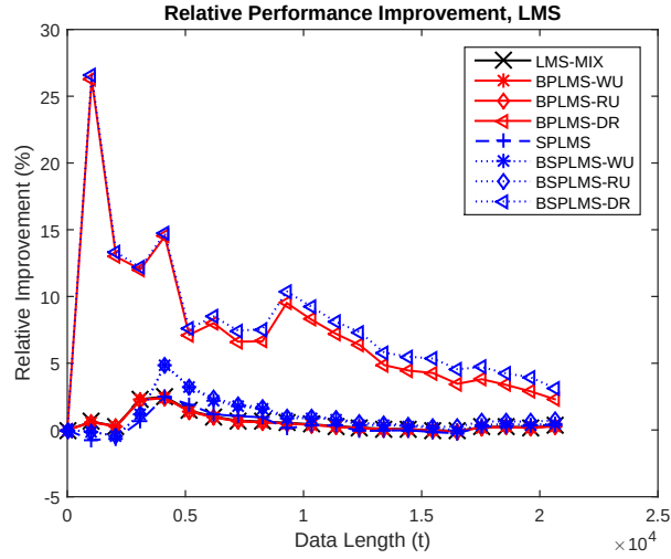
Figure 5.11: The performance of LMS-based boosting methods on the California Housing data set.
