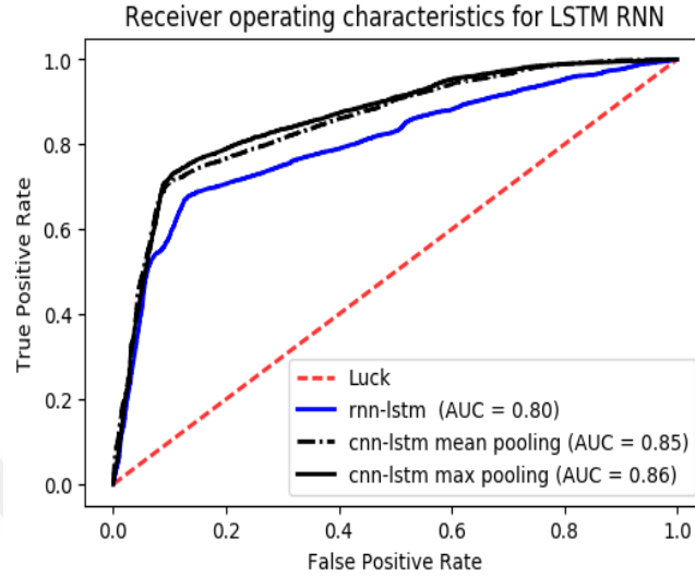
Figure 3.4: Receiver operating characteristics (ROC) for intrusion detection using CNN and RNNs-LSTM
