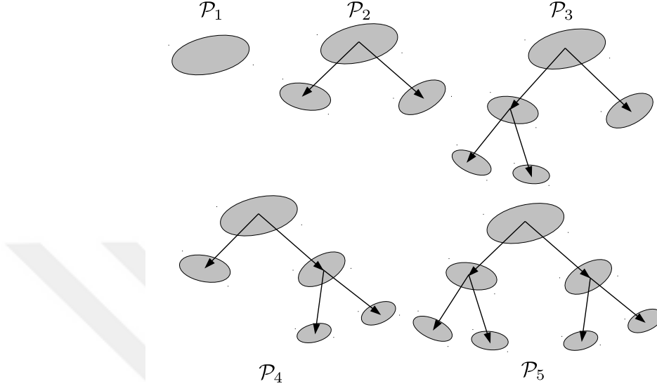
Figure 2.3: A doubly exponential number of partitions defining the piecewise models on time varying submanifold, each leaf node represents a subset defined by (2.2)
