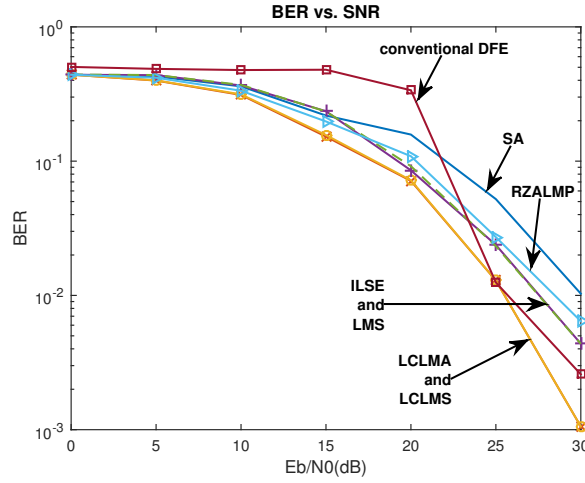
Figure 6.4: BER analysis of the first order methods, in a channel with 5% impulsive noise.
