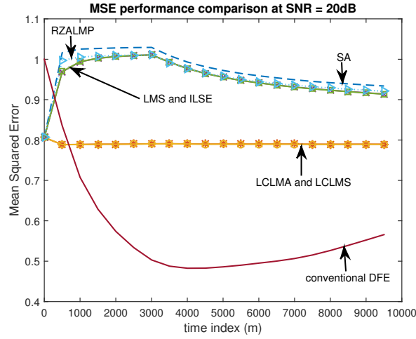
Figure 6.8: MSE analysis of different first order methods.
