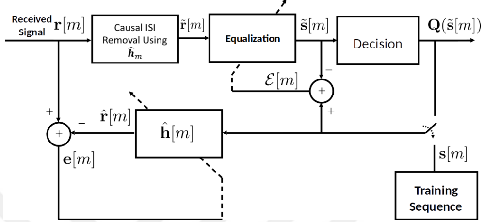
Figure 6.2: A detailed diagram for channel equalization and estimation block of Fig. 6.1. We introduce algorithms for channel estimation to determine how \hat{\mathbf{h}}[m] should be updated based on the error e[m] , for the specific case of channels suffered from the impulsive noise.
