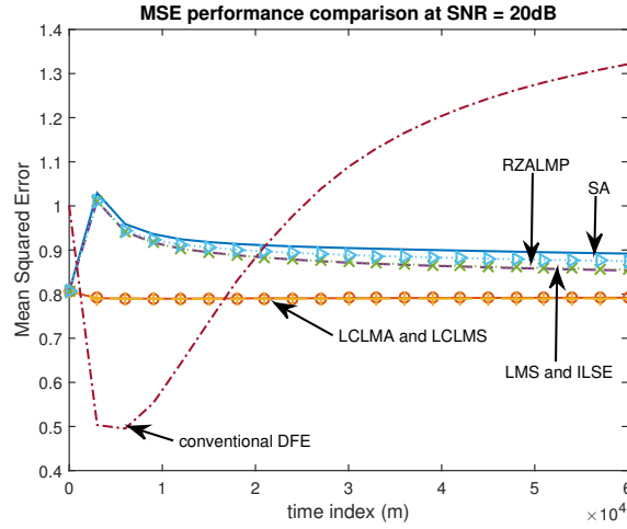
Figure 6.6: MSE analysis in a 20 dB SNR and 5% impulsive noise channel. The proposed first order methods, LCLMS and LCLMA outperform the conventional algorithms in terms of convergence rate
