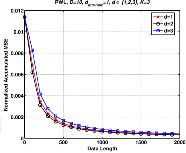
Figure 2.7: Sequential piecewise linear prediction of the desired data \hat{y}[n] of (2.26) with d = 1, 2, 3 and tree depth, K = 3 . The intrinsic dimension is d_{\text{intrinsic}} = 1
