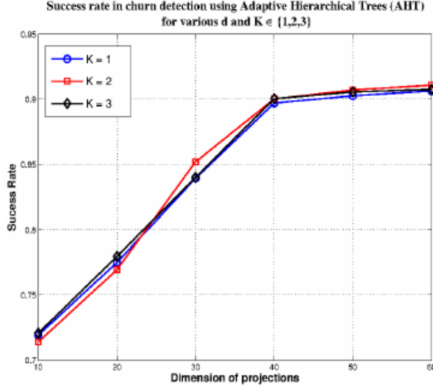
Figure 4.2: Success rate in Churn detection using Adaptive hierarchical Trees algorithm for logistic regression with various choices of d and K
