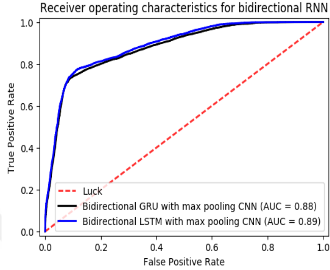
Figure 3.7: Receiver operating characteristics (ROC) for comparison of bidirectional RNNs with LSTM and GRU
