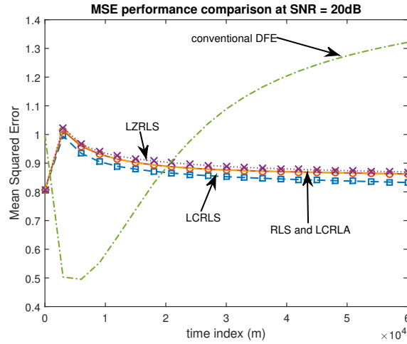
Figure 6.7: MSE analysis in a 20 dB SNR and 5% impulsive noise channel. The proposed second order method, LCRLS outperforms the conventional algorithms in terms of convergence rate
