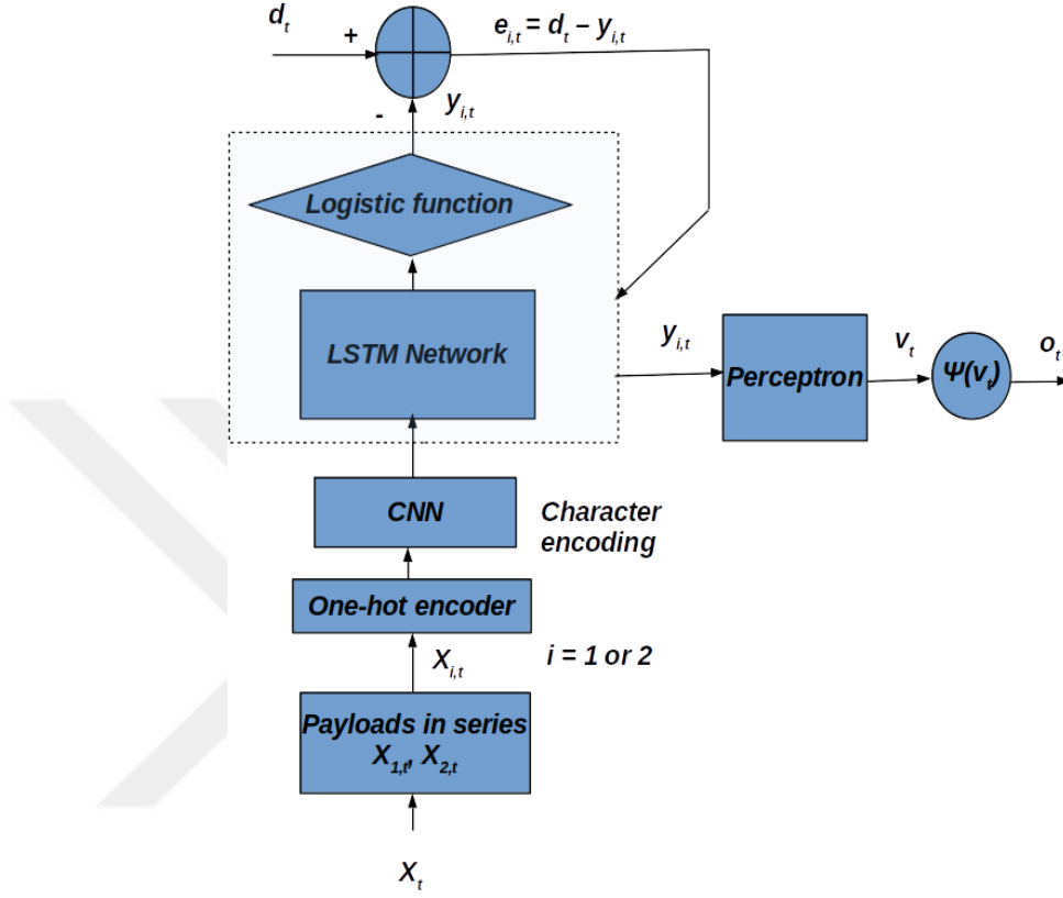
Figure 3.3: The proposed IDS model
