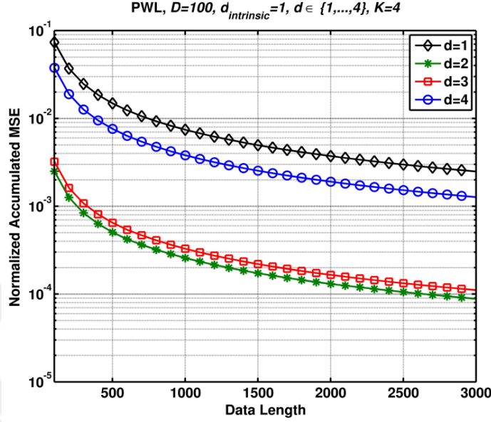
Figure 2.8: Piecewise linear regression on 100– dimensional time varying submanifold with intrinsic dimension d_{\text{intrinsic}} = 1 using adaptive Hierarchical trees. Normalized MSE are plotted for 3000 samples of online data using K = 4 and d = 1, \dots, 4
