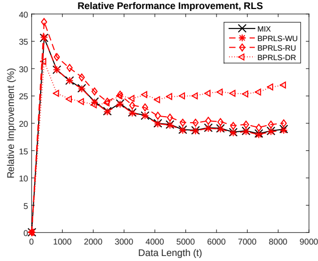
Figure 5.13: The performance of RLS-based boosting methods on the CompAct data set.
