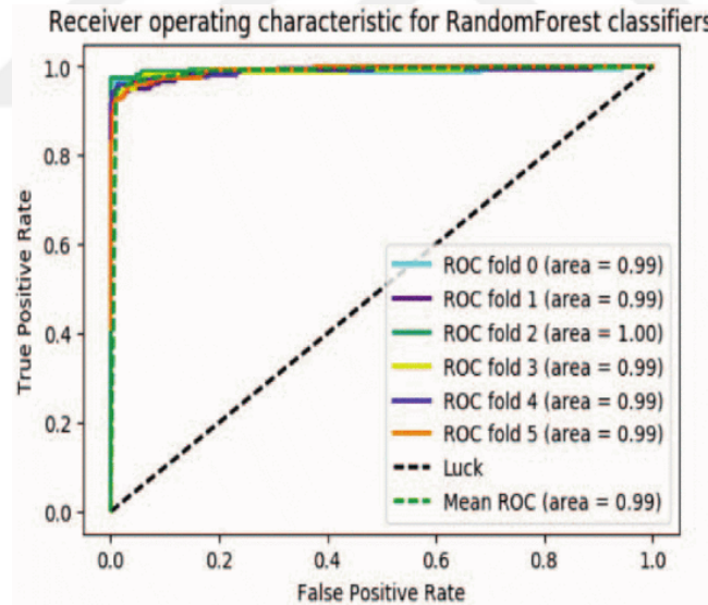
Figure 4.4: Receiver operating characteristics (ROC) for random forest classifiers with 5– fold cross-validation
