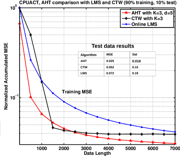
Figure 2.10: Performance Analysis of AHT on real data (Computer Activity) with d = 5 , D = 21 and K = 3 . 90% of the data is used for training and the remaining data is used as the test data.
