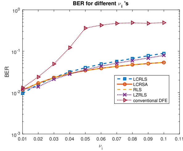
Figure 6.11: BER versus the probabilities of impulsive noise at 20 dB SNR, for the second order algorithms.
