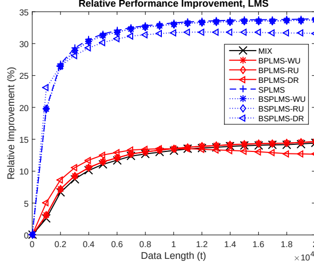
Figure 5.6: The relative improvement in ASE performance of the RLS-based algorithms in the stationary data experiment.
