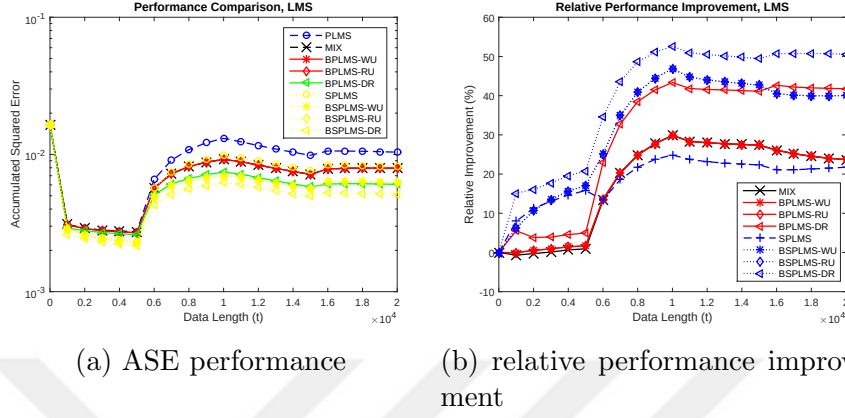
Figure 5.7: The performance results of the boosting approaches in the non-stationary experiment.
