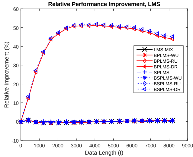
Figure 5.14: The performance of LMS-based boosting methods on the Bank data set.
