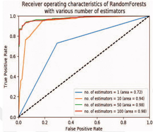
Figure 4.3: Receiver operating characteristics (ROC) for random forest classifiers
