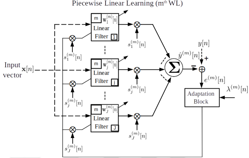
Figure 5.4: A sample piecewise linear adaptive filter, used as the m^{th} constituent WL in the system depicted in Fig. 5.2. This WL consists of J linear filters, one of which produces the estimate at each iteration n . Based on where the input vector at time n , \mathbf{x}[n] , lies in the input vector space, one of the s_j^{(m)}[n] 's is 1 and all others are 0. Hence, at each iteration only one of the linear filters is used for estimation and updated correspondingly.
