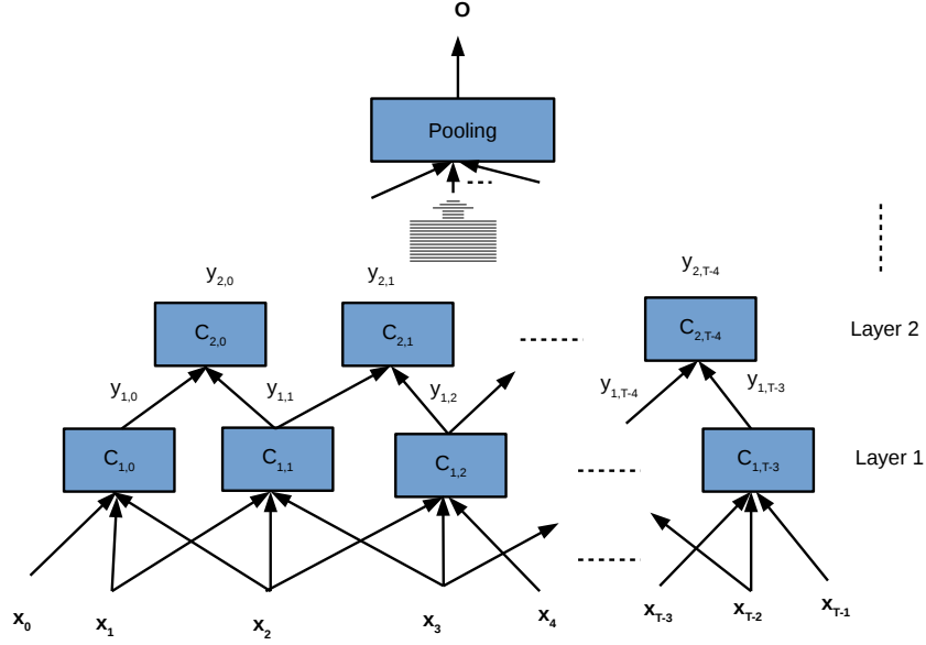
Figure 3.2: Multi-layer convolution neural network
