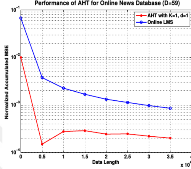
Figure 2.11: Performance Analysis of AHT on real data (Online News Popularity) with d = 1, D = 59 and K = 1 .
