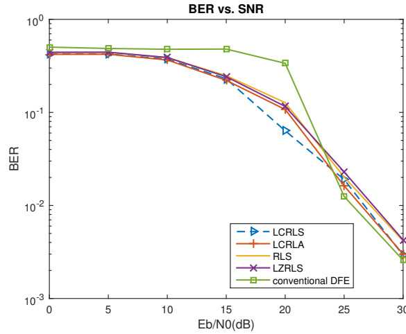
Figure 6.5: BER analysis of the second order methods, in a channel with 5% impulsive noise.
