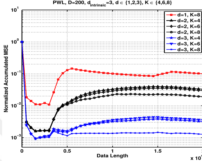
Figure 2.9: Normalized MSE based performance analysis using AHT with K \in \{4, 6, 8\} and d = \{1, 2, 3\} , to see the effect of these parameters on the time-varying submanifold tracking performance.
