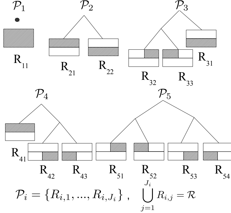
Figure 2.1: A full tree of depth 2 that represents all possible partitions of the two dimensional space, \mathcal{P} = \{\mathcal{P}_1, \dots, \mathcal{P}_{N_K}\} and N_K \approx (1.5)^{2^K} , where K is the depth of the tree. Here N_K = 5 .
