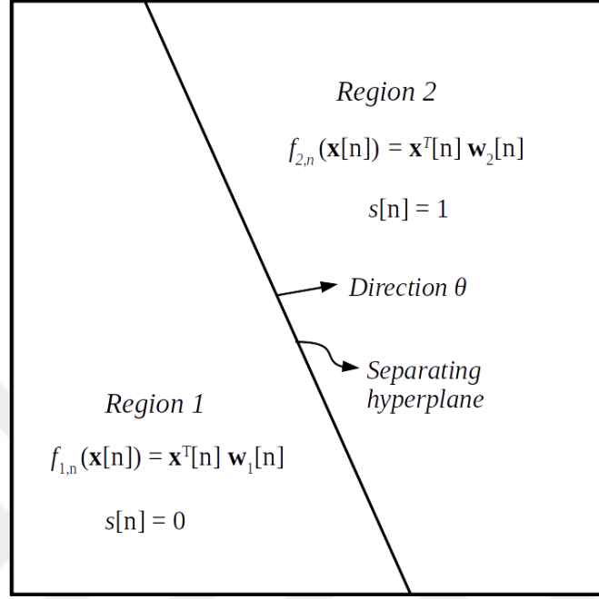
Figure 5.1: A 2-region partitioning of the input vector (i.e., \mathbf{x}[n] \in \mathbb{R}^2 ) space. The indicator function s[n] determines the region to which \mathbf{x}[n] belongs, i.e., s[n] = 0 represents that \mathbf{x}[n] is in Region 1 and s[n] = 1 represents that \mathbf{x}[n] is in Region 2
