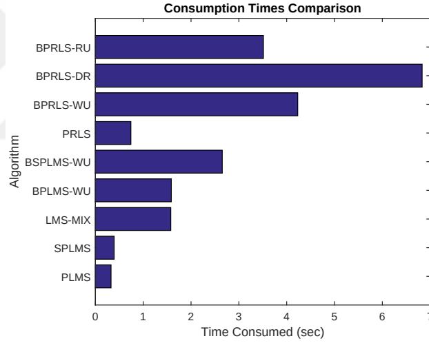
Figure 5.8: The time consumed by each algorithm in the non-stationary data experiment.
