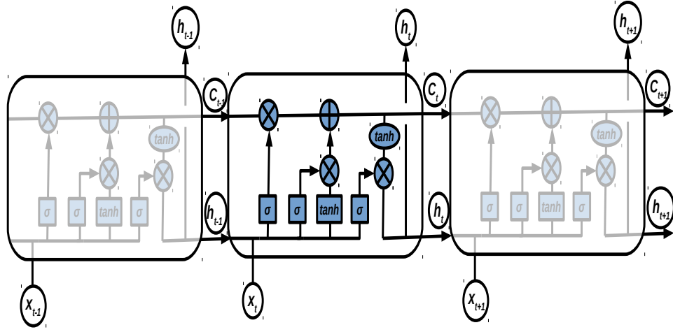
Figure 3.1: Long Short Term Memory Units (LSTM)
