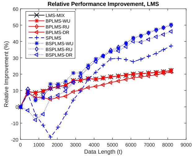
Figure 5.12: The performance of LMS-based boosting methods on the CompAct data set.
