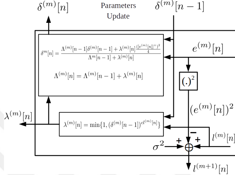
Figure 5.3: Parameters update block of the m th constituent WL, which is embedded in the m th WL block as depicted in Fig. 5.2. This block receives the parameter l^{(m)}[n] provided by the (m-1) th WL, and uses that in computing \lambda^{(m)}[n] . It also computes l^{(m+1)}[n] and passes it to the (m+1)^{th} WL. The parameter [e^{(m)}[n]]^+ represents the error of the thresholded estimate as explained in (5.9), and \Lambda^{(m)}[n] shows the sum of the weights \lambda^{(m)}[1], \dots, \lambda^{(m)}[n] . The WMSE parameter \delta^{(m)}[n-1] represents the time averaged weighted square error made by the m^{th} WL up to time n-1 .
