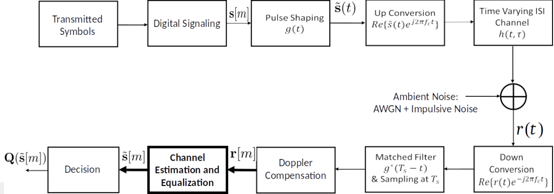
Figure 6.1: The block diagram shows the flow of transmitted and received signals through a time varying intersymbol interference (ISI) channel that is affected by AWGN and impulsive noise n(t) . The transmitted data \{s[m]\}_{m \geq 1} are modulated, "pulse shaped" with a raised cosine filter g(t) and up-converted to the carrier frequency f_c . The channels equalizer receives r[m] and generates the soft output \tilde{s}[m] . \mathbf{Q}(\tilde{s}[m]) is the hard estimation for the m^{th} transmitted symbol. We use the channel estimation to adapt the equalizer for reduction of ISI.
