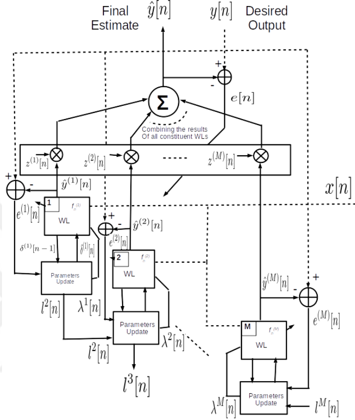
Figure 5.2: The block diagram of online boosting algorithm that combines M WLs. Each WL is a piecewise linear model that produces an estimate of the output y[n] for the input vector \mathbf{x}[n] . The final estimate \hat{y}[n] is generated by linear combinations of the constituent WLs. With each iteration, the parameters of WLs as well as the combination weights are updated based on \lambda^{(m)}[n] and e^{(m)}[n]
