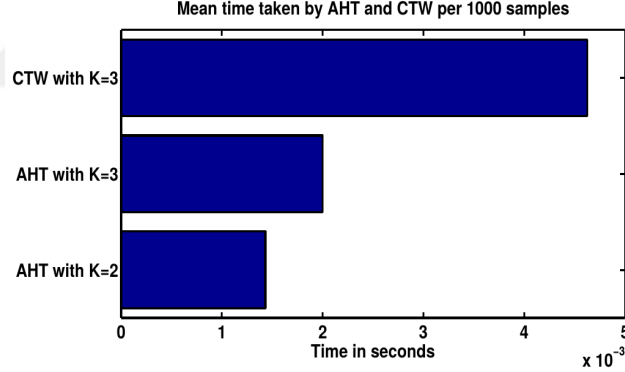
Figure 2.13: The comparison between the time consumption of different algorithms in the KDD CUP99 experiment.
