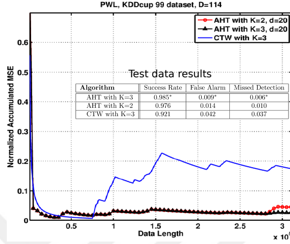
Figure 2.12: Performance Analysis of AHT on real data (KDD CUP99 Database) with d = 20 , D = 114 and K \in \{2, 3\} . 90% of the data is used for training and the remaining data is used for the test.
