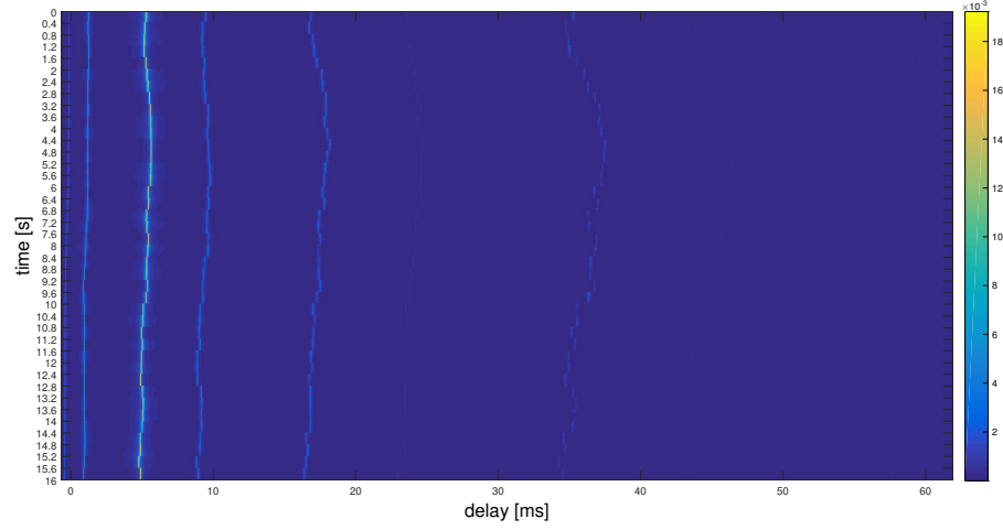
Figure 6.3: Time evolution of the magnitude baseband impulse response of the generated channel [195]
