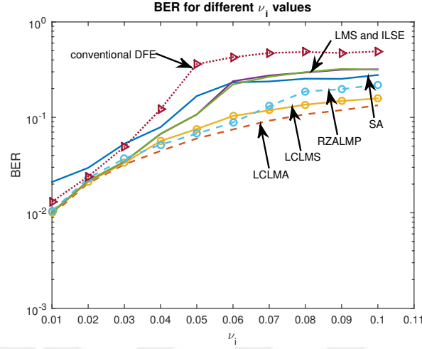
Figure 6.10: BER versus the probabilities of impulsive noise at 20 dB SNR, for the first order algorithms.
