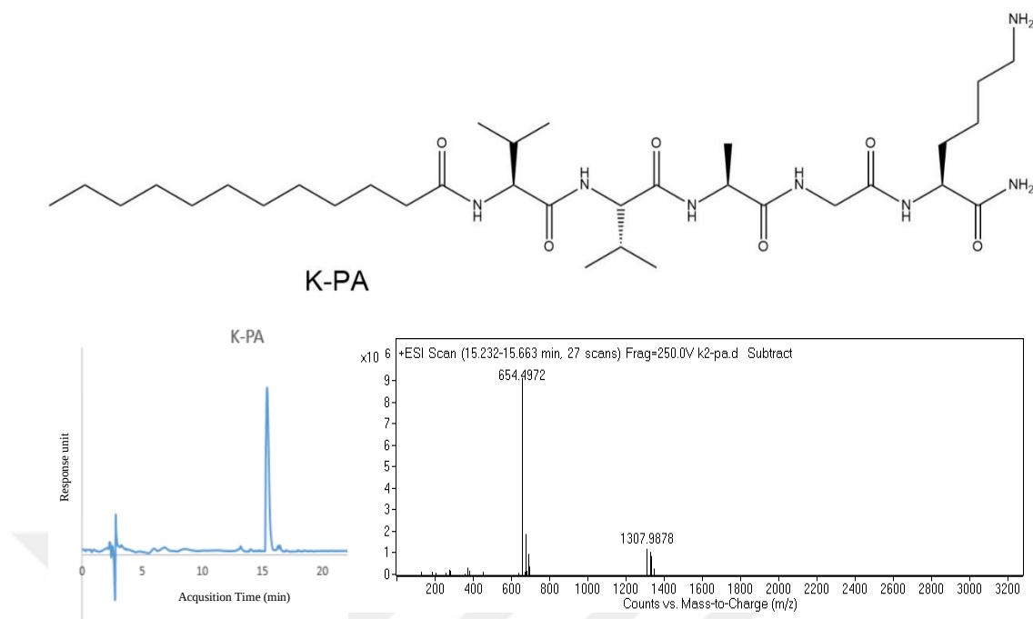
Figure 9: Chemical structure and LC-MS analyses of K-PA.
