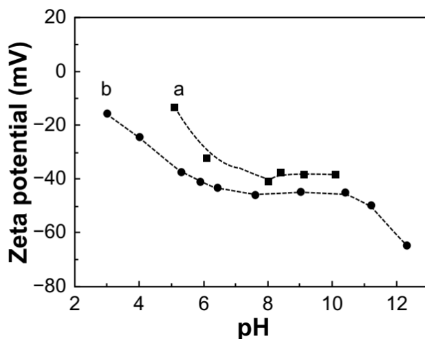
Figure 0-3 Zeta potential of silica nanoparticles in different pHs [14]
