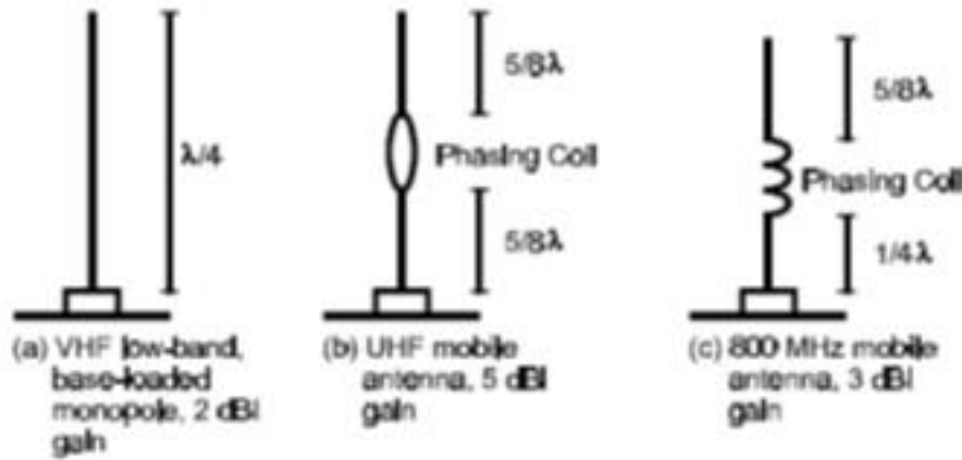
Figure 2.14: Examples of Antennas.
