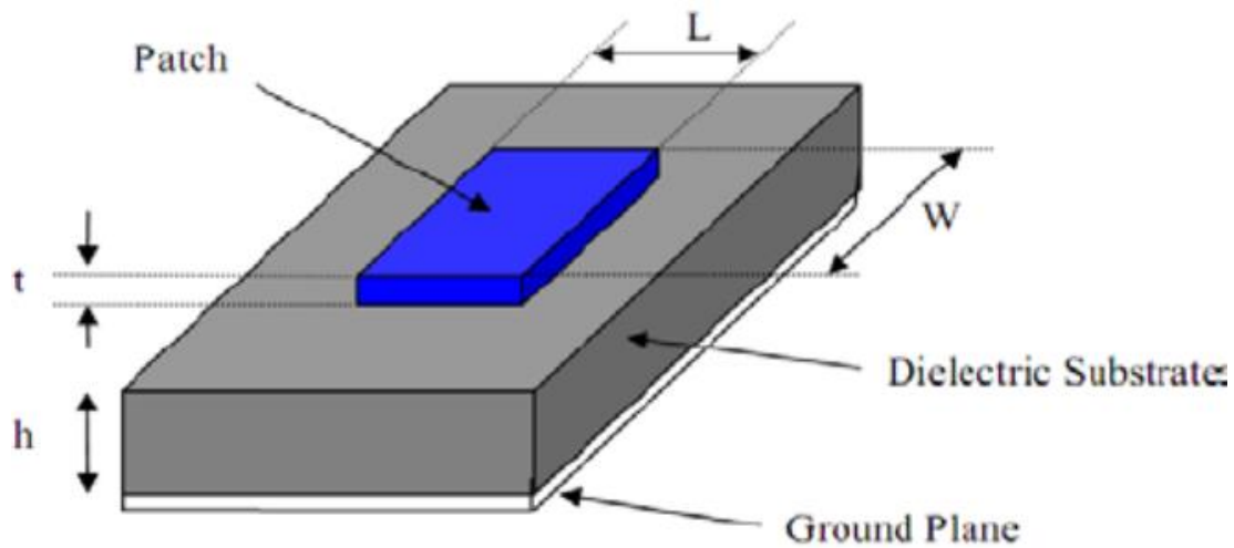
Figure 2.7: Dimensions of Patch Antenna.
