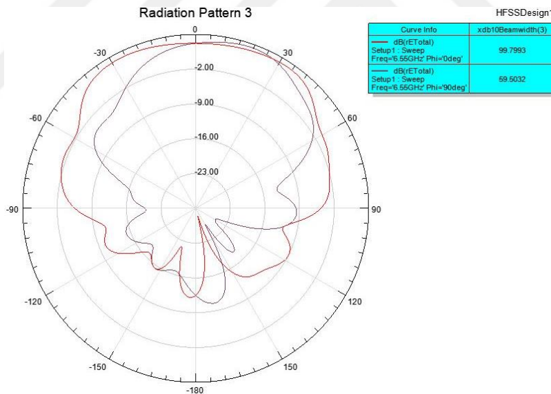
C. 3rd Frequency (6.55GHz)
