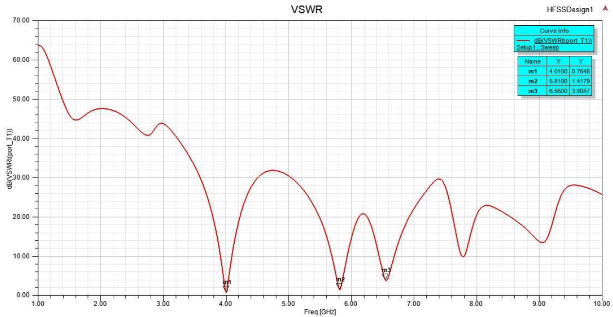
Figure 4.3: VSWR Graph of Microstrip Patch Antenna Design.
