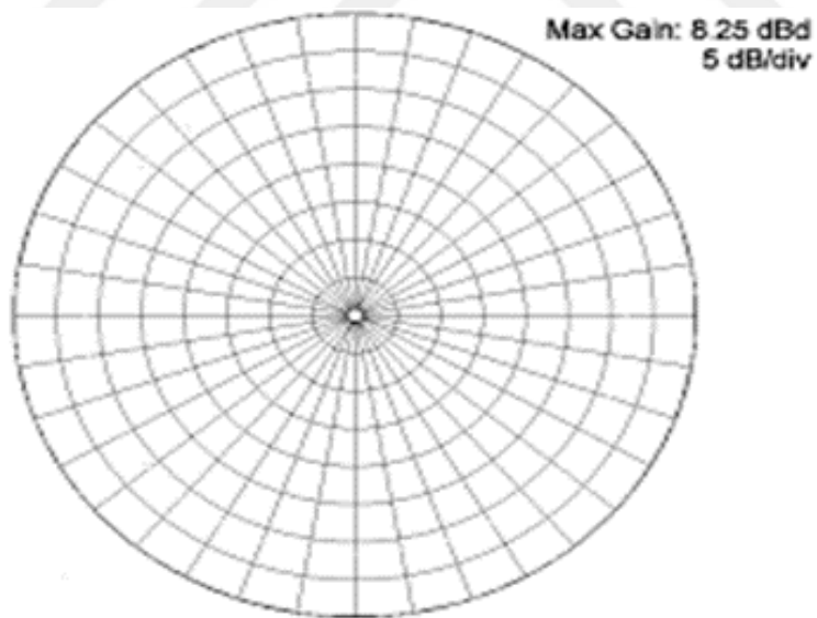
Figure 2.12: Omnidirectional pattern.
