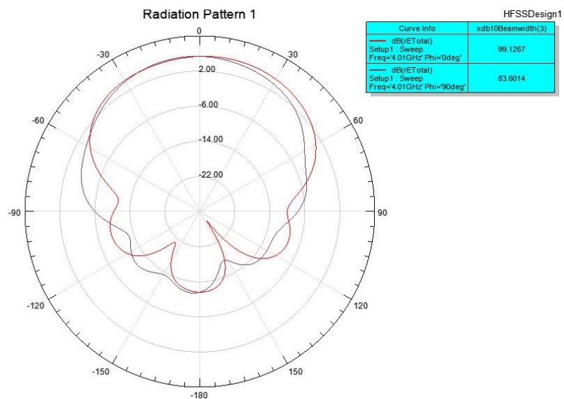
A. 1st Frequency (4.01GHz).
