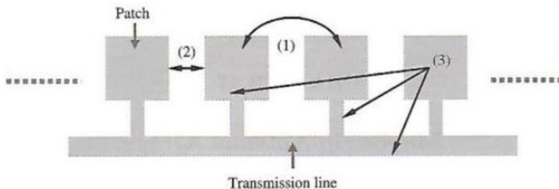
Figure 2.9: Mutual Coupling Visualization in an Antenna Array.
