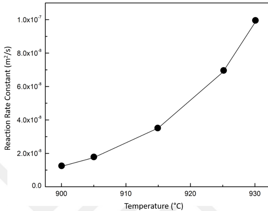
Figure 4.39 Reaction rate constant versus temperature diagram.
