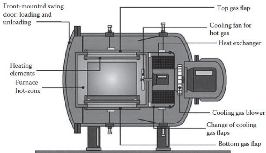
Figure 2.10 Schematic of the vacuum-brazing furnace.
