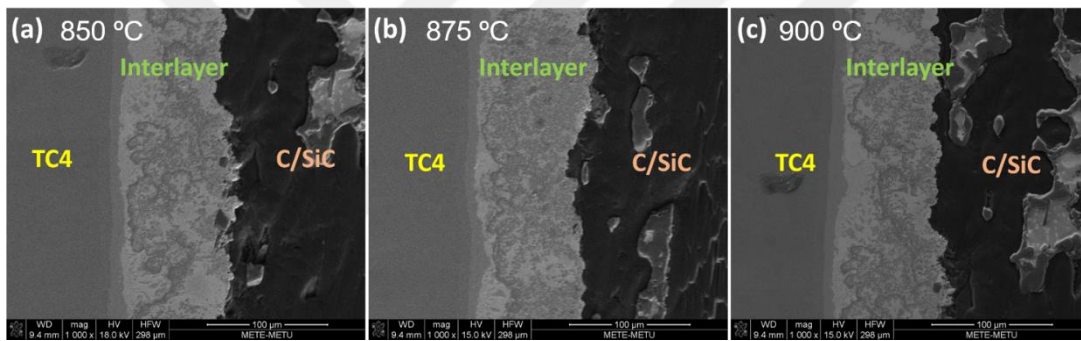
Figure 4.5 SEM micrographs of the interface between C/SiC composite and Ti6Al4V alloy joints brazed at a) 850 °C, b) 875 °C, and c) 900 °C
