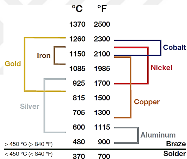
Figure 2.11 Brazing temperature ranges for different materials.
