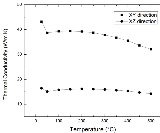
Figure 4.62 Thermal conductivity values of the 3D C/SiC composites.
