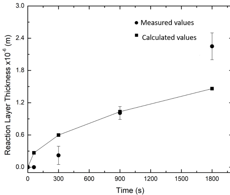
Figure 4.38 The comparison of the theoretical and experimental data of the reaction layer thickness obtained at a constant temperature of 915 °C.
