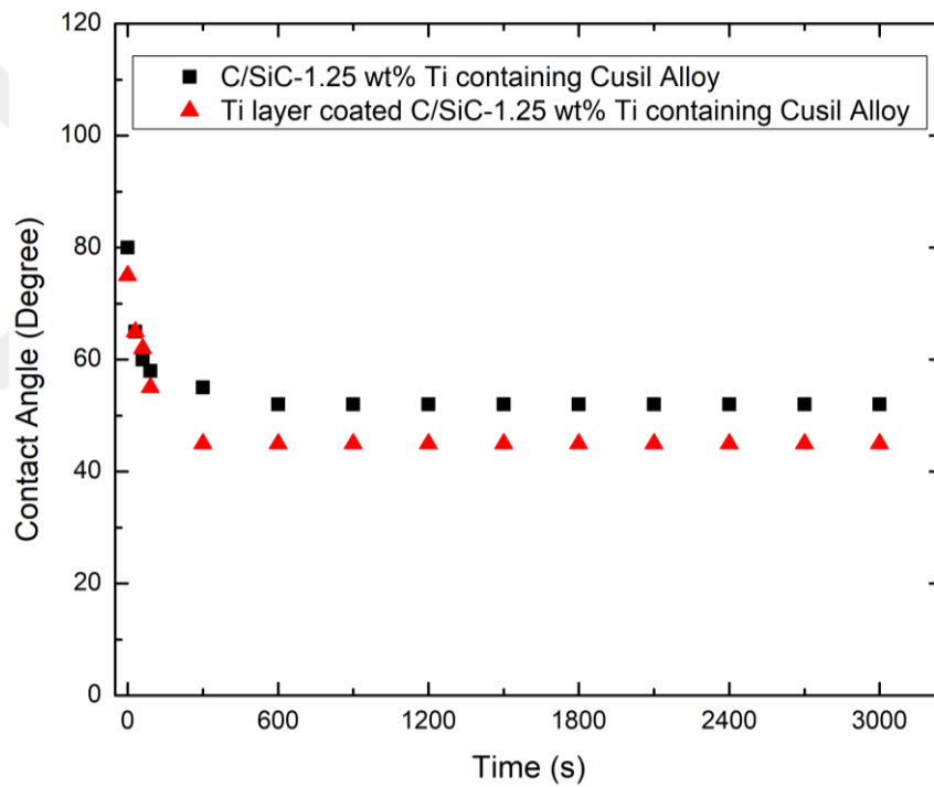
Figure 4.23 Effect of Ti layer coating on the ceramic composite surface and addition of Ti element to the brazing filler alloy on the contact angle variation of Cusil with respect to time at 780 °C.
