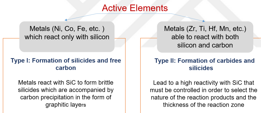
Figure 2.22 Classification of active elements for brazing.
