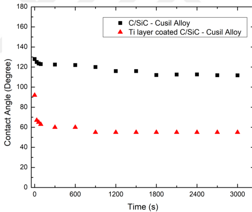
Figure 4.19 Effect of Ti layer coating on the contact angle variation of Cusil brazing filler alloy with respect to time at 780 °C.
