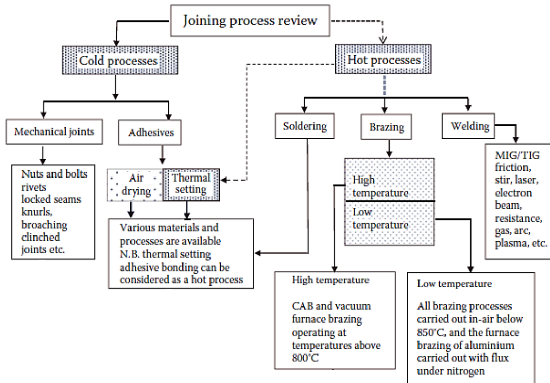
Figure 2.7 A list of the various joining techniques [37].
