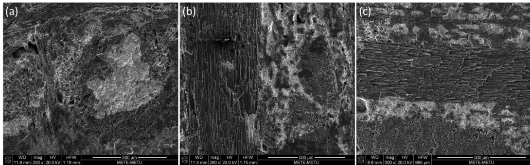
Figure 4.1 Microstructures of Ag-Cu brazing filler alloy over the C/SiC composite surface with brazing temperatures of a) 850, b) 875 and c) 900 °C.
