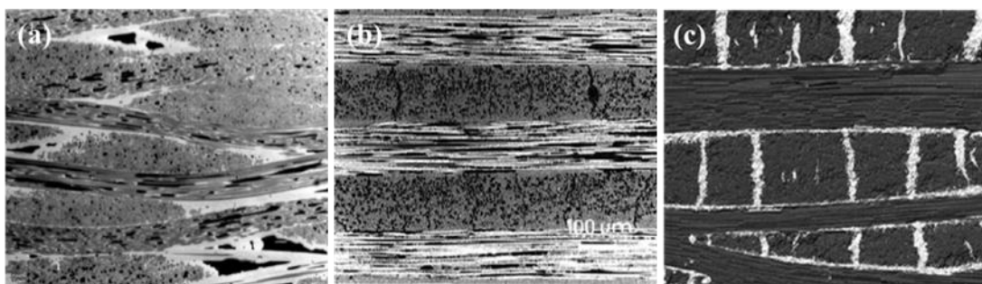
Figure 2.3 Microstructures of C/SiC composites depending on manufacturing methods a) Chemical vapor infiltration (CVI), b) Polymer infiltration and pyrolysis (PIP) and c) Liquid silicon infiltration (LSI) [13].
