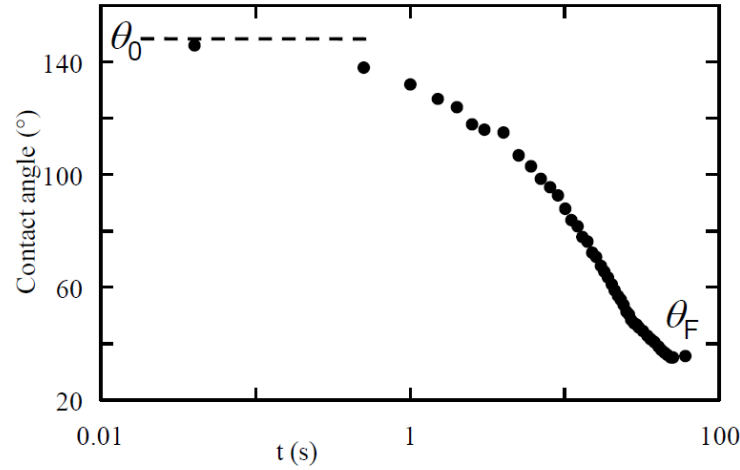
Figure 2.17 Contact angle versus time diagram of silicon on carbon [49].
