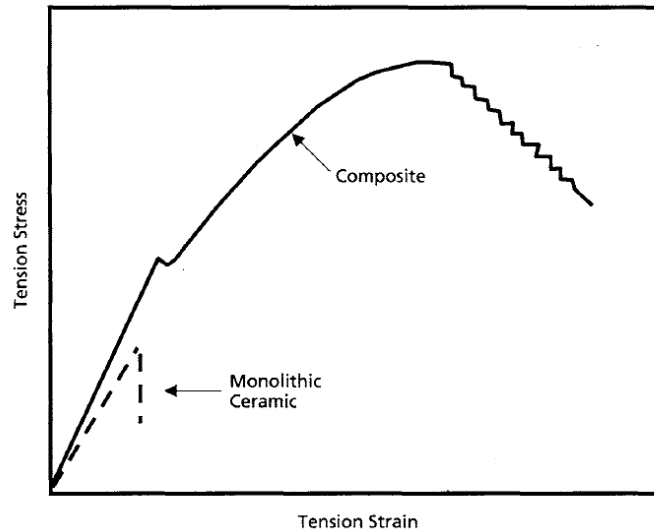
Figure 2.1 Stress-strain behavior comparison for ceramics and ceramic matrix composites [3].
