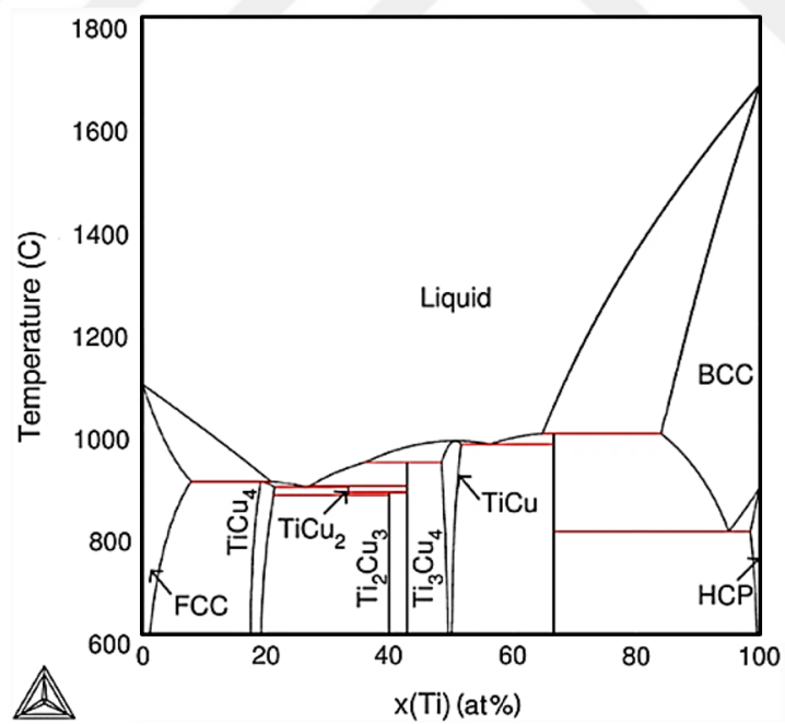
Figure 2.24 Cu-Ti Phase diagram [60].
