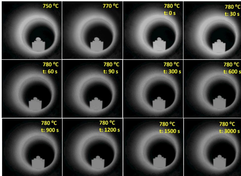
Figure 4.16 Morphological changes of Cusil brazing filler alloy on C/SiC composite surface under different temperature and time conditions.
