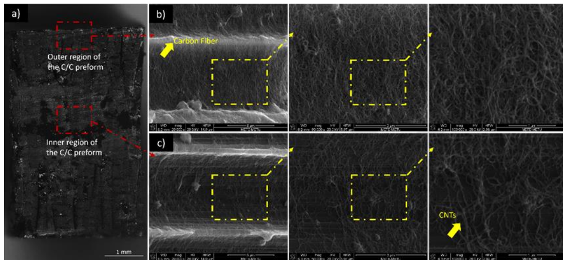
Figure 4.57 (a) View of the entire C/C preform in cross-section, with the CNTs distributed in a gradient manner (b) the outer part of the C/C preform and (c) the inner part of the C/C preform.
