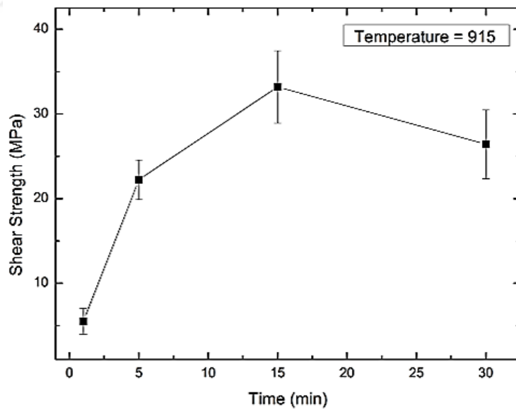
Figure 4.41 Shear test results of the brazed joints with respect to brazing time at constant brazing temperature.
