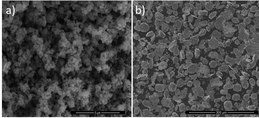
Figure 3.5 Additive materials used in the study a) nano-SiC powders, b) SiC micro-powders.
