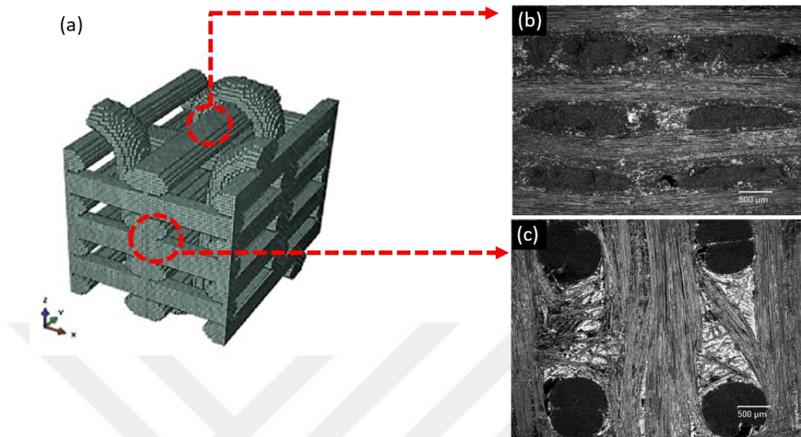
Figure 4.71 (a) Sketch of reinforcement architecture in 3D C/SiC composite (b) Micrograph of XY plane, (c) Micrograph of XZ plane.
