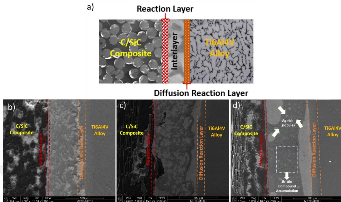
Figure 4.30 a) The schematic drawing of the C/SiC composite-Ti6Al4V alloy brazed joint. The microstructure of the interface between C/SiC composite and Ti6Al4V alloy joints brazed by Ticusil brazing filler alloy at b) 900 °C, c) 915 °C, and d) 930 °C.
