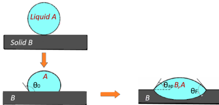
Figure 2.18 Schematic of dissolution wetting.
