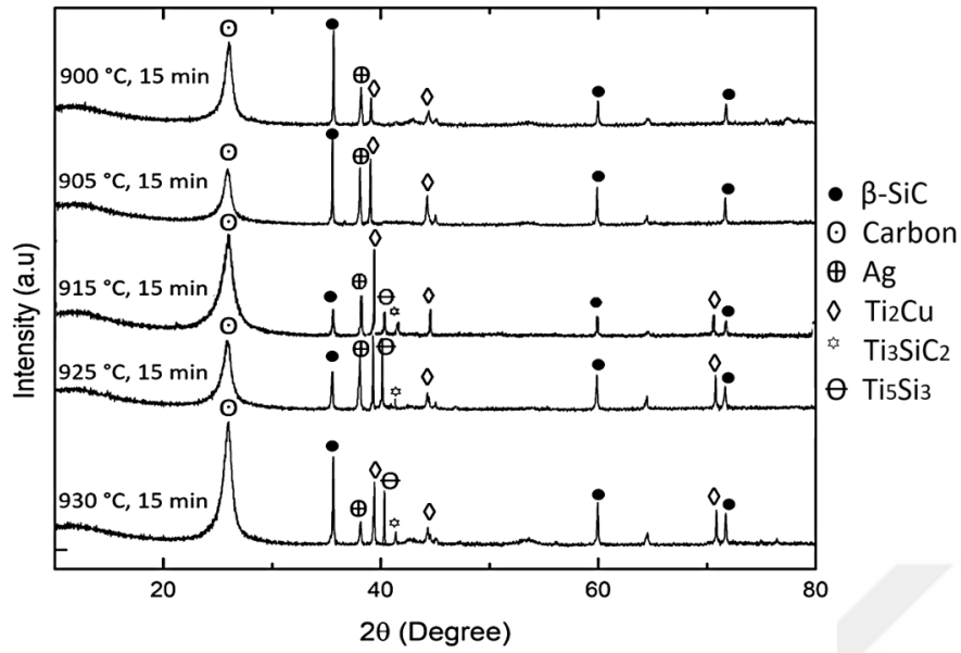
Figure 4.35 XRD results of the C/SiC composite/Ticusil interlayer interfaces with respect to varying brazing temperatures at constant brazing time of 15 min.
