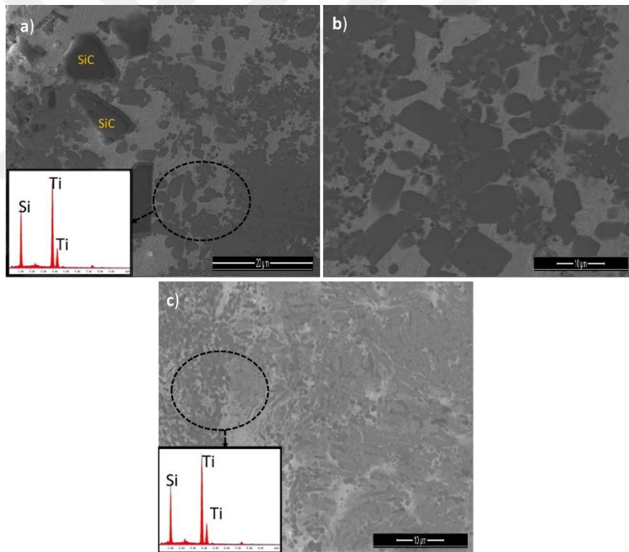
Figure 4.46 The microstructure of the interlayer between C/SiC composite and Ti6Al4V alloy joints brazed by Ticusil brazing filler alloy containing a) and b) 1 wt% micron level, c) 2 wt% nano level.
