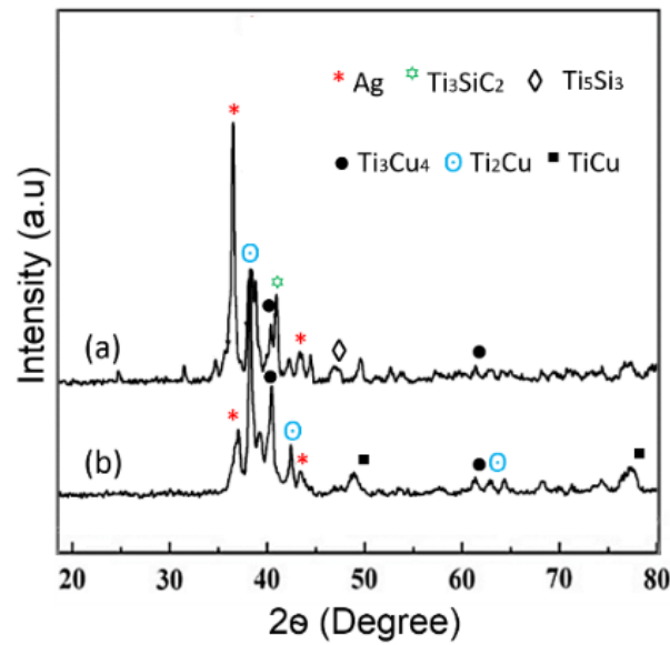
Figure 4.12 XRD analysis of (a) interface between Ti layer coated C/SiC composite and interlayer, (b) interface between Ti6Al4V alloy and interlayer.
