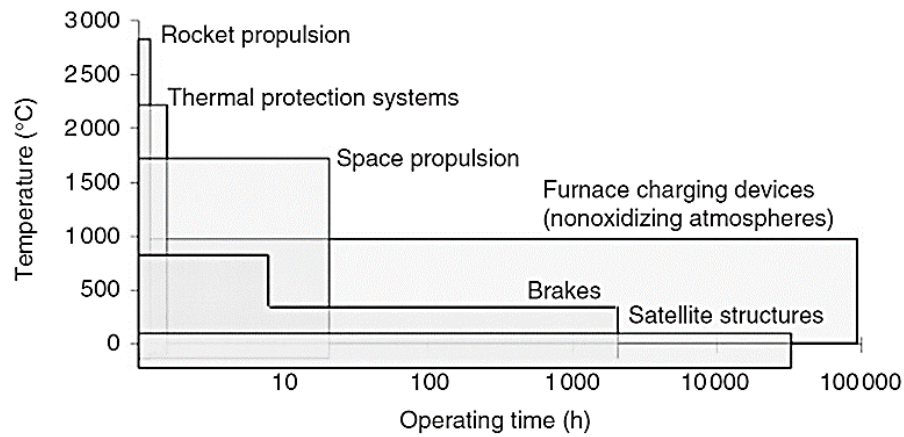
Figure 2.2 Service temperature and time-dependent application areas of C/SiC [10].
