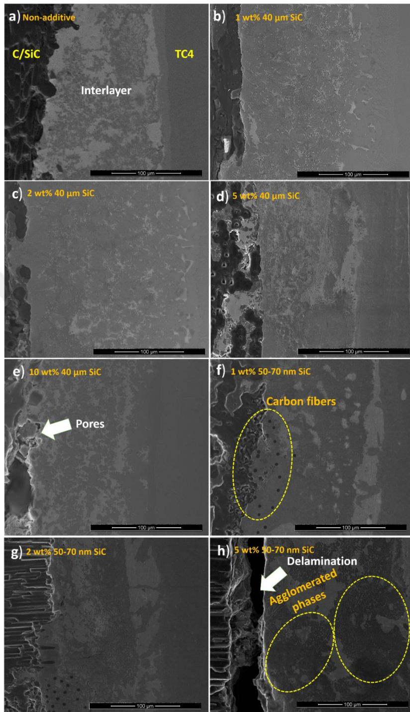
Figure 4.45 The microstructure of the interface between C/SiC composite and Ti6Al4V alloy joints brazed by Ticusil brazing filler alloy containing a) non-additive, b) 1 wt% micron level, c) 2 wt% micron level, d) 5 wt% micron level, e) 10 wt% micron level, f) 1 wt% nano level, g) 2 wt% nano level and h) 5 wt% nano level.
