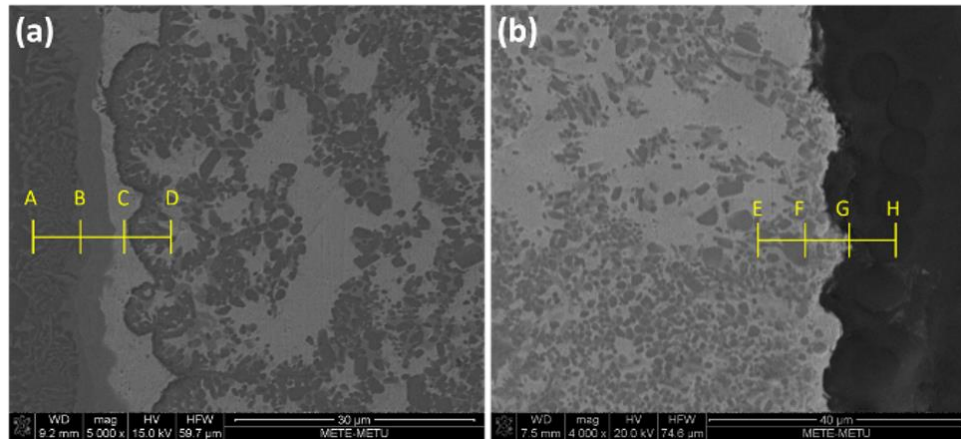
Figure 4.6. SEM micrographs of C/SiC Composite/Cusil-ABA/Ti6Al4V Alloy brazed at 875 °C, for 10 min a) the interface between Ti6Al4V alloy and the interlayer, b) the interface between C/SiC composite and the interlayer.
