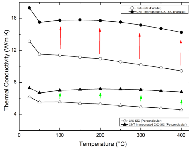
Figure 4.60 Thermal conductivity values of the C/C-SiC composites with and without CNT impregnation.
