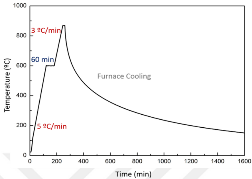
Figure 3.3 The temperature profile for brazing experiments.
