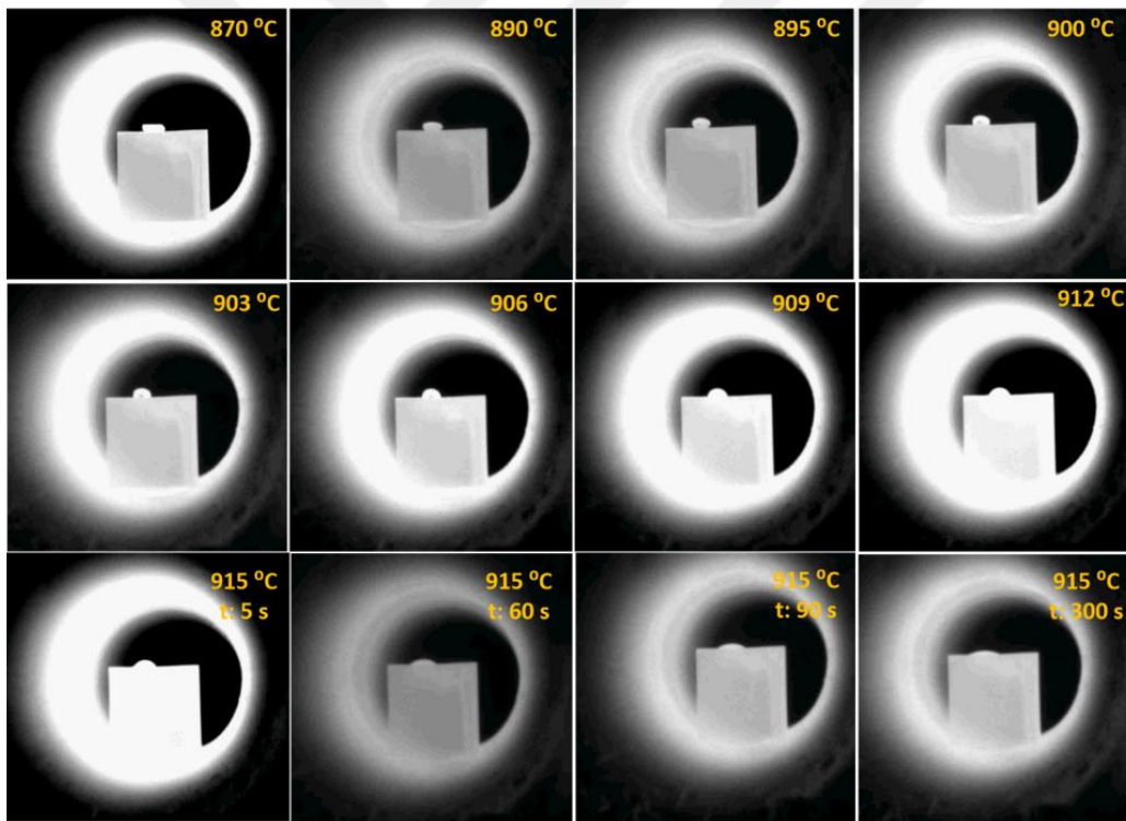
Figure 4.24 Morphological changes of Ticusil brazing filler alloy on monolithic SiC ceramic surface under different temperature and time conditions.
