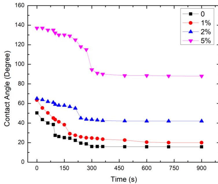
Figure 4.50 Change in measured contact angle as a function of time at 915 °C for brazing filler alloy with different nano level SiC additive amounts.
