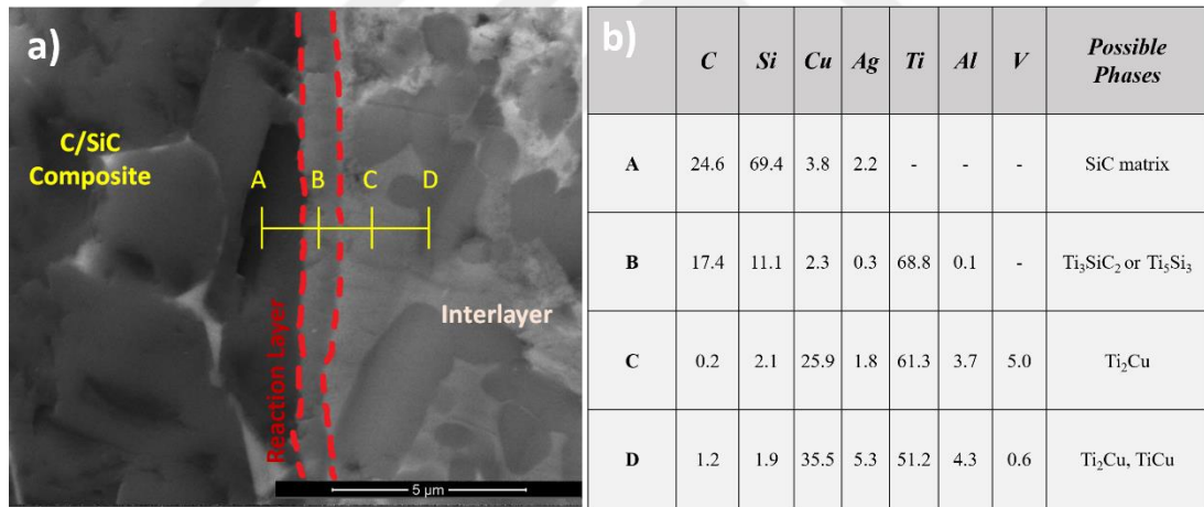
Figure 4.34 Elemental distribution along the C/SiC composite/Ticusil interlayer interface according to a) SEM micrograph, b) EDS line analysis presenting average chemical composition.
