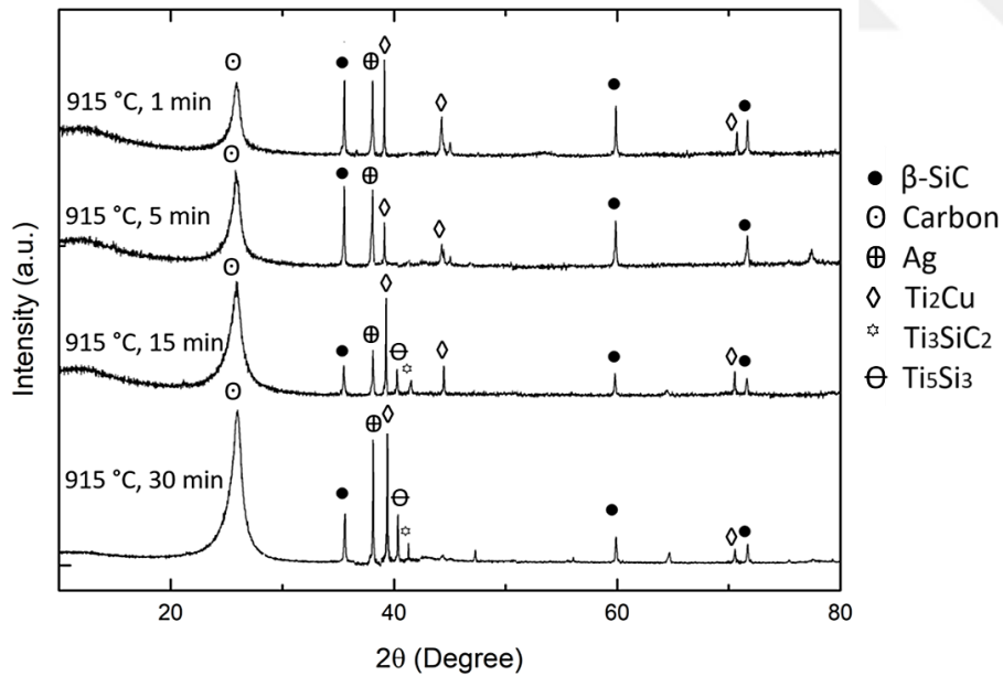
Figure 4.36 XRD results of the C/SiC composite/Ticusil interlayer interfaces with respect to varying brazing time at constant brazing temperature of 915 °C.
