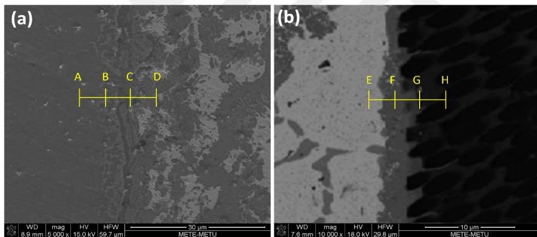
Figure 4.11 SEM micrographs of the interfaces between a) Ti6Al4V alloy and filler alloy and b) Ti layer coated C/SiC composite and filler alloy brazed by Cusil ABA at 875 °C for 10 min.
