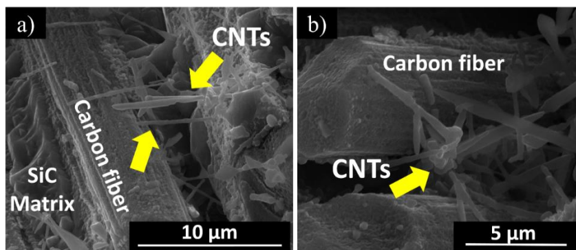
Figure 4.58 SEM microstructures of the CNT impregnated C/C-SiC composites.
