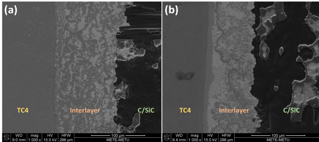
Figure 4.10 Microstructure of interface between C/SiC composite and Ti6Al4V alloy joints of (a) without Ti coating and (b) with Ti coating.
