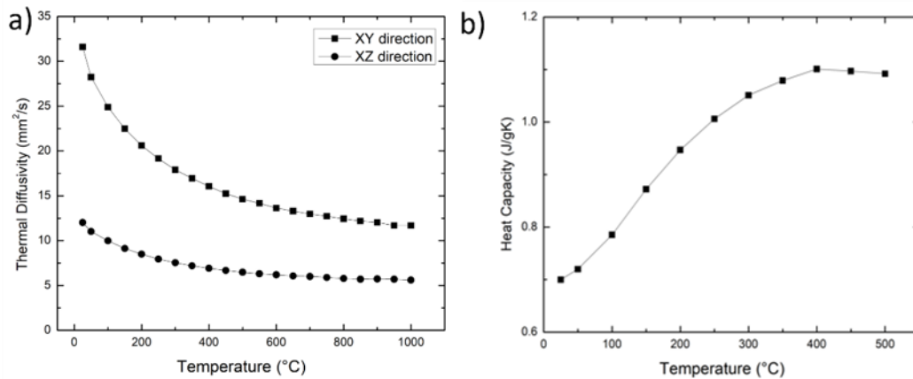
Figure 4.61 a) Thermal diffusivity and b) heat capacity values of the 3D C/SiC composite.
