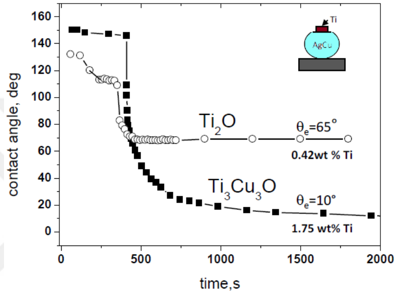
Figure 2.19 Ti concentration effect on the wetting behavior of Copper-Silver alloy on the alumina surface [53].
