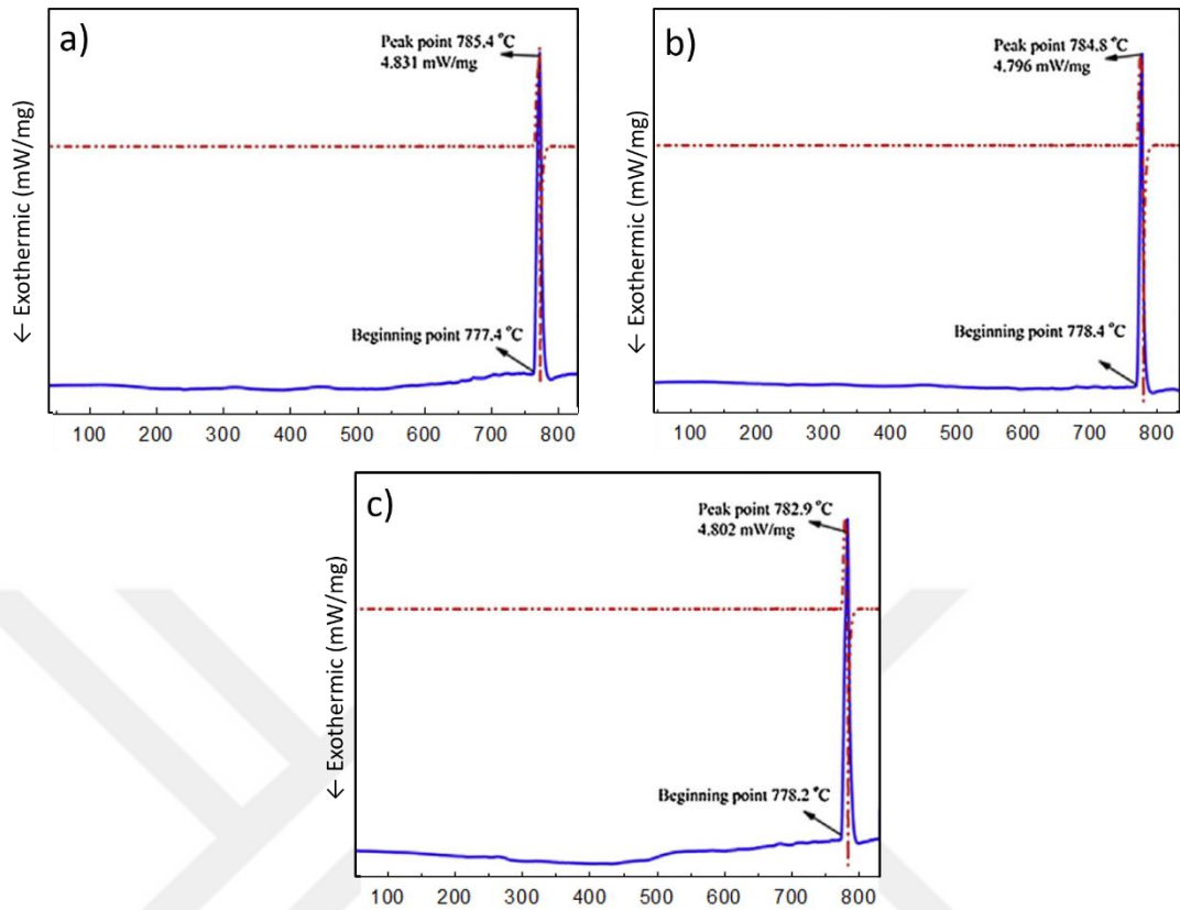
Figure 4.54 DSC curves for Ticusil brazing filler alloy containing a) non-additive b) 1 wt% micron level SiC and c) 2 wt% nano level SiC.
