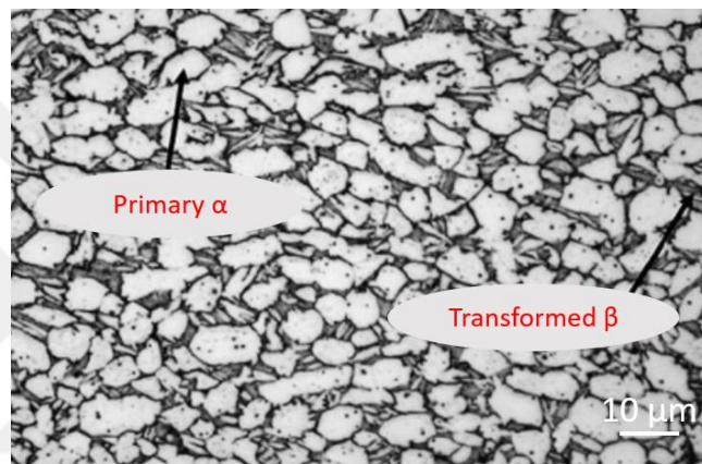
Figure 2.6 Microstructure of the Ti6Al4V alloy [30].
