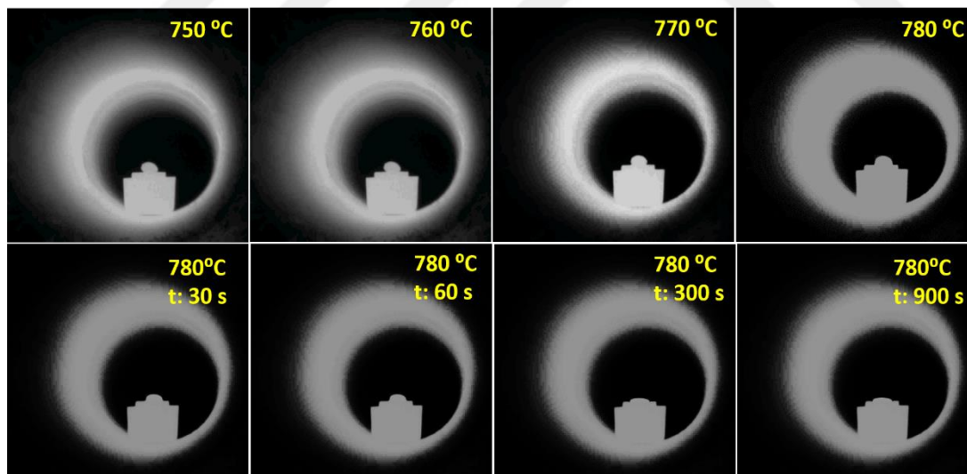
Figure 4.22 Morphological changes of 1.25 wt% Ti powder containing Cusil brazing filler alloy on the Ti layer coated C/SiC composite surface under different temperature and time conditions.
