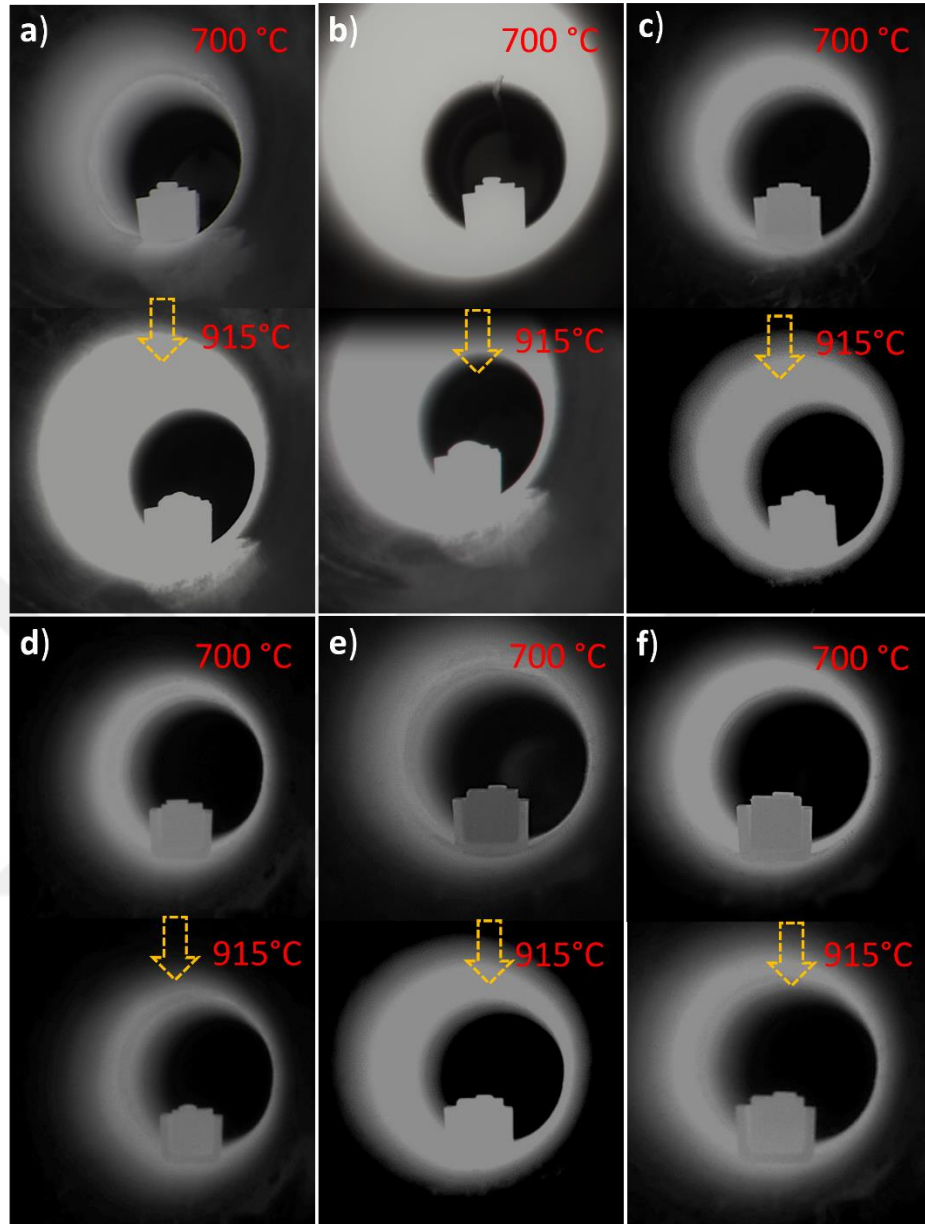
Figure 4.47 Morphological changes of brazing filler alloy on C/SiC composite surface containing different amounts of micron level SiC additive a) non-additive brazing filler alloy, b) 1 wt% micron level SiC, c) 2 wt% micron level SiC, d) 5 wt% micron level SiC, e) 10 wt% micron level SiC, f) 20 wt% micron level SiC.
