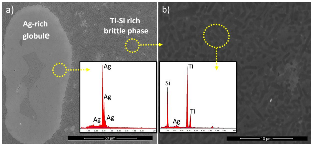
Figure 4.32 C/SiC composite/Ticusil interlayer at 930 °C for 15 min a) Ag-rich globules, b) Ti-Si rich brittle phases.
