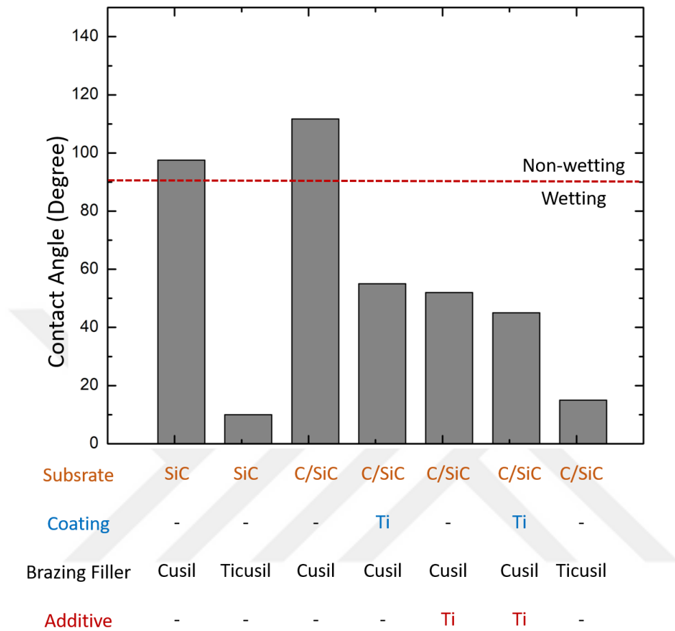
Figure 4.29 The effect of the presence of active Ti element in the coating layer and/or in the brazing filler material on the contact angle.
