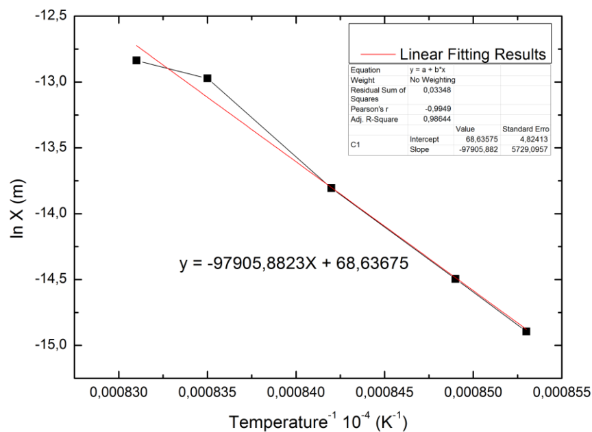
Figure 4.37 Linear fitting results for brazing time of 15 min.
