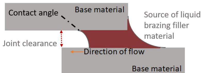
Figure 2.8 Schematic illustration of brazed joint.
