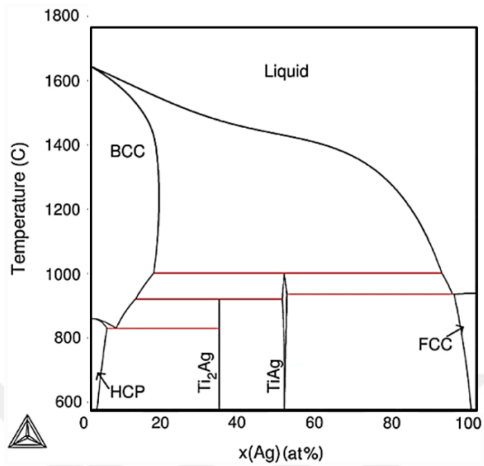
Figure 2.23 Ag-Ti Phase diagram [75,76].
