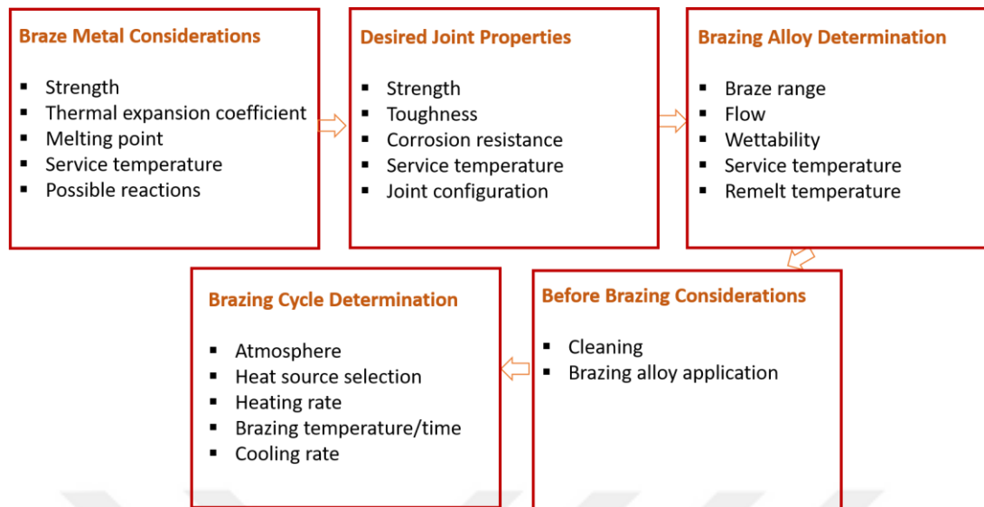
Figure 2.9 Critical steps for brazing process.
