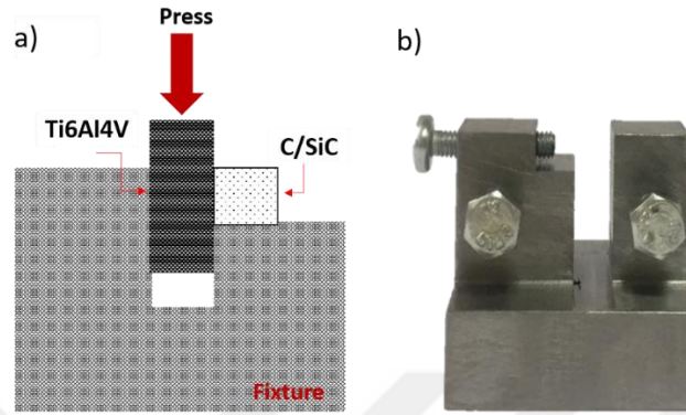
Figure 3.9 a) The schematics of the lap-shear test of the brazed joints and b) In-house designed fixture for the lap-shear test.
