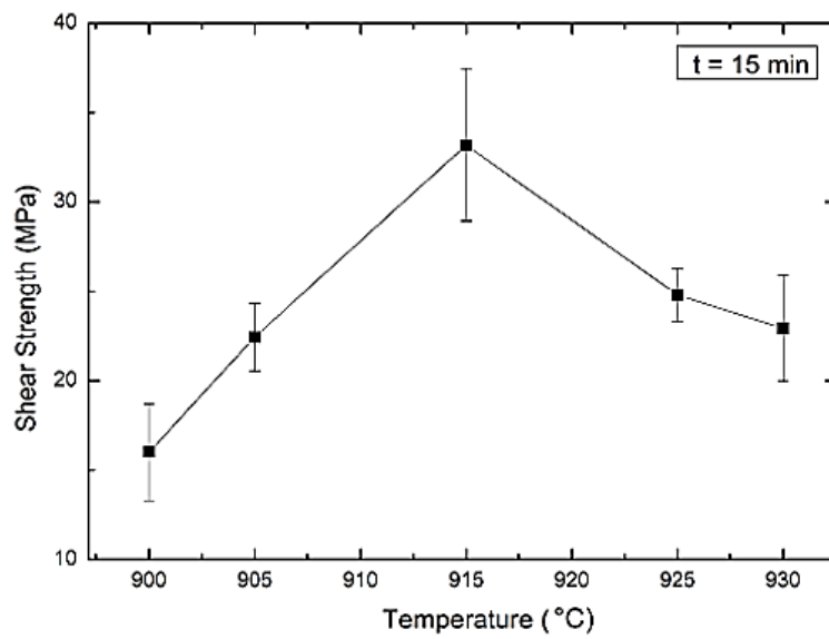
Figure 4.40 Shear test results of the brazed joints with respect to brazing temperature at constant brazing time.
