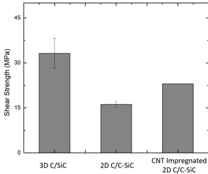
Figure 4.68 Mechanical property of the brazed joints between three different ceramic composites and Ti6Al4V alloy.
