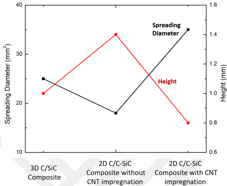
Figure 4.66 Fluidity of the Ticusil brazing filler alloy on different types of composites as presented by the spreading diameter and height of the droplet solidified after the wetting experiment.
