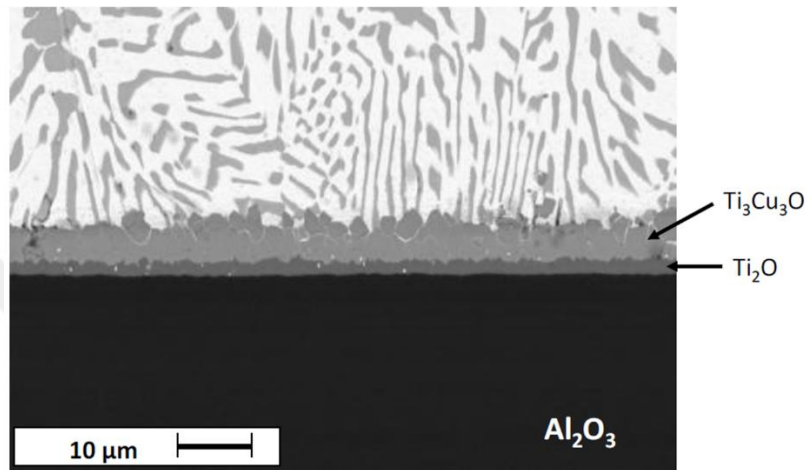
Figure 2.20 Microstructure of the interface between Alumina and Copper-Silver alloy after the wetting experiment [53].
