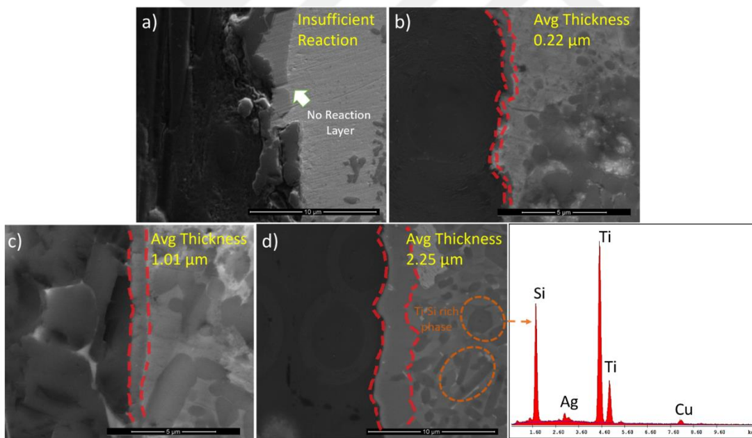
Figure 4.33 Average thickness values of the reaction layer at the C/SiC composite/Ticusil interlayer at constant brazing temperature of 915 °C with brazing time of a) 1 min, b) 5 min, c) 15 min, and d) 30 min.
