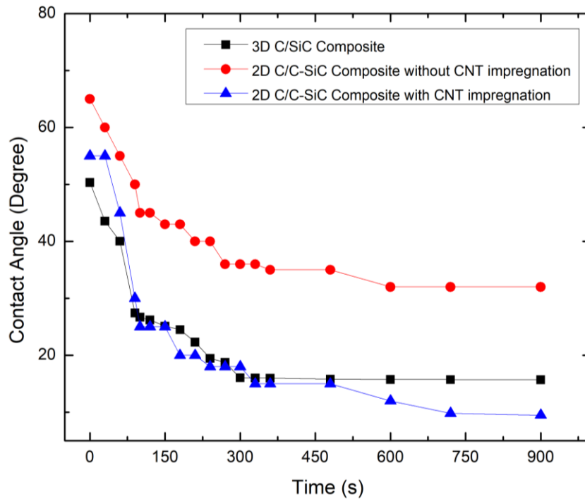
Figure 4.63 The variations of the contact angles with respect to time at the constant temperature of 915 °C for 3D C/SiC, 2D C/C-SiC and CNT impregnated 2D C/C-SiC configurations.
