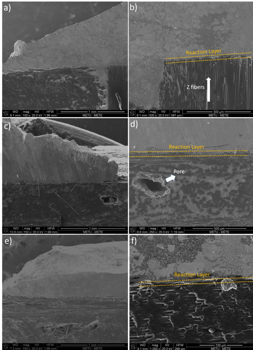
Figure 4.65 Cross-sectional views of the brazing filler alloy/ceramic composite surfaces after wetting experiments at 915 °C for 15 minutes a) 3D C/SiC composite b) reaction layer formation at the interface of the 3D C/SiC composite and brazing filler interlayer, c) 2D C/C-SiC composite, d) reaction layer formation at the interface of the 2D C/C-SiC composite and brazing filler interlayer, e) 2D C/C-SiC composite with CNT impregnation, f) reaction layer formation at the interface of the 2D C/C-SiC composite with CNT impregnation and brazing filler interlayer.
