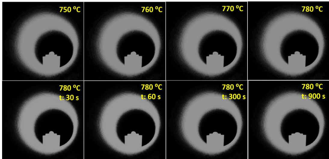
Figure 4.18 Morphological changes of Cusil brazing filler alloy on the Ti layer coated C/SiC composite surface under different temperature and time conditions.
