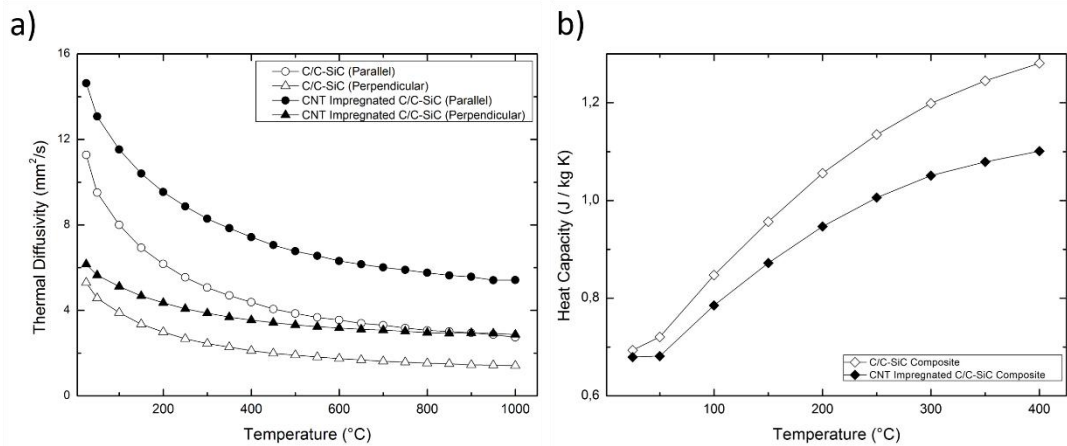
Figure 4.59 a) Thermal diffusivity and b) heat capacity values of the C/C-SiC composites.
