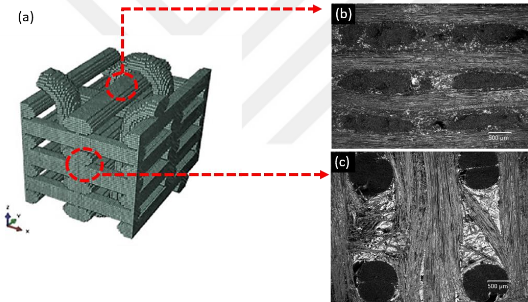
Figure 3.2 (a) Sketch of reinforcement architecture in 3D C/SiC composite (b) Micrograph of XY plane, (c) Micrograph of XZ plane.
