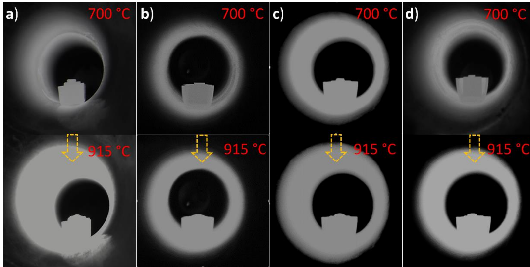
Figure 4.49 Morphological changes of brazing filler alloy on C/SiC composite surface containing different amounts of nano level SiC additive a) non-additive brazing filler alloy, b) 1 wt% nano level SiC, c) 2 wt% nano level SiC, d) 5 wt% nano level SiC.
