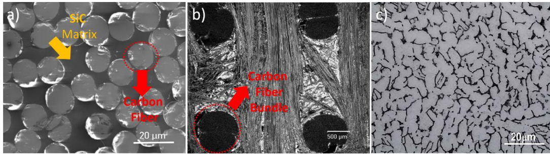
Figure 3.1 Microstructures of the initial materials used in the study a) XZ plane of the C/SiC composite, b) XZ plane view of the three-dimensional (3D) C/SiC composite and c) equiaxed microstructure of Ti6Al4V alloy containing \alpha (bright) and \beta (dark) phases.
