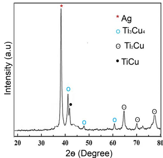
Figure 4.4 XRD analysis of Ti6Al4V/Cusil interlayer brazed at 875 °C for 10 min.
