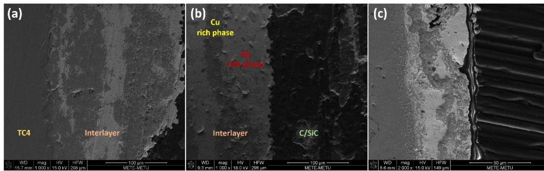
Figure 4.13 SEM micrographs of the interfaces between a) Ti6Al4V alloy and interlayer, b) interlayer and Ti layer coated C/SiC composite, c) the interlayer between C/SiC composite and Ti6Al4V alloy joints.
