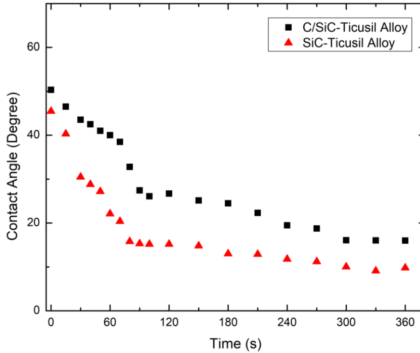
Figure 4.28 Contact angle variation of Ticusil brazing filler alloy with respect to time at 915 °C on both C/SiC composite and monolithic SiC ceramic.
