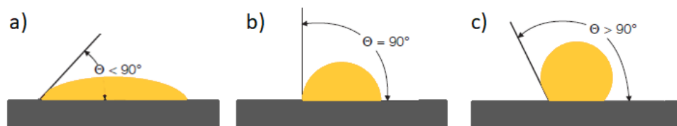
Figure 2.15 a) \theta_Y < 90^\circ ; strong wetting situation, b) \theta_Y = 90^\circ ; moderate wetting situation and c) \theta_Y > 90^\circ ; weak wetting situation.
