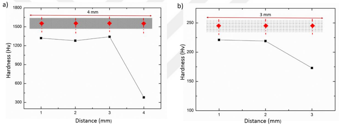
Figure 4.8 Microhardness analysis of C/SiC Composite/Cusil-ABA/Ti6Al4V alloy joint.
