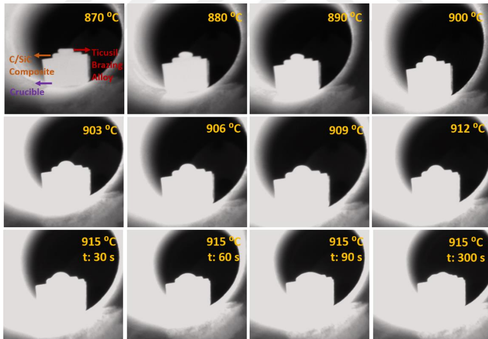
Figure 4.26 Morphological changes of brazing filler alloy on C/SiC composite surface under different temperature and time conditions.
