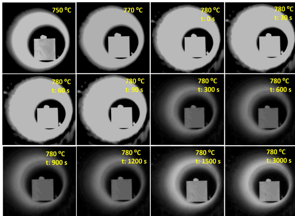
Figure 4.14 Morphological changes of Cusil brazing filler alloy on monolithic SiC ceramic surface under different temperature and time conditions.
