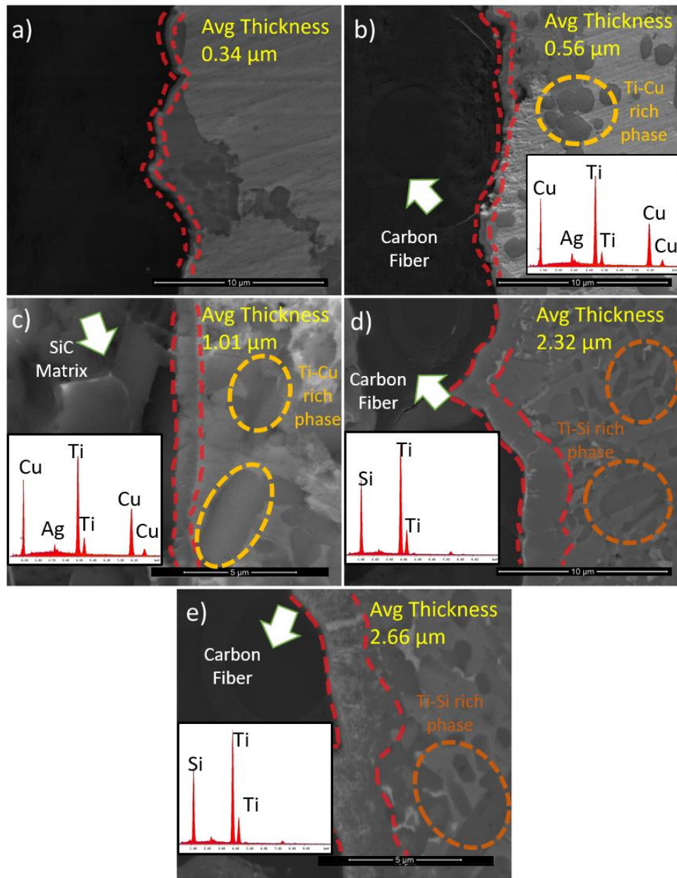
Figure 4.31 Average thickness values of the reaction layer at the C/SiC composite/Ticusil interlayer at constant brazing time of 15 min with brazing temperatures of a) 900 °C, b) 905 °C, c) 915 °C, d) 925 °C and e) 930 °C.
