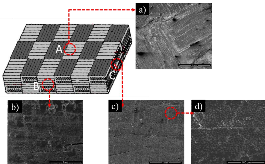
Figure 4.70 Sketch of the 2D plain woven C/C-SiC composite a) SEM micrograph of the surface A, b) SEM image of the surface B, c) SEM image of the surface C along fiber bundles, d) higher magnification image of the surface C.
