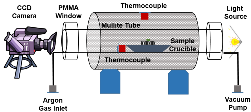
Figure 3.6 Schematic illustration of the in-house modified furnace used for wetting experiments.
