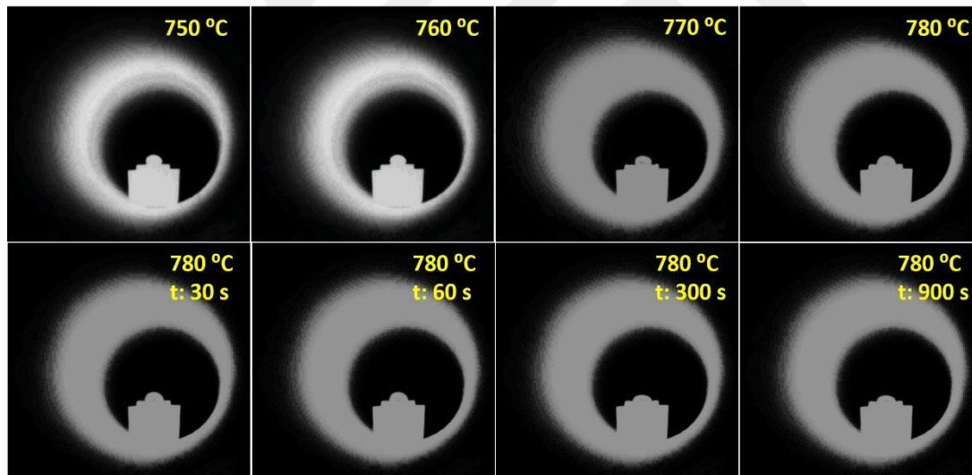
Figure 4.20 Morphological changes of 1.25 wt% Ti powder containing Cusil brazing filler alloy on C/SiC composite surface under different temperature and time conditions.
