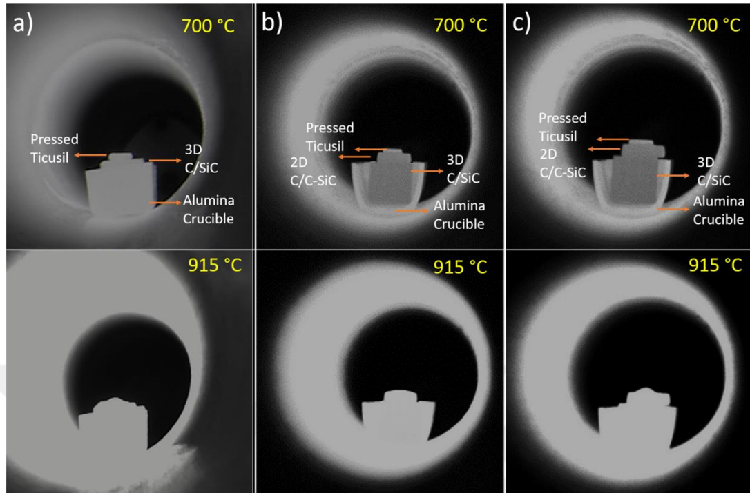
Figure 4.64 Morphological changes of Ticusil brazing filler alloy on different composite surfaces a) commercial 3D C/SiC composite, b) 2D C/C-SiC composite with CNT impregnation, c) 2D C/C-SiC composite without CNT impregnation.
