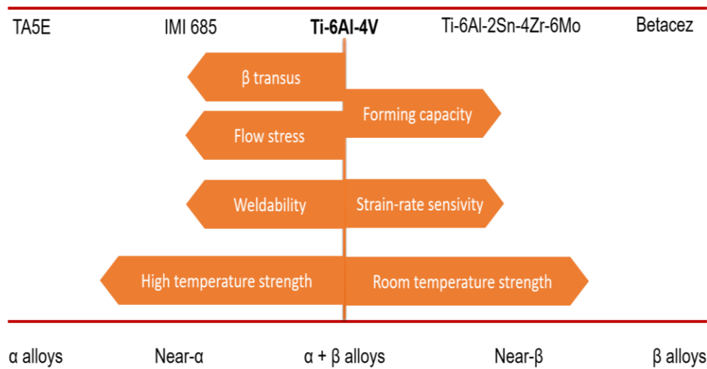
Figure 2.5 The key features of Titanium alloys [25].
