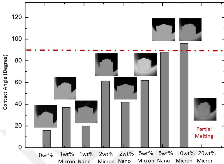
Figure 4.51 Effects of SiC additive particle size and content on the contact angle of the brazing filler alloy.
