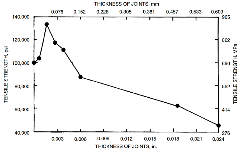
Figure 2.13 Effects of joint clearance on tensile strength of the brazed joints.
