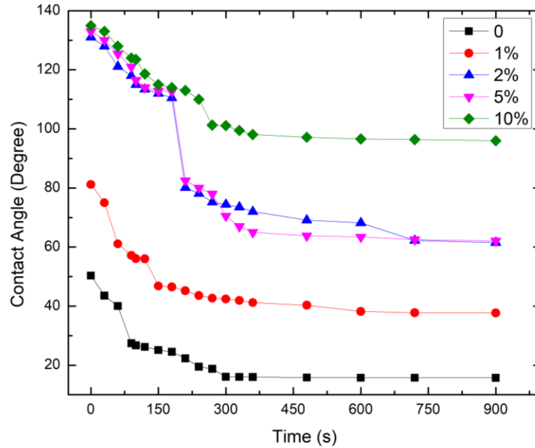
Figure 4.48 Change in measured contact angle as a function of time at 915 °C for brazing filler alloy with different micron level SiC additive amounts.
