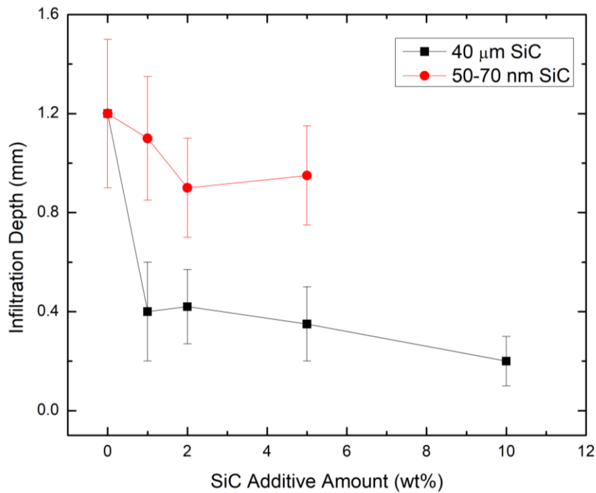
Figure 4.53 Infiltration depth values of the Ticusil brazing filler alloy in accordance with the different content and size of SiC additive.
