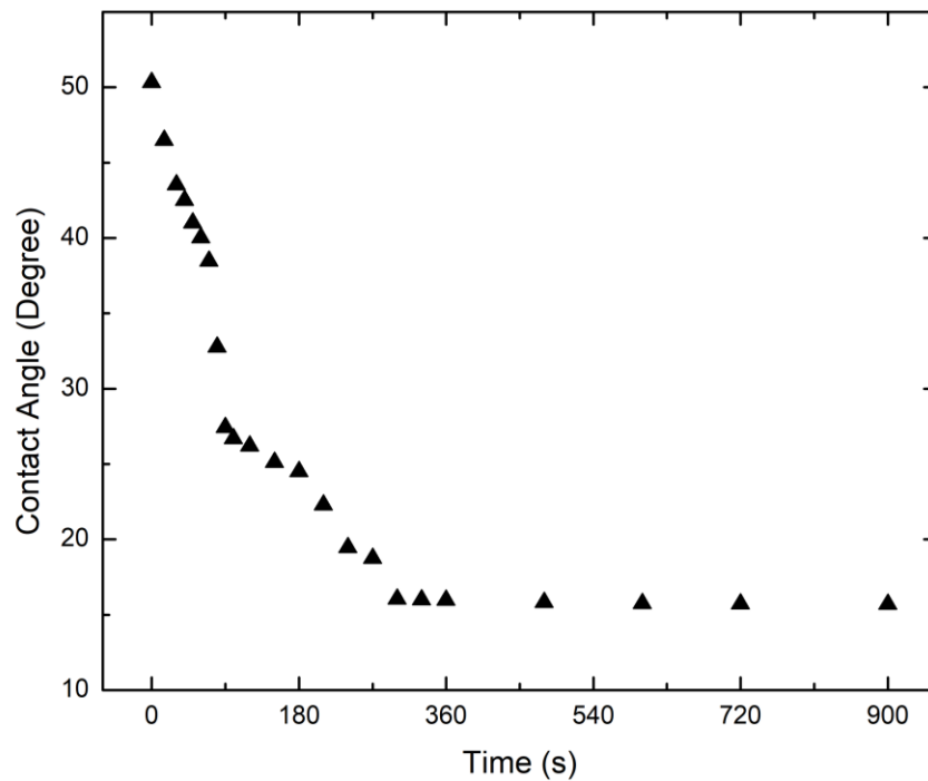
Figure 4.27 Change in the measured contact angle as a function of time at 915^\circ\text{C} .
