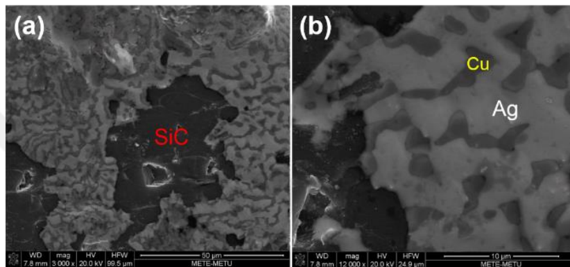
Figure 4.2 Microstructures of Cusil brazing filler alloy over the C/SiC surface.
