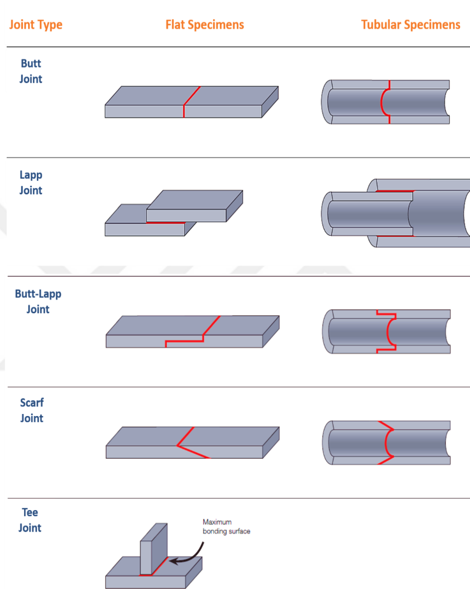
Figure 2.12 Braze joint configurations.
