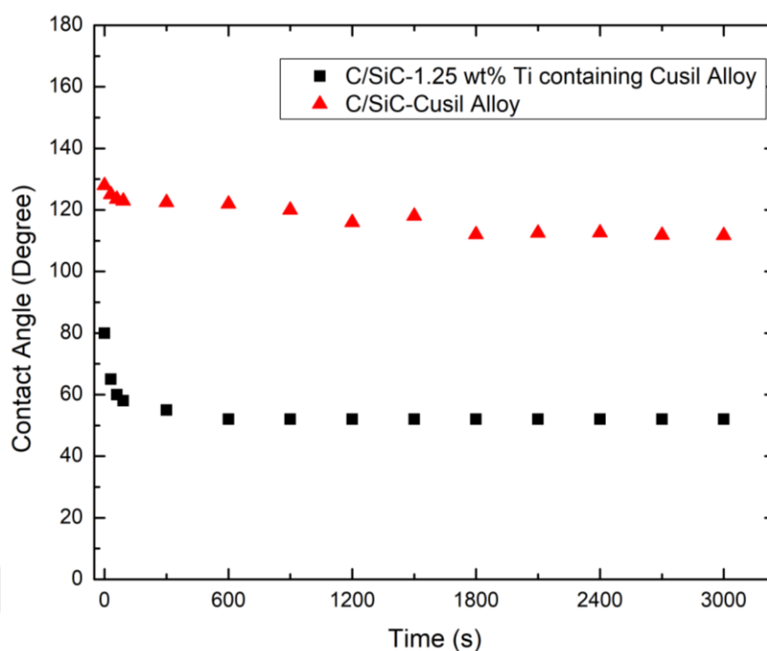
Figure 4.21 Contact angle variation of Cusil and 1.25 wt% Ti containing Cusil brazing filler alloys with respect to time at 780 °C.
