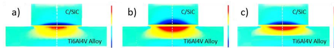
Figure 4.69 Residual stress distribution of the brazed joints upon cooling from the brazing temperature a) 3D C/SiC composite, b) 2D C/C-SiC composite without CNT impregnation, c) 2D C/C-SiC composite with CNT impregnation.
