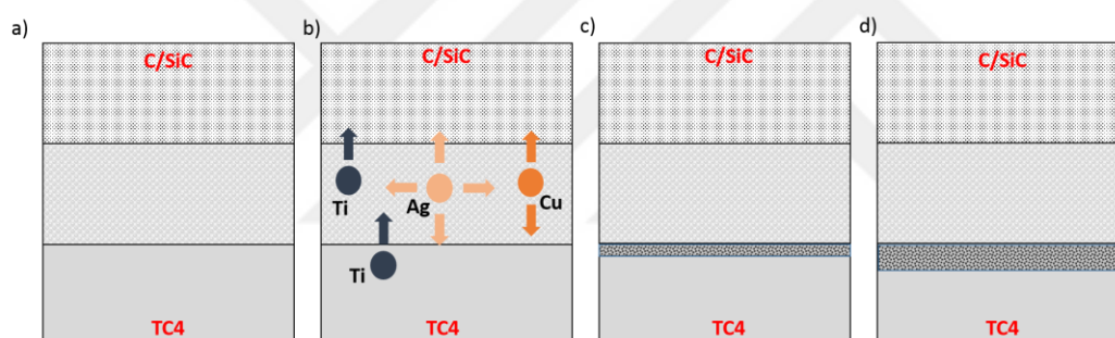
Figure 4.9 The interface evolution model for the C/SiC composite/Cusil-ABA/Ti6Al4V alloy joint.
