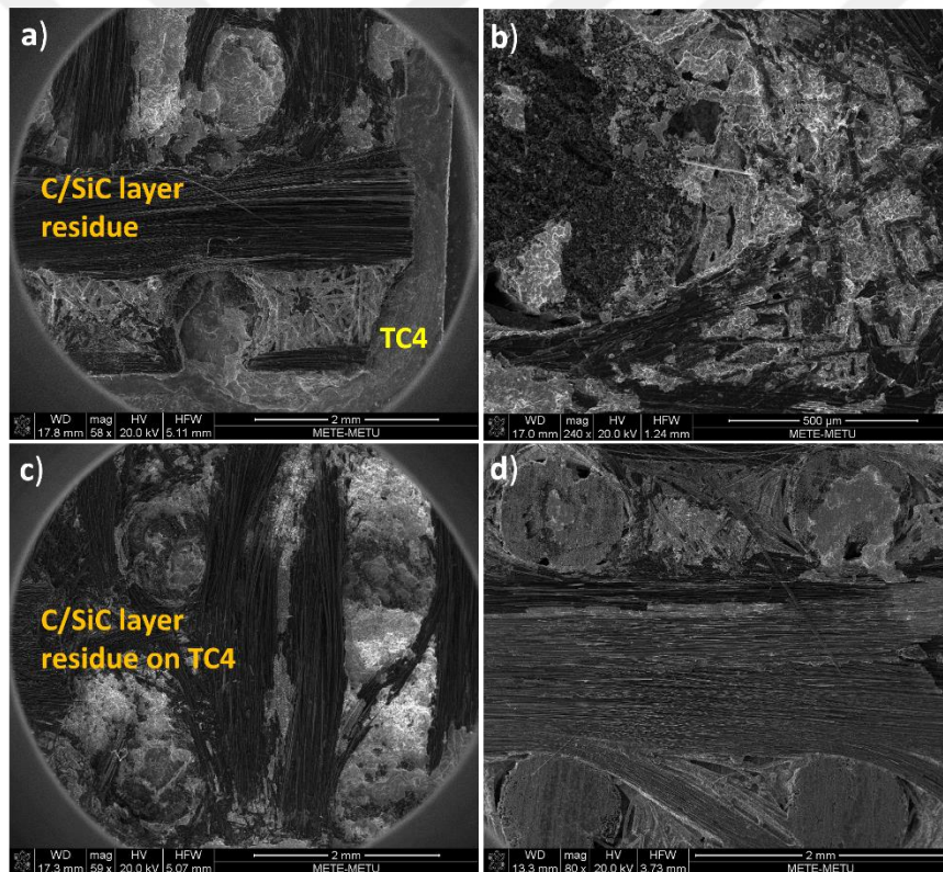
Figure 4.56 The fracture surface of the brazed joints a) C/SiC layer residual on Ti6Al4V alloy surface (2 wt% nano level), b) C/SiC composite surface (5 wt% nano level), c) C/SiC layer residual on Ti6Al4V alloy surface (1 wt% micron level), d) C/SiC composite surface (10 wt% micron level).
