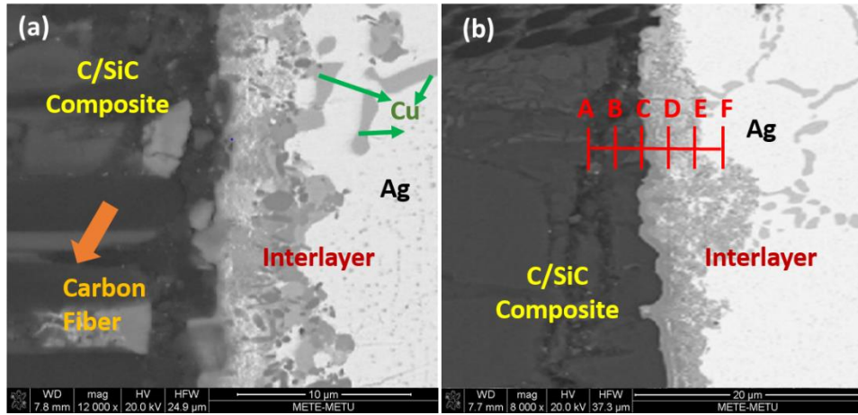
Figure 4.7 SEM micrographs of C/SiC Composite/Cusil-ABA/Ti6Al4V Alloy brazed at 875 °C, for 5 min a) and b) the interface between C/SiC composite and the interlayer.
