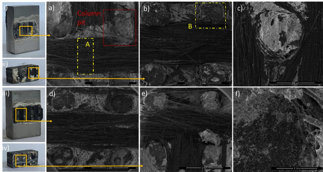
Figure 4.42 The fracture surface of the brazed joints at macro level i) Ti6Al4V alloy (930 °C, 15 min), ii) C/SiC composite (930 °C, 15 min), iii) Ti6Al4V alloy (915 °C, 15 min), iv) C/SiC composite (915 °C, 15 min); the fracture surfaces in micro level a) Ti6Al4V alloy (930 °C, 15 min), b) C/SiC composite (930 °C, 15 min), c) residual Ticusil alloy on the C/SiC composite surface (930 °C, 15 min), d) Ti6Al4V alloy (915 °C, 15 min), e) C/SiC composite (915 °C, 15 min), f) residual Ticusil alloy on the C/SiC composite surface (915 °C, 15 min).
