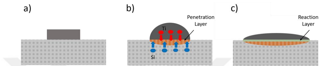
53. Figure 4.44 Wetting mechanism of the brazing filler alloy on the C/SiC composite surface.
