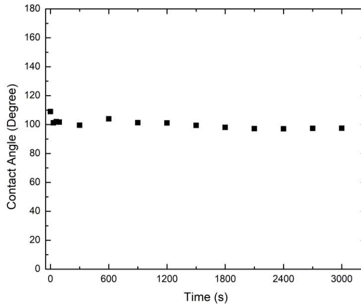
Figure 4.15 Contact angle variation of Cusil brazing filler alloy with respect to time at 780 °C on monolithic SiC ceramic.
