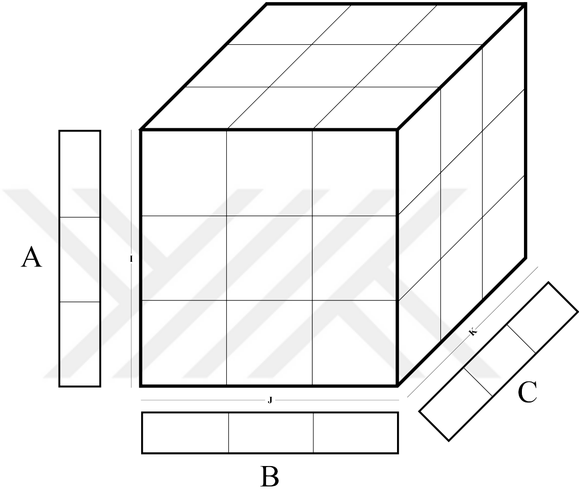
Figure 5.1: Tiling
