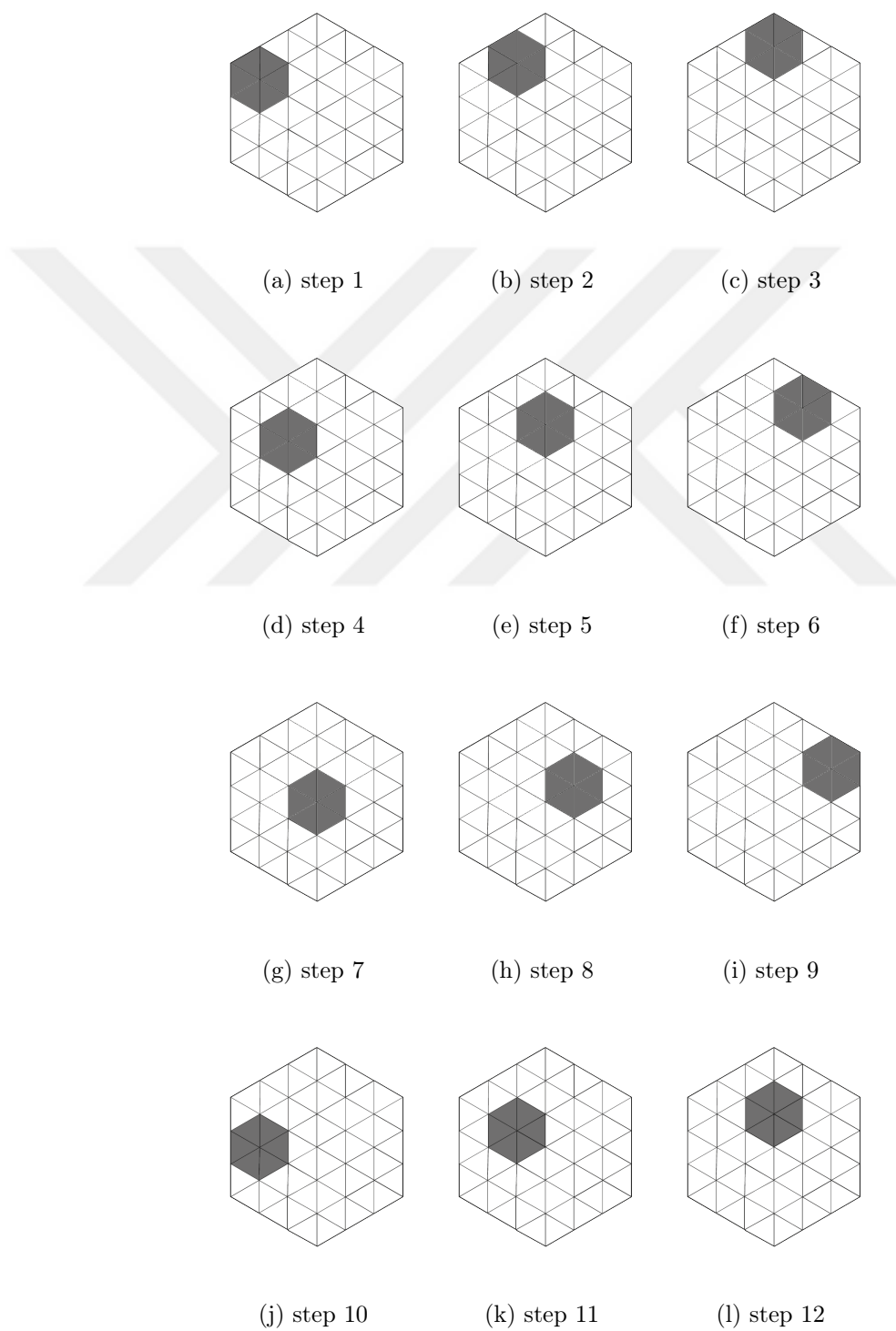
Figure 5.2: Tiling Algorithm 1
