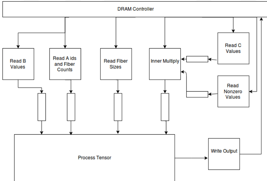
Figure 6.1: Tensor Computation Block Diagram
