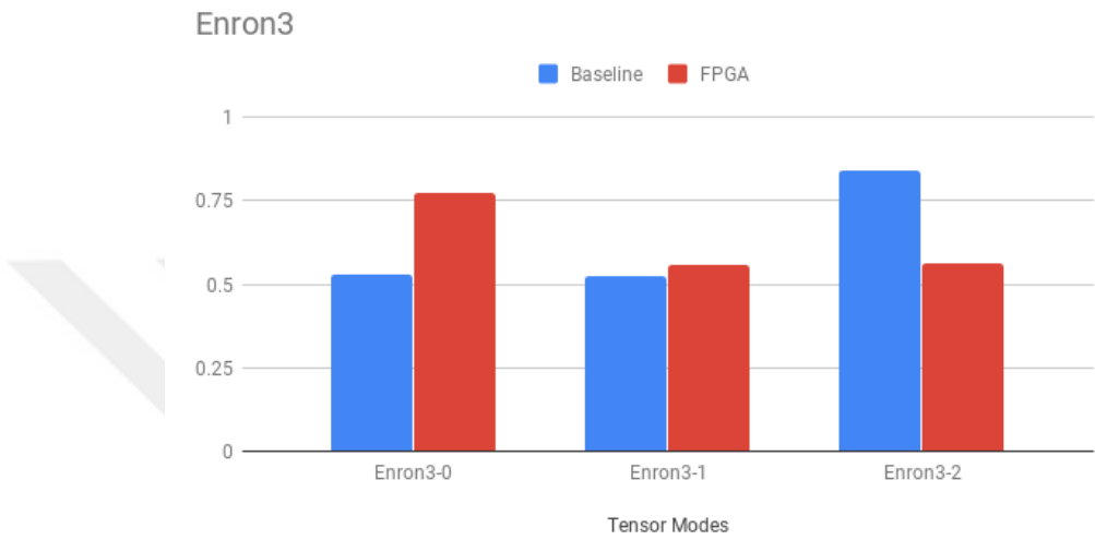
Figure 7.7: Enron3 Tensor Runtimes on Modes
