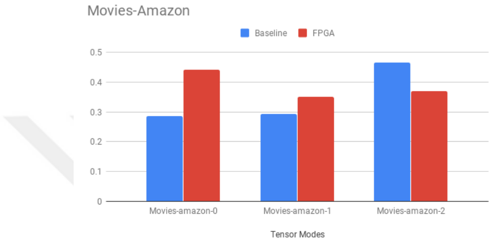
Figure 7.5: Movies-Amazon Tensor Runtimes on Modes
