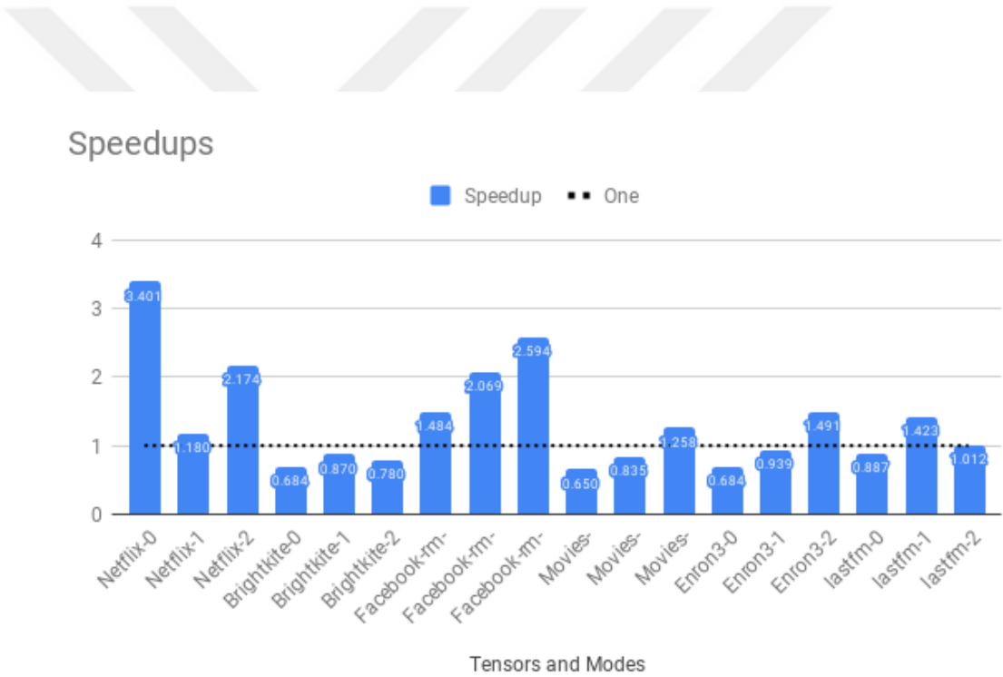
Figure 7.9: Speedups on Tensor Modes
