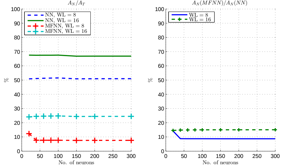
Figure 4.7: Relative area of MFNN and NN
