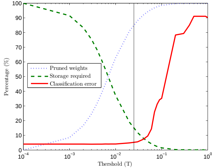
Figure 4.14: Pruning results for one-hidden-layer NN
