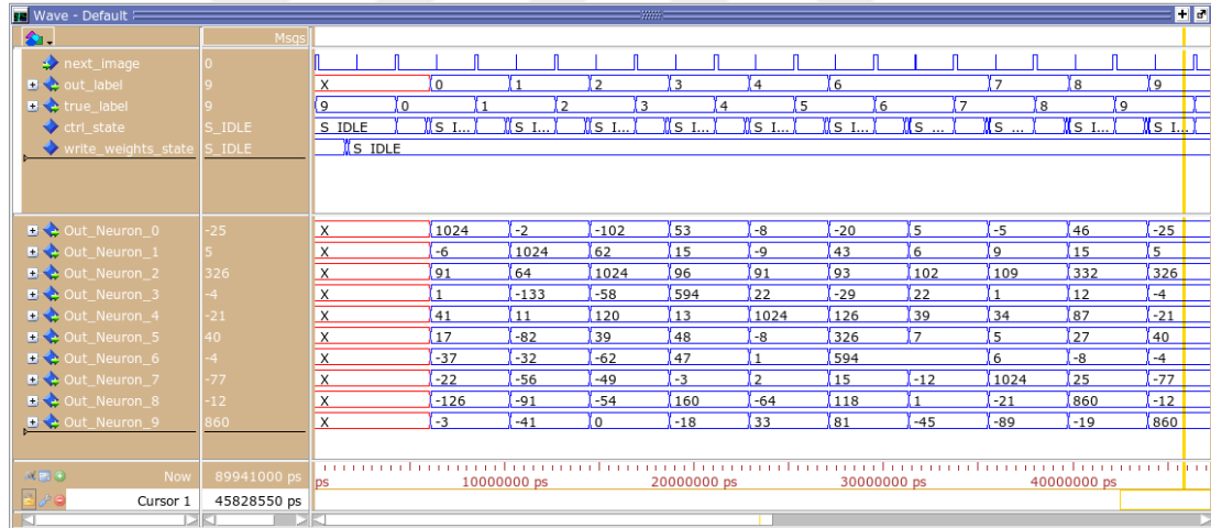
Figure 3.8: Wave from simulation for one-hidden-layer NN
