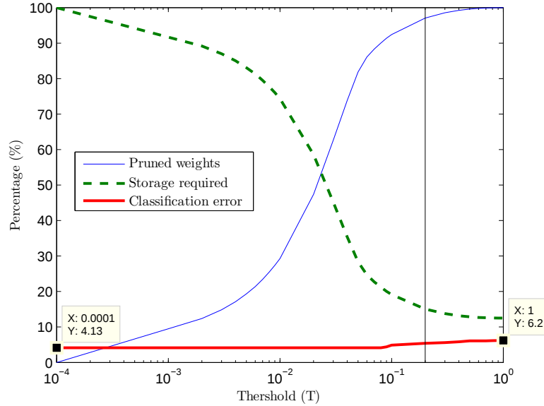
Figure 4.16: Enhanced pruning results for one-hidden-layer MFNN
