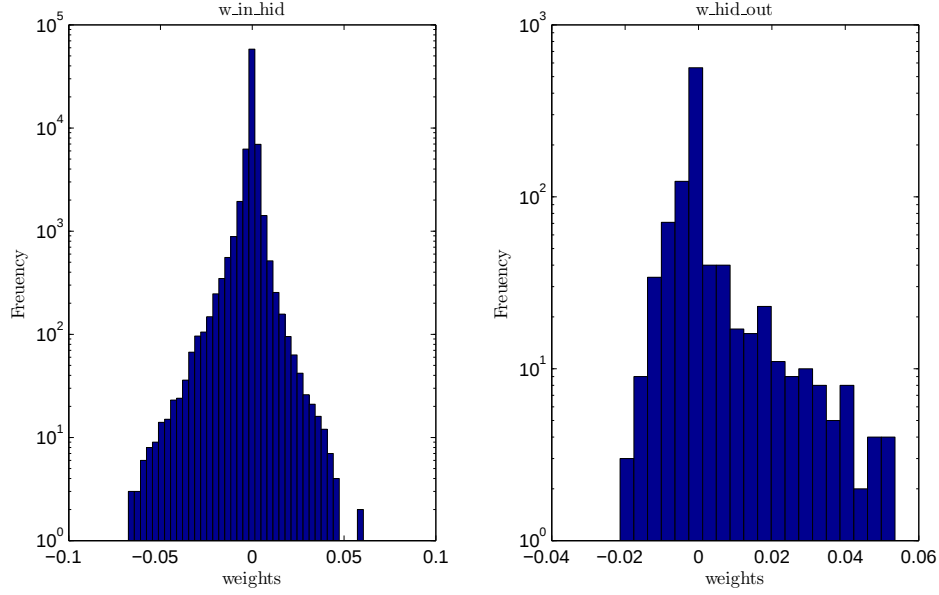
Figure 4.11: Weight distribution in one-hidden-layer MFNN
