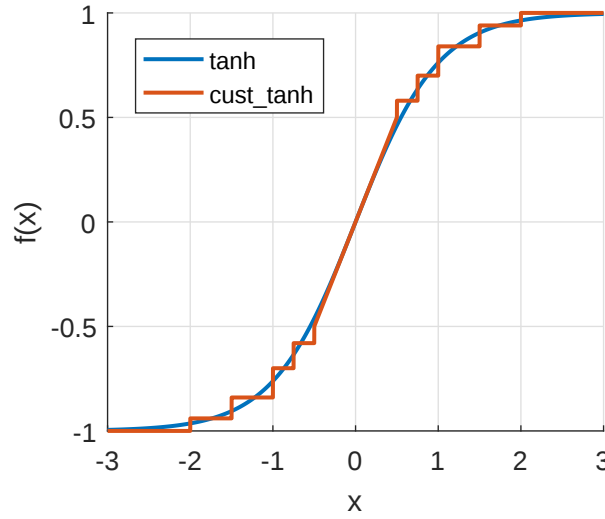
Figure 3.7: Approximation of tanh to a piecewise function
