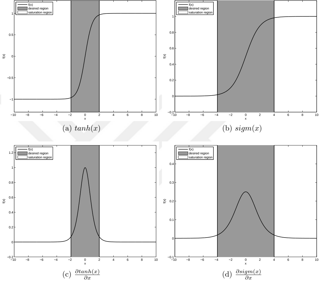
Figure 2.2: Activation functions with their derivatives
