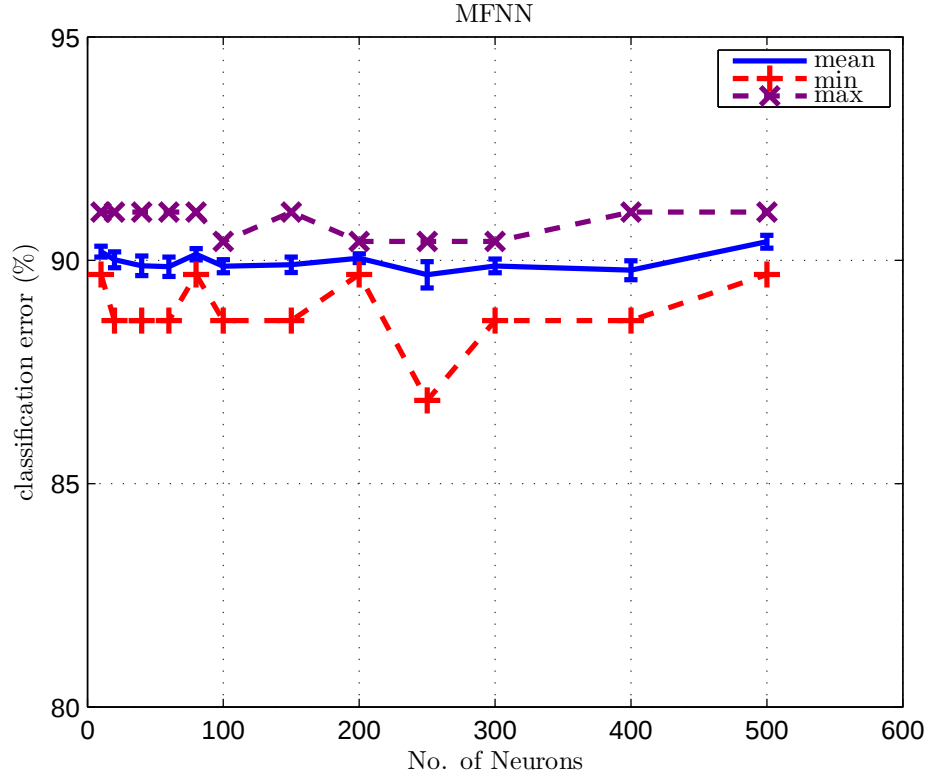
Figure 4.2: Classification error (%) in one-hidden-layer MFNN without normalization
