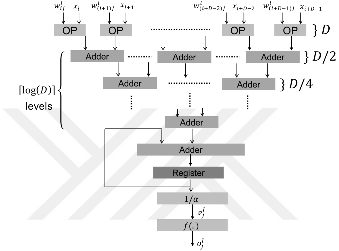
Figure 3.6: Hybrid neuron diagram of the j_{th} neuron in layer l + 1 with a parallel degree of D OP operations per cycle
