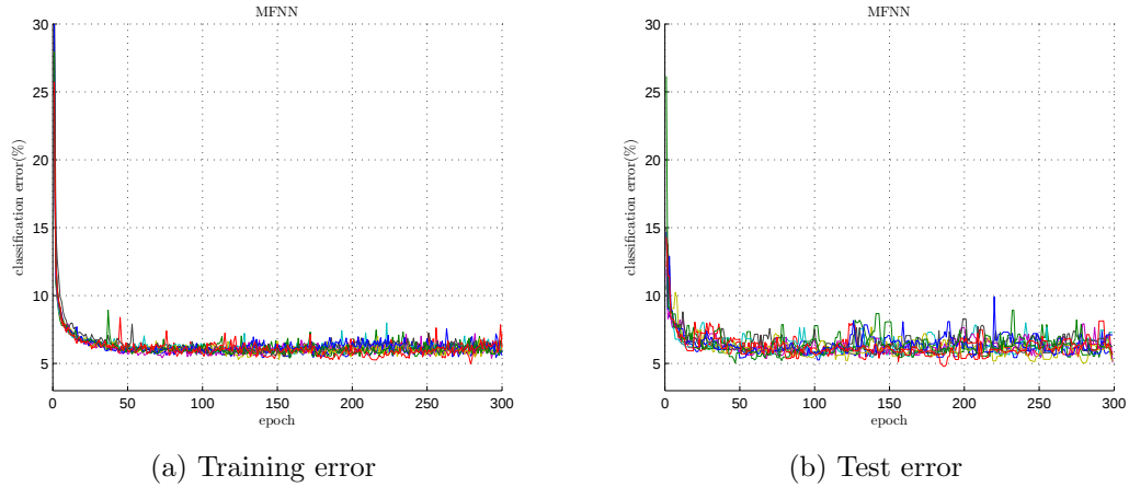
Figure 4.5: Classification error proration during training of MFNN
