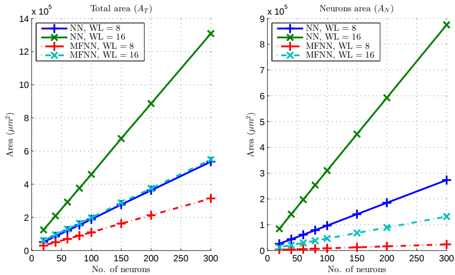
Figure 4.6: Area measurements of NN and MFNN for different word lengths
