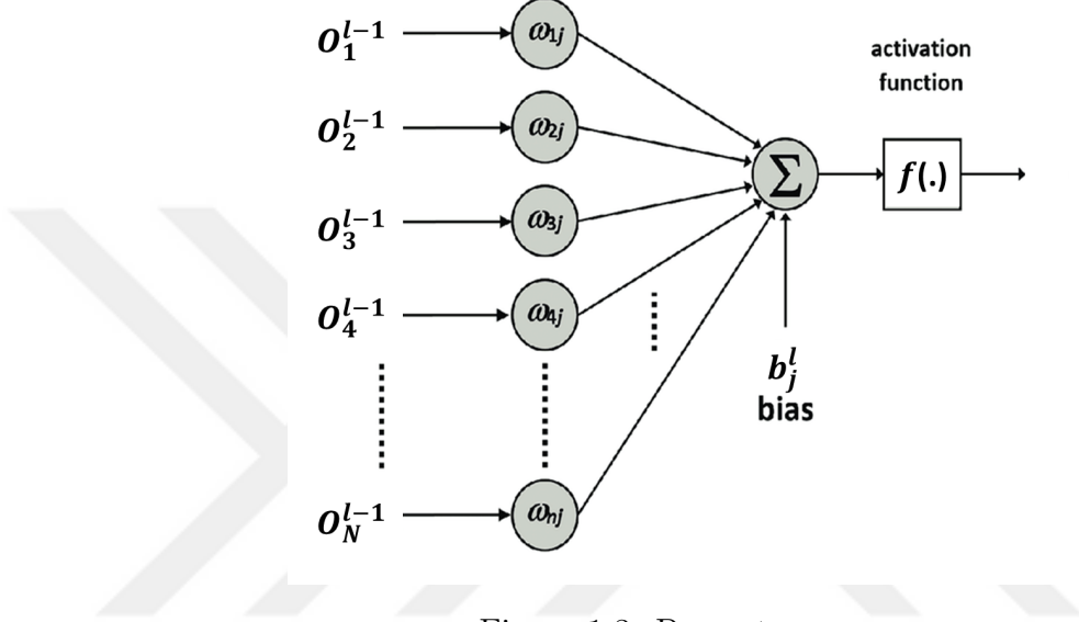
Figure 1.3: Perceptron
