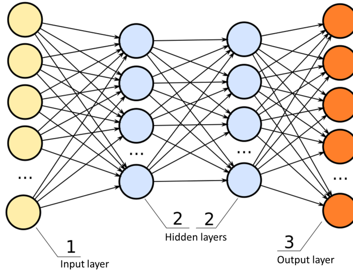
Figure 1.2: Multilayer Perceptron
