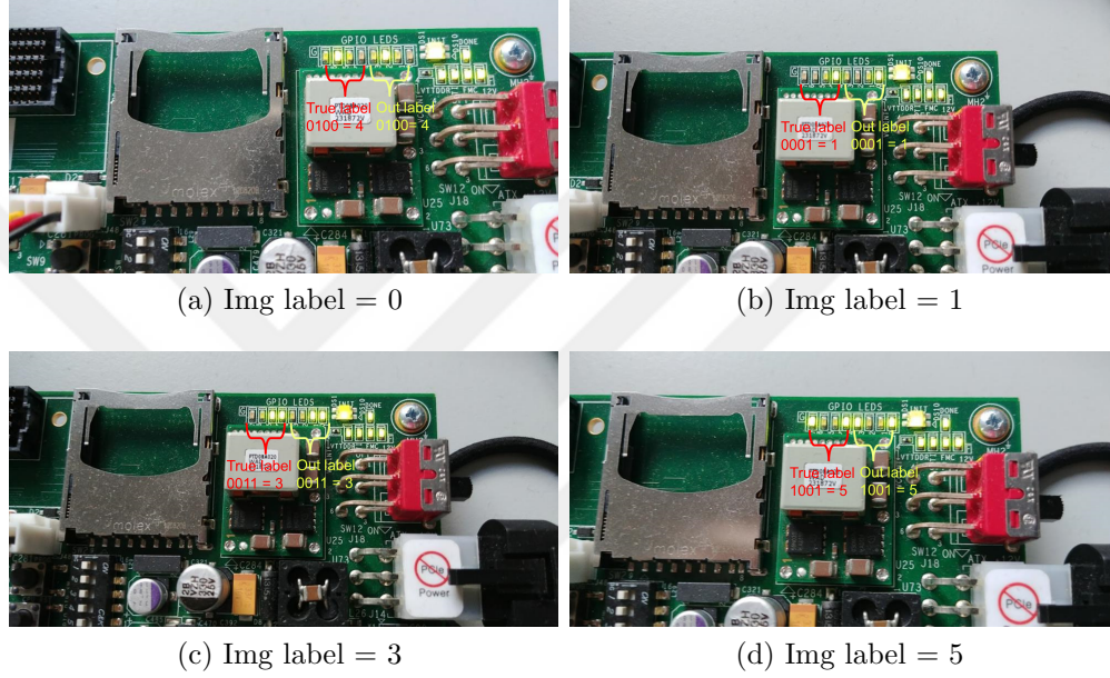
Figure 3.10: FPGA board operational with output and true labels
