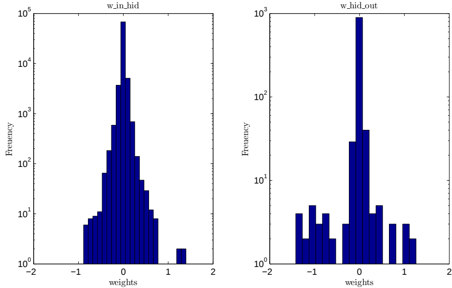
Figure 4.10: Weight distribution in one-hidden-layer NN
