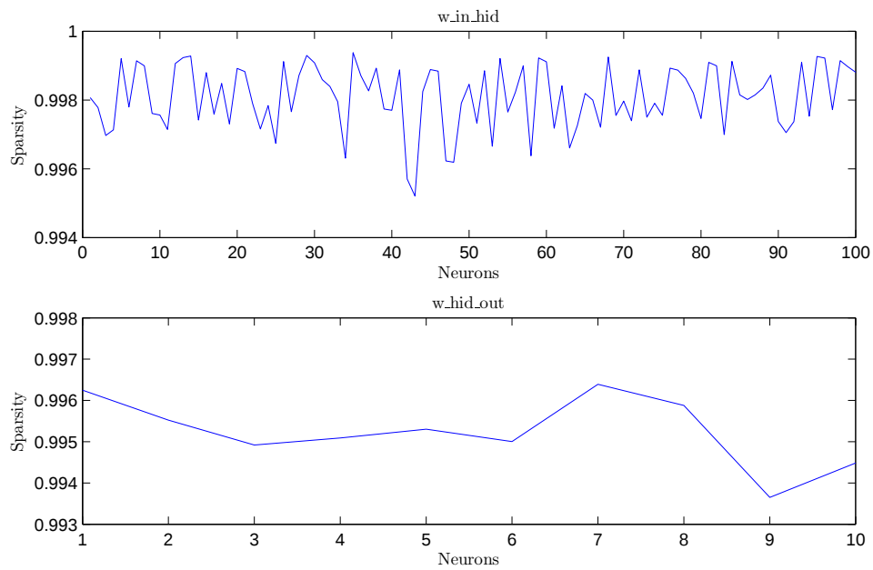
Figure 4.13: Weight sparsity in one-hidden-layer MFNN
