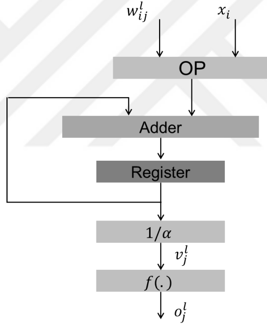
Figure 3.5: Serial neuron diagram of the j_{th} neuron in layer l + 1
