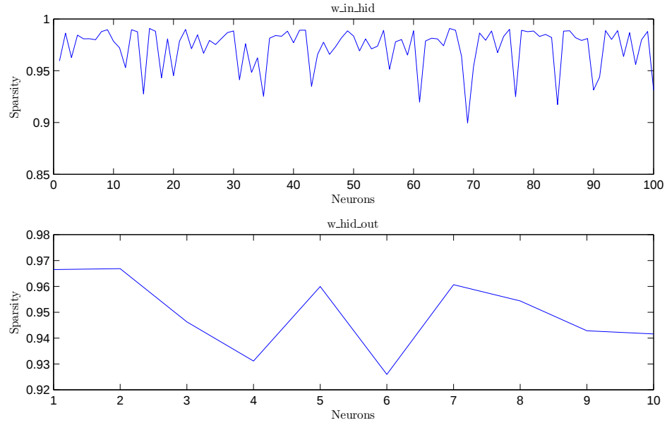
Figure 4.12: Weight sparsity in one-hidden-layer NN
