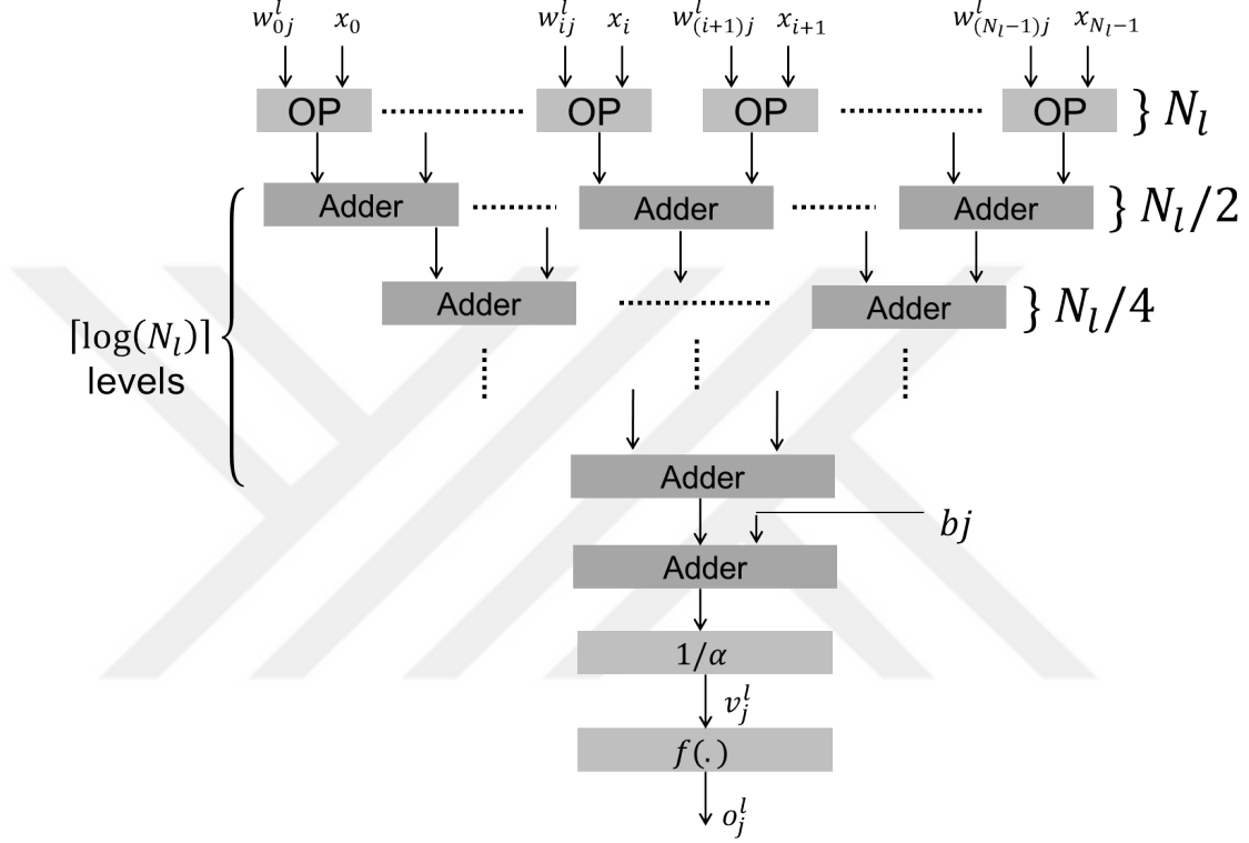
Figure 3.4: Parallel neuron diagram of the j_{th} neuron in layer l + 1
