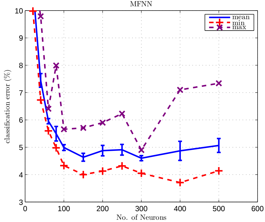
Figure 4.3: Classification error (%) in one-hidden-layer MFNN with normalization
