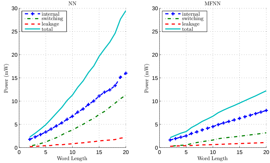
Figure 4.8: Power measurements of NN and MFNN for different word lengths
