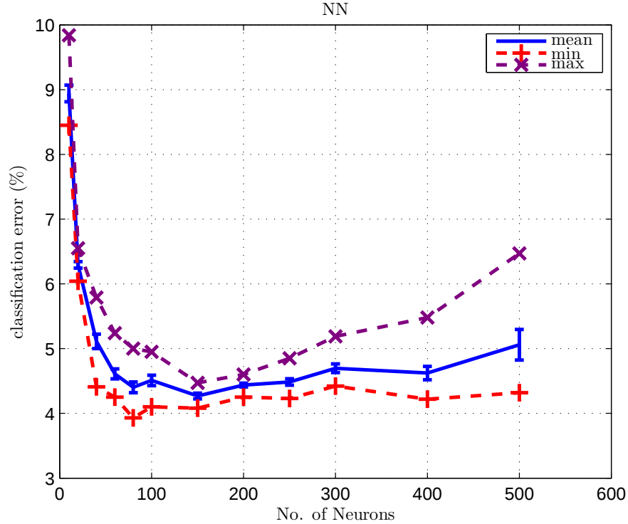
Figure 4.1: Classification error (%) in one-hidden-layer NN
