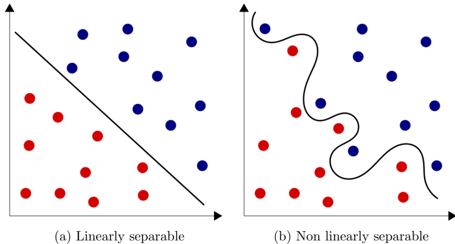
Figure 1.1: Data Separability
