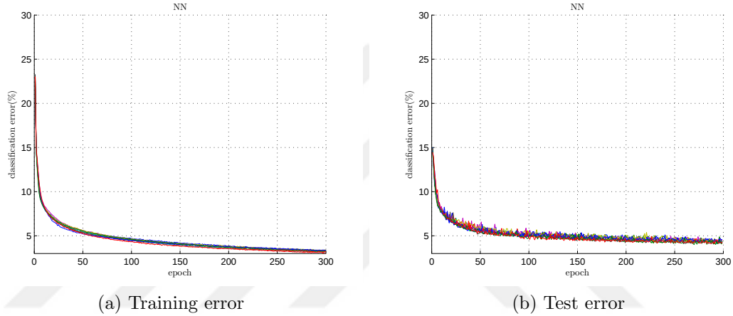
Figure 4.4: Classification error proration during training of NN
