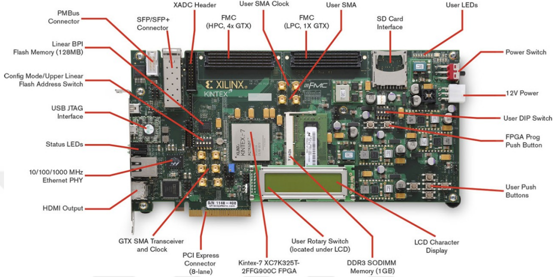
Figure 3.2: VC707 Evaluation Board [42]
