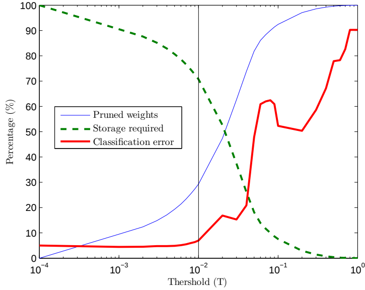
Figure 4.15: Pruning results for one-hidden-layer MFNN
