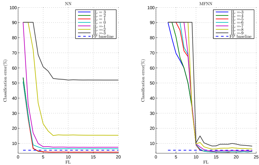
Figure 4.9: Classification error (%) for fixed-point one-hidden-layer NN and MFNN
