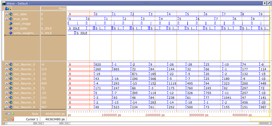
Figure 3.9: Wave from simulation for one-hidden-layer MFNN
