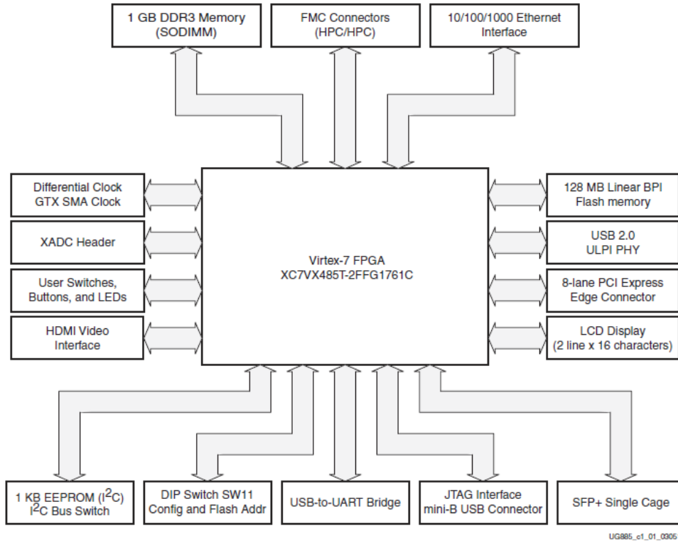
Figure 3.1: VC707 Evaluation Board schematic [42]
