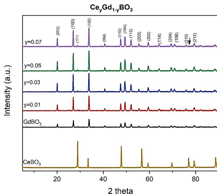
Figure 3.2. XRD patterns of \text{Ce}^{3+} doped \text{GdBO}_3 ( y for \text{Ce}^{3+} )
