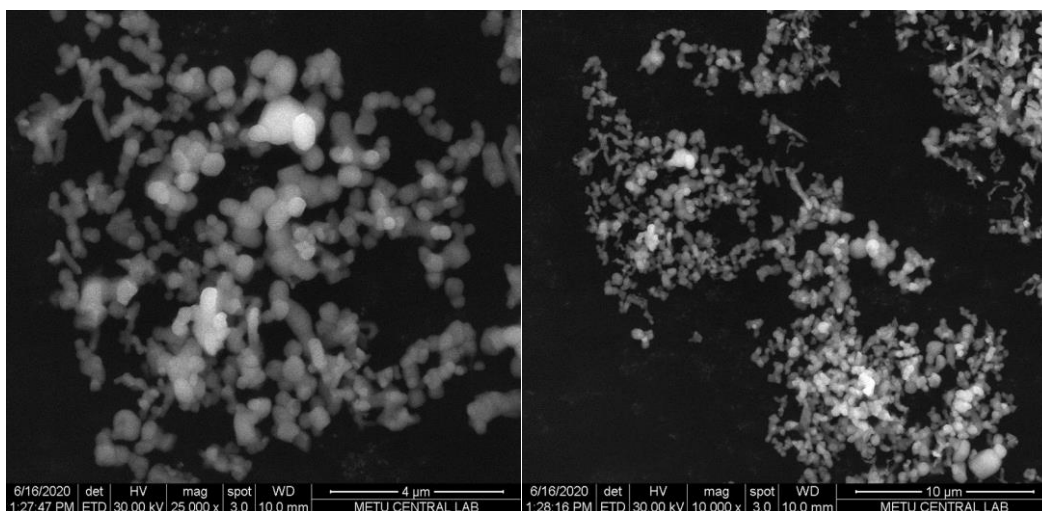
Figure 3.28. SEM images of \text{Ce}^{3+}/\text{Tb}^{3+}/\text{Yb}^{3+} doped \text{GdBO}_3
