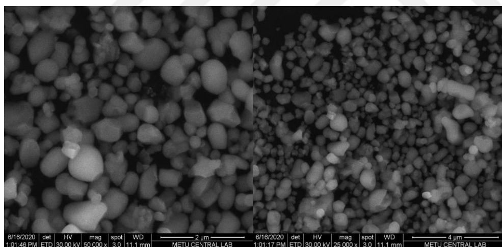
Figure 3.24. SEM images of \text{Ce}^{3+}/\text{Dy}^{3+} doped \text{GdBO}_3
