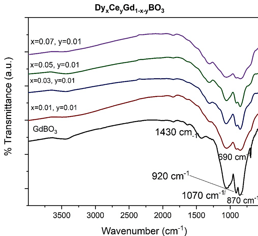
Figure 3.16. FTIR spectra of phosphors have 0.01 \text{Ce}^{3+} and changing the concentration of \text{Dy}^{3+} (x for \text{Dy}^{3+} and y for \text{Ce}^{3+} )
