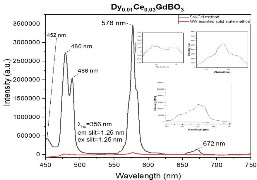
Figure 3.53. Emission spectra of the 1% Dy 3+ -3% Ce 3+ codoped GdBO 3 synthesized with sol-gel and microwave assisted solid-state method at 356 nm
