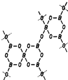
The tetraborate group ( a_6c_2 ), observed in the compound \text{Na}_2\text{O} \cdot 4 B_2O_3 .
