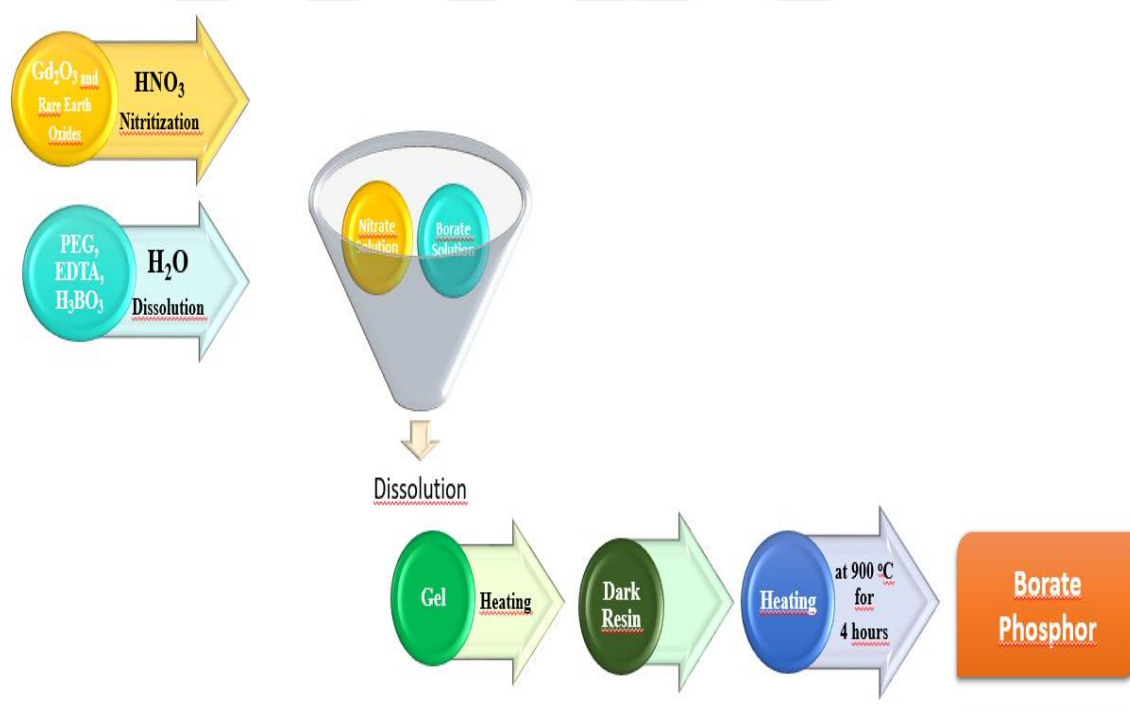
Figure 2.1. Schematic representation of the sol-gel method
