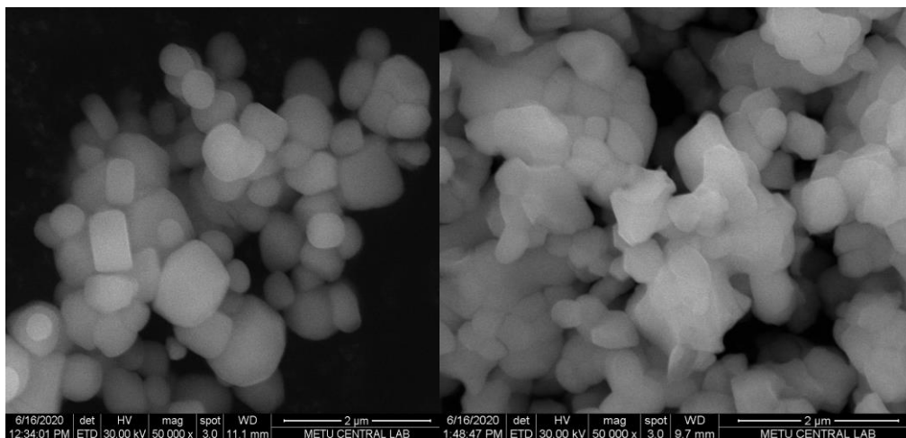
Figure 3.29. SEM images of Sol-Gel synthesized (right) and solid-state synthesized 5% \text{Ce}^{3+} doped \text{GdBO}_3 phosphors
