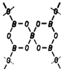
The pentaborate group ( a_4c ), observed in the compounds \alpha\text{-K}_2\text{O} \cdot 5 B_2O_3 and \beta\text{-K}_2\text{O} \cdot 5 B_2O_3 .
