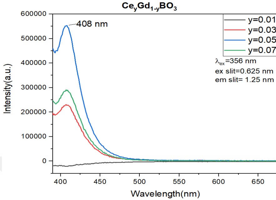
Figure 3.33. Emission spectra of \text{Ce}^{3+} single doped \text{GdBO}_3 at 356 nm without filter
