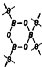
The triborate group ( a_2c ), observed in the compound \text{Cs}_2\text{O} \cdot 3 B_2O_3 .
