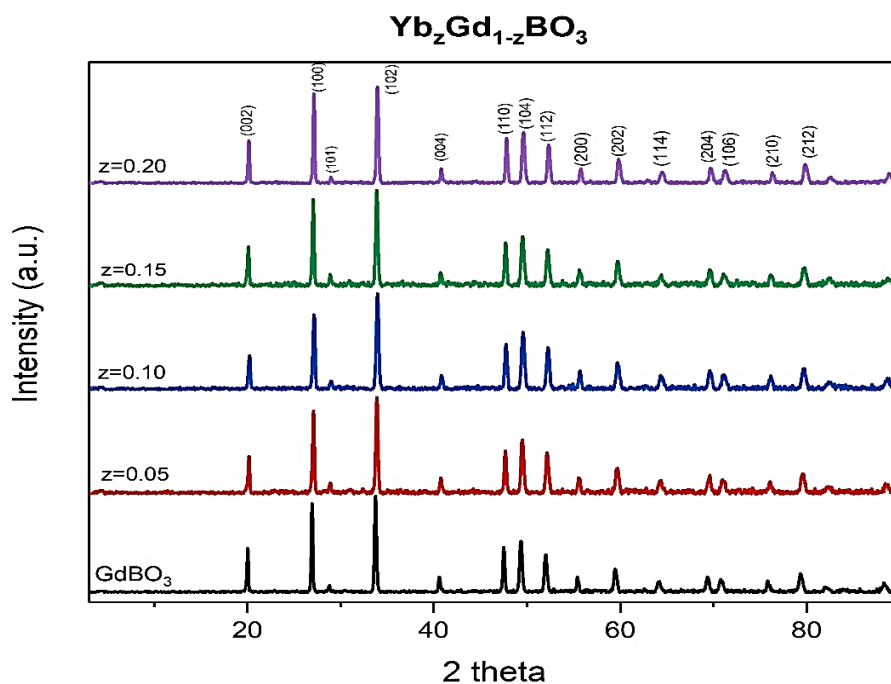
Figure 3.9. Single doped \text{GdBO}_3 with changing \text{Yb}^{3+} concentration ( z=5\% , 10\% , 15\% , 20\% )
