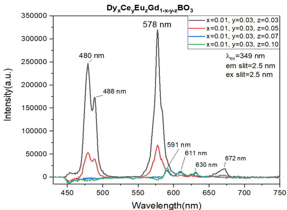
Figure 3.42. Emission spectra of 1% \text{Dy}^{3+} , 3% \text{Ce}^{3+} doped and \text{Eu}^{3+} doped \text{GdBO}_3 with changing \text{Eu}^{3+} concentration at 349-nm excitation
