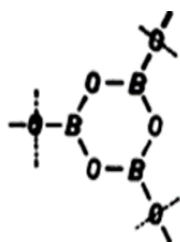
The boroxol ring ( a_3 ), observed in vitreous B_2O_3 .
