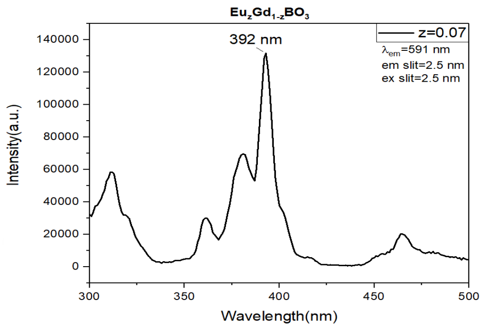
Figure 3.35. The excitation spectrum of Eu 3+ doped GdBO 3
