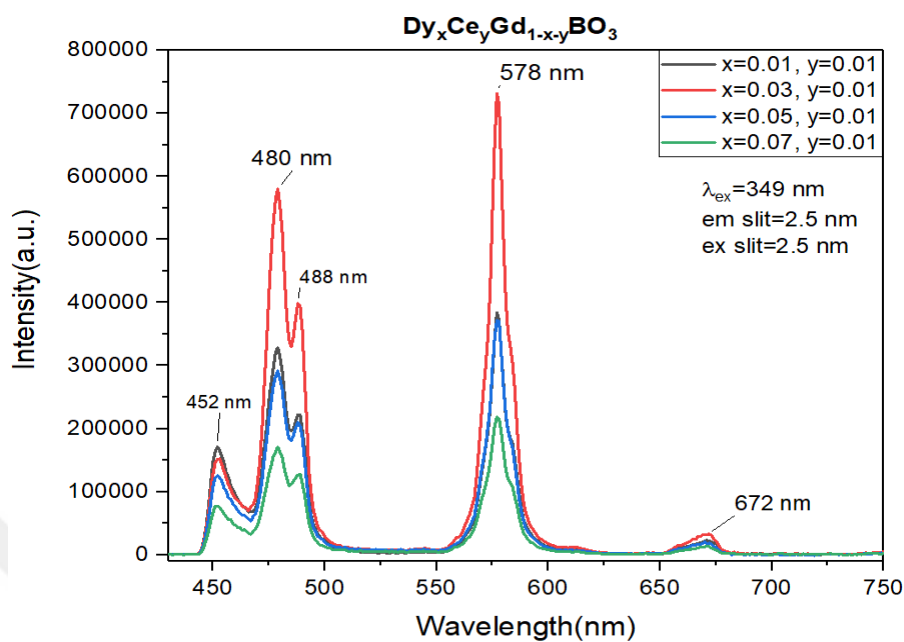
Figure 3.37. Emission spectra of 1% \text{Ce}^{3+} fixed and \text{Dy}^{3+} doped with changing concentration at 349 nm
