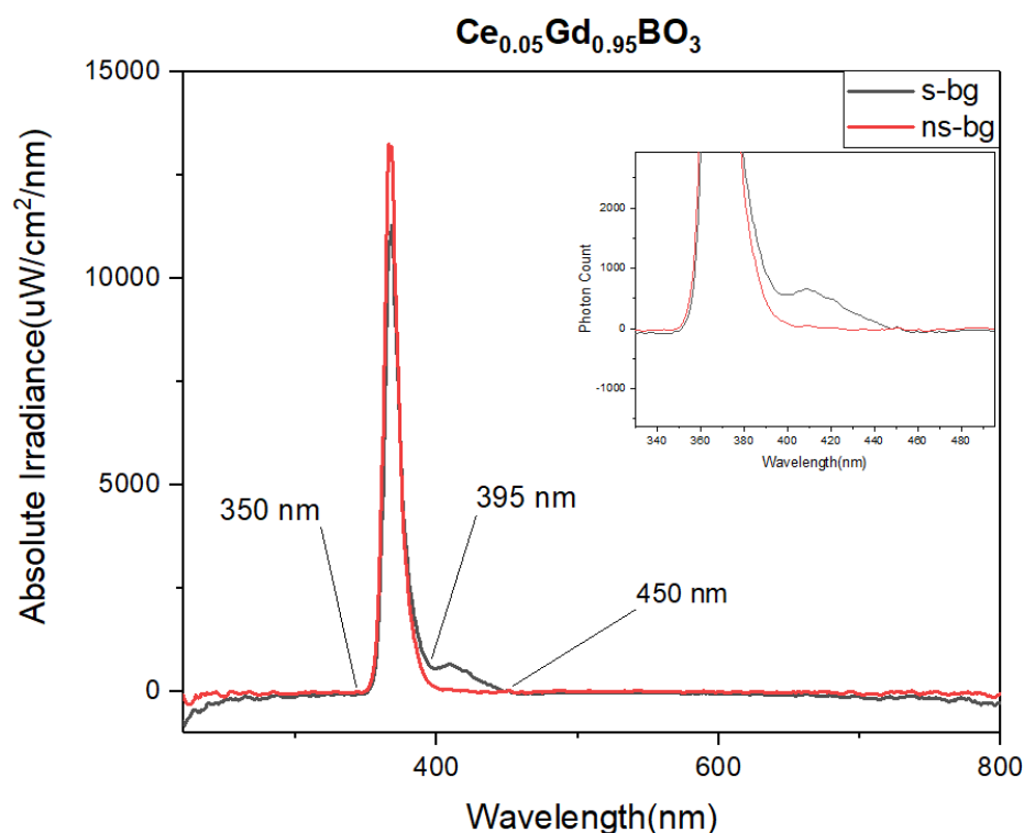
Figure 3.60. Absorption and emission regions used for the calculation of 0.05 \text{Ce}^{3+} doped (in terms of mole) doped \text{GdBO}_3
