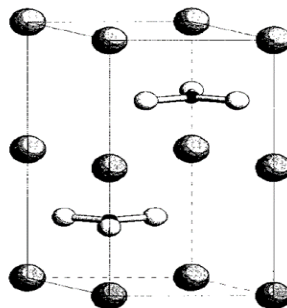
Figure 1.16. High-Temperature crystal structure of GdBO 3 (Ren et al., 1999)
