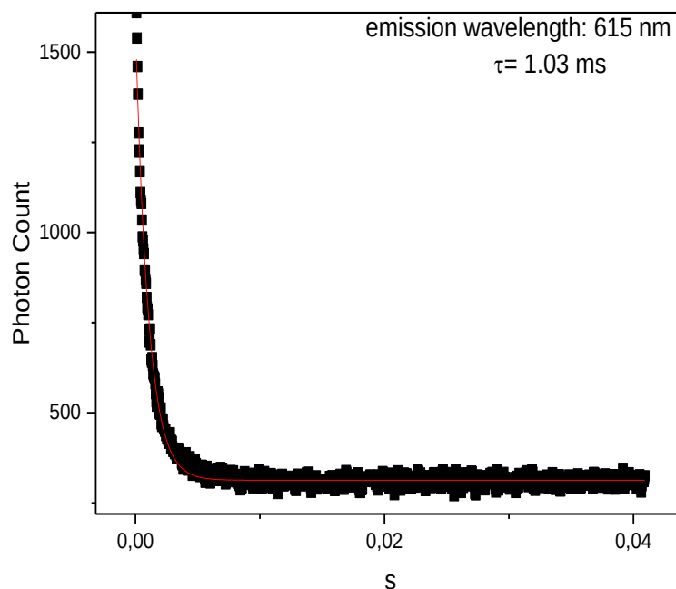
Figure 3.56. Decay curve of 7% \text{Eu}^{3+} doped \text{GdBO}_3
