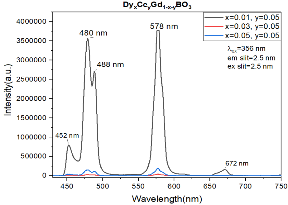
Figure 3.41. Emission spectra of 5% \text{Ce}^{3+} fixed and \text{Dy}^{3+} doped with changing concentration at 356 nm
