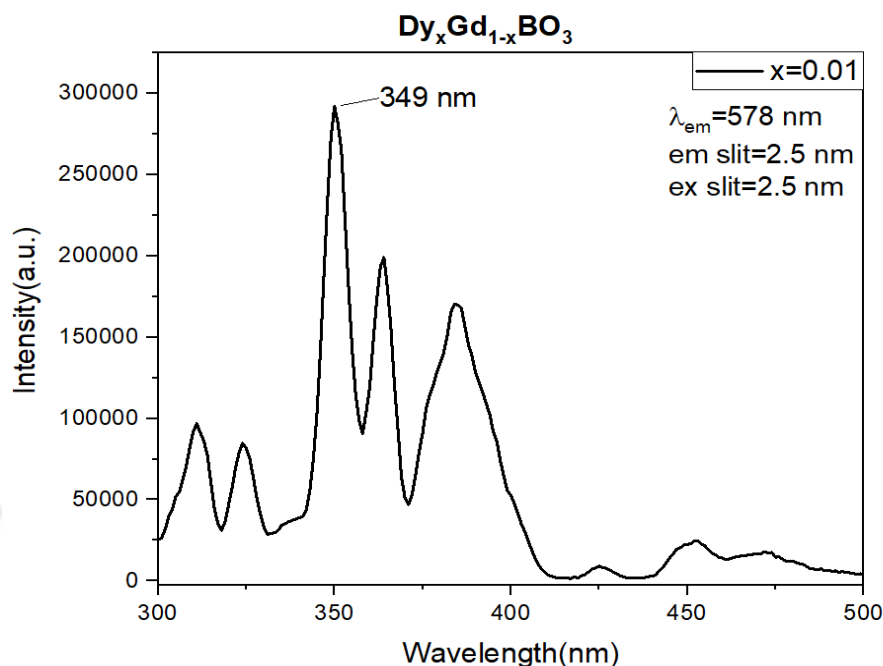
Figure 3.30. The excitation spectrum of \text{Dy}^{3+} single doped \text{GdBO}_3
