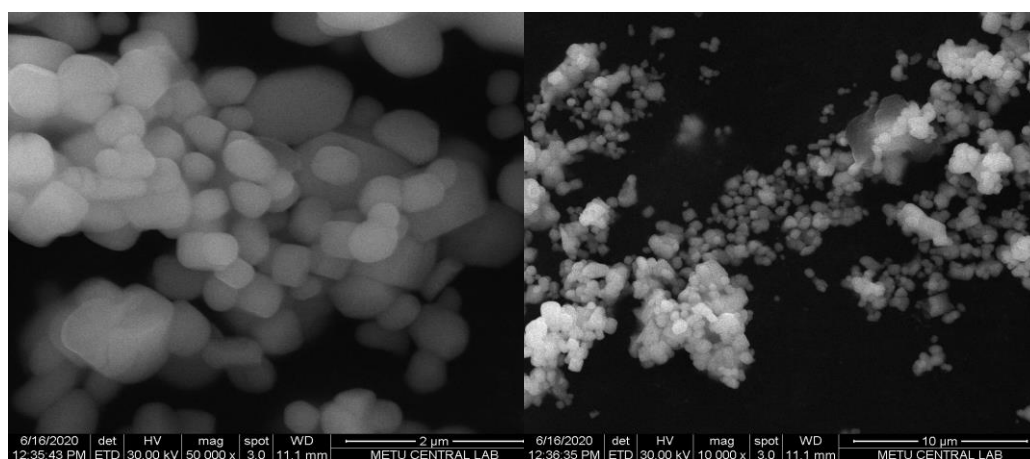
Figure 3.23. SEM images of \text{Ce}^{3+} doped \text{GdBO}_3
