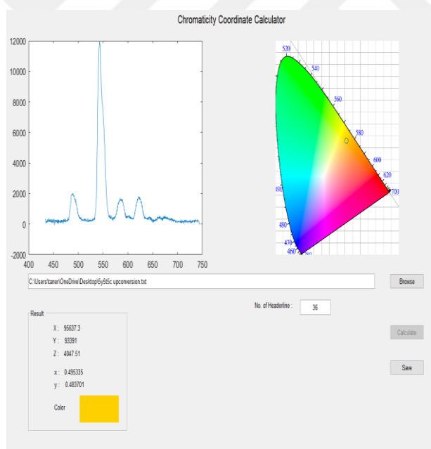
Figure 3.70. CIE calculation of 5% Tb 3+ , 5% Ce 3+ , and 5% Yb 3+ triple doped GdBO 3 with upconversion
