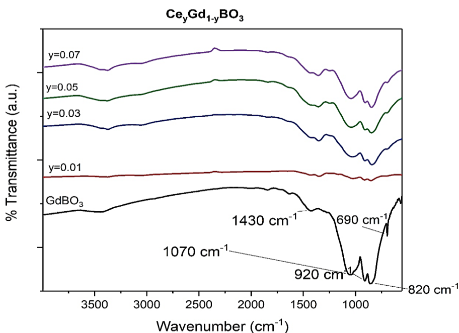
Figure 3.14. FTIR spectra of \text{Ce}^{3+} doped compounds with changing concentration of \text{Ce}^{3+} ( y for \text{Ce}^{3+} )
