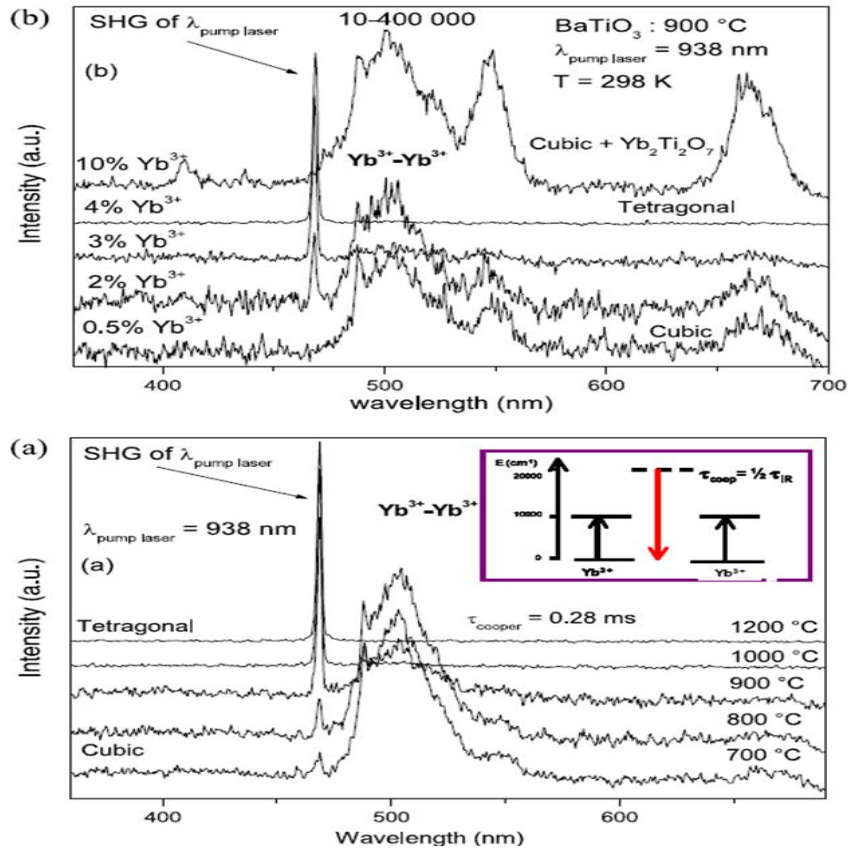
Figure 1.30. Second Harmonic Generation (SGH) signal, the upconversion emission spectrum of rare earth impurities under \text{Yb}^{3+} under pumping in the IR and visible cooperative emission spectrum of \text{Yb}^{3+} ion pairs at room temperature of (a) 1% \text{Yb}^{3+} -doped \text{BaTiO}_3 nano-crystals heated at different temperatures, (b) \text{BaTiO}_3 nanocrystals prepared at 900 °C and doped with varying concentrations of \text{Yb}^{3+} . (Amami et al., 2007)
