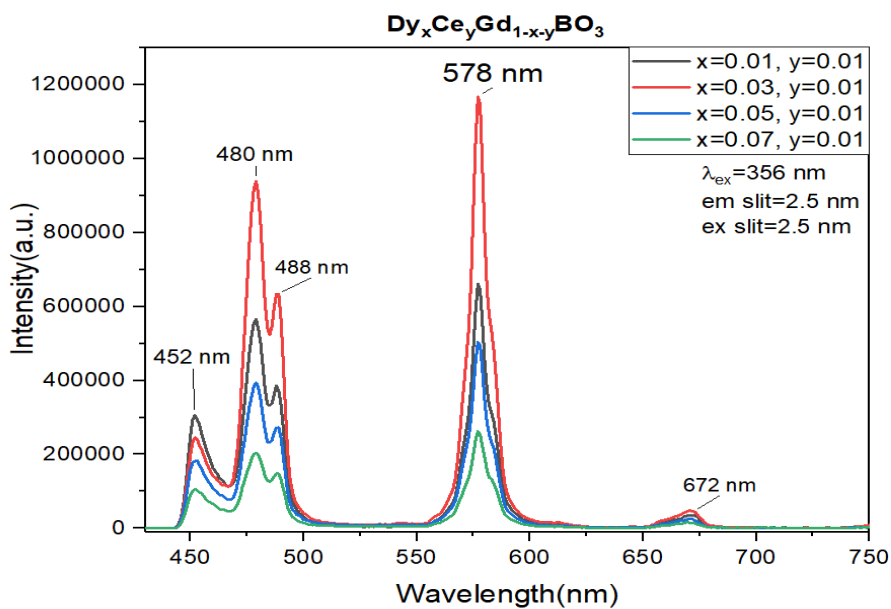
Figure 3.38. Emission spectra of 1% \text{Ce}^{3+} fixed and \text{Dy}^{3+} doped with changing concentration at 331 nm without filter
