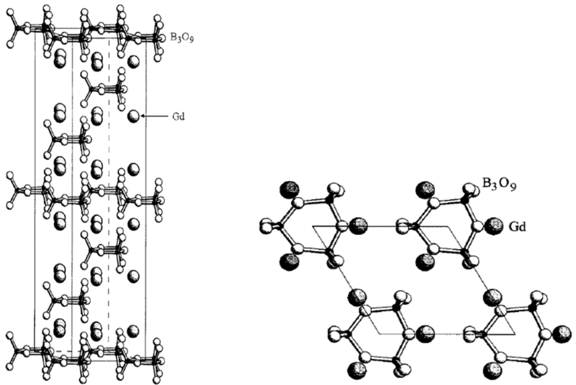
Figure 1.15. Low-Temperature crystal structure of GdBO 3 and B 3 O 9 9- sheets in the structure (Ren et al., 1999)
