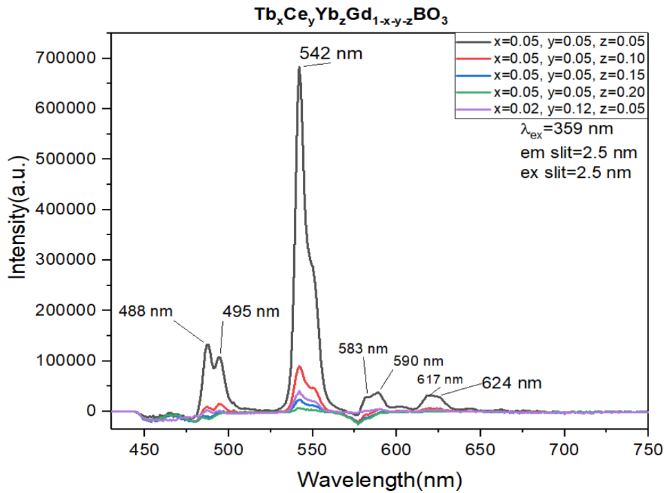
Figure 3.49. Downconversion photoluminescence spectra of triple doped \text{GdBO}_3
