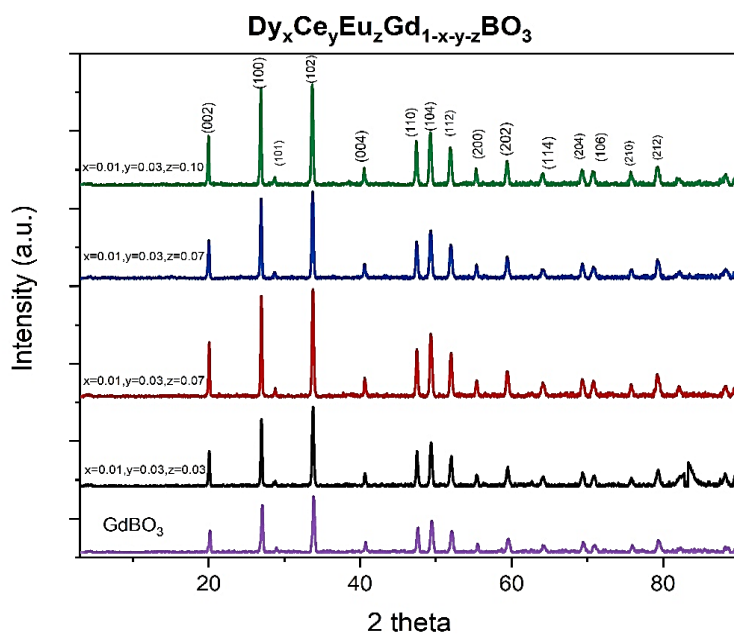
Figure 3.7. XRD patterns of \text{GdBO}_3 with fixed \text{Ce}^{3+} and \text{Dy}^{3+} concentration and changing \text{Eu}^{3+} concentration
