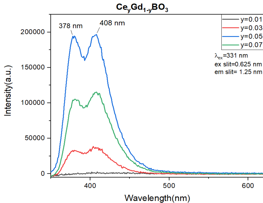
Figure 3.34. Emission spectra of \text{Ce}^{3+} single doped \text{GdBO}_3 with changing concentration at 331-nm excitation without filter
