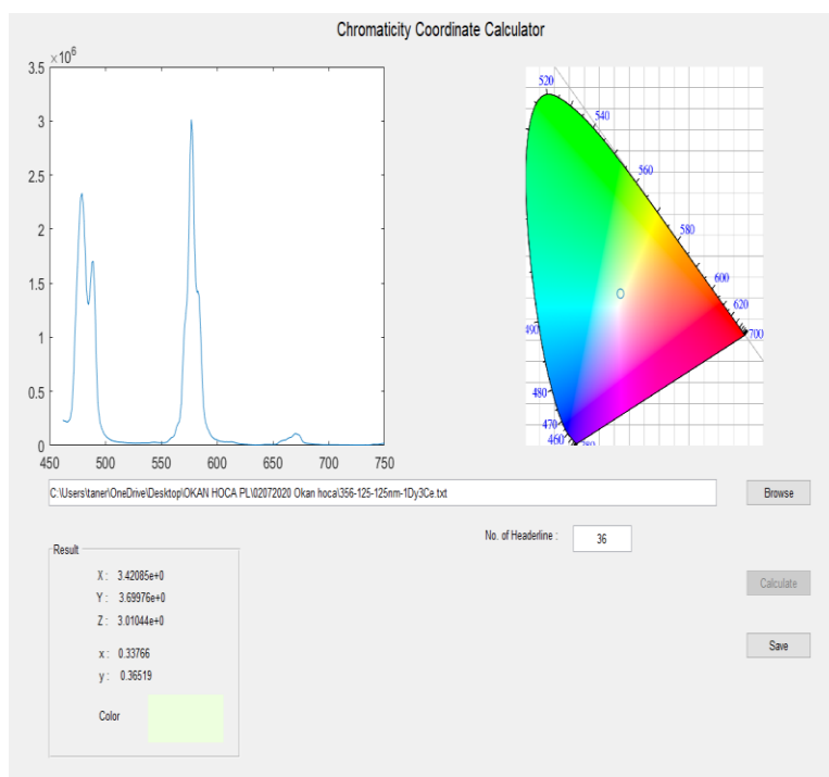
Figure 3.67. CIE calculation of 1% \text{Dy}^{3+} , 3% \text{Ce}^{3+} codoped \text{GdBO}_3
