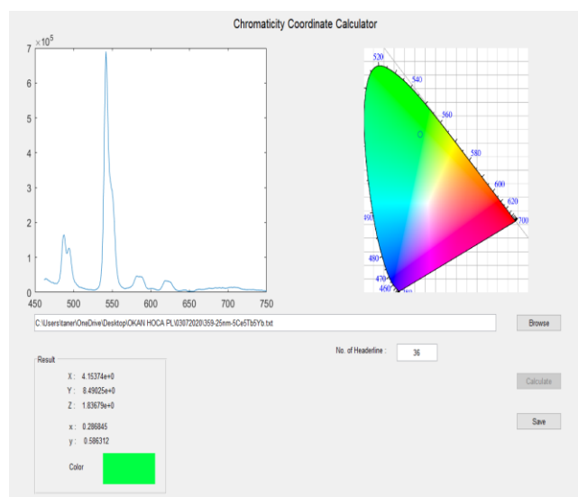
Figure 3.69. CIE calculation of 1% Tb 3+ , 3% Ce 3+ , 1% Yb 3+ triple doped GdBO 3 with downconversion
