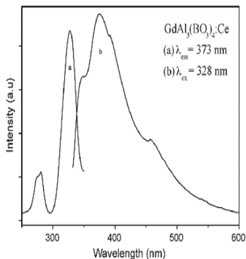
Figure 1.24. Excitation and the emission spectra of \text{Ce}^{3+} ions (C. H. Yang, Y. X. Pan and Q. Y. Zhang, 2007.)
