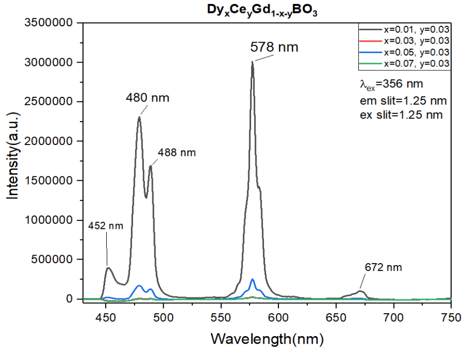
Figure 4.3. Photoluminescence measurement of \text{Ce}^{3+}/\text{Dy}^{3+} codoped \text{GdBO}_3 under Excitation 356 nm with an emission filter
