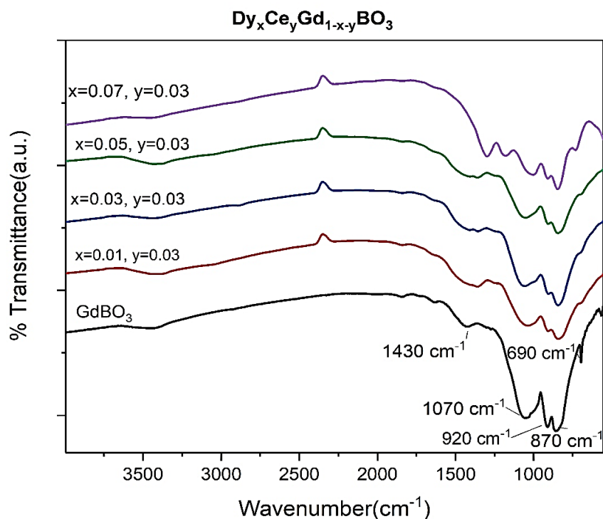
Figure 3.17. FTIR spectra of compounds have 0.03 \text{Ce}^{3+} and changing the concentration of \text{Dy}^{3+} (x for \text{Dy}^{3+} and y for \text{Ce}^{3+} )
