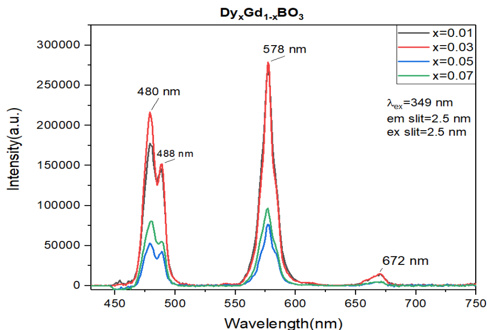
Figure 3.31. Emission spectra of \text{Dy}^{3+} single doped \text{GdBO}_3
