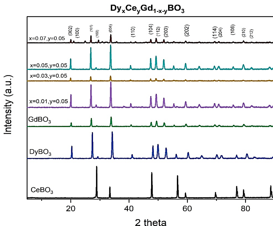
Figure 3.6. X-ray diffraction pattern of compounds have 5% \text{Ce}^{3+} (mol%) and changing concentration of \text{Dy}^{3+} (x for \text{Dy}^{3+} and y for \text{Ce}^{3+} )
