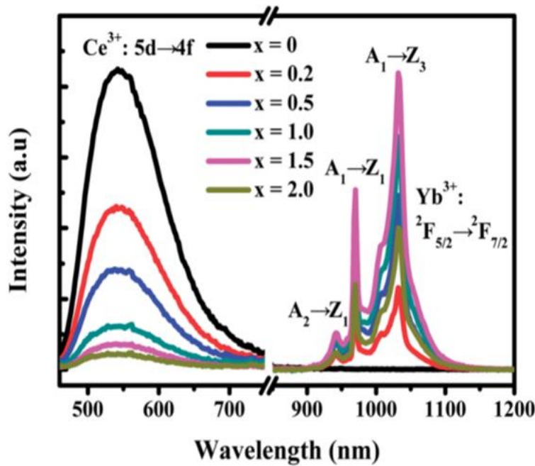
Figure 1.31. Concentration-dependent emission spectra of 0.1 \text{Ce}^{3+} - x\text{Yb}^{3+} codoped glass ceramics ( x=0-2.0 ) (Fang et al., 2014)
