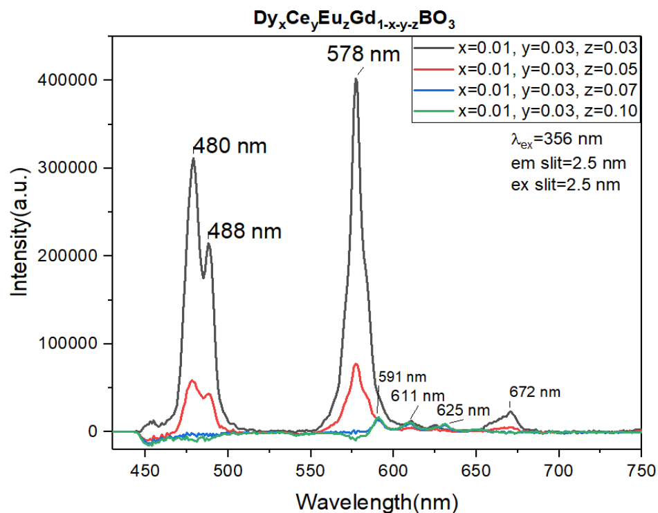
Figure 3.43. Emission spectra of 1% Dy 3+ , 3% Ce 3+ doped and Eu 3+ doped GdBO 3 with changing Eu 3+ concentration at 356-nm excitation
