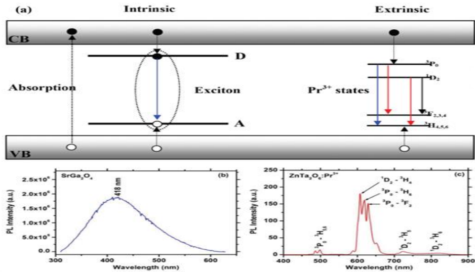
Figure 1.3. (a) The diagram shows emission from both intrinsic and extrinsic defects (b) An emission spectrum and (c) An emission spectrum of \text{ZnTa}_2\text{O}_4:\text{Pr}^{3+} (Luyanda L. Noto, Hendrik C. Swart, Bakang M. Mothudi, 2011)
