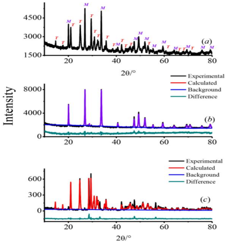
Figure 1.19. (a) is the experimental resulting of synthesized GdBO 3 by hydrothermal method and then annealed at 800 °C, (b) is single-phase monoclinic GdBO 3 , and (c) is a single-phase triclinic GdBO 3 synthesized by polyol method annealed at 800 °C by polyol method. (The markers T and M in the first one show peaks corresponding to the triclinic and monoclinic forms of GdBO 3 )(Nair, Nigam, Sudarsan, Rao, et al., 2018)
