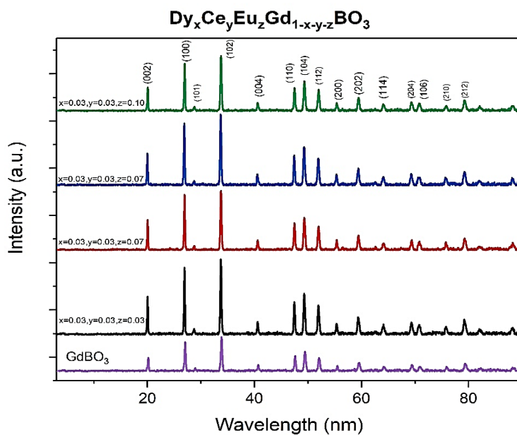
Figure 3.8. XRD patterns of \text{GdBO}_3 with fixed \text{Ce}^{3+} and \text{Dy}^{3+} concentration and changing \text{Eu}^{3+} concentration
