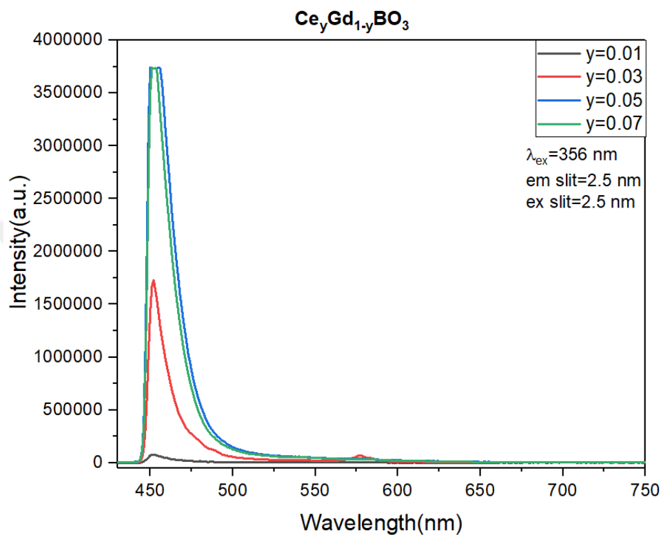
Figure 4.1. Photoluminescence Measurement of \text{Ce}^{3+} Doped \text{GdBO}_3 under 356 nm with filter
