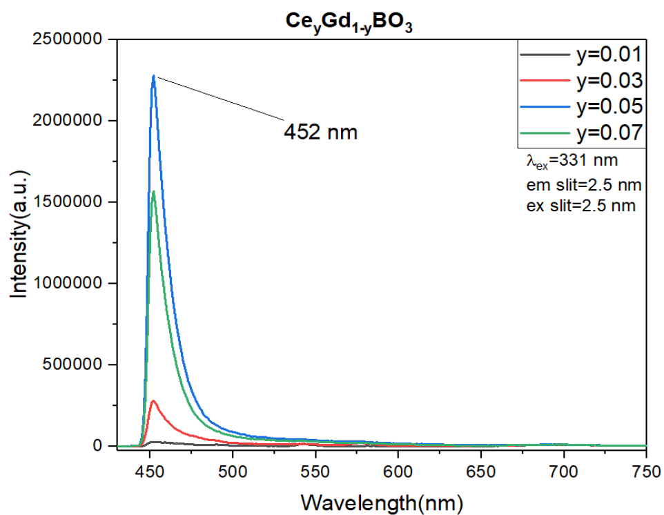
Figure 4.2. Photoluminescence measurement of \text{Ce}^{3+} doped \text{GdBO}_3 under excitation 331 nm
