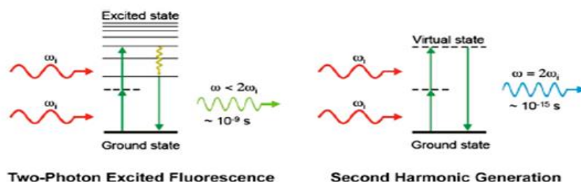
Figure 1.14. The schematic representations of (a) two-photon absorption and (b) second-harmonic generation (Pantazis et al., 2010)
