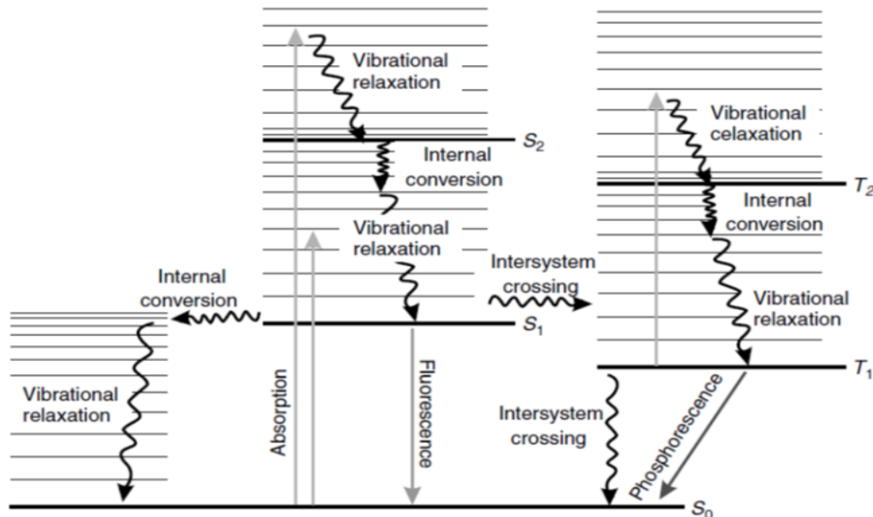
Figure 1.4. Jablonski diagram (Sauer, Hofkens, & Enderlein, 2011).
