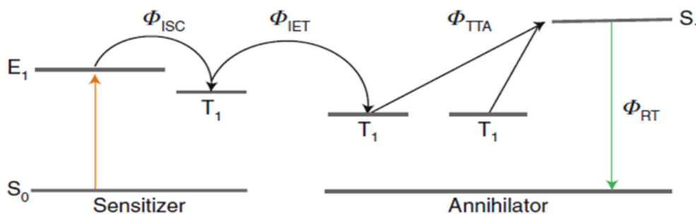
Figure 1.11. Schematic representation of TTA upconversion (ISC: intersystem crossing, IET: interface energy transfer, TTA: triplet-triplet annihilation, RT: radiative transfer) (Wen et al., 2019)
