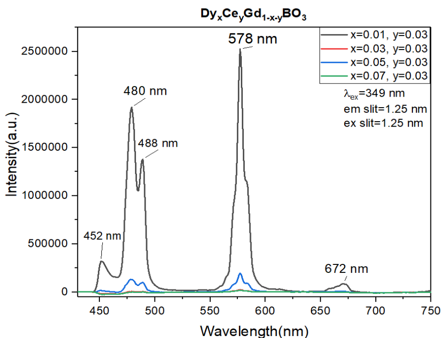
Figure 3.39. Emission spectra of 3% \text{Ce}^{3+} fixed and \text{Dy}^{3+} doped with changing concentration at 349 nm
