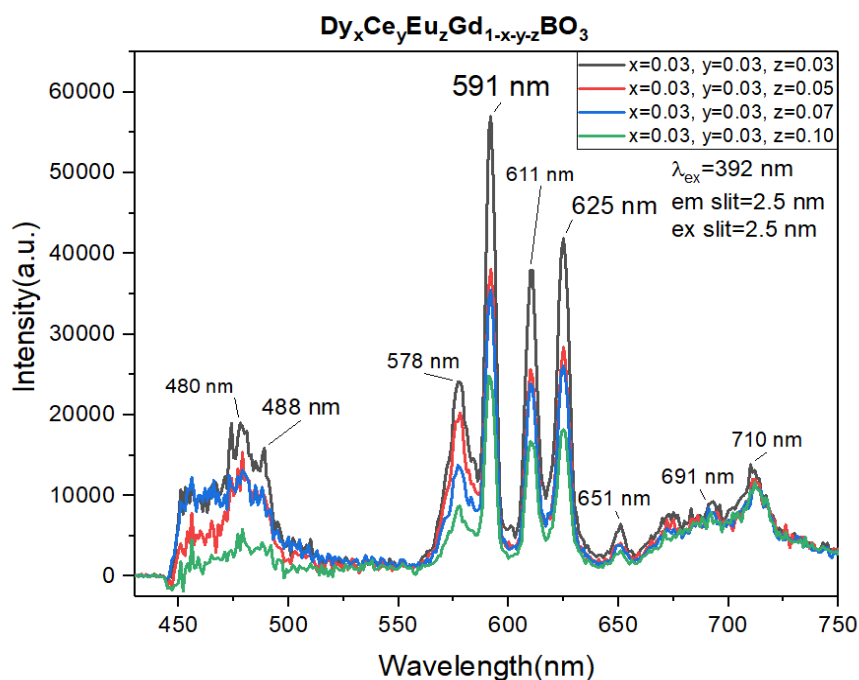
Figure 3.47. Emission spectra of 3% Dy 3+ , 3% Ce 3+ doped and Eu 3+ doped GdBO 3 with changing Eu 3+ concentration at 392-nm excitation
