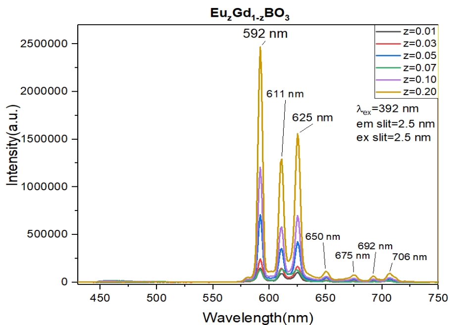
Figure 3.36. Emission spectra of Eu 3+ single doped GdBO 3 at 392 nm
