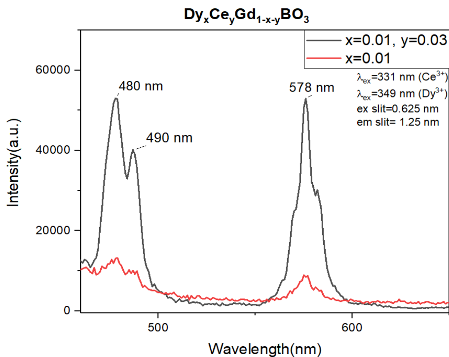
Figure 4.4. Photoluminescence measurements of \text{Dy}^{3+} doped under excitation and \text{Ce}^{3+}/\text{Dy}^{3+} Cooped \text{GdBO}_3 under Excitation 331 nm
