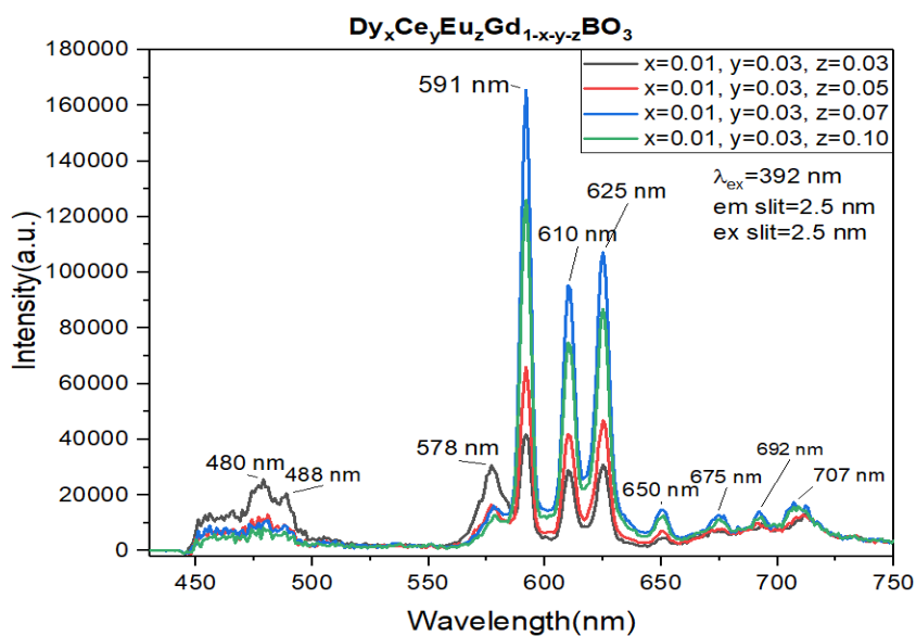
Figure 3.44. Emission spectra of 1% Dy 3+ , 3% Ce 3+ doped and Eu 3+ doped GdBO 3 with changing Eu 3+ concentration at 392-nm excitation
