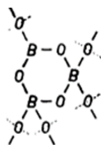
The di-triborate group ( ac_2 ), observed in the compound K_2O \cdot 2 B_2O_3 .
