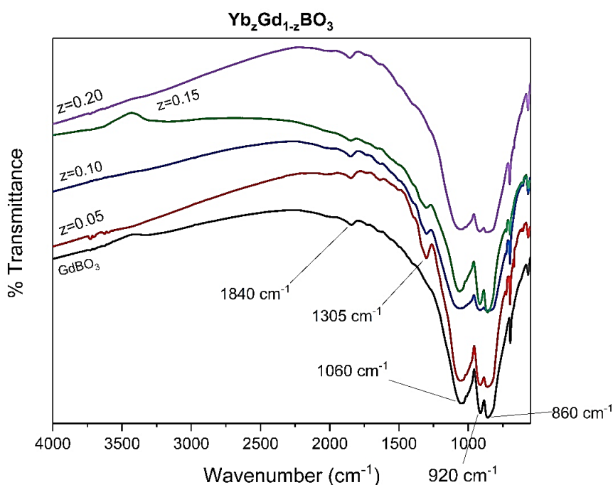
Figure 3.21. FTIR spectra of \text{GdBO}_3 with changing \text{Yb}^{3+} concentration
