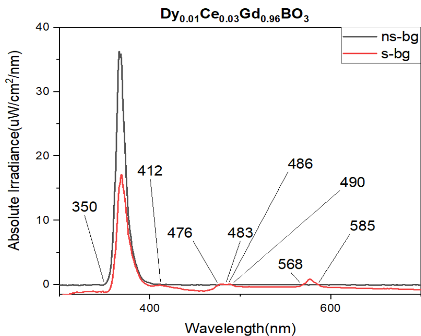
Figure 3.63. Absorption and emission regions used for the calculation of 0.01 Dy 3+ -0.03 Ce 3+ doped (in terms of mole)
