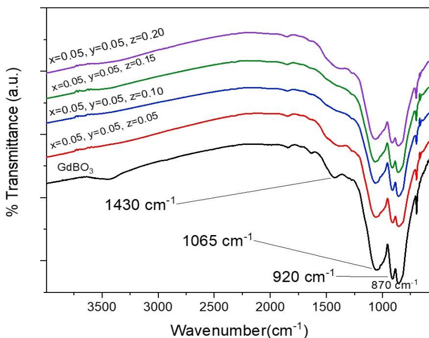
Figure 3.22. FTIR spectra of \text{GdBO}_3:0.05\text{Tb}, 0.05\text{Ce} with changing \text{Yb}^{3+} concentration
