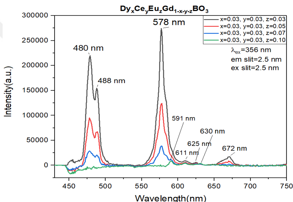
Figure 3.46. Emission spectra of 3% \text{Dy}^{3+} , 3% \text{Ce}^{3+} doped and \text{Eu}^{3+} doped \text{GdBO}_3 with changing \text{Eu}^{3+} concentration at 356-nm excitation
