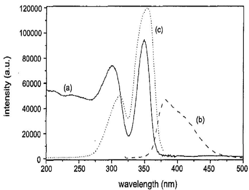
Figure 1.26. Optical characteristics of \text{Lu}_2\text{Si}_2\text{O}_7:\text{Ce} single crystals: (a) absorption spectrum, (b) emission spectrum, (c) fluorescence excitation spectrum (under 400 nm wavelength)(Pauwels et al., 2000)
