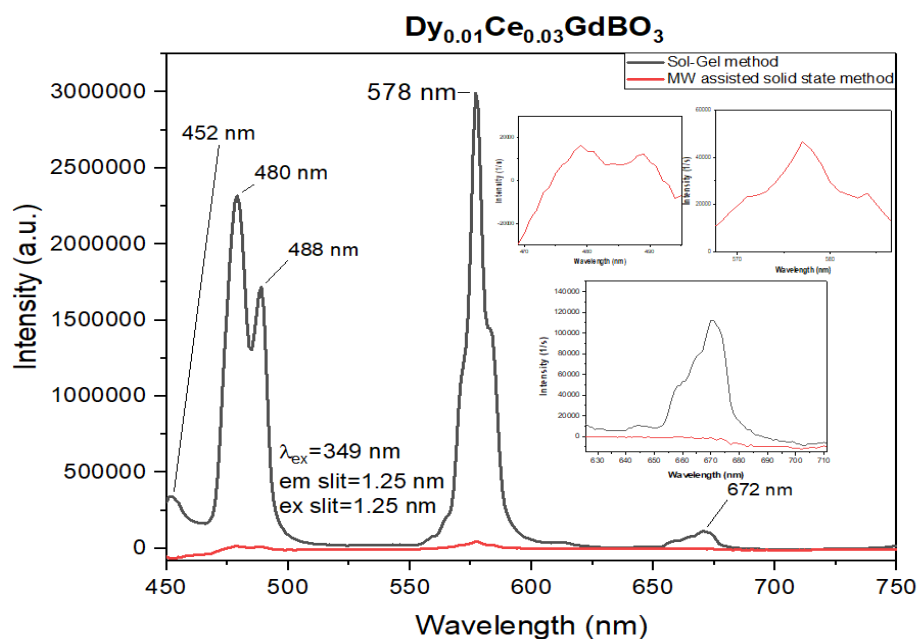
Figure 3.54. Emission spectra of the 1% Dy 3+ -3% Ce 3+ codoped GdBO 3 synthesized with sol-gel and microwave assisted solid-state method at 349 nm
