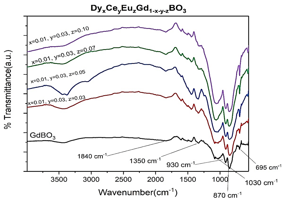
Figure 3.19. FTIR spectra of \text{GdBO}_3:0.01\text{Dy}, 0.03\text{Ce} with changing \text{Eu}^{3+} concentration
