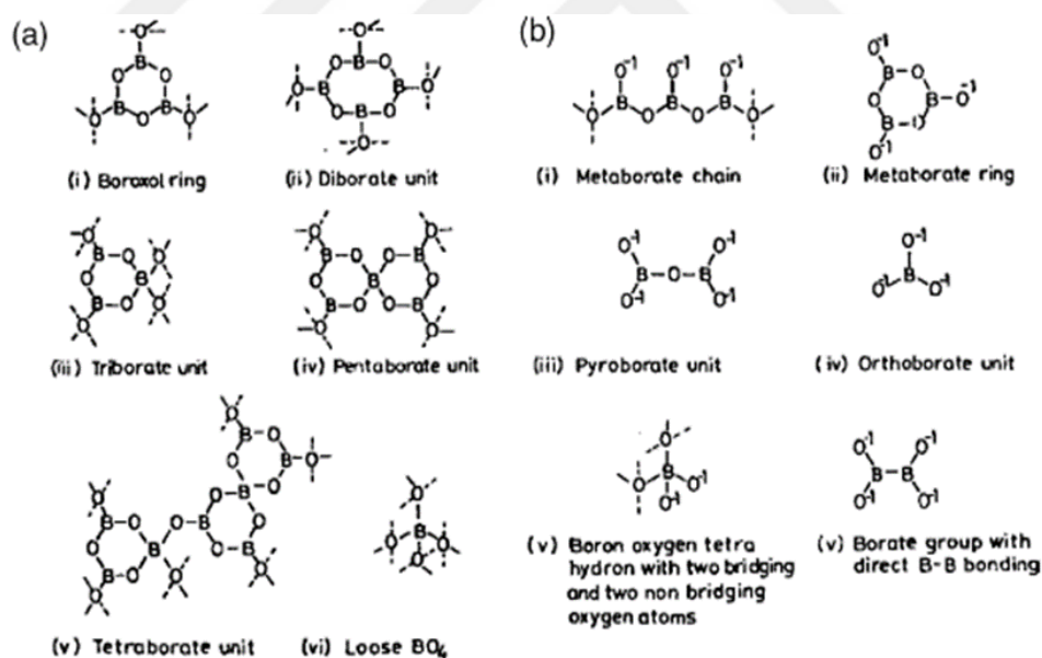
Figure 3.11. Some borate groups (Edukondalu et al., 2014)
