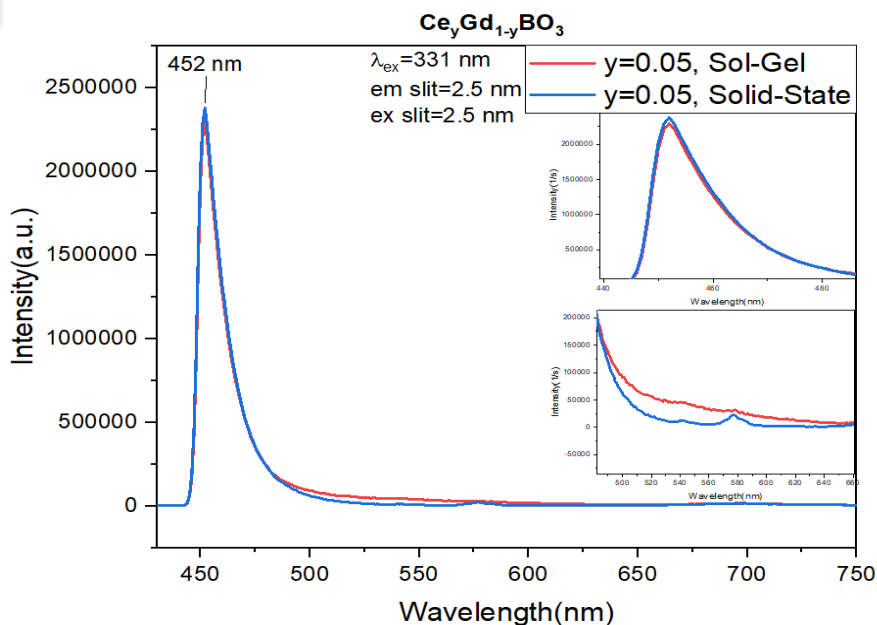
Figure 3.52. Emission spectra of 5% \text{Ce}^{3+} doped \text{GBO}_3 synthesized with sol-gel and microwave assisted solid-state methods
