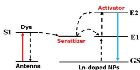
Figure 1.12. Schematic representation of dye-sensitized upconversion process (Duan et al., 2018)
