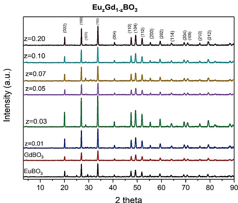
Figure 3.3. XRD patterns of \text{Eu}^{3+} doped \text{GdBO}_3 ( z for \text{Eu}^{3+} )
