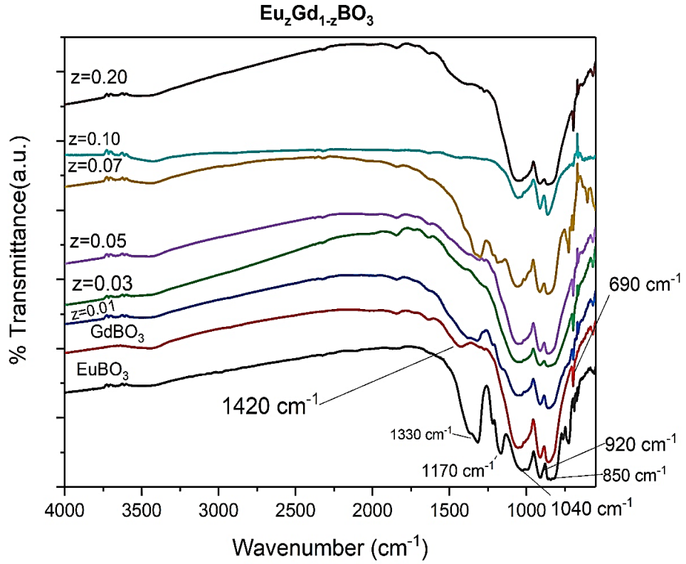
Figure 3.15. FTIR spectra of \text{Eu}^{3+} doped compounds with changing \text{Eu}^{3+} concentration ( z for \text{Eu}^{3+} )
