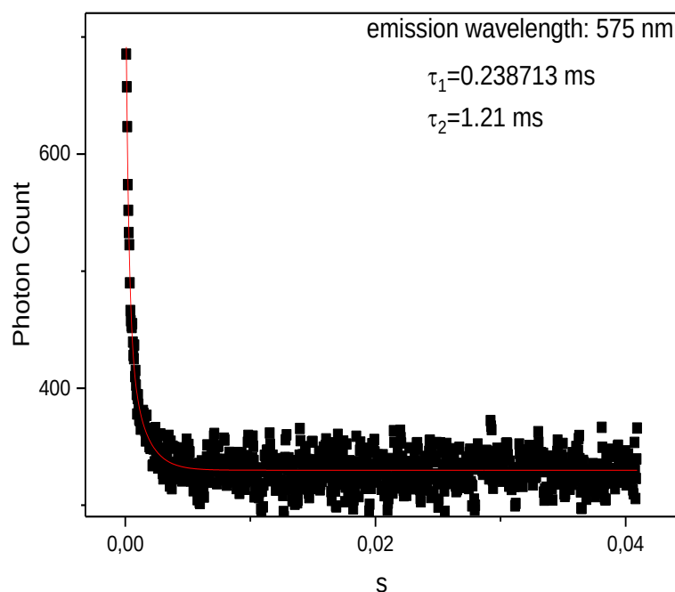
Figure 3.58. Decay curve of 1% Dy 3+ /3% Ce 3+ doped GdBO 3 at 575 nm
