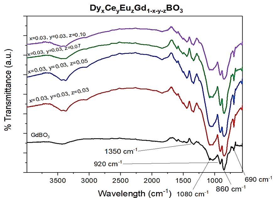
Figure 3.20. FTIR spectra of \text{GdBO}_3:0.01\text{Dy}, 0.03\text{Ce} with changing \text{Eu}^{3+} concentration
