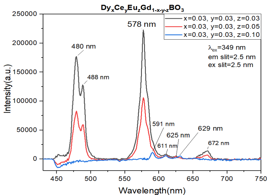
Figure 3.45. Emission spectra of 3% Dy 3+ , 3% Ce 3+ doped and Eu 3+ doped GdBO 3 with changing Eu 3+ concentration at 349-nm excitation
