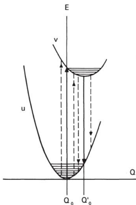
Figure 1.7. Representation of configurational coordinate diagram.
