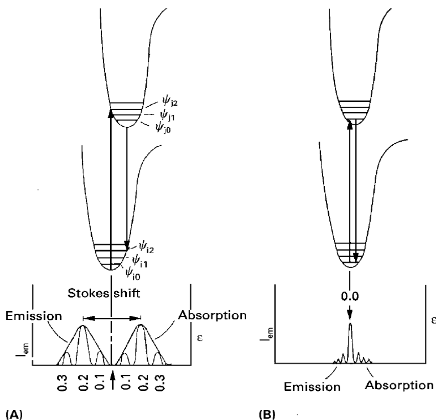
Figure 1.8. Potential energy diagrams for two cases of excited state distortions: (A) non-zero distortion and (B) zero distortion.
