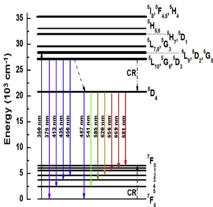
Figure 1.28. Energy level diagram of Terbium ion (Juárez-Batalla, Meza-Rocha, Muñoz, Camarillo, & Caldiño, 2016)
