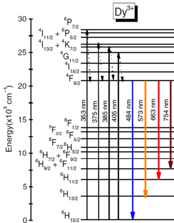
Figure 1.23. Emission wavelengths of \text{Dy}^{3+} ion (Alves et al., 2016)
