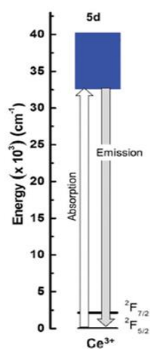
Figure 1.25. Energy level diagram of \text{Ce}^{3+} ion (Shrivastava et al., 2017)
