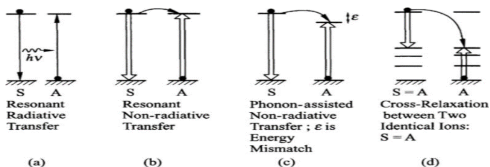
Figure 1.9. Energy transfer processes: (a) Resonant Radiative Transfer, (b) Resonant Non-radiative Transfer, (c) Phonon-assisted Non-radiative Transfer, (d) Cross-Relaxation between Two Identical Ions (A is for activator and S is for sensitizer) (Q. Y. Zhang & Huang, 2010)
