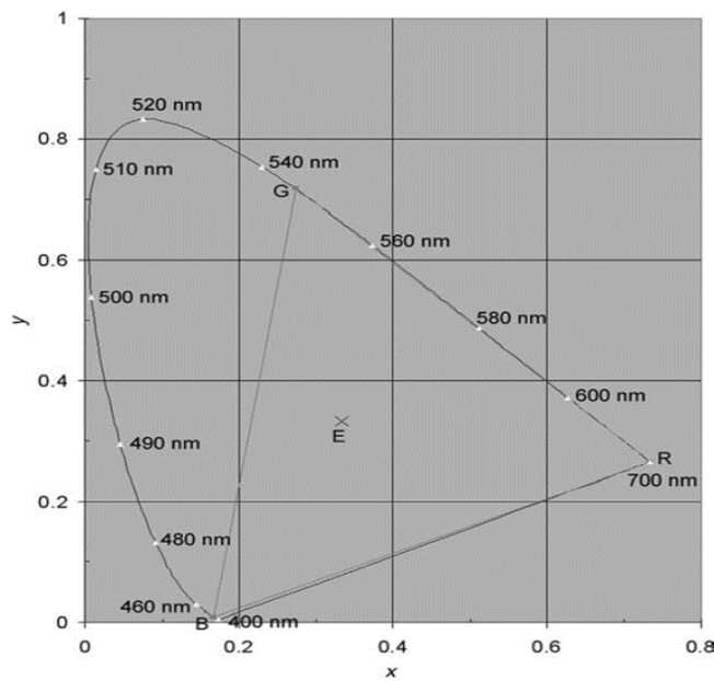
Figure 1.32. x, y chromaticity diagram of the CIE 1931 trichromatic system. The triangle shown refers to the R, G, B primaries put to use to define the CIE trichromatic system.
