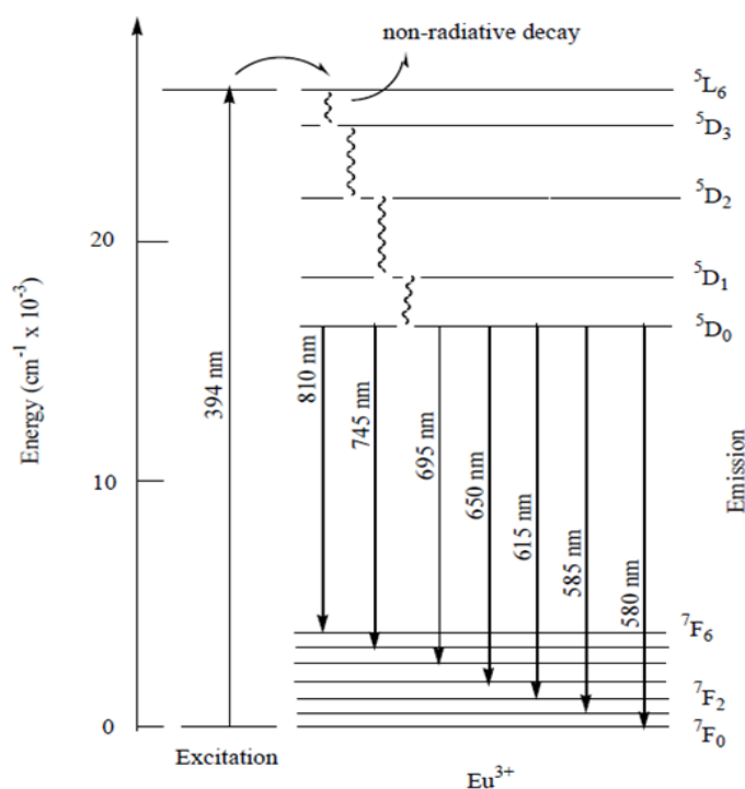
Figure 1.27. Energy level diagram of \text{Eu}^{3+} (Nassar et al., 2009)
