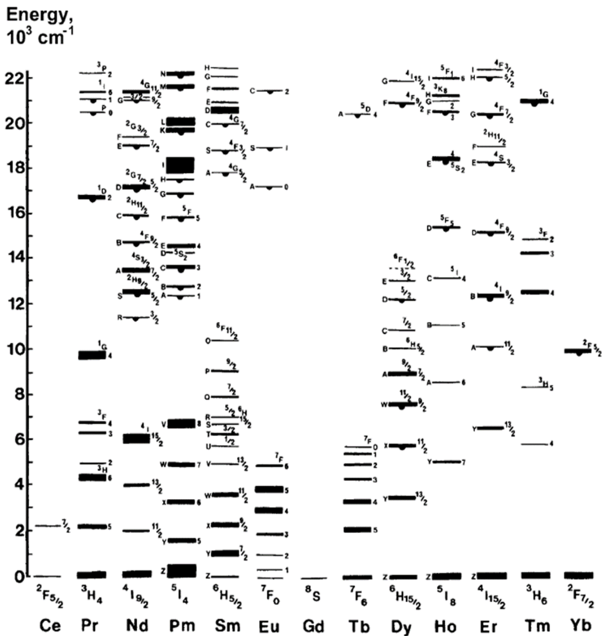
Figure 1.22. Dieke diagram (rare-earth ions in LaCl 3 ) (Sorokina, 2003)
