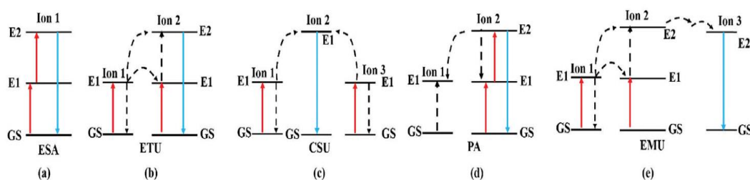
Figure 1.13. Upconversion processes for Ln-doped UCNPs. GS: ground state; E1 and E2: excited states: ESA: excited-state absorption; ETU: energy transfer upconversion; CSU: cooperative sensitization upconversion; PA: photon avalanche; EMU: energy migration upconversion(Duan et al., 2018)
