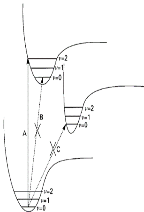
Figure 1.6. The Franck-Codon principle. Only the vertical electronic transition is allowed.
