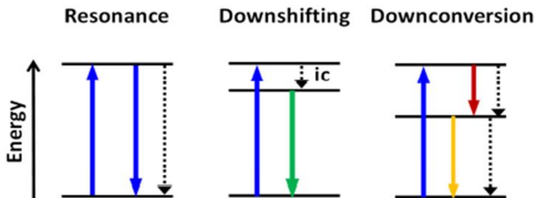
Figure 1.10. Energy diagram which describes resonance, downshifting, and downconversion (Devi, Devi, & Singh, 2020)
