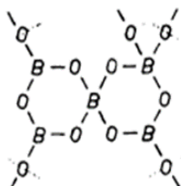
The di-pentaborate group ( a_3c_2 ), observed in the compound Na_2O \cdot 2 B_2O_3 .
