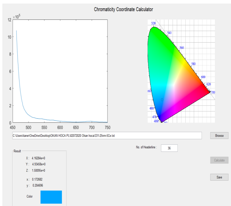
Figure 3.65. CIE calculation of 5% \text{Ce}^{3+} doped \text{GdBO}_3
