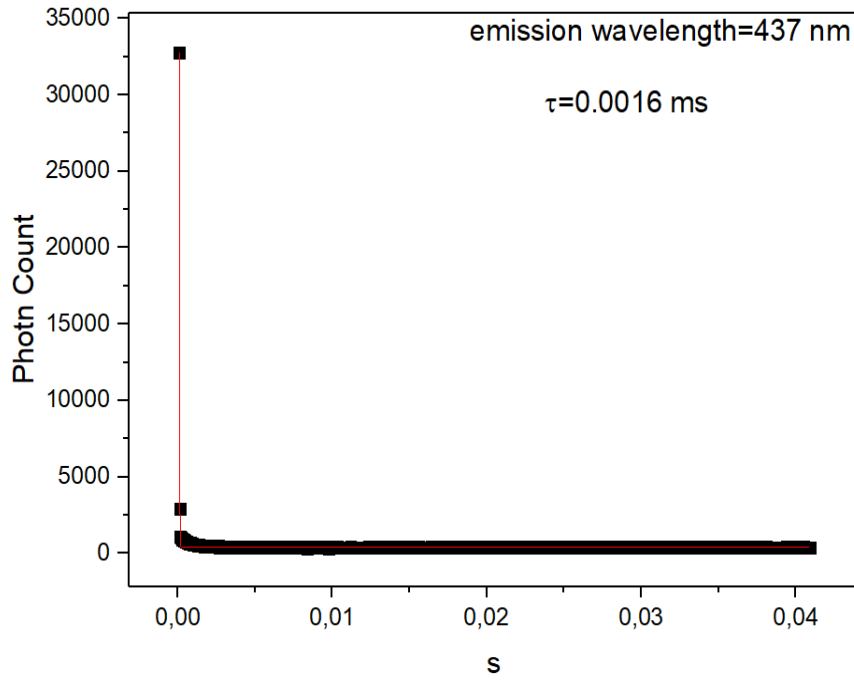
Figure 3.57. Decay curve of 1% Dy 3+ /3% Ce 3+ doped GdBO 3 at 437 nm
