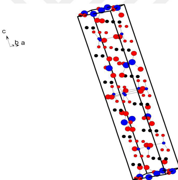
Figure 1.18. Representation of the crystal structure of GdBO 3 (black ones are Gd 3+ , blue ones are B 3+ and red ones are O 2- ions) (SEYYİDOĞLU, 2009)
