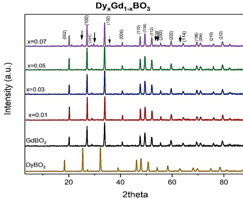
Figure 3.1. XRD patterns of \text{Dy}^{3+} doped \text{GdBO}_3 ( x for \text{Dy}^{3+} )
