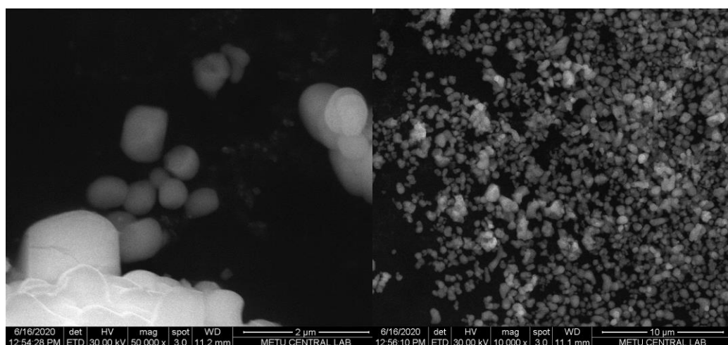
Figure 3.25. SEM images of \text{Eu}^{3+} doped \text{GdBO}_3
