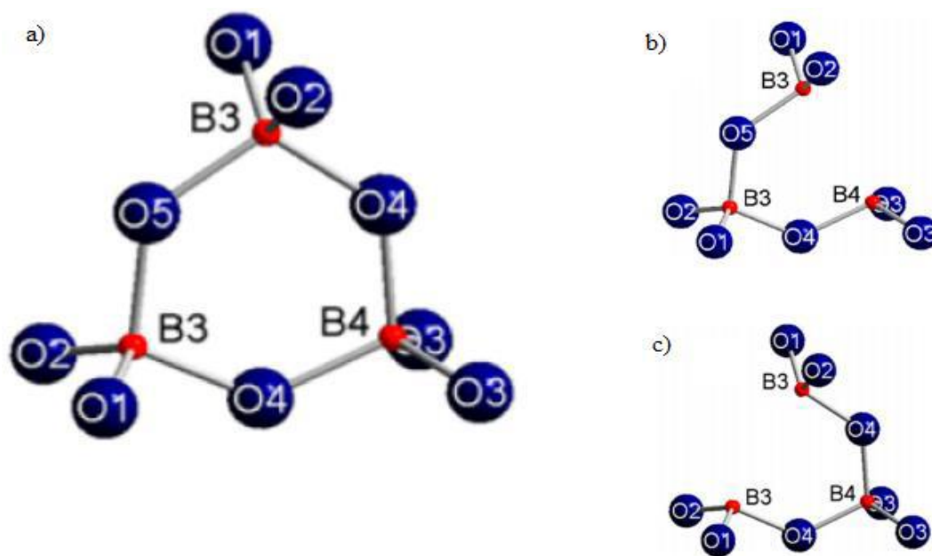
Figure 3.12. a) B_3O_9^{9-} ring (b and c) coordination spheres of the B cations without one O4 or O5
