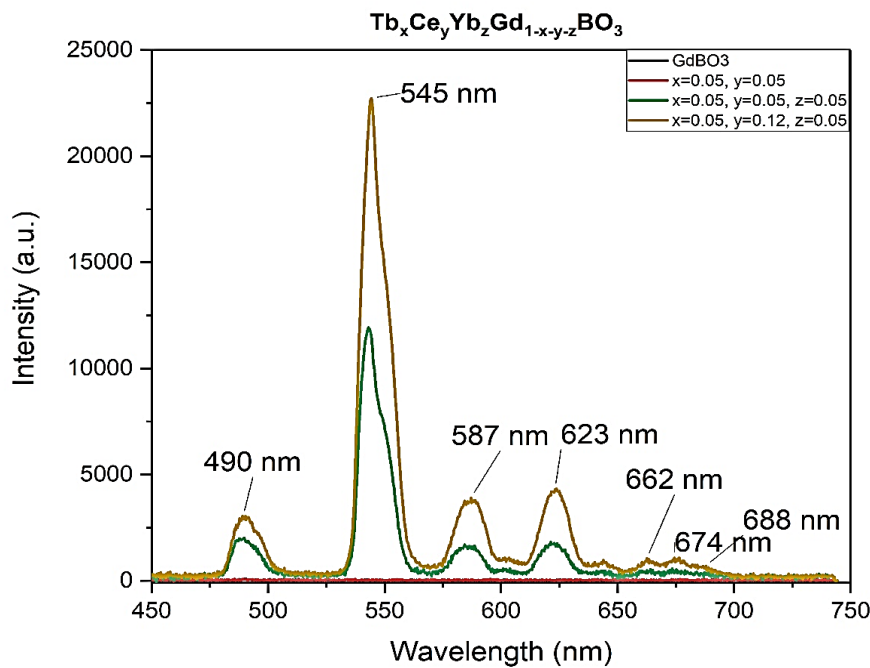
Figure 3.51. Upconversion photoluminescence spectra of triple doped \text{GdBO}_3
