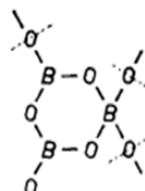
The triborate group with one non-bridging oxygen ion ( abc ), observed in the compound Na_2O \cdot 2 B_2O_3 .
