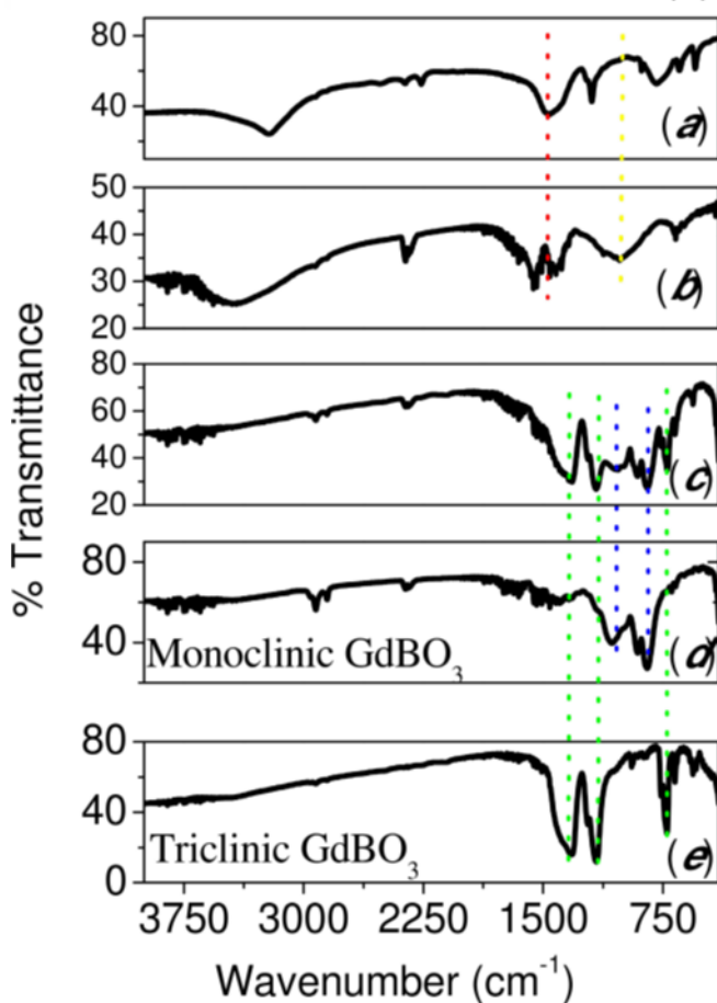
Figure 1.20. FTIR measurements of (a) boric acid (b) as prepared sample obtained by hydrothermal method, (c) as prepared sample subjected to annealing at 400 °C, (d) single-phase monoclinic \text{GdBO}_3 , and (e) single-phase triclinic \text{GdBO}_3
