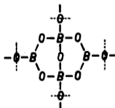
The diborate group ( a_2c_2 ), observed in the compound \text{Li}_2\text{O} \cdot 2 B_2O_3 .
