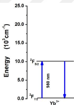
Figure 1.29. Energy state diagram of \text{Yb}^{3+} ion (Sun et al., 2014)
