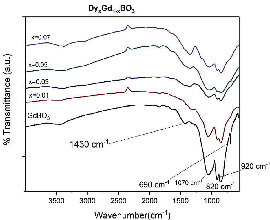
Figure 3.13. FTIR spectra of \text{Dy}^{3+} doped phosphors with changing concentration of \text{Dy}^{3+} ( x for \text{Dy}^{3+} )
