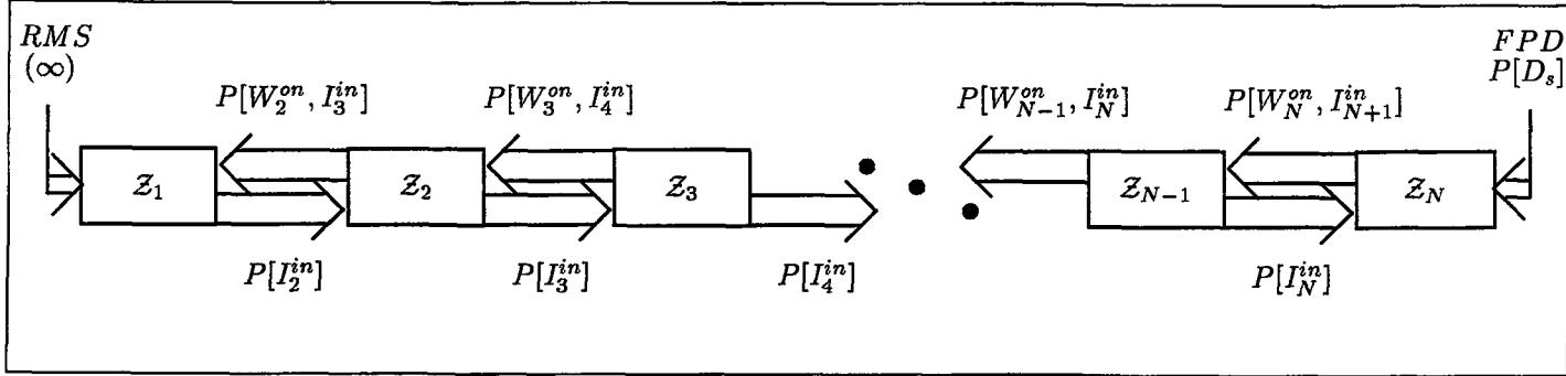
Figure 3.3: Model of the production system constituted from models of isolated single-stage sub-systems. RMS(\infty) denotes the infinite supply of raw material and FPD P[D_s] denotes the external finished product demand.
