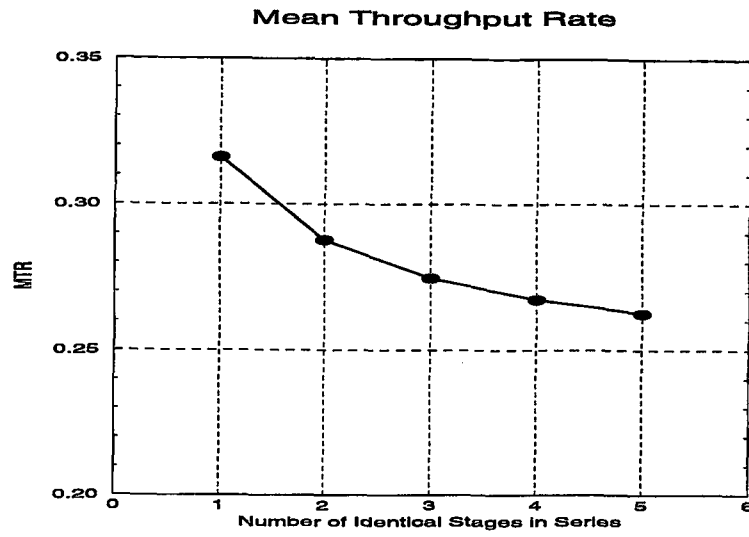
Figure A.1: Increasing the number of identical stages in series, decreases the mean throughput rate of the system with a decreasing rate.
