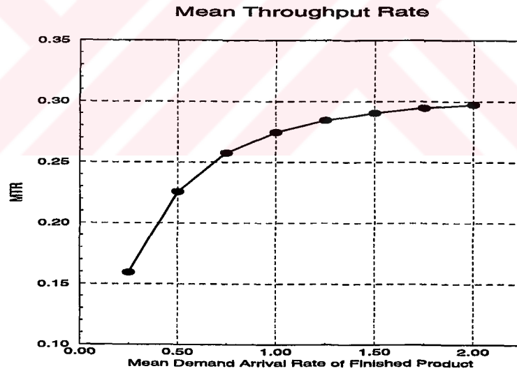
Figure A.2: Increasing mean demand arrival rate of finished product, increases the mean throughput rate of the system with a decreasing rate.
