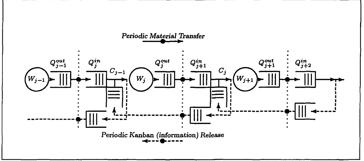
Figure 3.2: An isolated single-stage pull production subsystem Z_j .
