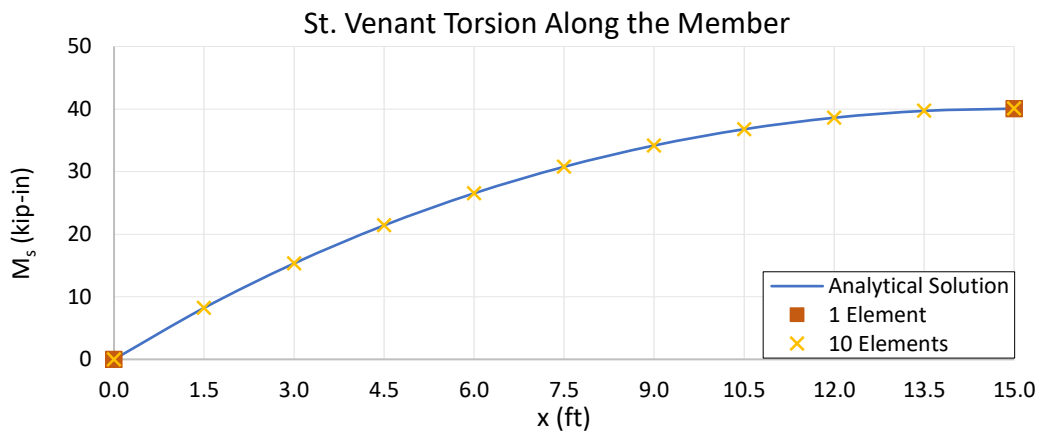
Figure 3-4 Verification Problem 1: St. Venant torsion along the member.
