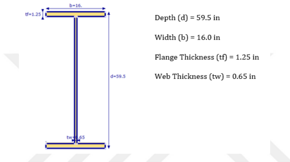
Figure 4-1 Straight Exterior Girder: Cross-sectional dimensions.
