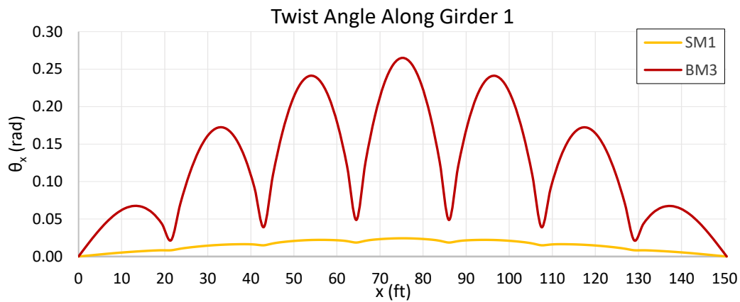
Figure 4-27 Twist angle along Girder 1 for models SM1 and BM3.
