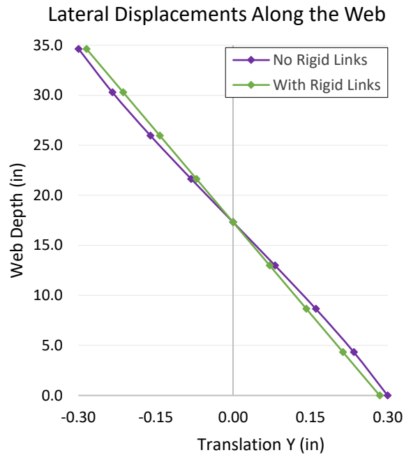
Figure 3-10 Shell Model 3: Lateral displacements along the web.
