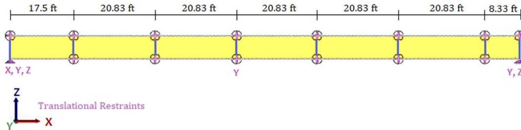
Figure 4-3 Side View: Cross-frame locations.
