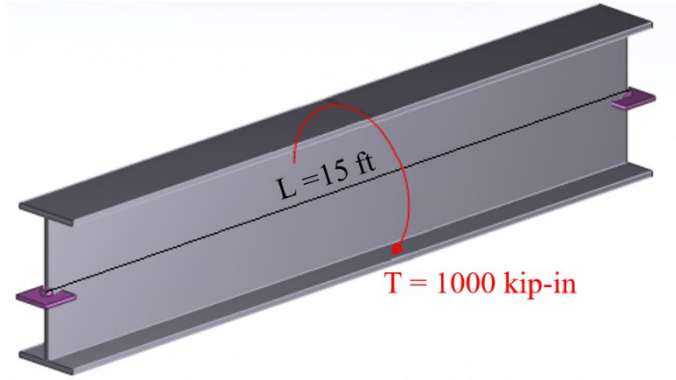
Figure 3-18 Geometry of Verification Problem 2.
