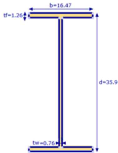
Figure 3-1 Cross-sectional dimensions of the example section.
