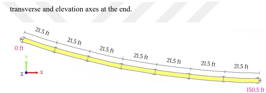
Figure 4-15 Plan View: Cross-frame locations.
