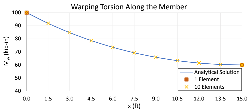
Figure 3-5 Verification Problem 1: Warping torsion along the member.
