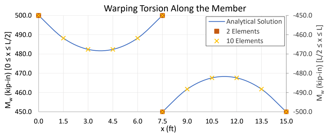
Figure 3-21 Verification Problem 2: Warping torsion along the member.
