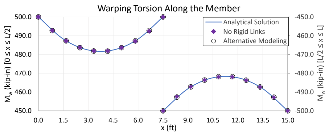
Figure 3-25 Shell Models: Warping torsion along the member.
