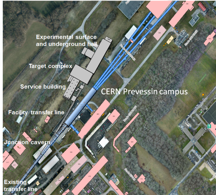
Figure 3.1: Location of the facility
