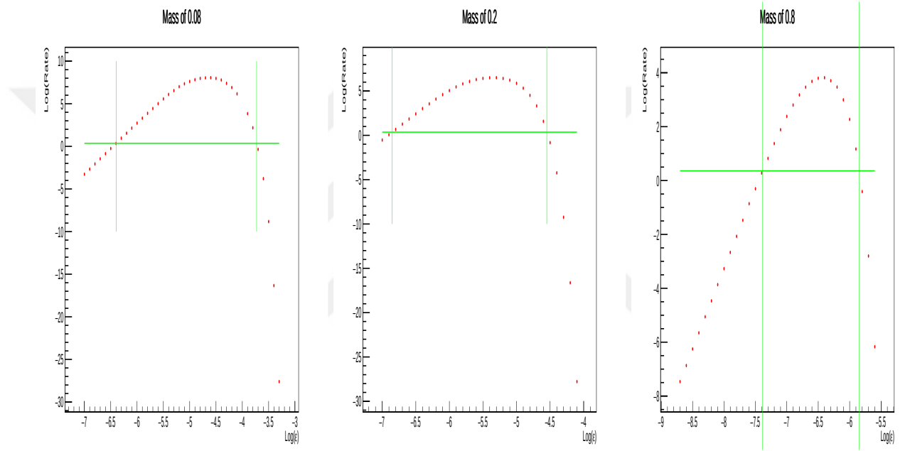
Figure 5.11: The lower and upper limits of g_{a\gamma} (vertical green lines) for three different m_a values.
