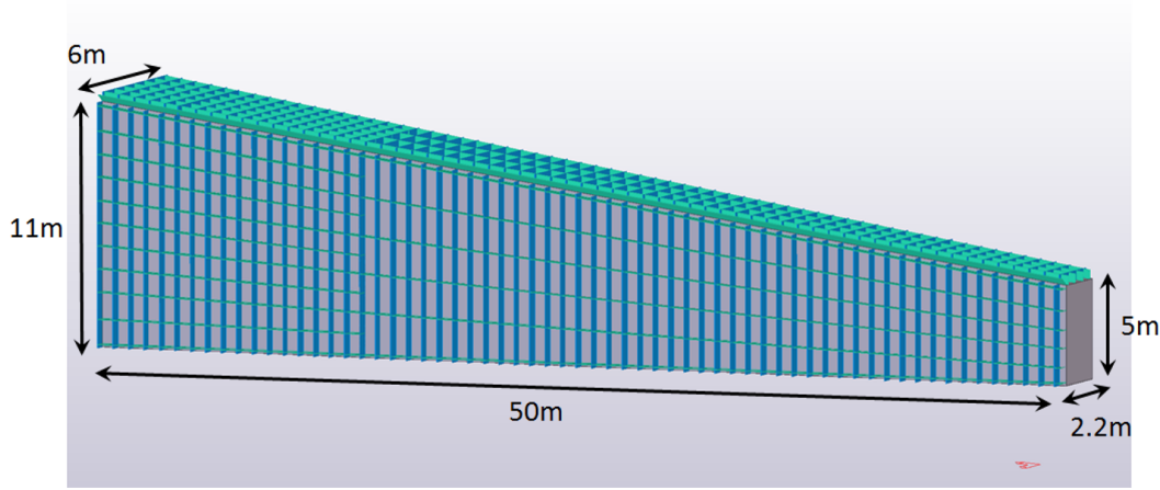
Figure 3.5: Schematic of decay vessel
