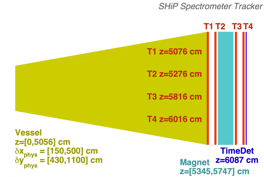
Figure 3.9: Positions of the tracking stations along the beam axis(z)
