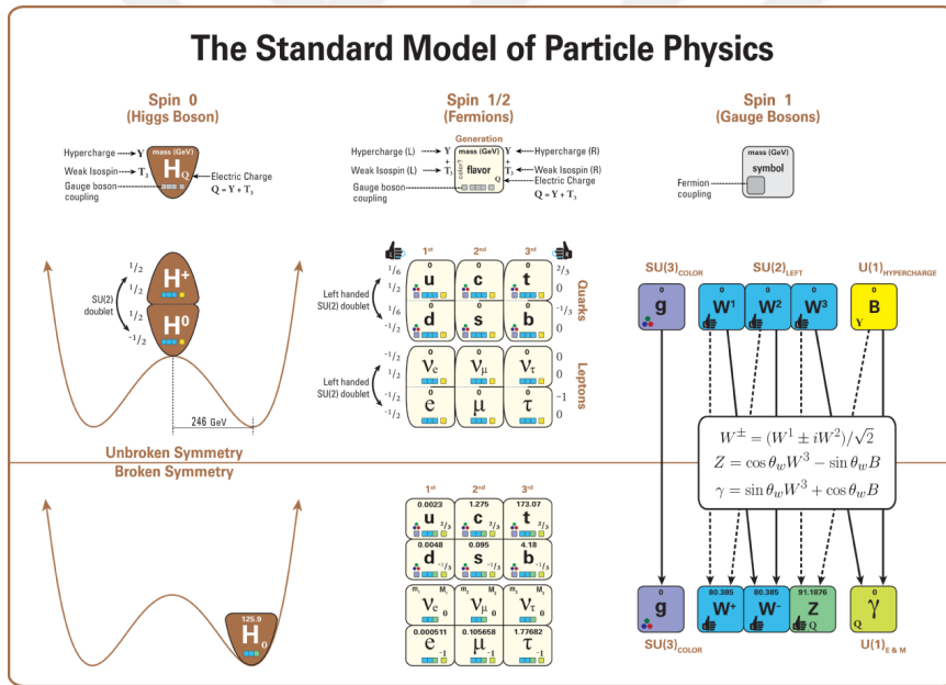
Figure 2.1: (Un)broken symmetries of the Standard Model
