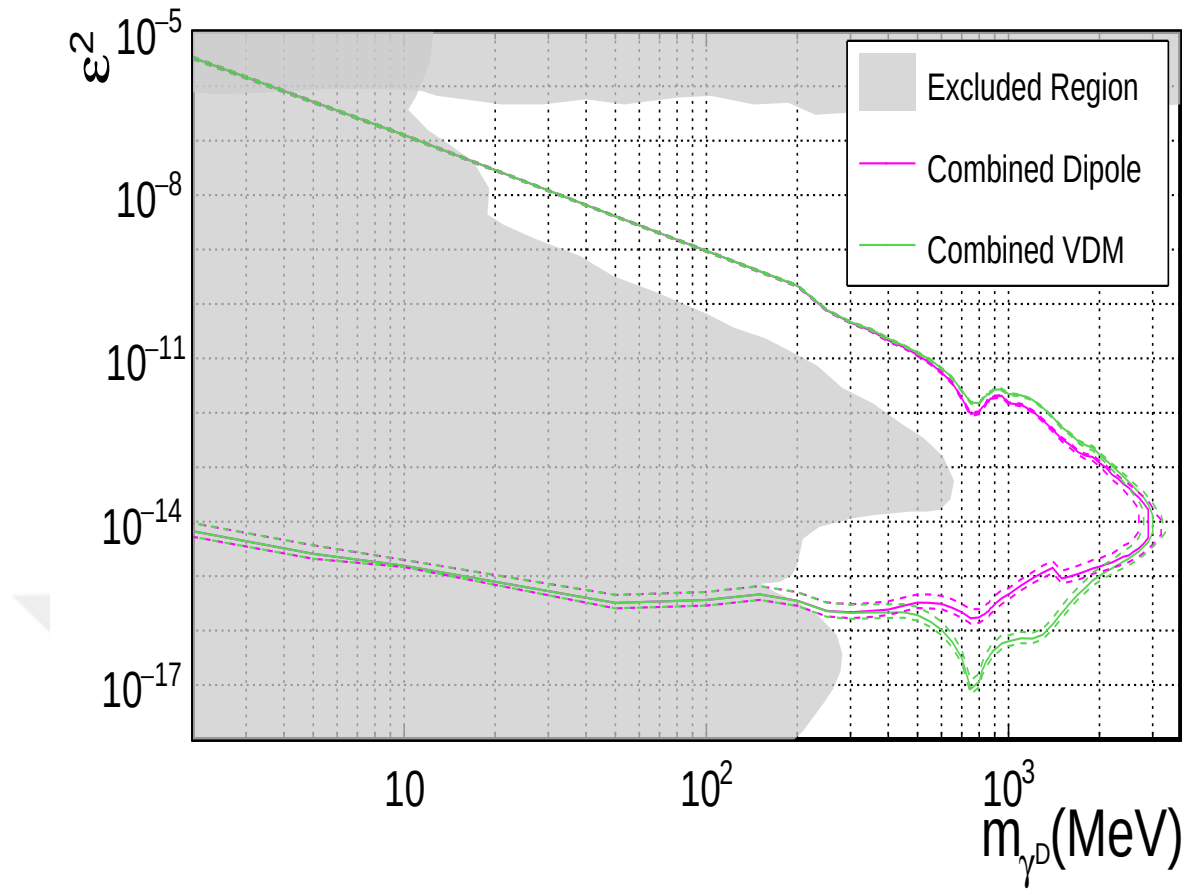
Figure 6.2: The combined exclusion contour for the dark photon search at SHiP.
