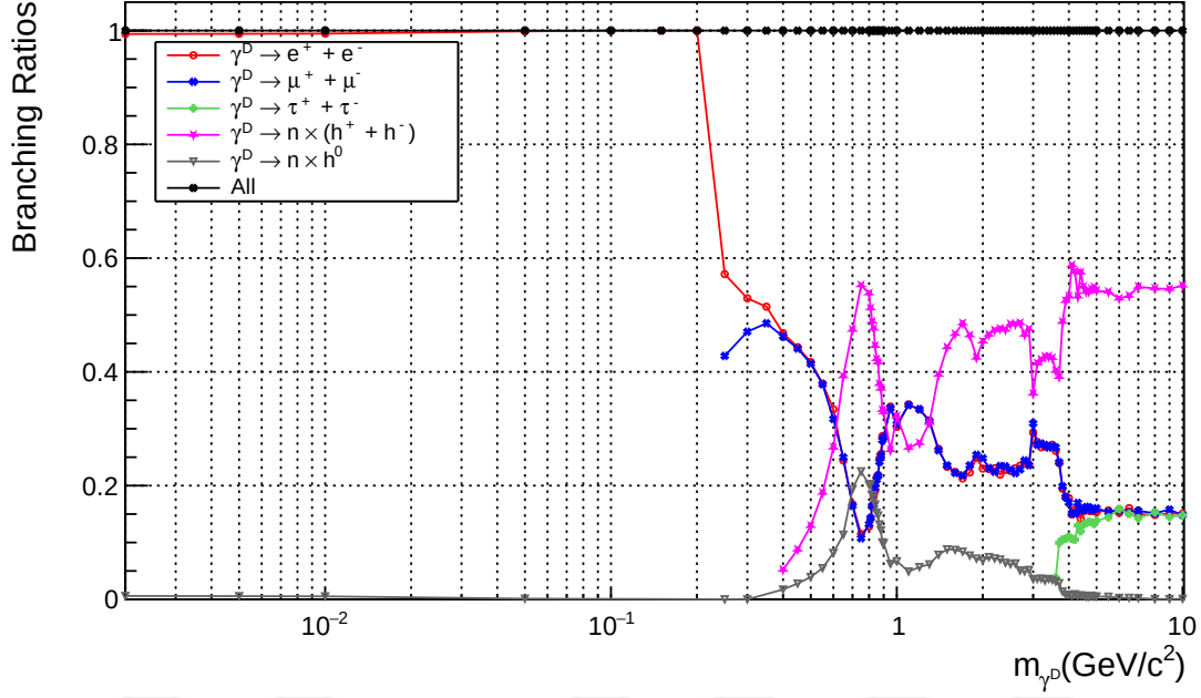
Figure 4.5: \gamma^D BR as a function of m_{\gamma^D}
