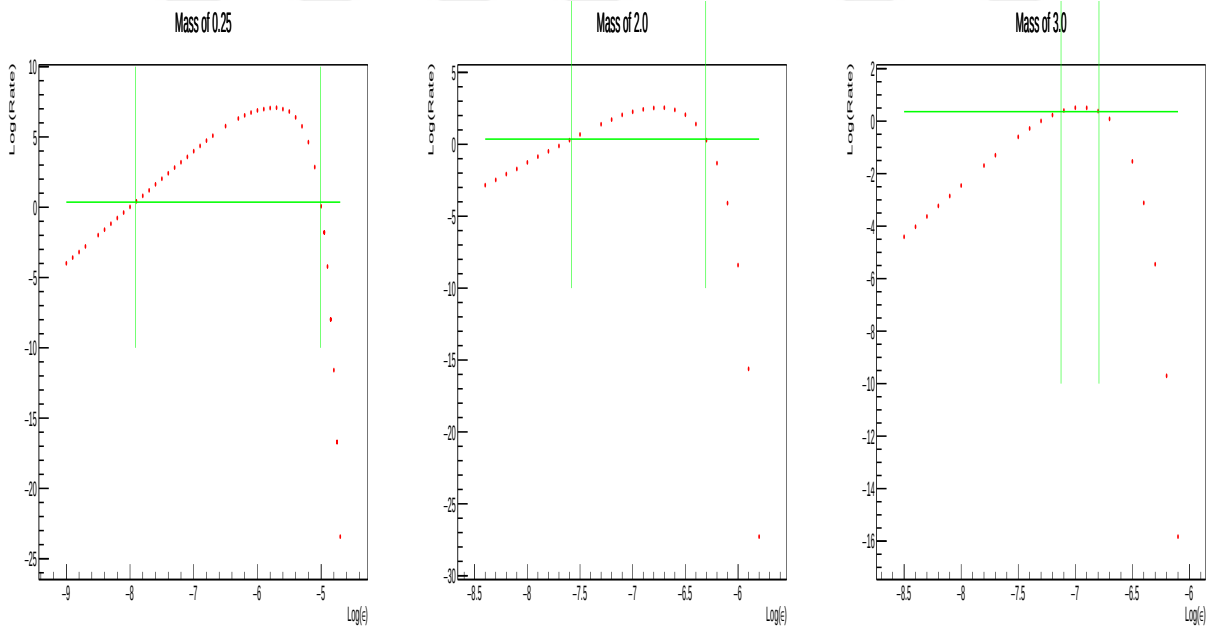
Figure 4.18: The lower and upper limits of \varepsilon (vertical green lines) for three different m_{\gamma D} values.
