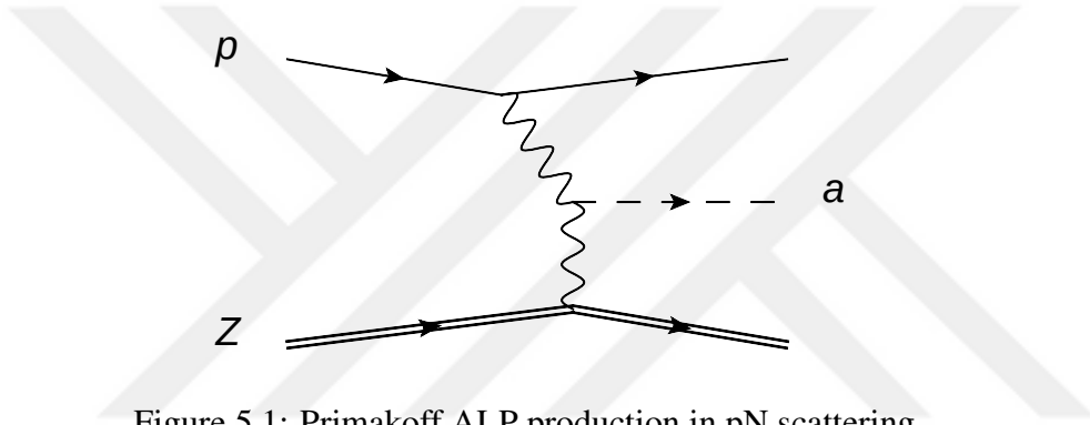
Figure 5.1: Primakoff ALP production in pN scattering
