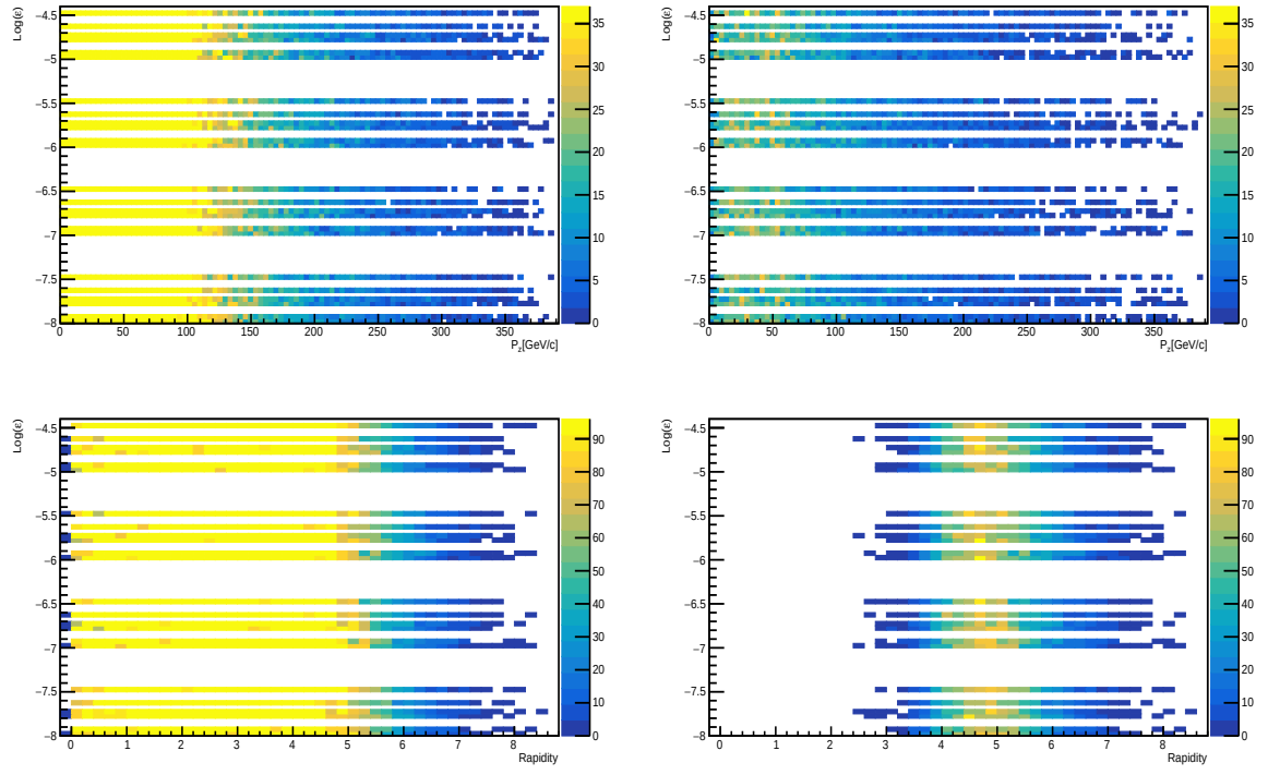
Figure 4.12: \epsilon versus P_z and \epsilon versus rapidity distributions of the decay products in the pbrem production at the m_{\gamma^D} = 1.0 GeV. On left: the purified events. On right: the vessel selected events.
