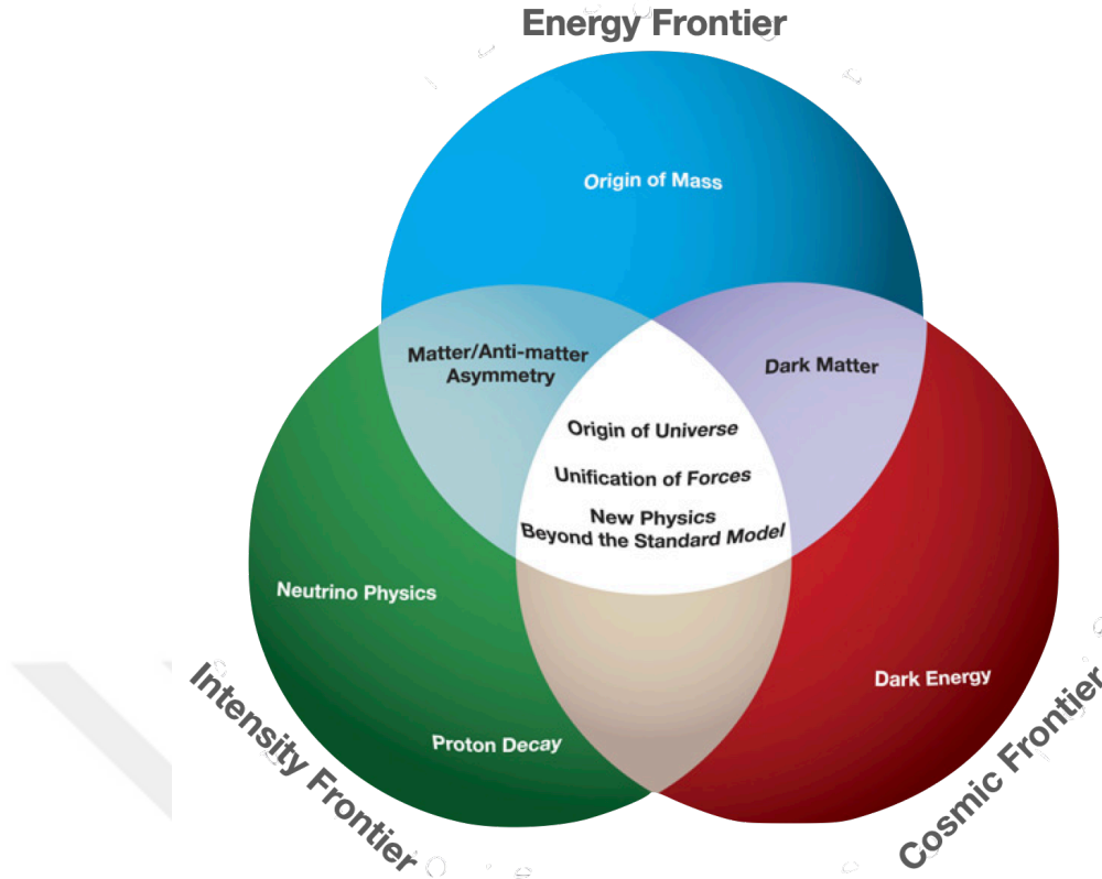
Figure 1.2: Possible research topics at the three frontiers.
