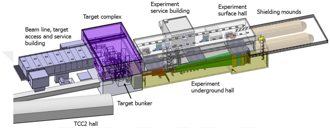
Figure 3.4: Planned facility layout
