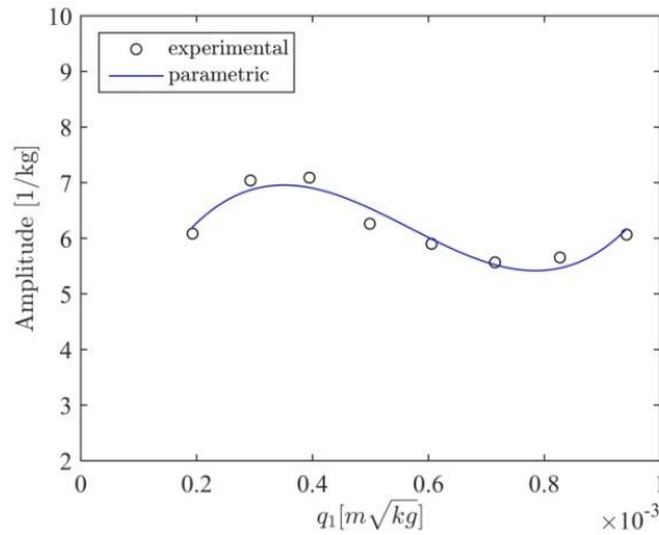
Figure 4-6. Variation of the modal constant corresponding to the 1 st mode of the T-beam with modal response level
