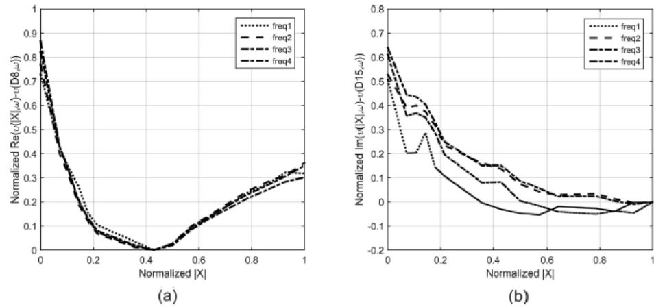
Fig. 24. Cross-section views of the real (left) and imaginary (right) parts of the relative describing surface of nonlinearity of the control fin actuation mechanism at different frequencies.
