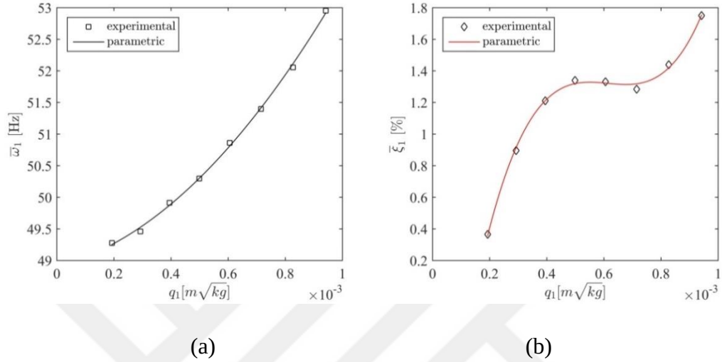
Figure 4-5. Variation of the modal parameters corresponding to the 1 st mode of the T-beam with modal response level (a) natural frequency (b) viscous modal damping ratio
