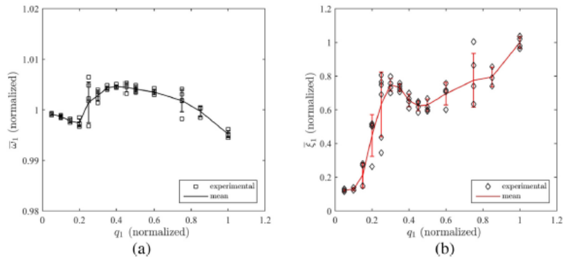
Fig. 23. Variation of the modal parameters corresponding to the 1st mode of the missile structure with modal response level (a) natural frequency (b) viscous modal damping ratio.
