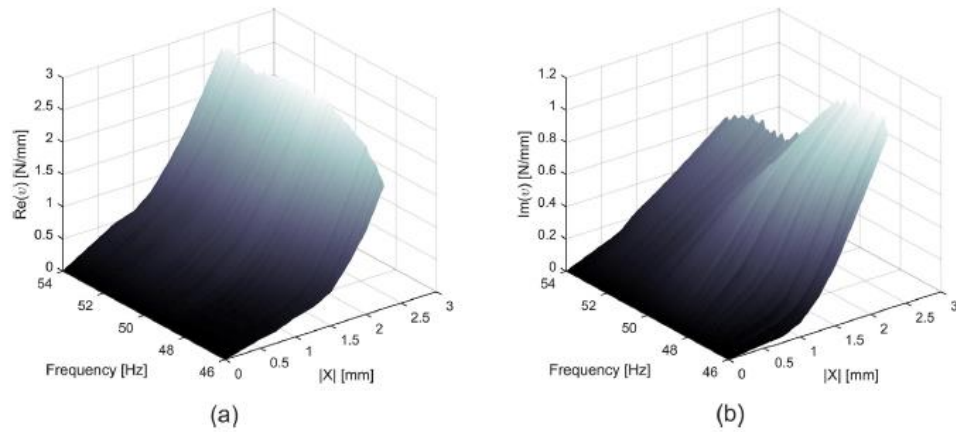
Fig. 5. Real (left) and imaginary (right) parts of the describing surface of nonlinearity for the T-beam.
