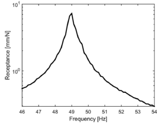
Fig. 6. Receptance of the underlying linear system of the T-beam estimated by using the DSM.
