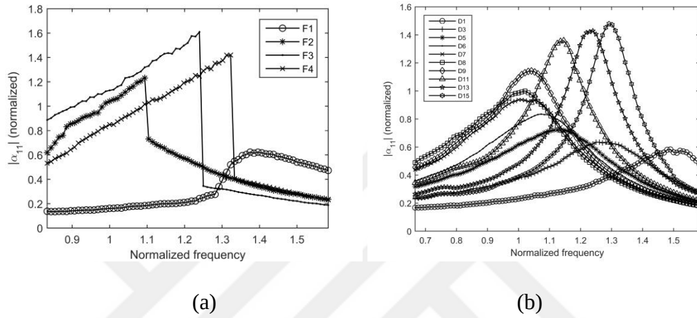
Figure 4-32. Frequency response functions of the control fin actuation mechanism at the driving point: (a) Constant-force FRFs measured by the classical constant-force testing (b) constant-response FRFs measured with RCT
