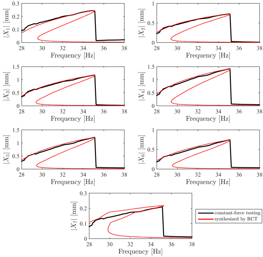
Figure 4-20. Comparison of the constant-force frequency response curves synthesized by using the identified nonlinear modal parameters of the geometrically nonlinear beam with the ones obtained from classical force-control testing at F=0.175 N force level
