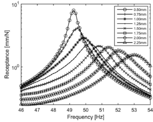
Fig. 2. Receptances of the T-beam measured by response-controlled stepped sine tests at various constant displacement amplitudes.
