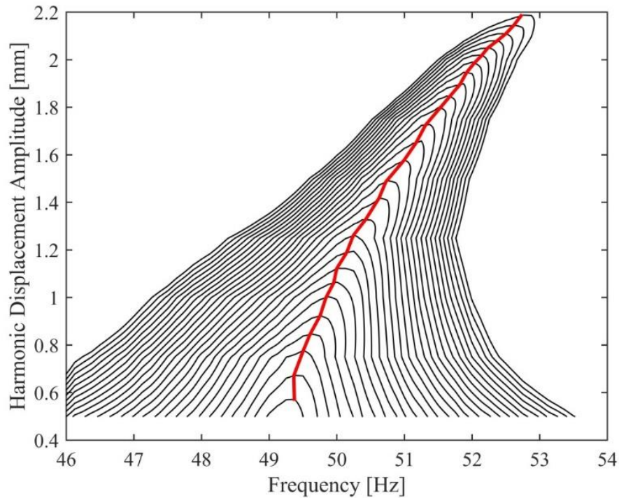
Figure 4-11. Constant-force frequency response curves (0.1 N-1.4N) and the backbone curve of the T-beam at the T-junction obtained by cutting the HFS with various constant force planes
