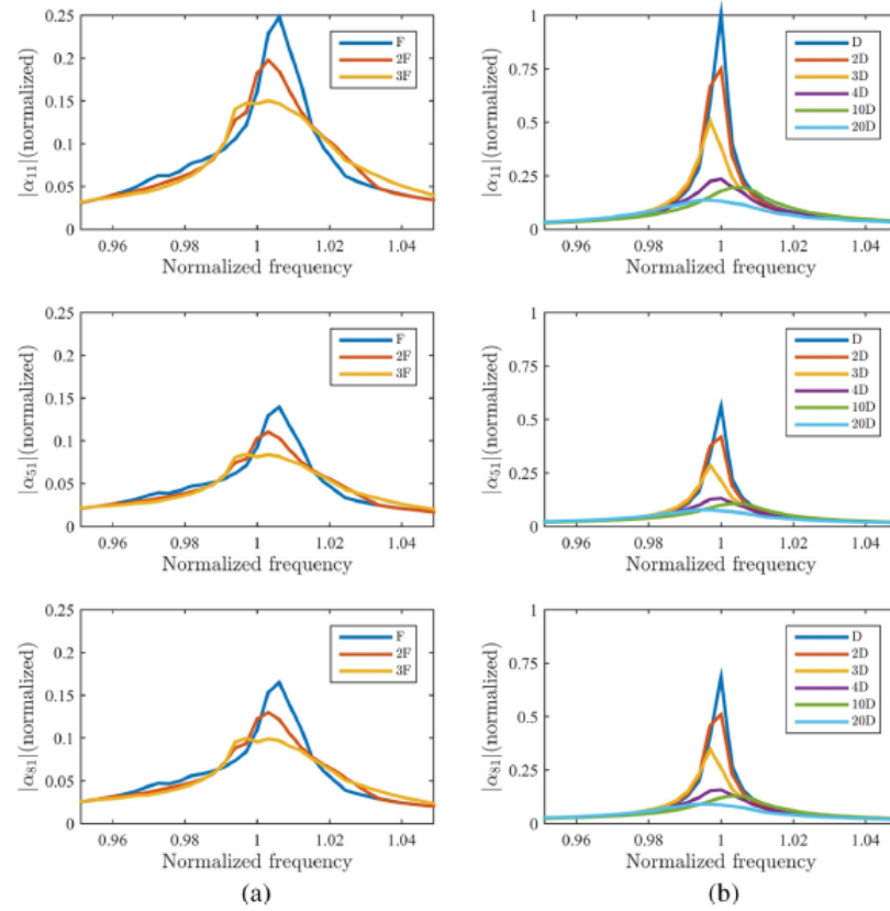
Fig. 22. (a) Constant-force FRFs of the missile structure measured by the classical force-control approach (b) constant-response FRFs of the missile structure measured by the RCT approach.
