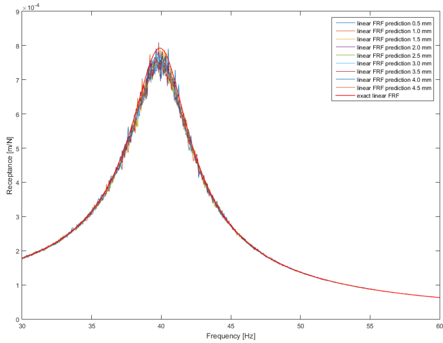
Figure 3-17. FRF of the underlying linear system of the SDOF system with cubic stiffness and Coulomb friction elements estimated by using the identified describing surface of nonlinearity
