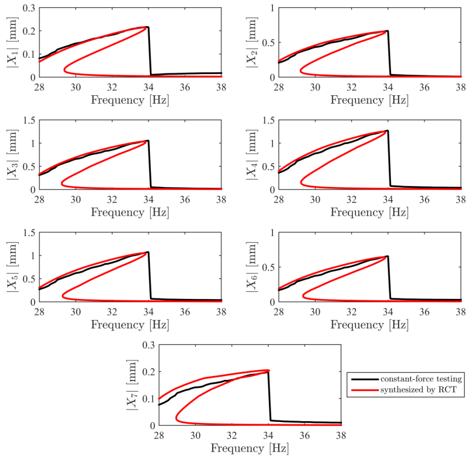
Figure 4-19. Comparison of the constant-force frequency response curves synthesized by using the identified nonlinear modal parameters of the geometrically nonlinear beam with the ones obtained from classical force-control testing at F=0.150 N force level
