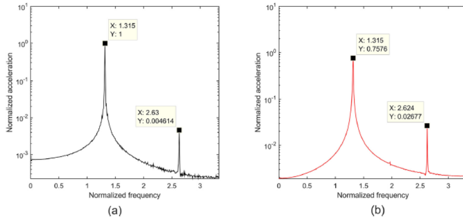
Fig. 22. Typical FFTs of time data samples collected during stepped-sine testing of the control fin actuation mechanism: (a) response-controlled test (D15 amplitude level) (b) force-controlled test (F4 amplitude level).
