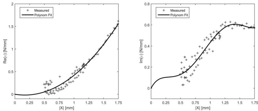
Figure 4-42. Real (left) and imaginary (right) parts of the describing function of nonlinearity of the T-beam
