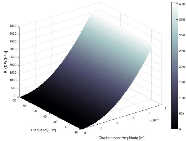
Figure 3-13. The real part of the describing surface of nonlinearity of the SDOF system with cubic stiffness and Coulomb friction elements
