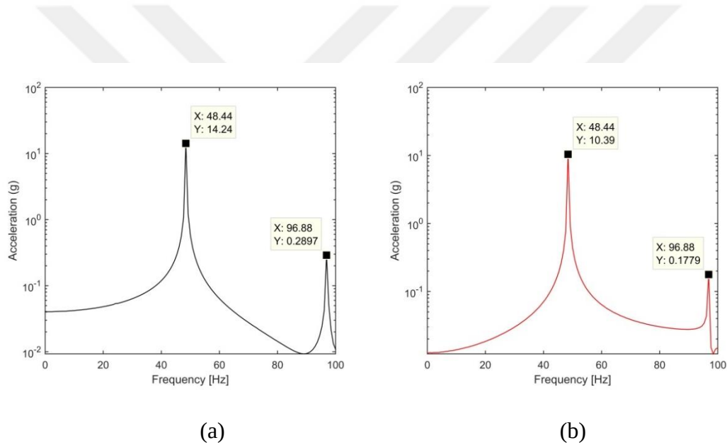
Figure 4-4. Typical FFTs of time data samples collected during stepped-sine testing of the T-beam: (a) response-controlled test (1.50 mm amplitude level) (b) force-controlled test (1.0 N amplitude level)
