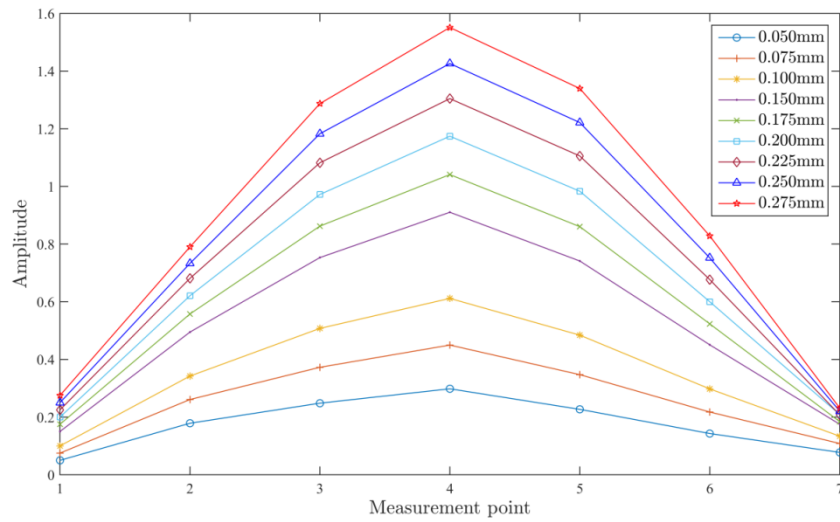
Figure 4-17. Variation of the 1 st NNM of the geometrically nonlinear beam with response level
