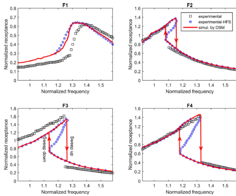
Fig. 26. Comparison of the simulation results obtained by the DSM of the control fin actuation mechanism with the experimental data obtained from force-controlled stepped-sine testing and HFS (response-controlled stepped-sine testing).
