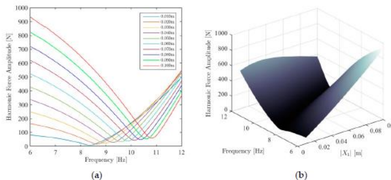
Figure 5. Construction of the HFS corresponding to the 1st DOF by combining harmonic force spectra with linear interpolation. (a) Harmonic excitation force spectra; (b) HFS of the 1st DOF [16].
