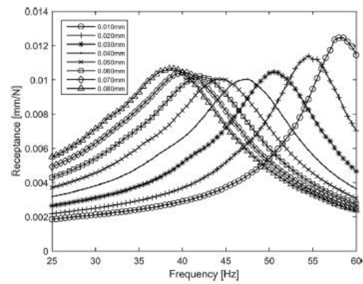
Fig. 14. Receptances of the dummy mass on elastomeric vibration isolators measured by response-controlled stepped sine tests at various constant displacement amplitudes.
