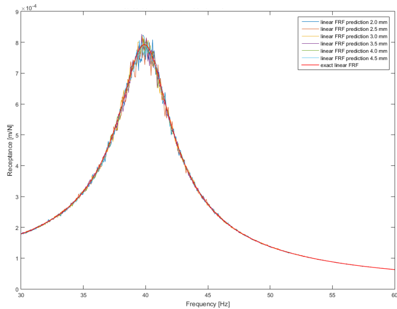
Figure 3-8. FRF of the underlying linear system that is estimated by using identified describing surface of nonlinearity of the SDOF system with cubic stiffness
