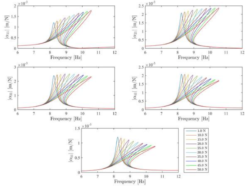
Fig. 3. Constant-force FRFs of the 5 DOF system with cubic stiffness, obtained by force-controlled stepped-sine testing simulations.
