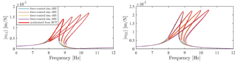
Fig. 11. Comparison of the constant-force FRFs obtained from simulated experiment, with the FRFs synthesized by using nonlinear modal parameters of the 5 DOF nonlinear system at several different forcing amplitude levels.
