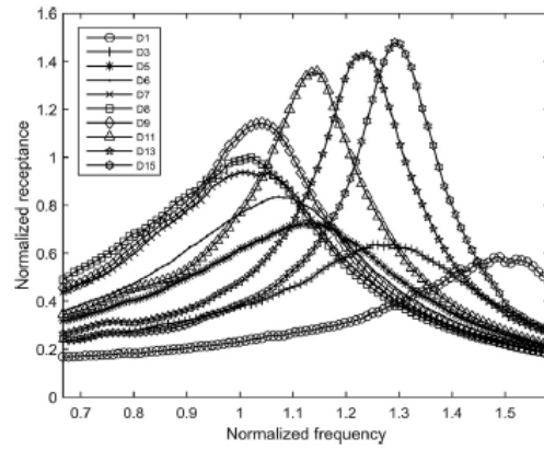
Fig. 21. Receptances of the control fin actuation mechanism measured by response-controlled stepped sine tests at various constant displacement amplitudes.
