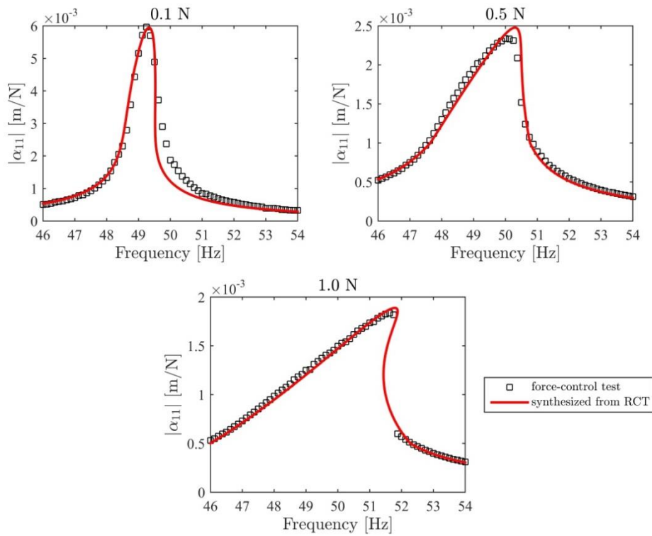
Figure 4-7. Comparison of the constant-force FRFs obtained from the force-control test with the FRFs synthesized by using the nonlinear modal parameters of the T-beam
