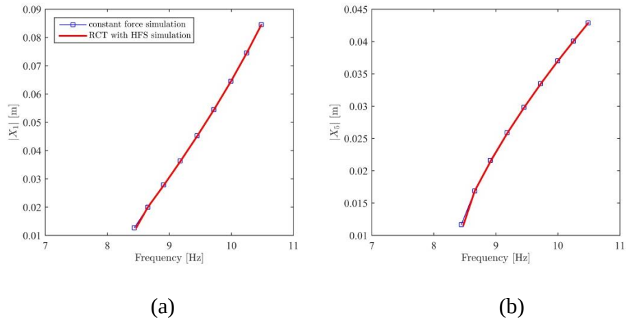
Figure 2-19. Comparison of the backbone curves obtained from RCT with HFS simulations with those obtained from constant force simulations (a) backbone curve of the 1 st DOF (b) backbone curve of the 5 th DOF
