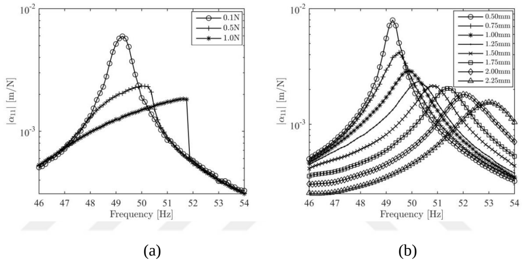
Figure 4-3. (a) Constant-force FRFs of the T-beam measured by the classical force-control approach (b) constant-response FRFs of the T-beam measured by the RCT approach
