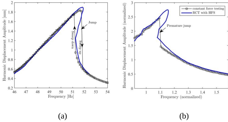
Figure 2-2. Frequency response curves measured in constant-force stepped-sine testing compared to the ones measured by RCT with HFS: (a) the jump phenomenon (b) the premature jump
