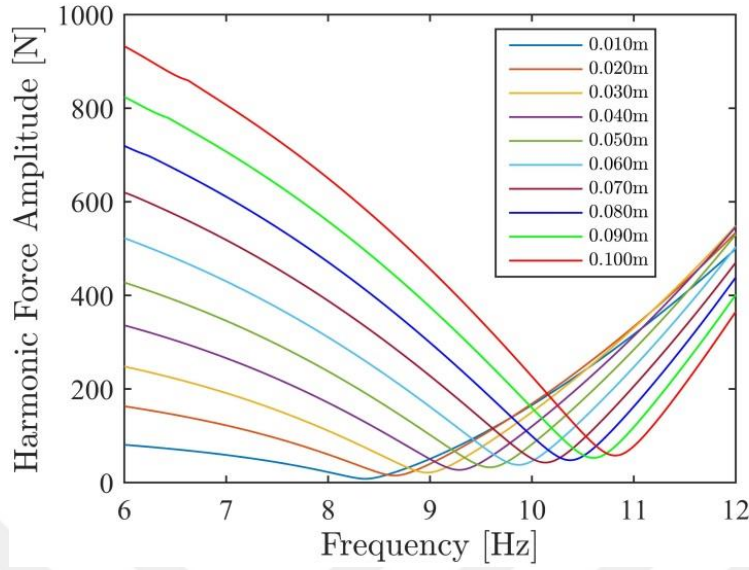
Figure 2-6. Harmonic force spectra of the driving point (1 st DOF) of the 5 DOF nonlinear system obtained from the RCT simulations
