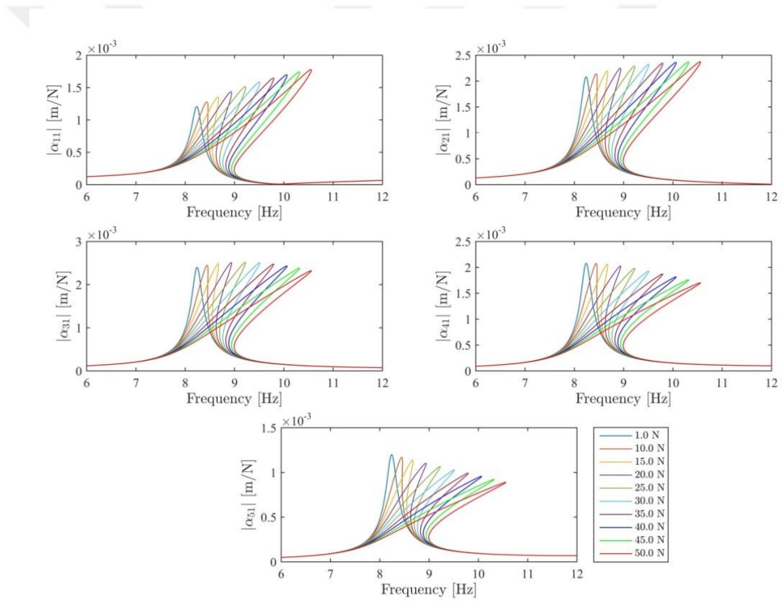
Figure 2-5. Constant-force FRFs of the 5 DOF system with cubic stiffness, obtained by the force-controlled stepped-sine testing simulations
