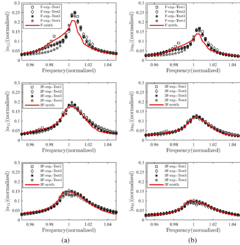
Fig. 26. Comparison of the constant-force FRFs obtained from force-controlled test, with FRFs synthesized by using nonlinear modal parameters of the missile: (a) driving point FRF (point 1 in Fig. 21) (b) FRF between tail point (point 8 in Fig. 21) and driving point.
