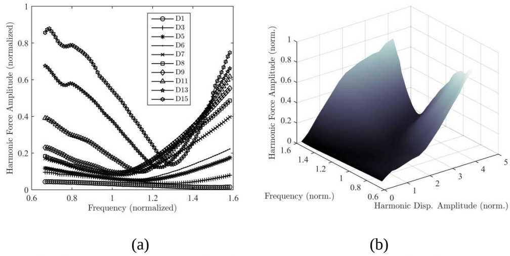
Figure 4-36. (a) Harmonic force spectra of the control fin actuation mechanism measured by RCT (b) HFS of the control fin actuation mechanism at the driving point, constructed by combining harmonic force spectra
