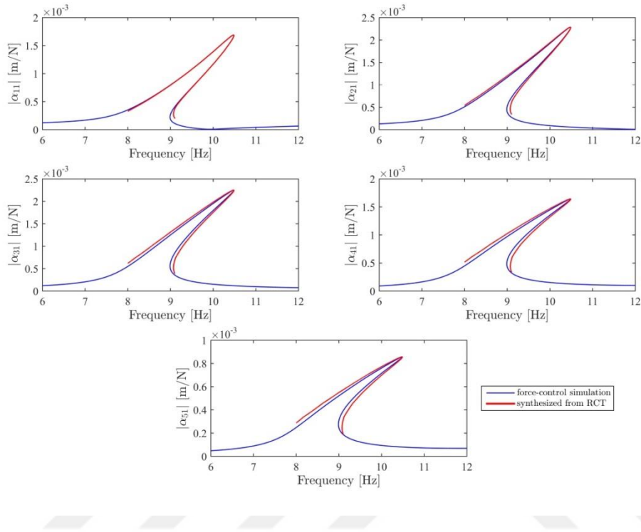
Figure 2-12. Comparison of the constant-force FRFs obtained from the simulated experiment, with the FRFs synthesized by using the nonlinear modal parameters of the 5 DOF nonlinear system at 50 N forcing amplitude level
