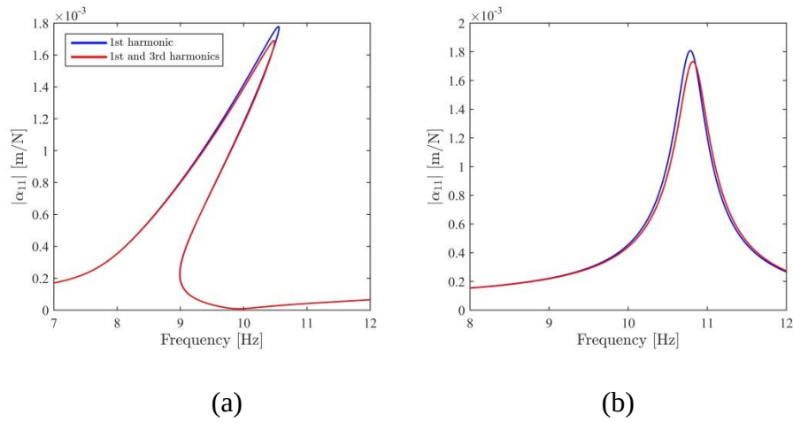
Figure 2-4. Effect of the 3 rd harmonic on the FRFs (a) constant-force driving point FRF at 50 N (b) constant-response driving point FRF at 0.10 m
