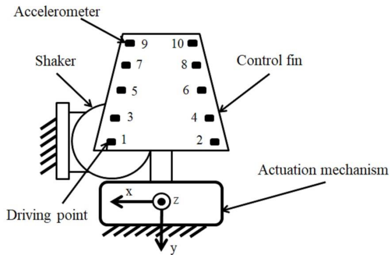
Figure 4-31. Sketch of the experimental setup for the control fin actuation mechanism
