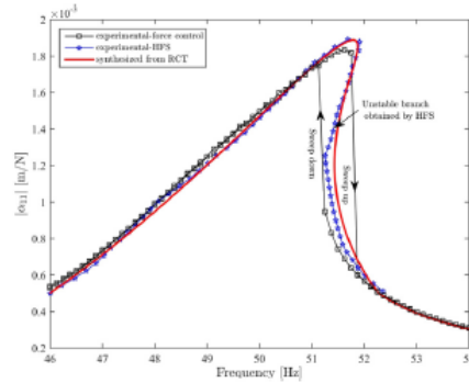
Fig. 20. Comparison of the receptances of the T-beam extracted by using the HFS approach with the ones synthesized by using nonlinear modal parameters identified from RCT, and with the original receptances obtained from force-control experiment at 1 N.
