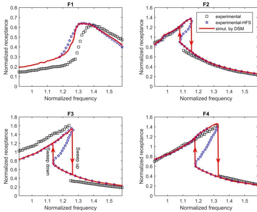
Figure 4-54. Comparison of the simulation results obtained by the DSM of the control fin actuation mechanism with the experimental data obtained from force-controlled stepped-sine testing and the HFS (response-controlled stepped-sine testing)
