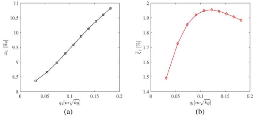
Fig. 8. Variation of the modal parameters corresponding to the 1st mode of the 5 DOF nonlinear system with modal response level (a) natural frequency (b) viscous modal damping ratio.
