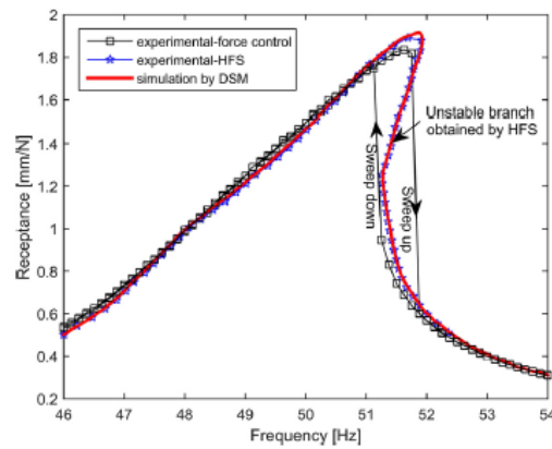
Fig. 12. Comparison of the receptances measured by the HFS of the T-beam at F = 1 N with the DSM simulation results and the receptances measured by using force-controlled stepped-sine testing.
