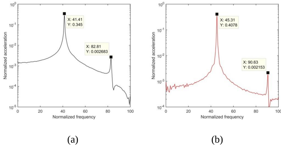
Figure 4-47. Typical FFTs of time data samples collected during stepped-sine testing of the dummy mass on elastomeric vibration isolators: (a) response-controlled test (0.05 mm amplitude level) (b) force-controlled test (5.0 N amplitude level)
