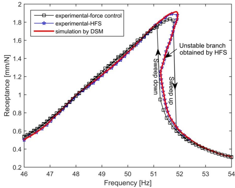
Figure 4-44. Comparison of the receptances measured by the HFS of the T-beam at F=1\text{N} with the DSM simulation results and the receptances measured by using force-controlled stepped-sine testing
