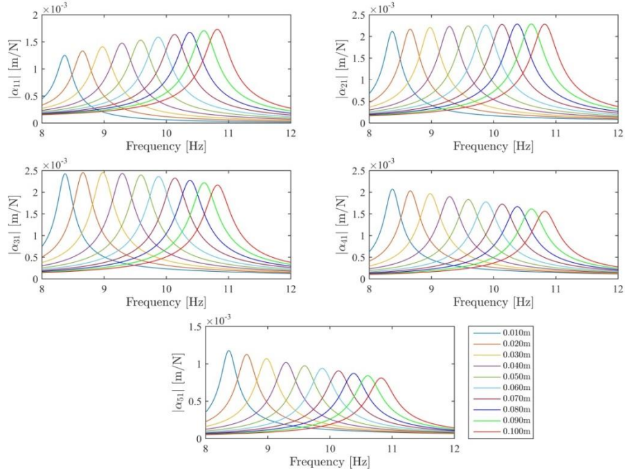
Figure 2-7. Constant-response FRFs of the 5 DOF system with cubic stiffness, obtained from the RCT simulations
