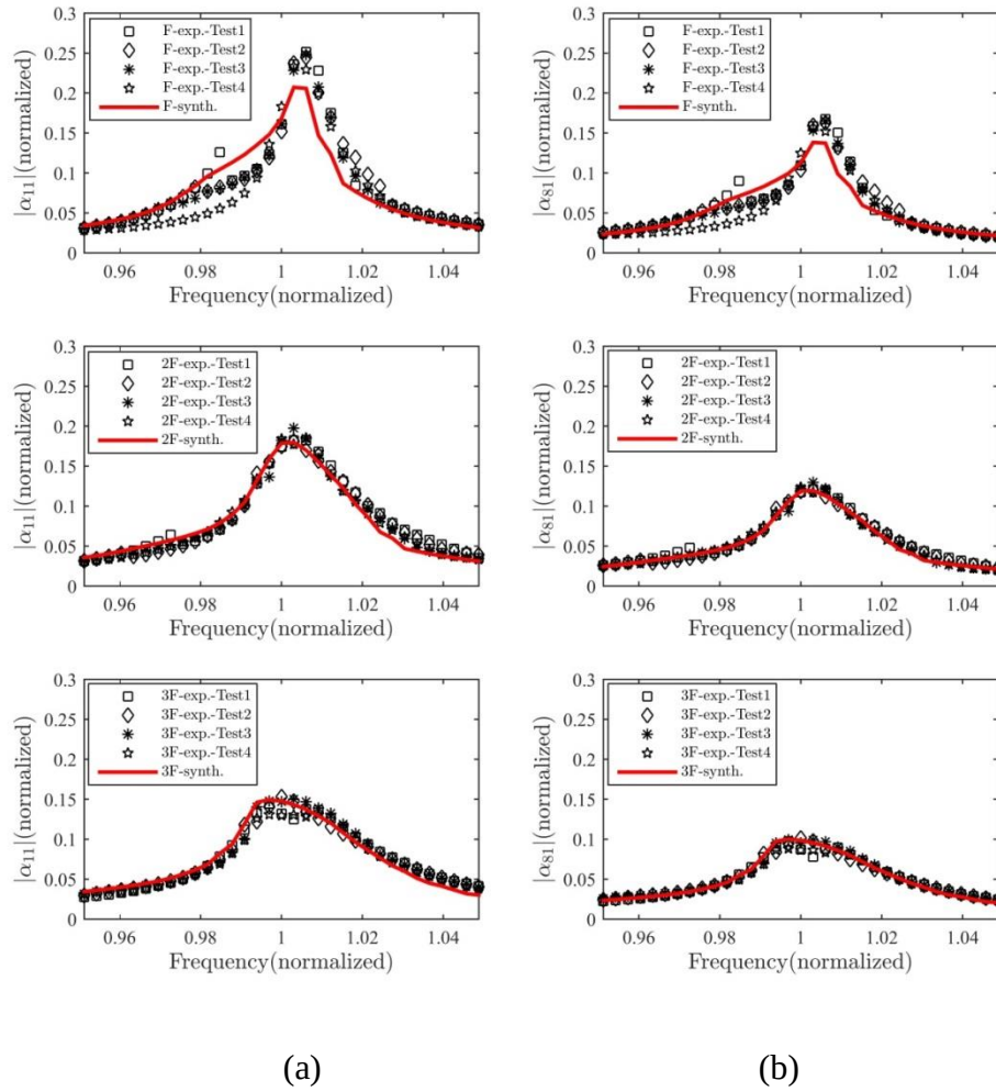
Figure 4-29. Comparison of the constant-force FRFs obtained from force-controlled testing, with the FRFs synthesized by using the nonlinear modal parameters of the missile structure: (a) driving point FRF (point1 in Figure 4-24) (b) FRF between tail point (point 8 in Figure 4-24) and driving point
