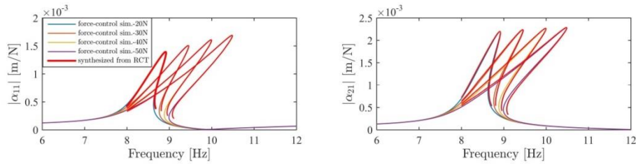
Figure 2-13. Comparison of the constant-force FRFs obtained from the simulated experiment, with the FRFs synthesized by using the nonlinear modal parameters of the 5 DOF nonlinear system at several different forcing amplitude levels
