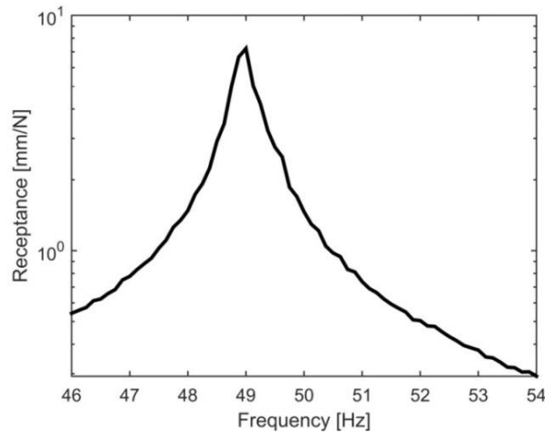
Figure 4-41. Receptance of the underlying linear system of the T-beam estimated by using the DSM
