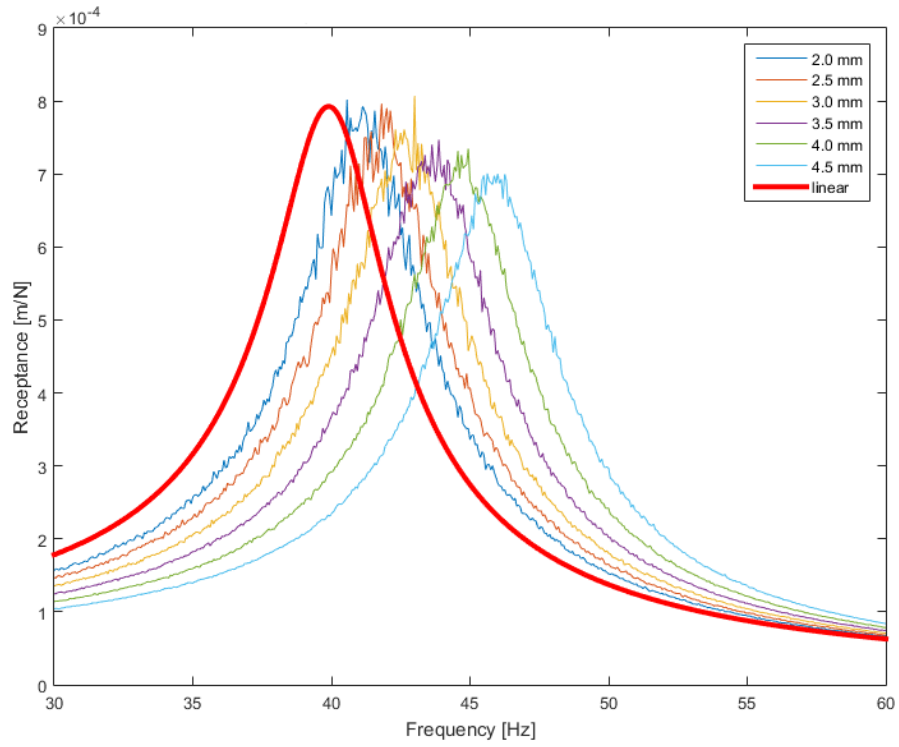
Figure 3-2. Constant-response FRFs of the SDOF system with cubic stiffness nonlinearity obtained from virtual response-controlled stepped-sine testing
