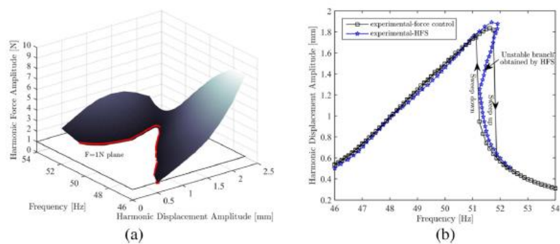
Fig. 19. (a) Determination of the harmonic response spectrum with any existing unstable branch by cutting HFS with a constant force plane (b) Comparison of the response spectrum obtained by HFS with the one obtained by force controlled testing.
