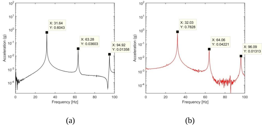
Figure 4-14. FFTs of time data recorded at the driving point of the geometrically nonlinear beam (a) Response-controlled test (0.150 mm amplitude level) (b) force-controlled test (0.175 N amplitude level)
