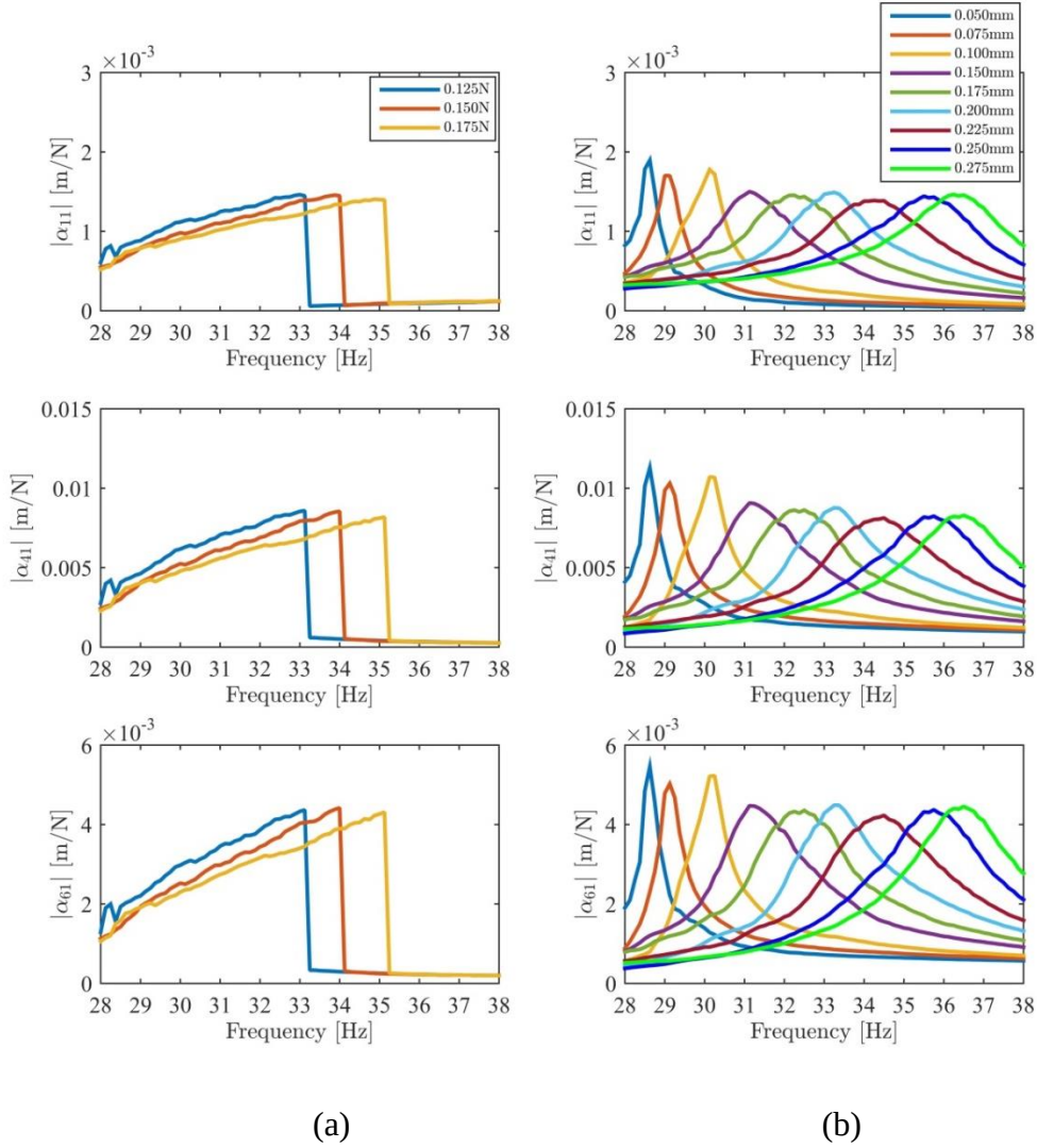
Figure 4-13. Frequency response functions of the geometrically nonlinear clamped-clamped beam: (a) Constant-force FRFs measured by the classical constant-force testing (b) quasi-linear constant-response FRFs measured with RCT
