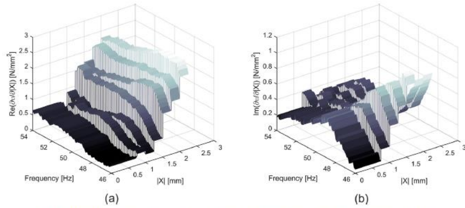
Fig. 4. Real (left) and imaginary (right) parts of the partial derivative of the describing surface of the nonlinearity for the T-beam.
