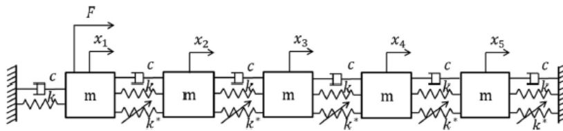
Fig. 1. 5 DOF system with cubic stiffness nonlinearity.
