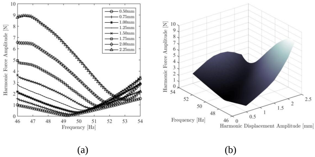
Figure 4-8. (a) Harmonic force spectra of the T-beam measured during RCT (b) HFS of the T-beam constructed by collecting harmonic force spectra and using linear interpolation
