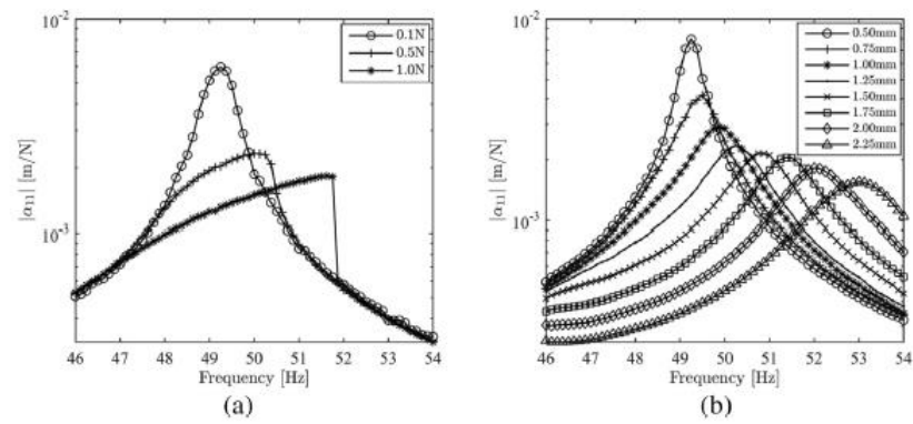
Fig. 14. (a) Constant-force FRFs of the T-beam measured by the classical force-control approach (b) constant-response FRFs of the T-beam measured by the RCT approach.
