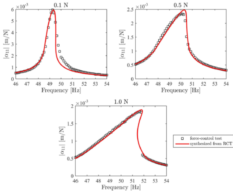
Fig. 17. Comparison of constant-force FRFs obtained from force-control test with FRFs synthesized by using nonlinear modal parameters of the T-beam.
