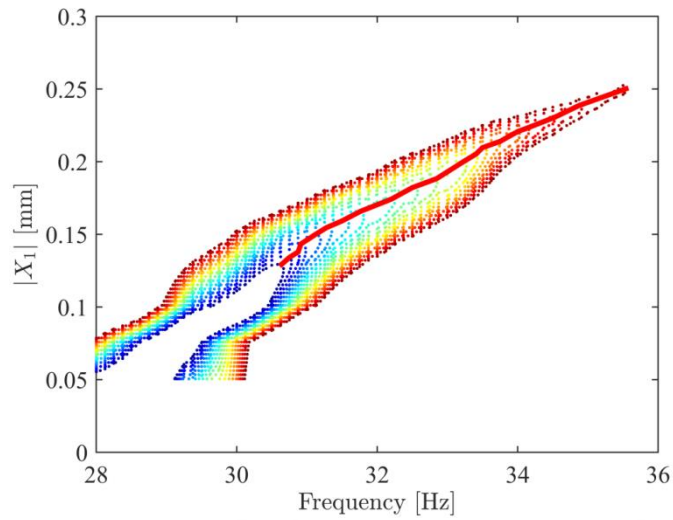
Figure 4-23. Constant-force frequency response curves and the backbone curve of the geometrically nonlinear beam at the driving point obtained by cutting the HFS with various constant force planes
