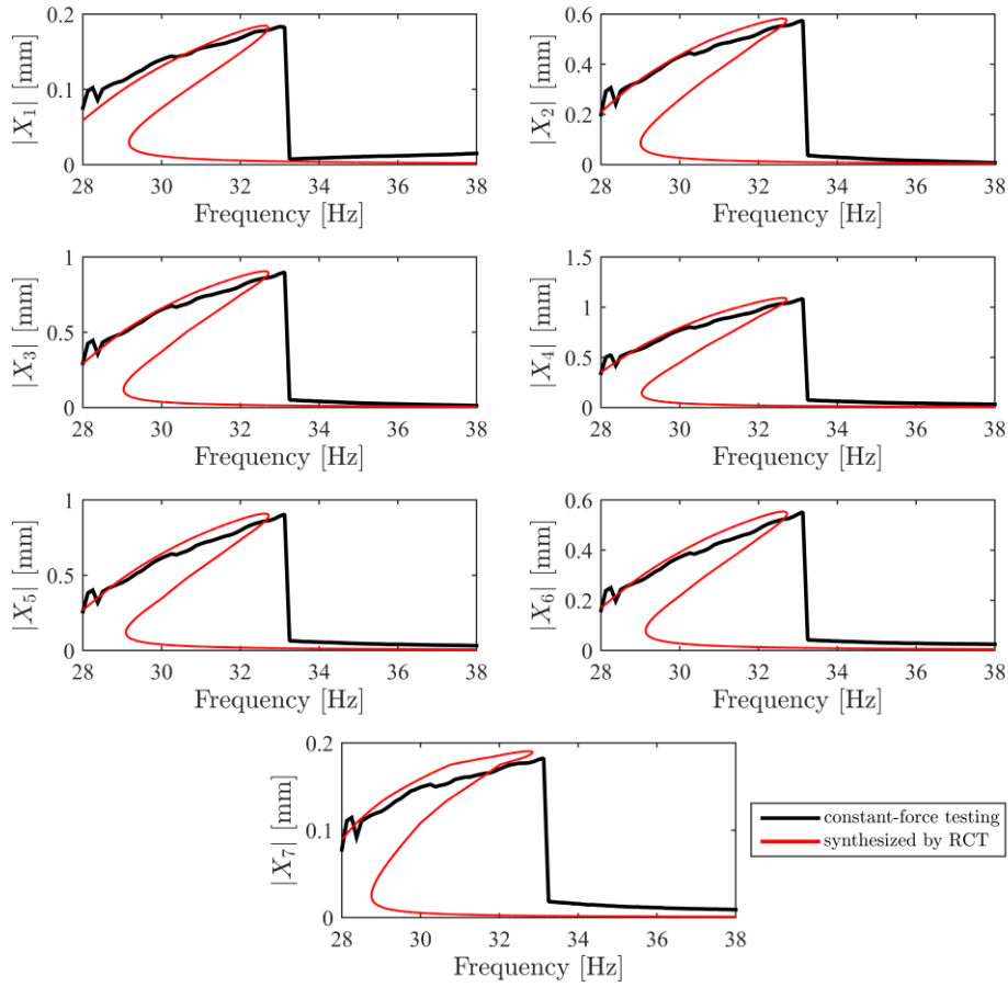
Figure 4-18. Comparison of the constant-force frequency response curves synthesized by using the identified nonlinear modal parameters of the geometrically nonlinear beam with the ones obtained from classical force-control testing at F=0.125 N force level
