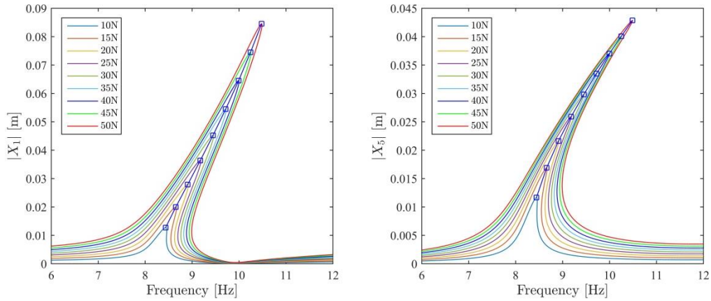
Figure 2-16. Determination of the backbone curves (blue square markers) of the 5 DOF nonlinear system corresponding to the 1 st and 5 th DOFs by using constant-force stepped-sine testing
