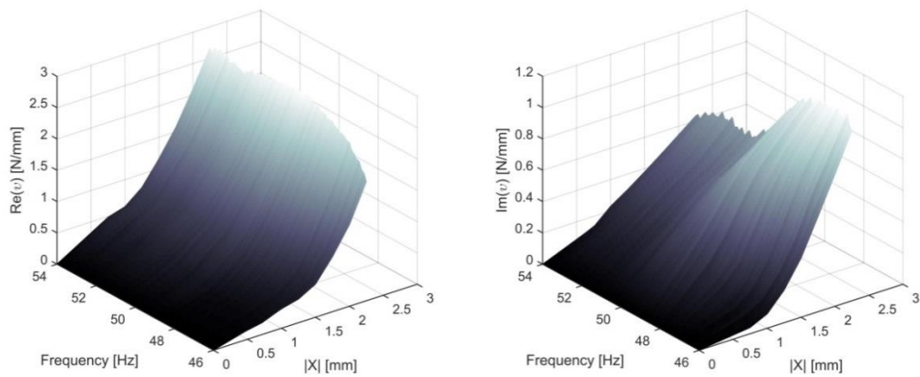
Figure 4-40. Real (left) and imaginary (right) parts of the describing surface of nonlinearity for the T-beam
