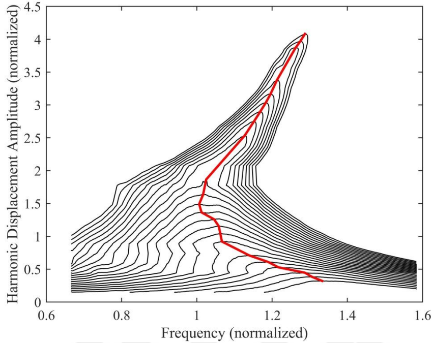
Figure 4-38. Constant-force frequency response curves and the backbone curve of the real control fin actuation mechanism at the driving point, obtained by cutting the HFS with various constant force planes
