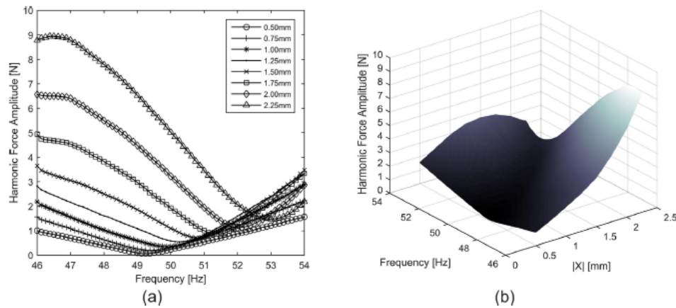
Fig. 10. HFS of the T-beam, obtained by response-controlled stepped sine test. Left: harmonic force spectra measured during the response-controlled stepped sine tests. Right: HFS constructed by collecting harmonic force spectra by using linear interpolation.
