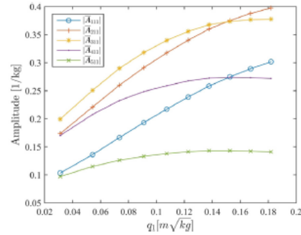
Fig. 9. Variation of the modal constants corresponding to the 1st mode of the 5 DOF nonlinear system with modal response level.
