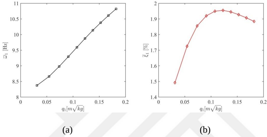
Figure 2-10. Variation of the modal parameters corresponding to the 1 st mode of the 5 DOF nonlinear system with the modal response level (a) natural frequency (b) viscous modal damping ratio
