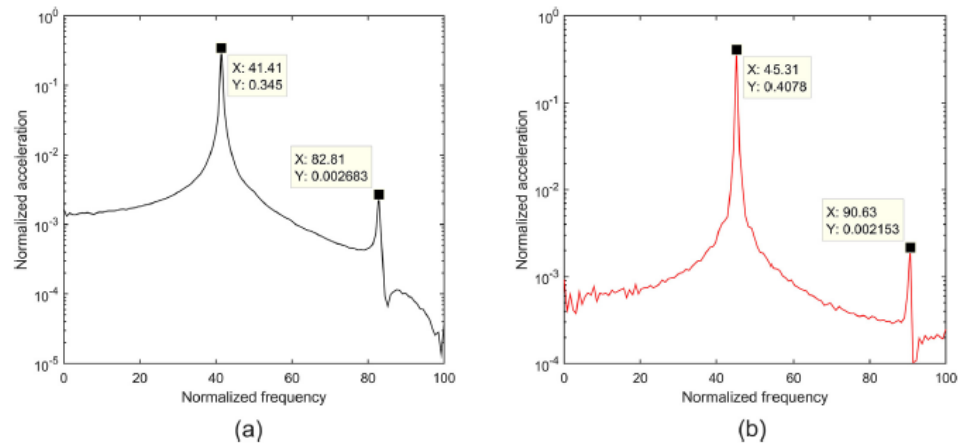
Fig. 15. Typical FFTs of time data samples collected during stepped-sine testing of the dummy mass on elastomeric vibration isolators: (a) response-controlled test (0.05 mm amplitude level) (b) force-controlled test (5.0 N amplitude level).
