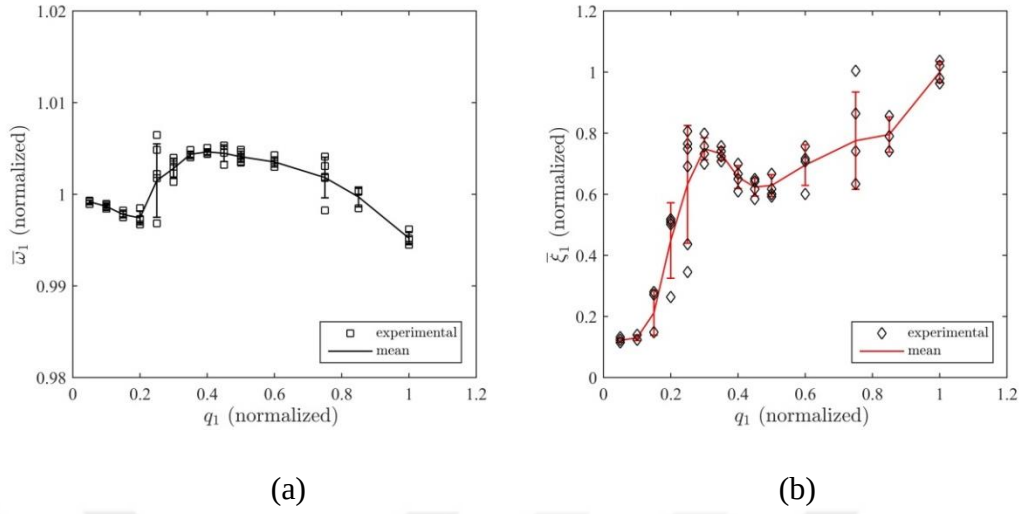
Figure 4-26. Variation of the modal parameters corresponding to the 1 st mode of the missile structure with modal response level (a) natural frequency (b) viscous modal damping ratio
