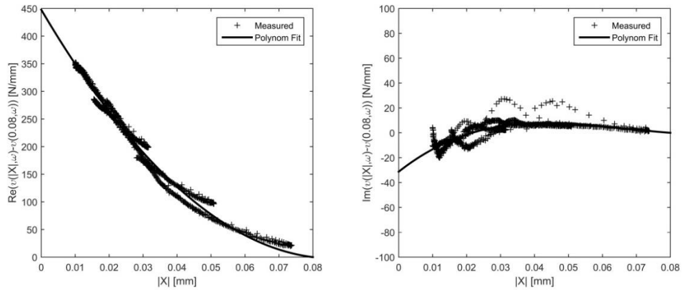
Figure 4-50. Real (left) and imaginary (right) parts of the relative describing function of nonlinearity of the dummy mass on elastomeric vibration isolators
