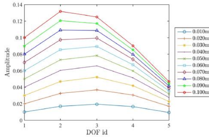
Fig. 6. The shape change of the 1st NNM of the 5 DOF nonlinear system with increasing displacement amplitude level.
