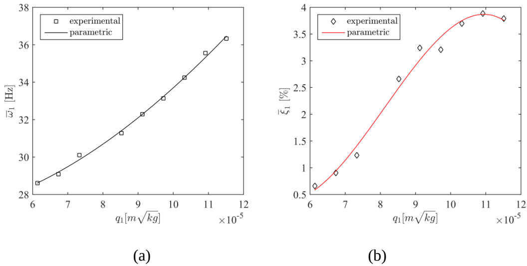
Figure 4-15. Variation of the modal parameters corresponding to the 1 st mode of the geometrically nonlinear beam with modal response level: (a) Natural frequency (b) viscous modal damping ratio
