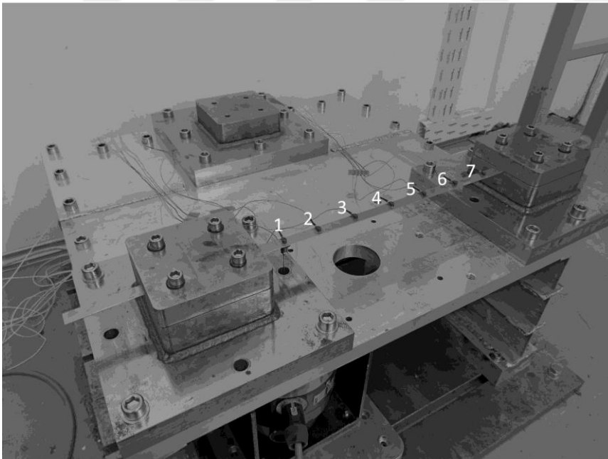
Figure 4-12. Geometrically nonlinear clamped-clamped beam experimental setup
