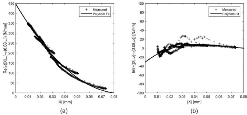
Fig. 18. Real (left) and imaginary (right) parts of the relative describing function of nonlinearity of the dummy mass on elastomeric vibration isolators.
