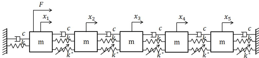
Figure 2-3. 5 DOF system with cubic stiffness nonlinearity
