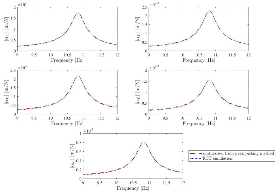
Figure 2-9. Comparison of the constant-response FRFs obtained from the RCT simulation, with the FRFs synthesized by using the modal parameters identified from the pick-peaking method at the 0.10 mm amplitude level
