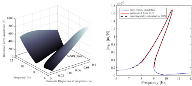
Fig. 12. (a) HFS of the 5 DOF nonlinear system (b) Comparison of the receptances extracted by using the HFS approach, with the ones synthesized by using the nonlinear modal parameters identified from RCT, and with the original receptances obtained from simulated force-control experiment at 50 N.
