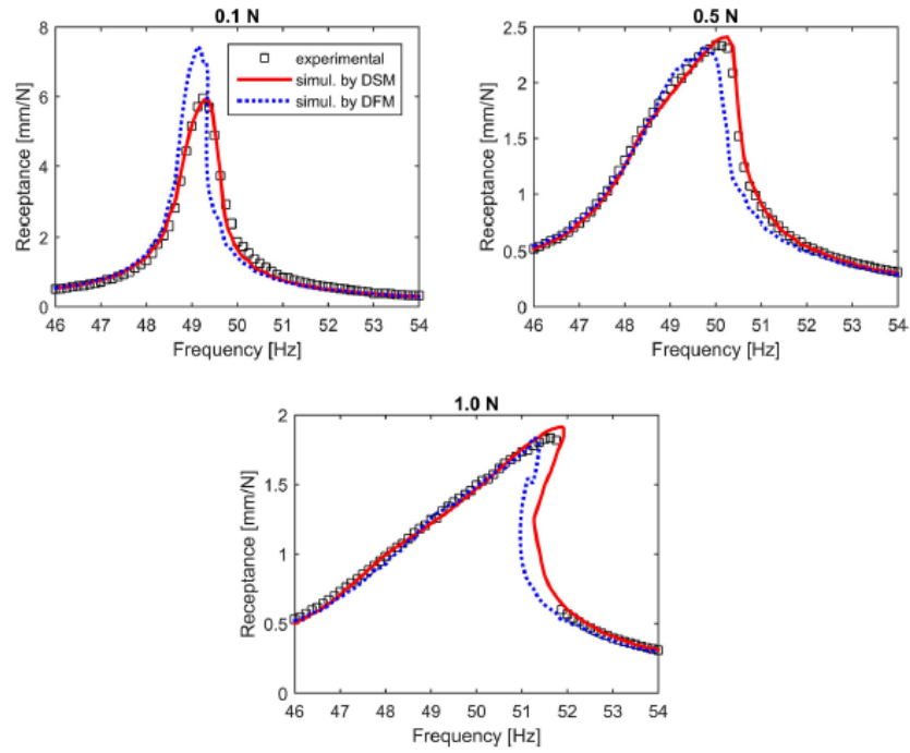
Fig. 9. Comparison of the simulation results obtained by the DSM and the DFM with the experimental data of the T-beam obtained from force-controlled stepped-sine testing.
