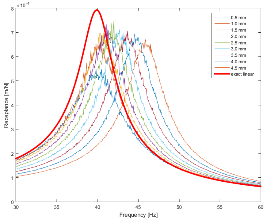
Figure 3-10. Constant-response FRFs of the SDOF system with cubic stiffness and Coulomb friction elements obtained from virtual response-controlled stepped-sine testing
