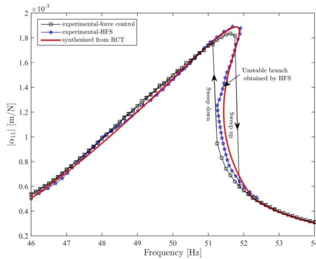
Figure 4-10. Comparison of the receptances of the T-beam extracted by using the HFS approach with the ones synthesized by using the nonlinear modal parameters identified from RCT, and with the original receptances obtained from the force-control experiment at 1 N
