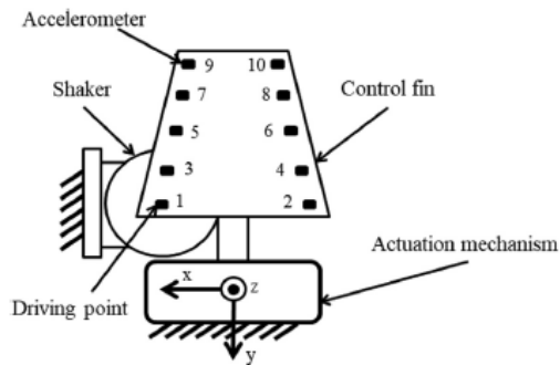
Fig. 20. Sketch of the experimental setup for the control fin actuation mechanism.
