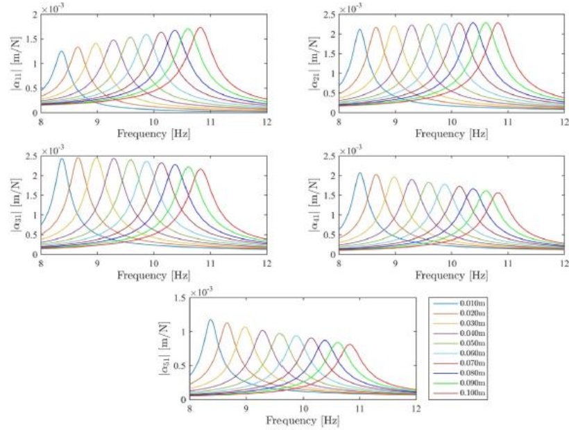
Fig. 5. Constant-response FRFs of the 5 DOF system with cubic stiffness, obtained from RCT simulations.
