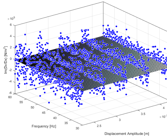
Figure 3-4. The imaginary part of the partial derivative of the describing surface of nonlinearity of the SDOF system with cubic stiffness element
