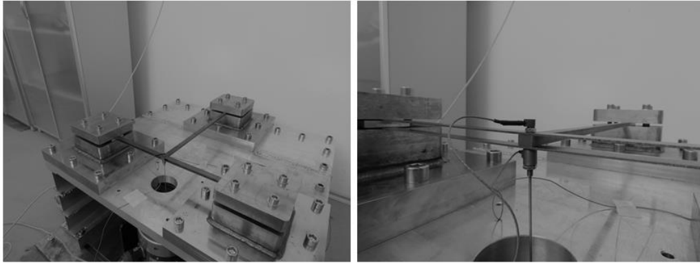
Figure 4-1. The T-beam experimental setup
