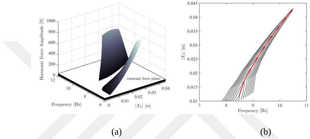
Figure 2-18. (a) HFS of the 5 th DOF cut with constant force planes (b) extraction of constant-force frequency response curves (black-ranging from 10 N to 50 N with 5 N increments) and backbone curve (red) of the 5 th DOF from HFS
