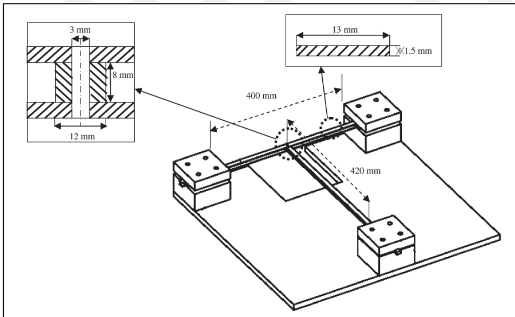
Figure 4-2. Dimensions of the T-beam test rig
