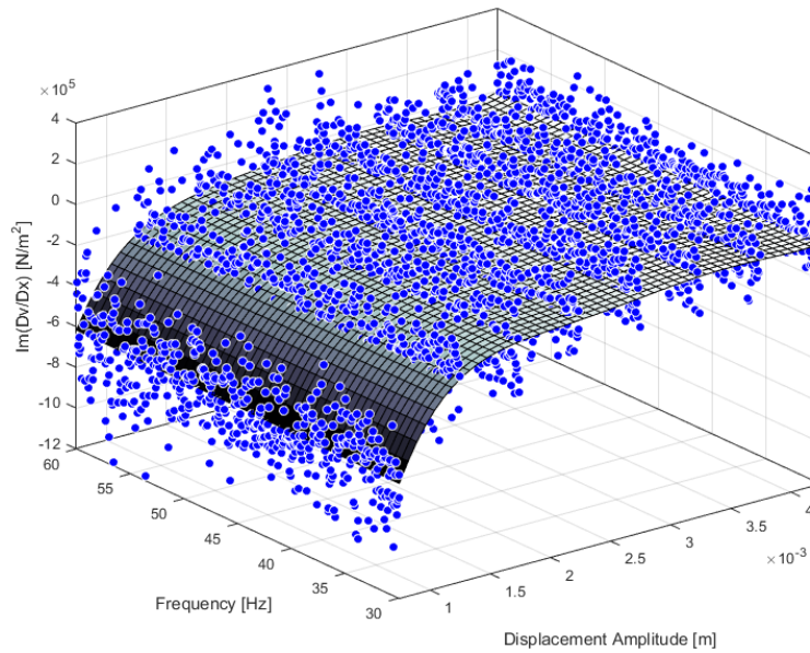
Figure 3-12. The imaginary part of the partial derivative of the describing surface of nonlinearity of the SDOF system with cubic stiffness and Coulomb friction elements
