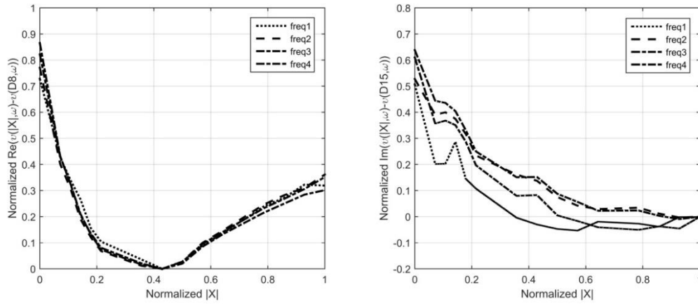
Figure 4-53. Cross-section views of the real (left) and imaginary (right) parts of the relative describing surface of nonlinearity of the control fin actuation mechanism at different frequencies
