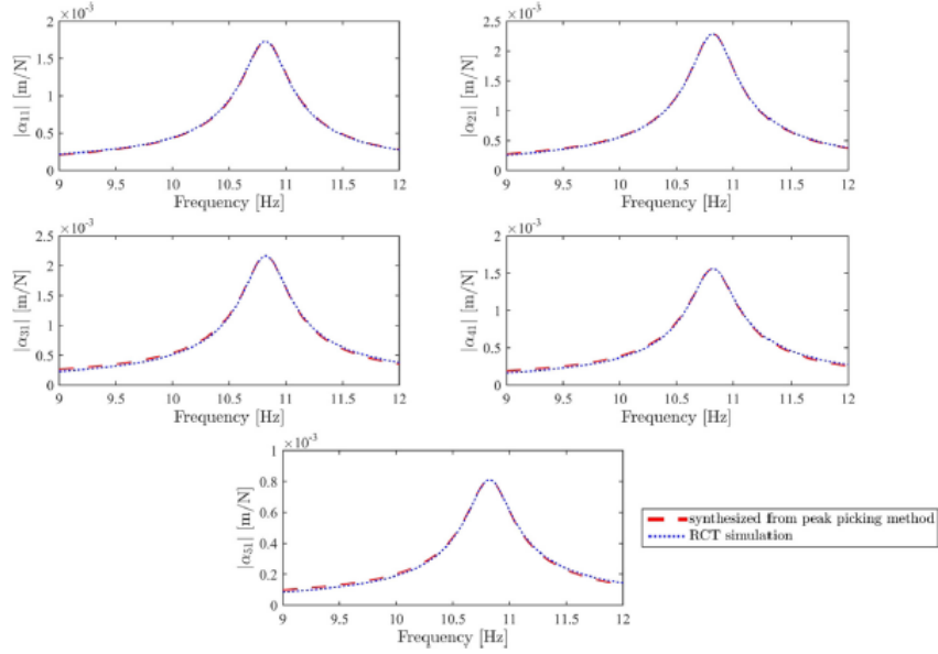
Fig. 7. Comparison of the constant-response FRFs obtained from RCT simulation, with the FRFs synthesized by using modal parameters identified from pick-peaking method at 0.10 mm amplitude level.
