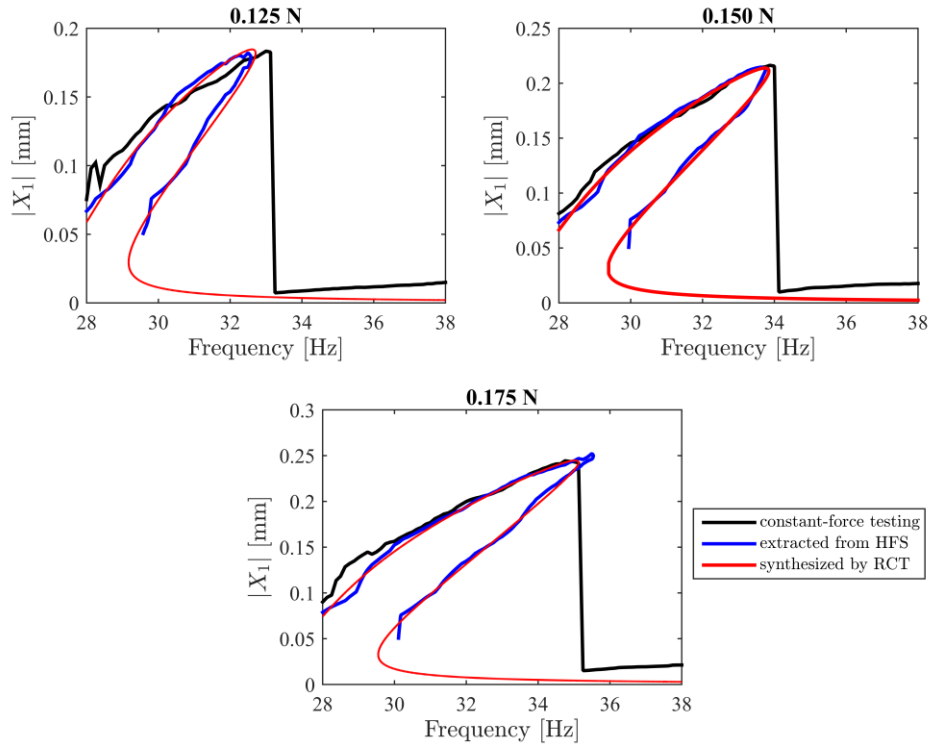
Figure 4-22. Comparison of the frequency response curves of the geometrically nonlinear beam extracted from the HFS with the ones synthesized by using nonlinear modal parameters and with the ones measured by classical constant force stepped-sine testing
