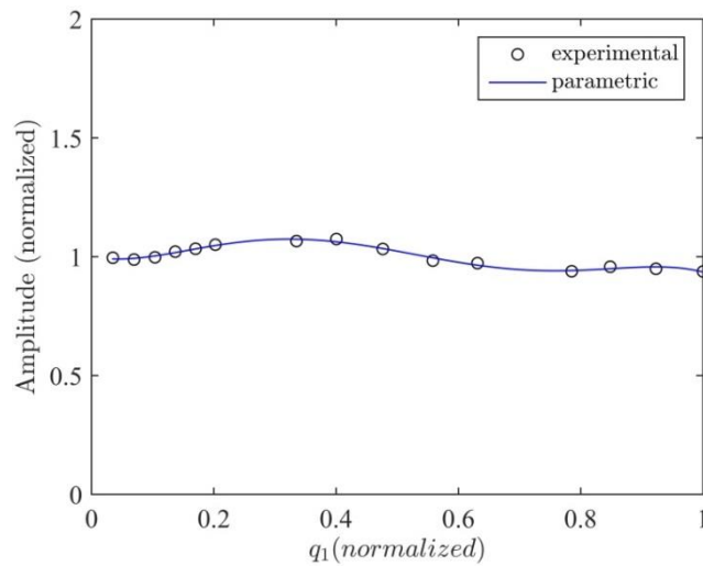
Figure 4-35. Variation of the modal constant corresponding to the 1 st mode of the control fin actuation mechanism with modal response level
