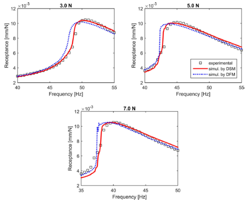
Fig. 19. Comparison of the simulation results obtained by the DSM and the DFM, with the experimental data of the dummy mass on elastomeric vibration isolators obtained from force-controlled stepped-sine testing.
