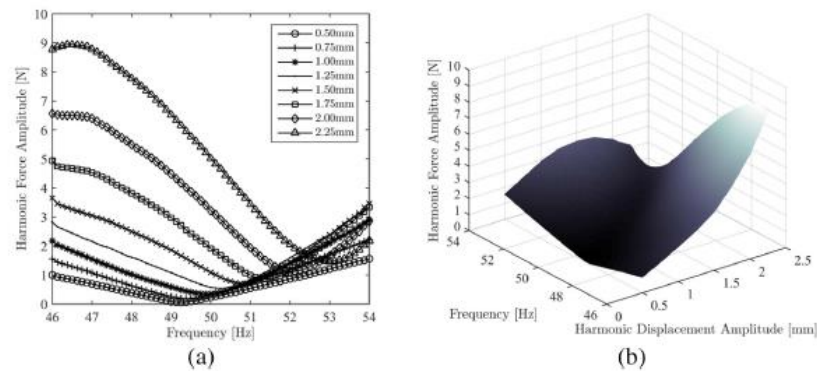
Fig. 18. (a) Harmonic force spectra of the T-beam measured during RCT (b) HFS of the T-beam constructed by collecting harmonic force spectra and using linear interpolation.
