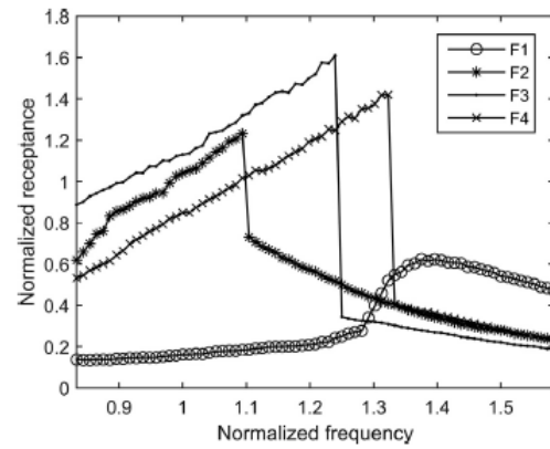
Fig. 25. Receptances of the control fin actuation mechanisms measured by force-controlled stepped sine tests at various constant force amplitudes.
