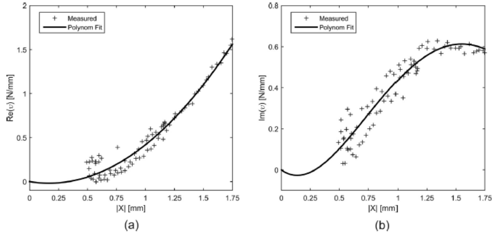
Fig. 8. Real (left) and imaginary (right) parts of the describing function of nonlinearity of the T-beam.
