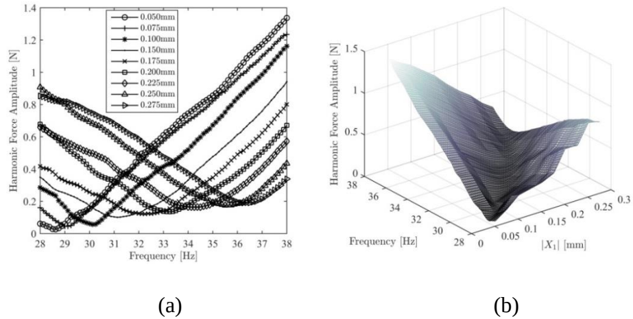
Figure 4-21. (a) Harmonic excitation force spectra of the geometrically nonlinear beam measured during RCT (b) HFS of the driving point constructed by combining harmonic force spectra with linear interpolation
