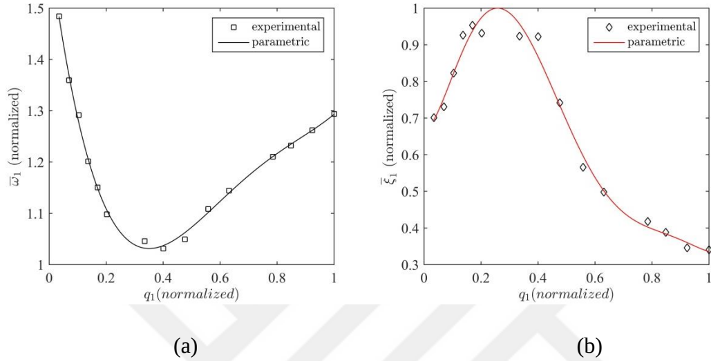
Figure 4-34. Variation of the modal parameters corresponding to the 1 st mode of the control fin actuation mechanism with modal response level (a) natural frequency (b) viscous modal damping ratio
