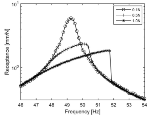
Fig. 7. Receptances of the T-beam measured by force-controlled stepped sine tests at various constant force amplitudes.
