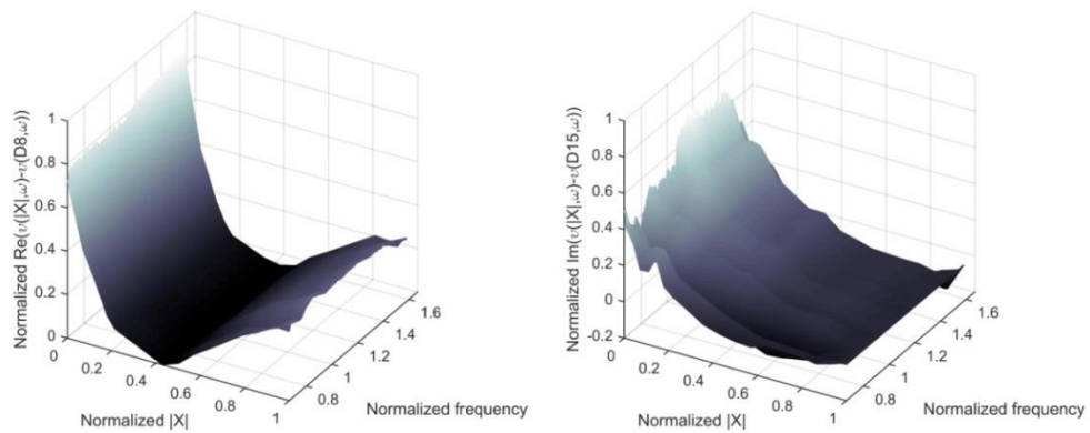
Figure 4-52. Real (left) and imaginary (right) parts of the relative describing surface of nonlinearity for the control fin actuation mechanism
