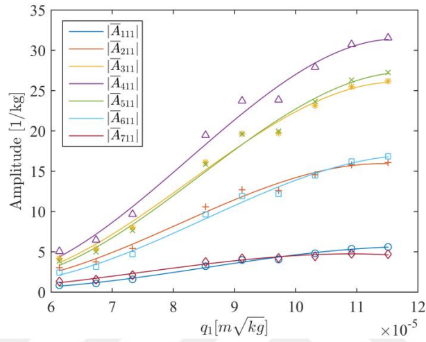
Figure 4-16. Variation of the modal constants corresponding to the 1 st mode of the geometrically nonlinear beam with modal response level
