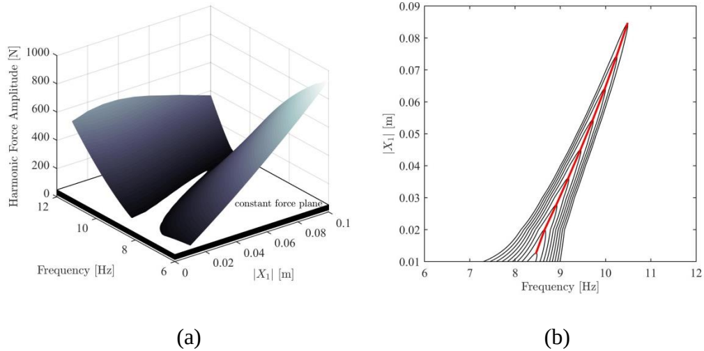
Figure 2-17. (a) HFS of the 1 st DOF cut with constant force planes (b) extraction of constant-force frequency response curves (black-ranging from 10N to 50N with 5N increments) and identification of the backbone curve (red) of the 1 st DOF from HFS
