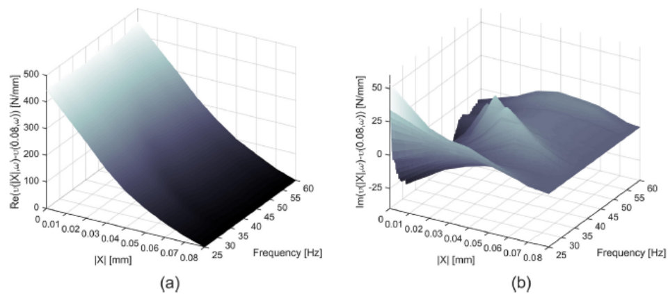
Fig. 16. Real (left) and imaginary (right) parts of the relative describing surface of the nonlinearity of the elastomeric vibration isolators.
