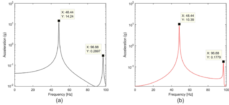
Fig. 3. Typical FFTs of time data samples collected during stepped-sine testing of the T-beam: (a) response-controlled test (1.50 mm amplitude level) (b) force-controlled test (1.0 N amplitude level).
