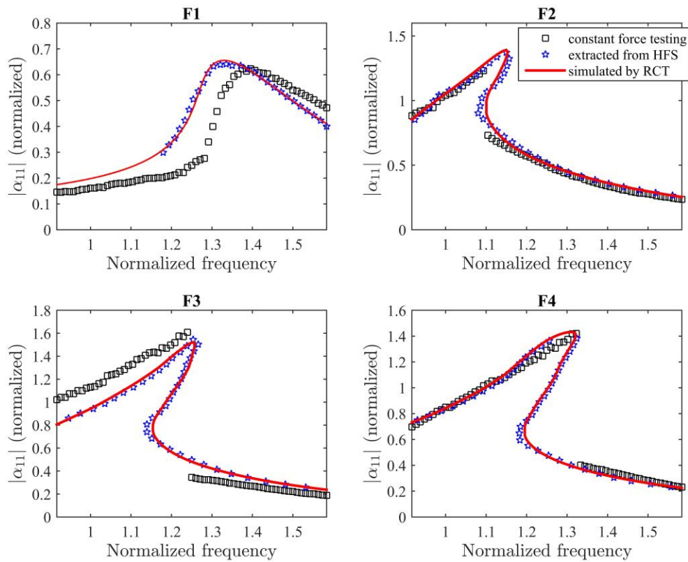
Figure 4-37. Comparison of the driving point receptances of the control fin actuation mechanism synthesized from the identified nonlinear modal parameters with the receptances directly measured from constant-force testing and with the receptances extracted from HFS
