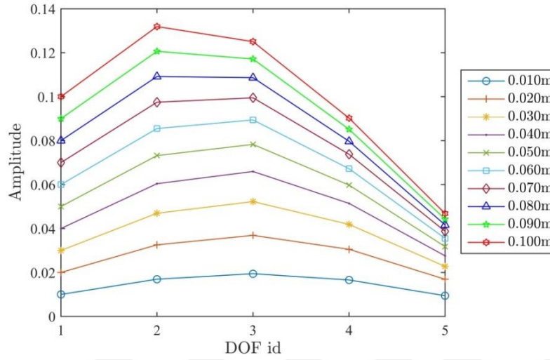
Figure 2-8. The shape change of the 1 st NNM of the 5 DOF nonlinear system with the increasing displacement amplitude level
