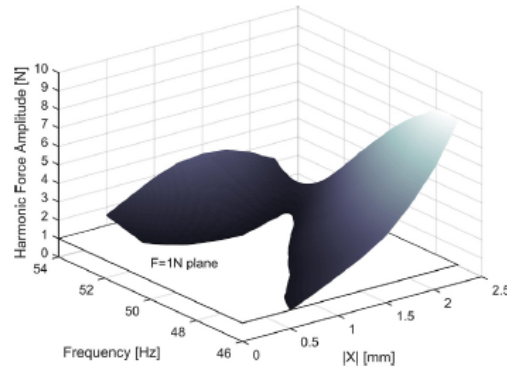
Fig. 11. HFS cut of the T-beam with constant harmonic force plane F = 1 N.
