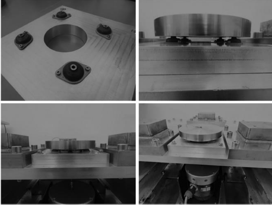
Fig. 13. Experimental setup of the dummy mass on elastomeric vibration isolators.
