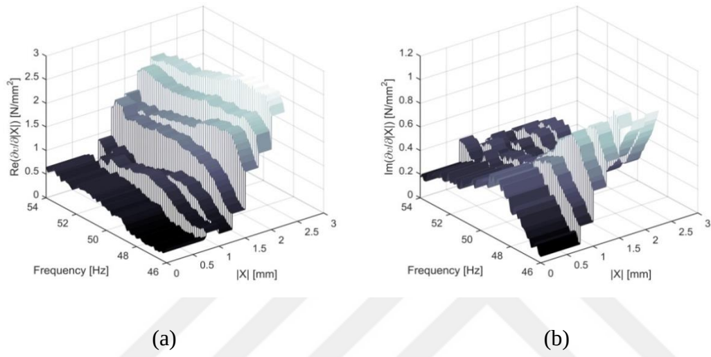
Figure 4-39. Real (left) and imaginary (right) parts of the partial derivative of the describing surface of nonlinearity for the T-beam
