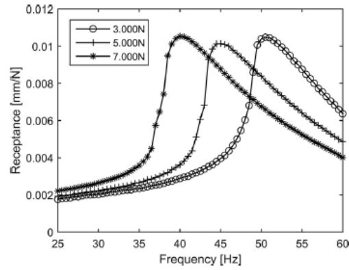
Fig. 17. Receptance curves of the dummy mass on elastomeric vibration isolators measured by force-controlled stepped sine tests at three different force amplitudes.
