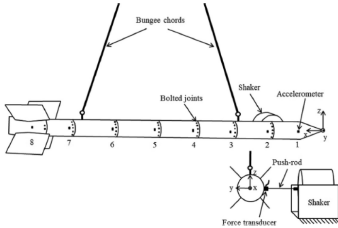
Fig. 21. Sketch of the experimental setup of the real missile.
