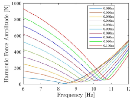
Fig. 4. Harmonic force spectra of the driving point (1st DOF) of the 5 DOF nonlinear system obtained from RCT simulations.
