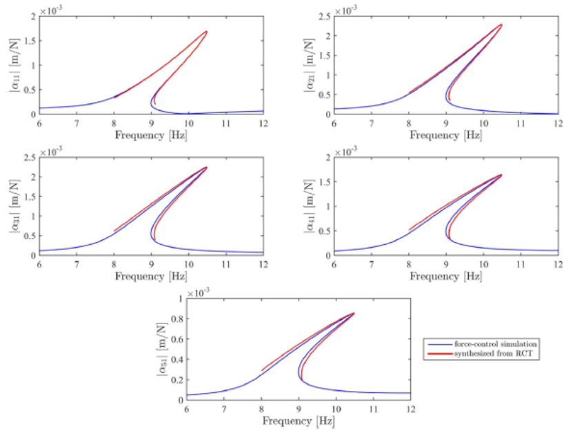
Fig. 10. Comparison of the constant-force FRFs obtained from simulated experiment, with the FRFs synthesized by using nonlinear modal parameters of the 5 DOF nonlinear system at 50 N forcing amplitude level.
