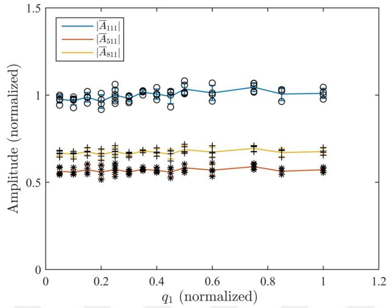
Figure 4-27. Variation of the modal constants corresponding to the 1 st mode of the missile structure with modal response level
