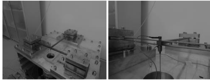
Fig. 13. The T-beam experimental setup.
