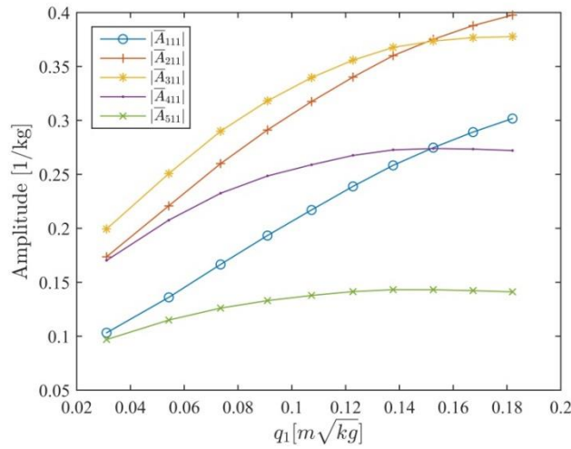
Figure 2-11. Variation of the modal constants corresponding to the 1 st mode of the 5 DOF nonlinear system with the modal response level
