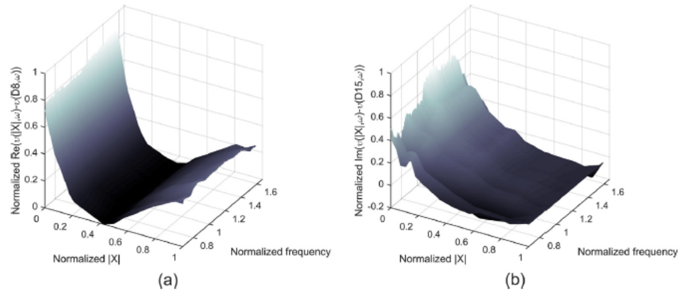
Fig. 23. Real (left) and imaginary (right) parts of the relative describing surface of nonlinearity for the control fin actuation mechanism.
