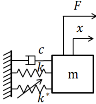
Figure 3-1. SDOF system with cubic stiffness nonlinearity
