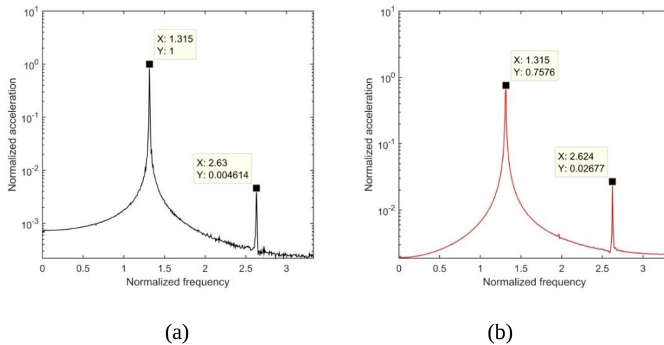
Figure 4-33. Typical FFTs of time data samples collected during stepped-sine testing of the control fin actuation mechanism: (a) response-controlled test (D15 amplitude level) (b) force-controlled test (F4 amplitude level)
