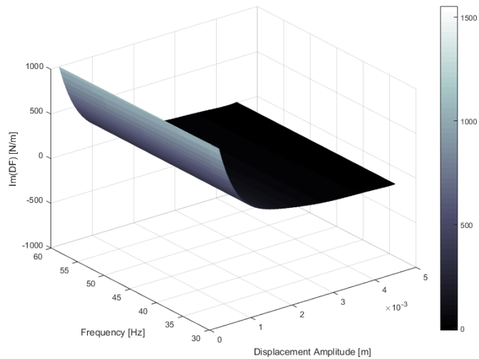
Figure 3-14. The imaginary part of the describing surface of nonlinearity of the SDOF system with cubic stiffness and Coulomb friction elements
