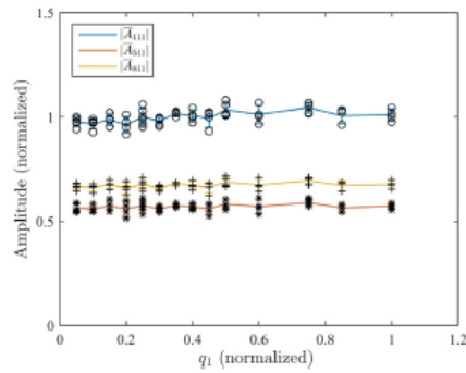
Fig. 24. Variation of modal constants corresponding to the 1st mode of the missile structure with modal response level.
