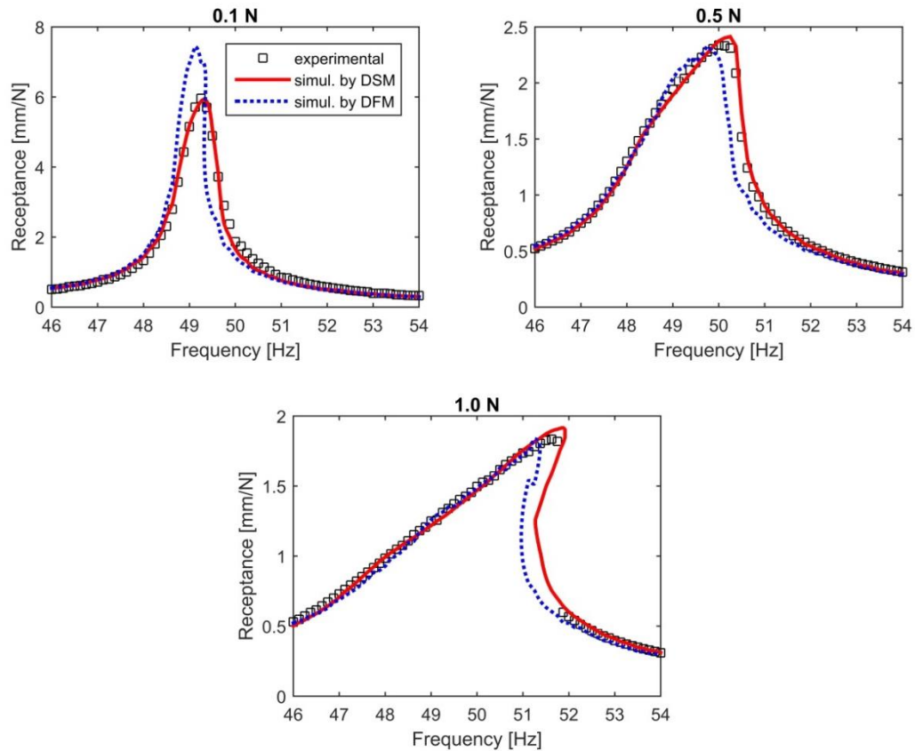
Figure 4-43. Comparison of the simulation results obtained by the DSM and the DFM with the experimental data of the T-beam obtained from force-controlled stepped-sine testing
