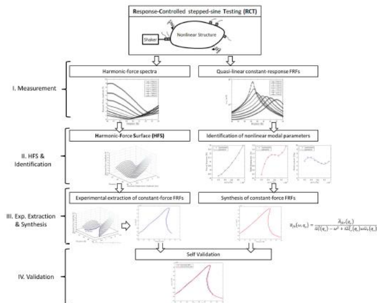
Figure 2. Experimental modal analysis with RCT and HFS.
