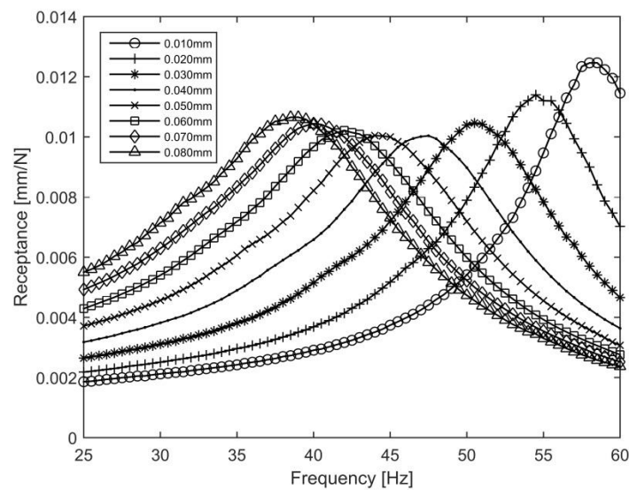
Figure 4-46. Receptances of the dummy mass on elastomeric vibration isolators measured by response-controlled stepped sine tests at various constant displacement amplitudes
