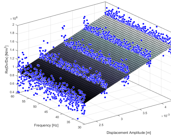
Figure 3-3. The real part of the partial derivative of the describing surface of nonlinearity of the SDOF system with cubic stiffness element
