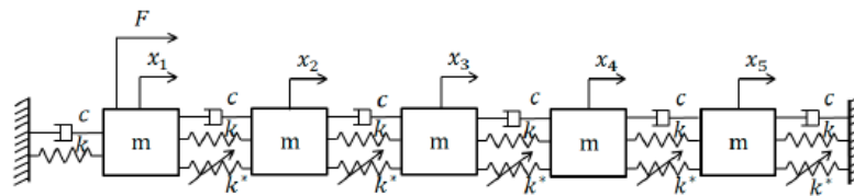
Figure 3. The 5 DOF system with cubic stiffness nonlinearity [16].
