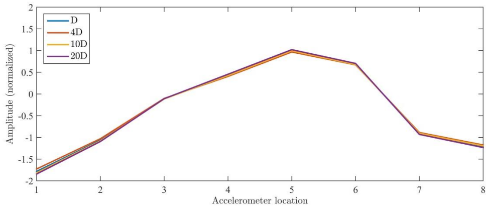
Figure 4-28. 1 st NNM of the missile structure experimentally extracted by using the modal constants identified from RCT
