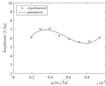
Fig. 16. Variation of the modal constant corresponding to the 1st mode of the T-beam with modal response level.
