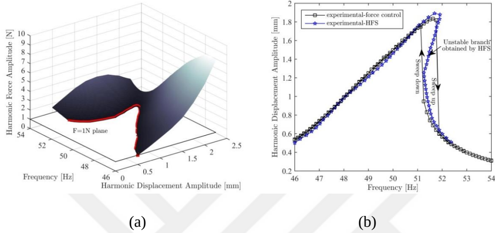
Figure 4-9. (a) Determination of the harmonic response spectrum with any existing unstable branch by cutting the HFS with a constant force plane (b) Comparison of the response spectrum obtained from the HFS with the one obtained by force-controlled testing
