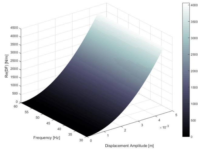
Figure 3-5. The real part of the describing surface of nonlinearity of the SDOF system with cubic stiffness element
