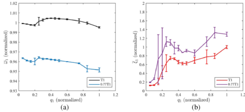
Fig. 27. Effect of bolt preload on the modal parameters (a) natural frequency (b) viscous modal damping ratio.
