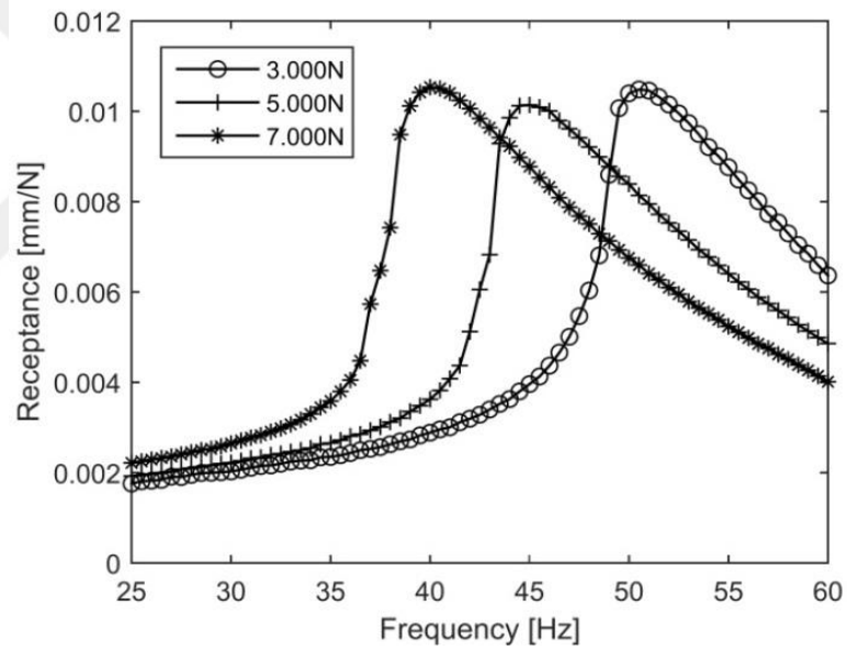
Figure 4-49. Receptance curves of the dummy mass on elastomeric vibration isolators measured by the force-controlled stepped sine tests at three different force amplitudes
