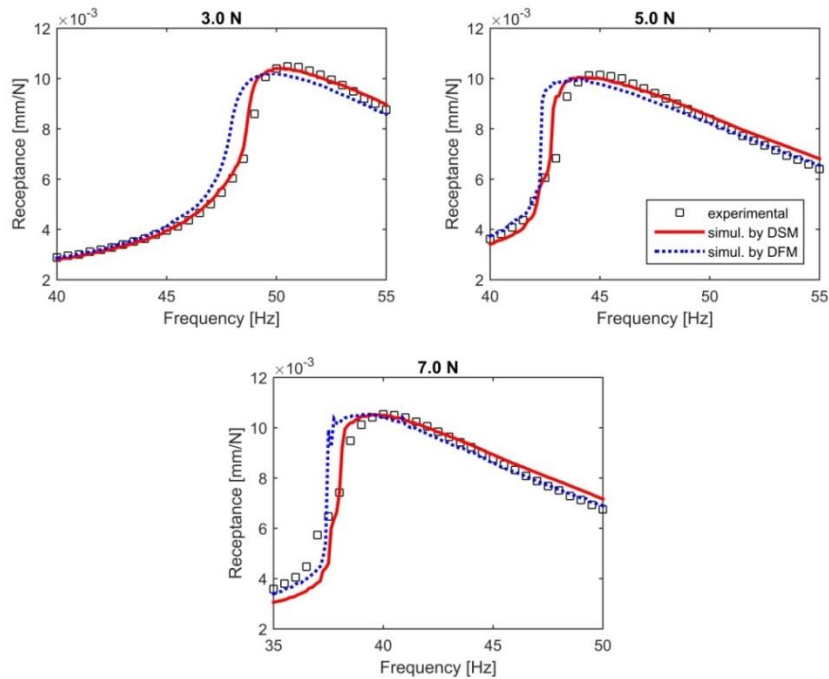
Figure 4-51. Comparison of the simulation results obtained by the DSM and the DFM, with the experimental data of the dummy mass on elastomeric vibration isolators obtained from force-controlled stepped-sine testing
