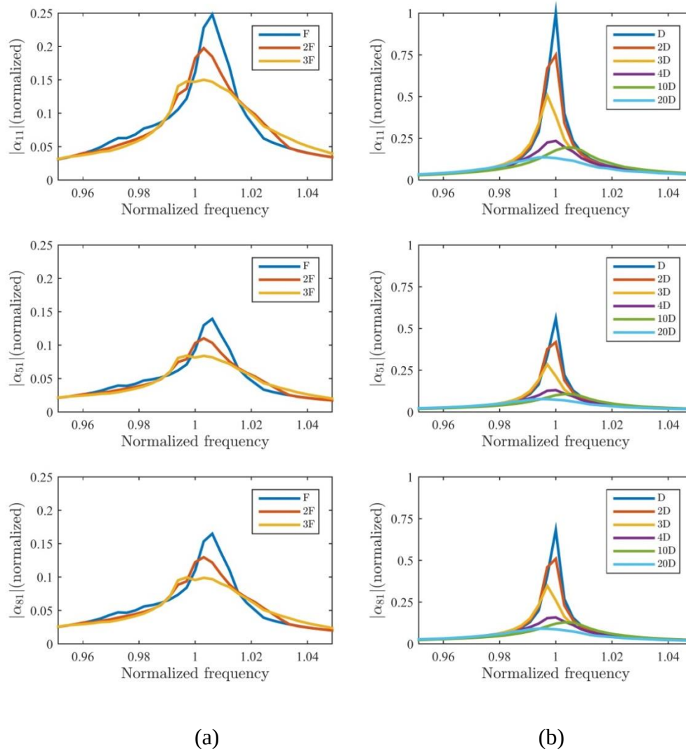
Figure 4-25. (a) Constant-force FRFs of the missile structure measured by the classical force-control approach (b) constant-response FRFs of the missile structure measured by the RCT approach
