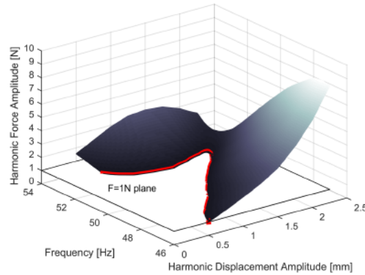
Fig. 2. Determination of the harmonic response spectrum with any existing unstable branch by cutting HFS with a constant force plane
