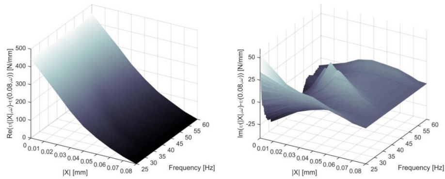
Figure 4-48. Real (left) and imaginary (right) parts of the relative describing surface of the nonlinearity of the elastomeric vibration isolators
