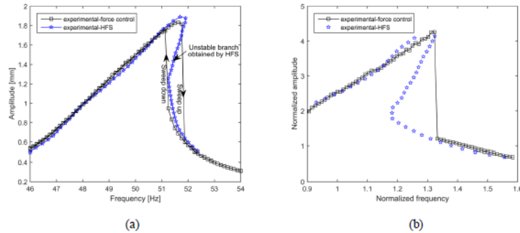
Fig. 3. Comparison of nonlinear frequency responses obtained by RCT with the ones measured by classical force-control test: (a) Bench mark test structure with cubic stiffness (b) Control fin actuation mechanism of a real missile
