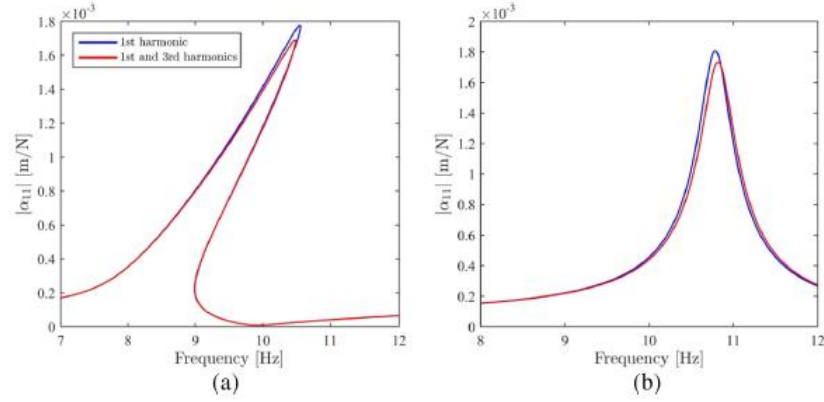
Fig. 2. Effect of the 3rd harmonic on the FRFs (a) constant-force driving point FRF at 50 N (b) constant-response driving point FRF at 0.10 m.
