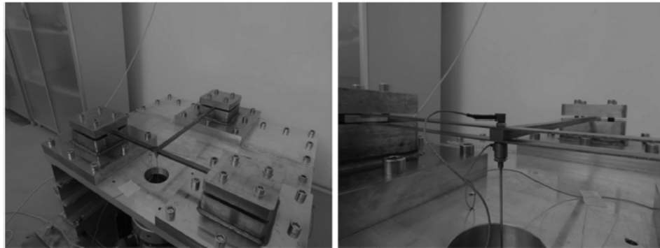
Fig. 1. T-beam experimental setup.
