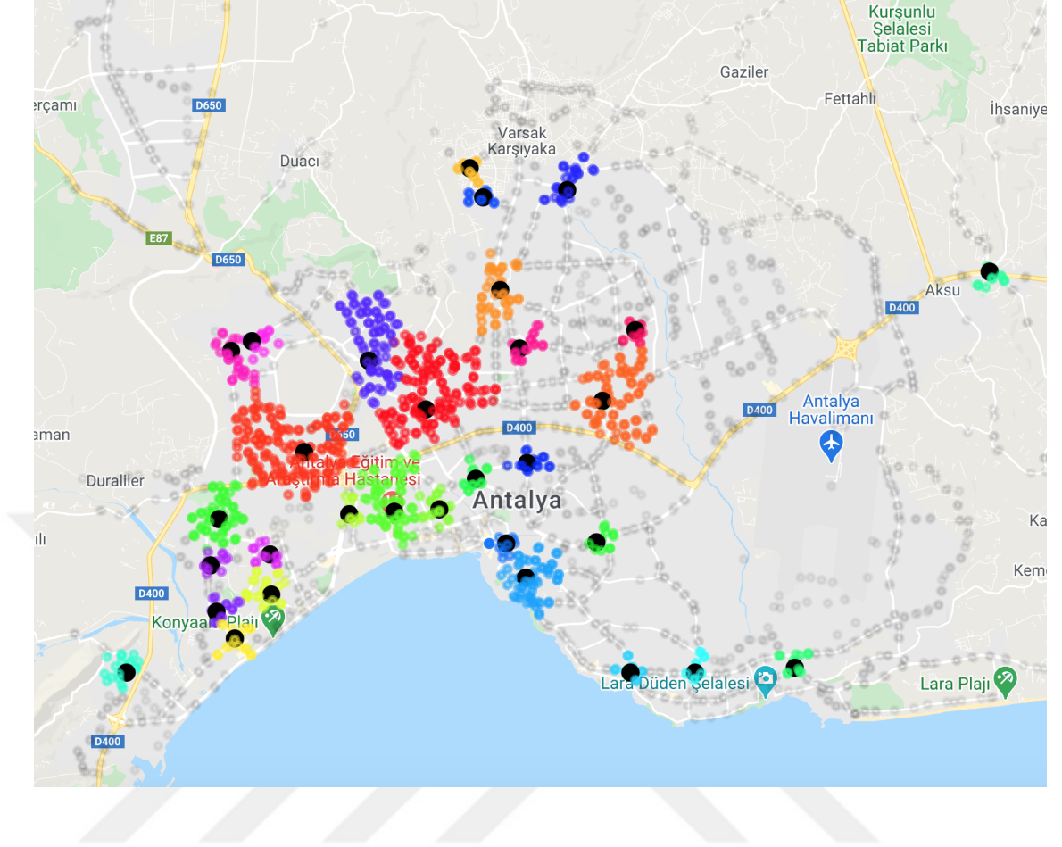
Figure 4.23. DBSCAN with MinPts = 12 and epsilon = 400
