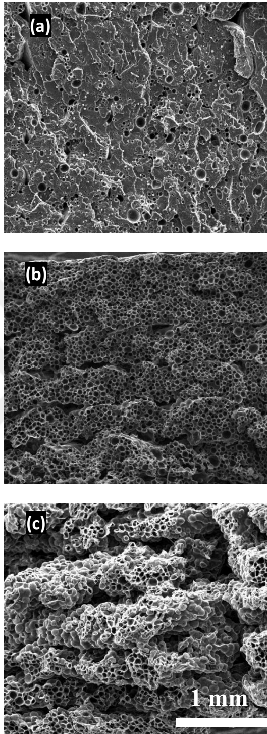
Figure 11. Cross-section SEM images of 3D-printed samples with a variable flow rate of (a) 100 %, (b) 50 %, (c) and 25 %.
