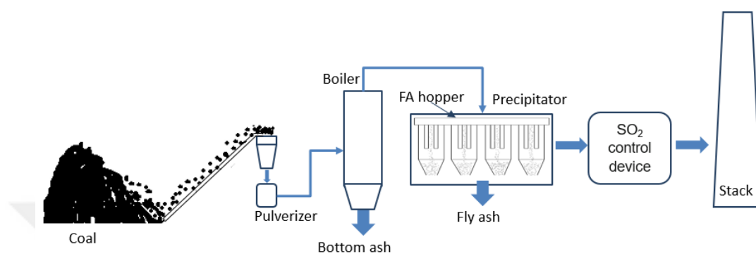
Figure 21. FA generation and collection in a pulverized coal-fired power plant (Adapted from (Chou 2012)).
