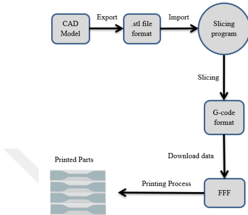
Figure 3. Data Processing in FFF.
